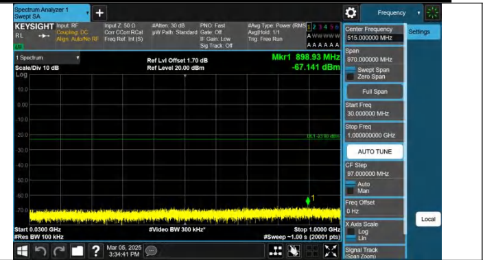
Band2-1.4MHz-QPSK-18900-1RB#5-30~1000-PASS
