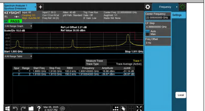
Band2-15MHz-QPSK-19125-1RB#74-PASS
