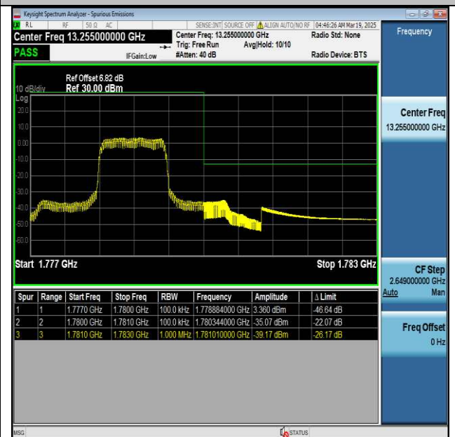
Band66_10MHz_QPSK_132622_6_High
