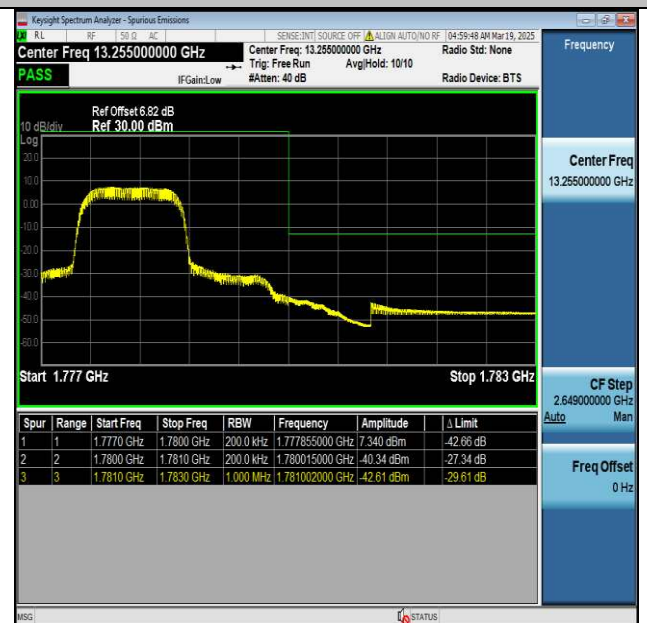
Band66_20MHz_QPSK_132572_6_High
