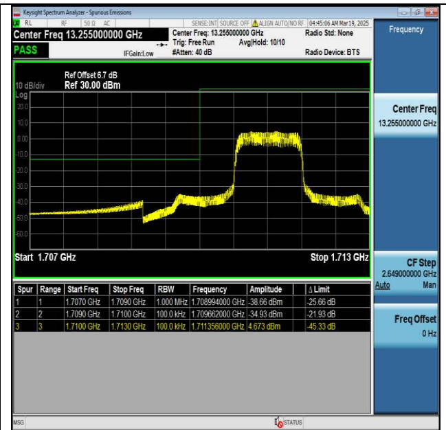
Band66_10MHz_QPSK_132022_6_Low
