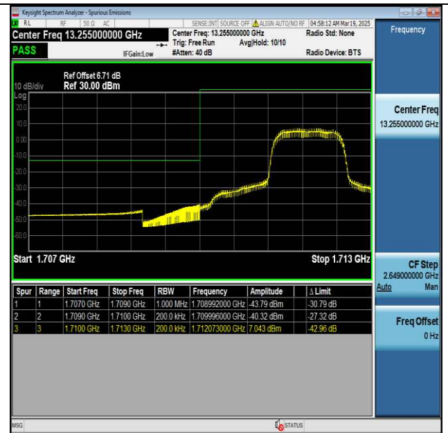
Band66_20MHz_QPSK_132072_6_Low
