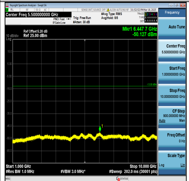
Band26(814-824)-10MHz-QPSK-26740-PASS_1_High
