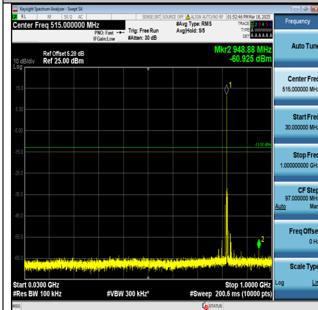
Band26(814-824)-10MHz-QPSK-26740-PASS_1_High
