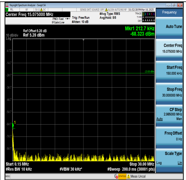
Band26(814-824)-10MHz-QPSK-26740-PASS_1_High
