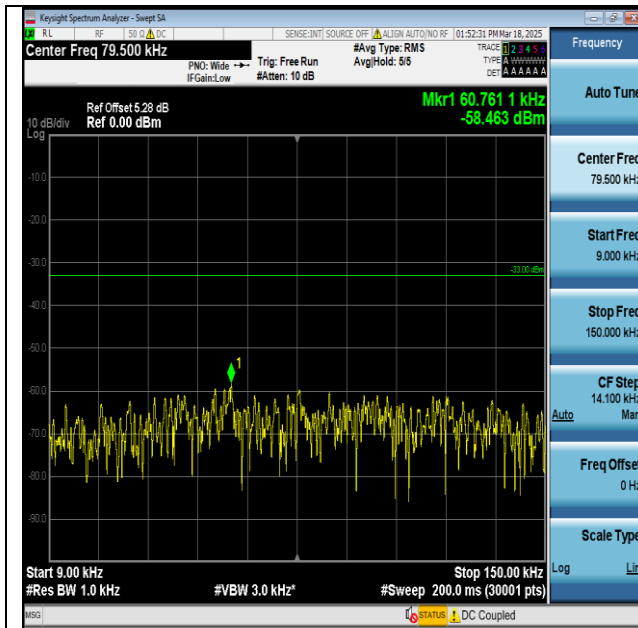
Band26(814-824)-10MHz-QPSK-26740-PASS_1_High
