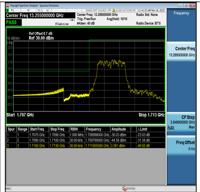
Band4_3MHz_QPSK_19965_6_Low
