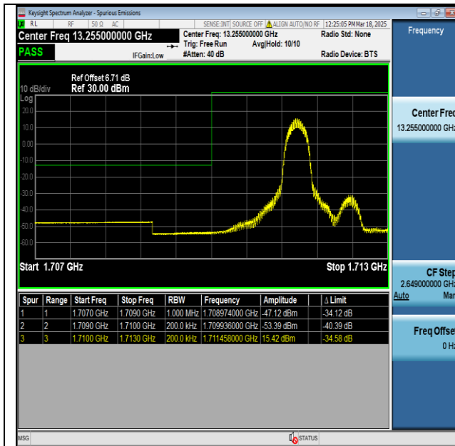
Band4_20MHz_QPSK_20050_1_Low
