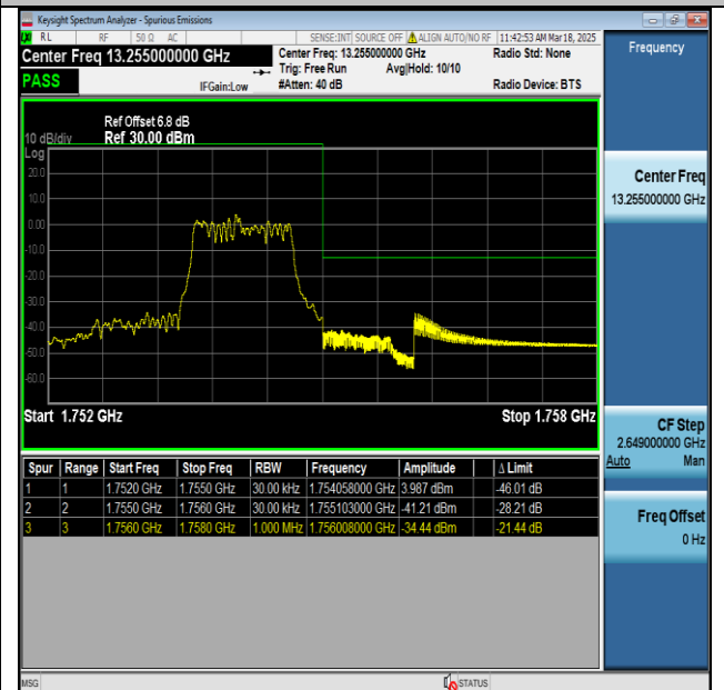
Band4_3MHz_QPSK_20385_6_High
