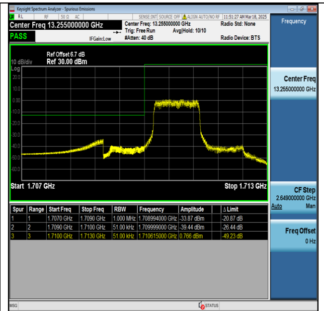
Band4_5MHz_QPSK_19975_6_Low
