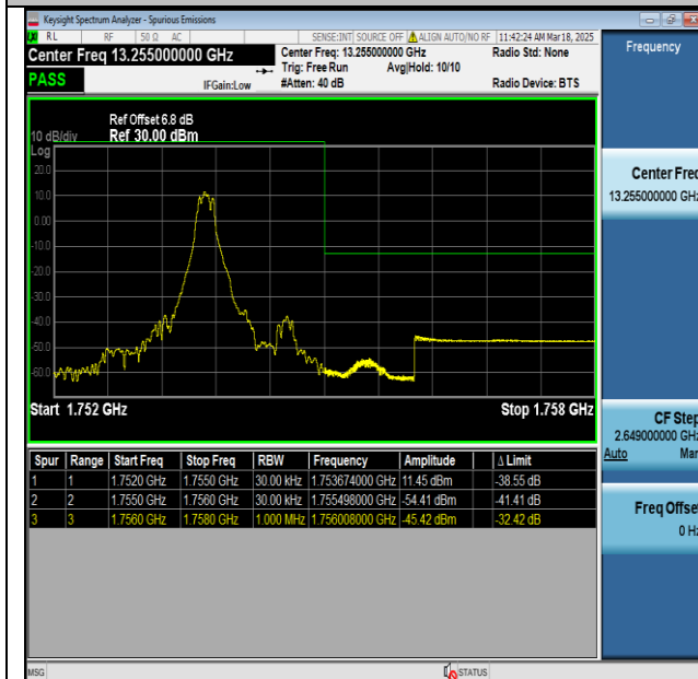
Band4_3MHz_QPSK_20385_1_High
