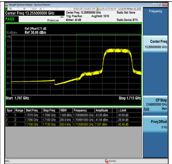
Band4_20MHz_QPSK_20050_6_Low
