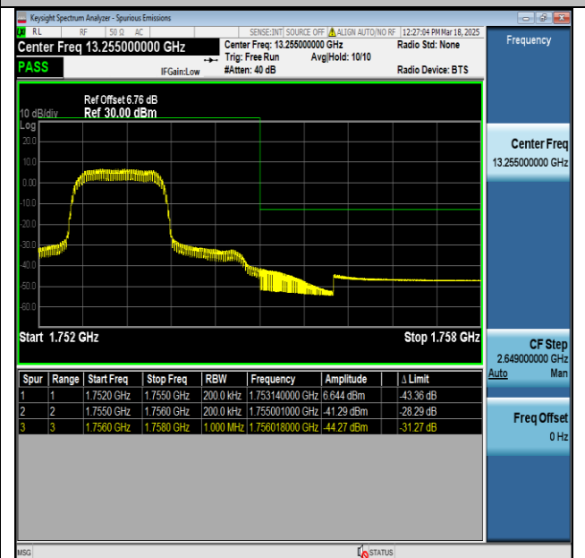
Band4_20MHz_QPSK_20300_6_High
