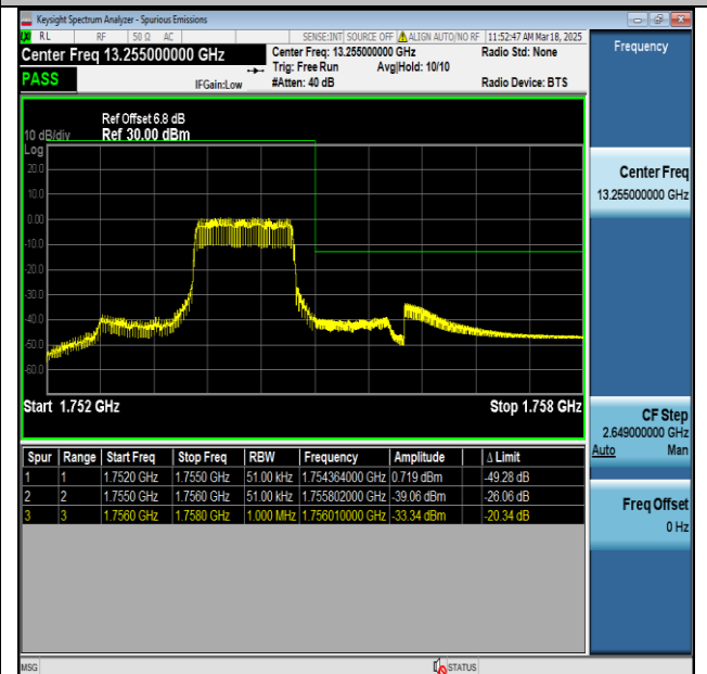
Band4_5MHz_QPSK_20375_6_High
