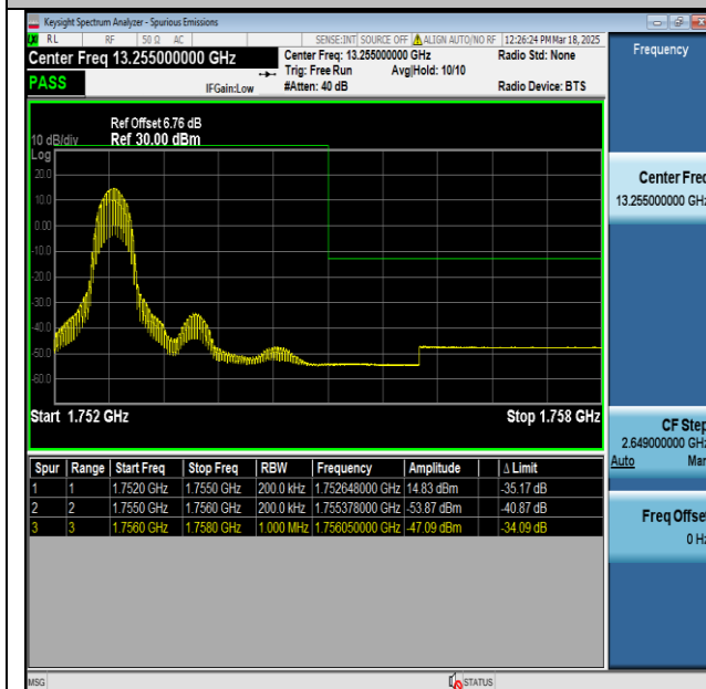
Band4_20MHz_QPSK_20300_1_High
