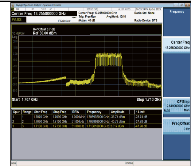
Band4_5MHz_QPSK_19975_6_Low
