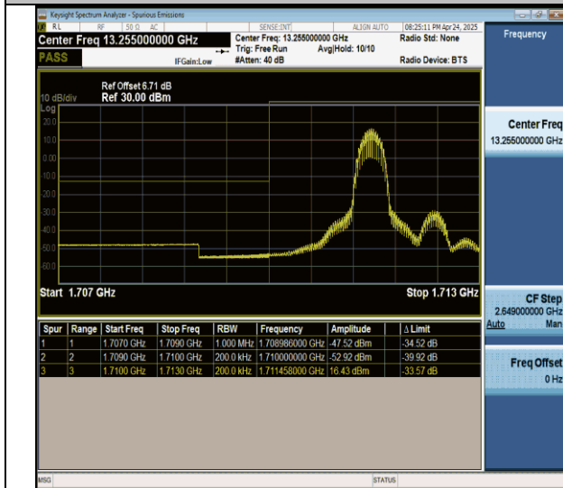
Band4_20MHz_QPSK_20050_1_Low
