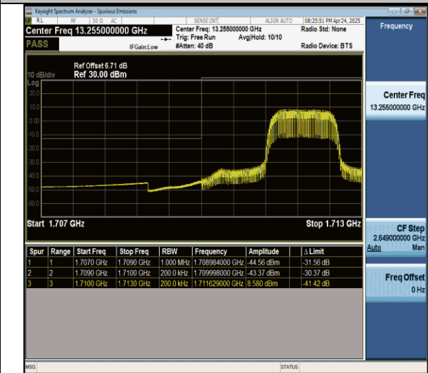
Band4_20MHz_QPSK_20050_6_Low
