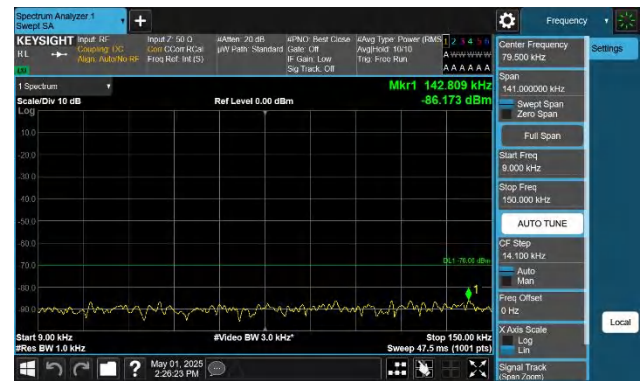
Band48-5MHz-QPSK-55990-1RB#24-0.009~0.15-PASS
