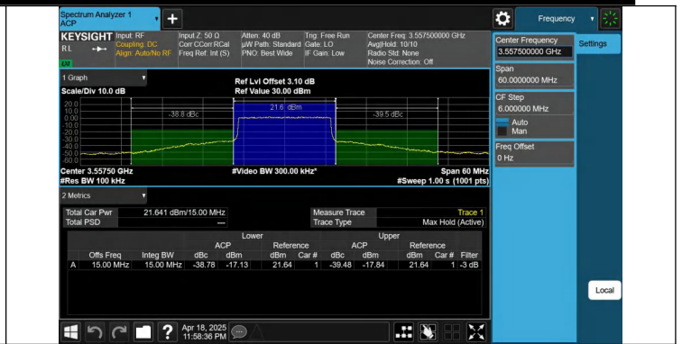
Band48-15MHz-64QAM-55315-75RB#0-PASS
