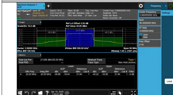
Band48-20MHz-64QAM-55340-1RB#0-PASS
