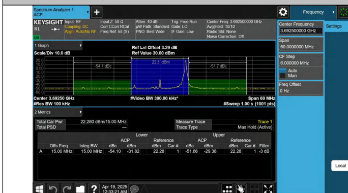
Band48-15MHz-64QAM-56665-1RB#74-PASS
