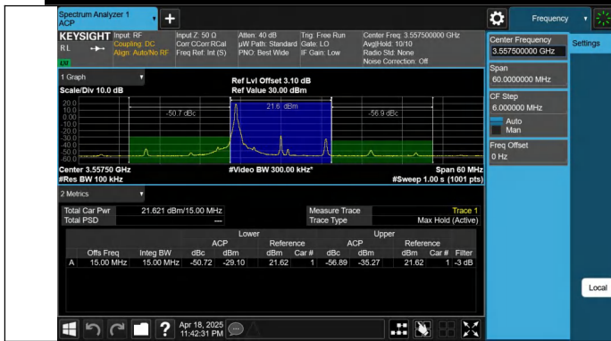
Band48-15MHz-16QAM-55315-1RB#0-PASS
