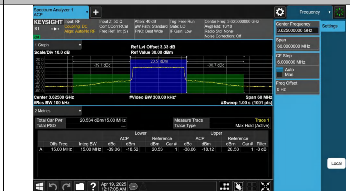
Band48-15MHz-16QAM-55990-1RB#74-PASS
