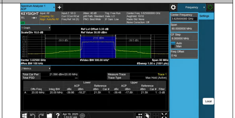
Band48-20MHz-64QAM-55990-1RB#0-PASS
