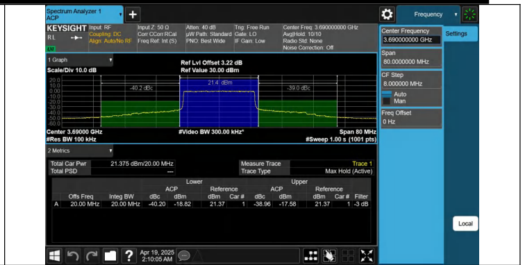
Band48-20MHz-QPSK-56640-100RB#0-PASS
