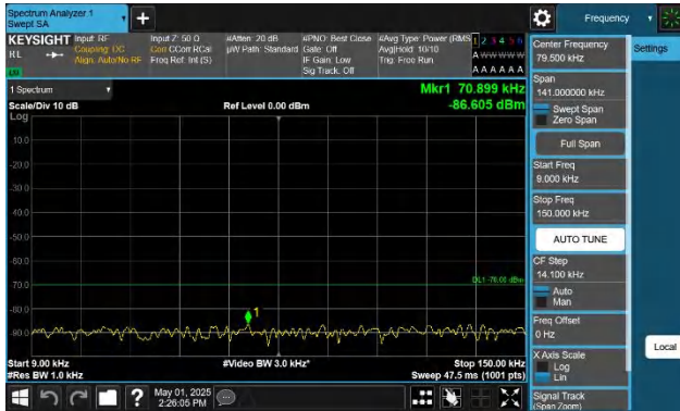
Band48-5MHz-QPSK-55265-1RB#0-0.009~0.15-PASS
