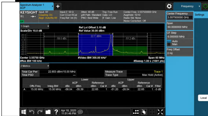
Band48-15MHz-64QAM-55315-1RB#74-PASS
