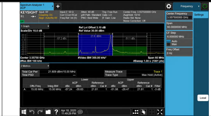
Band48-15MHz-16QAM-55315-1RB#74-PASS
