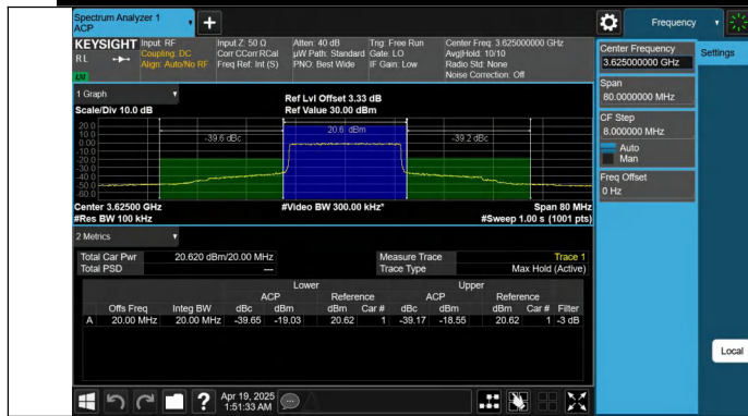
Band48-20MHz-16QAM-55990-100RB#0-PASS
