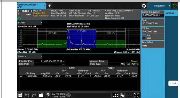
Band48-15MHz-16QAM-55315-75RB#74-PASS
