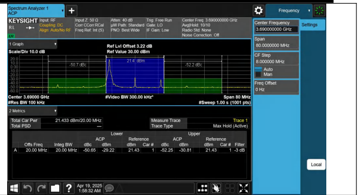
Band48-20MHz-16QAM-56640-1RB#0-PASS
