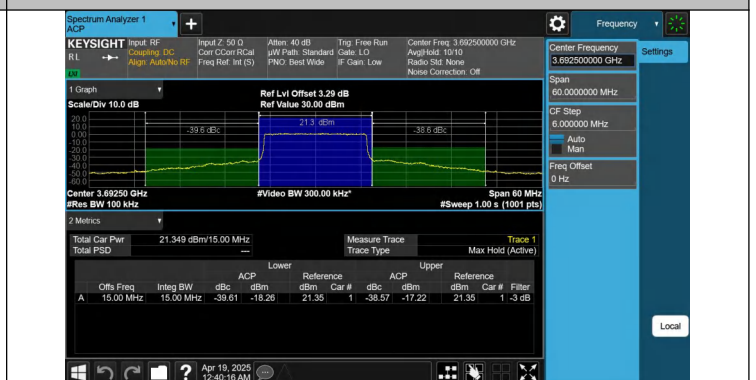
Band48-15MHz-64QAM-56665-75RB#0-PASS
