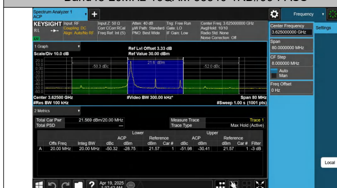
Band48-20MHz-16QAM-55990-1RB#0-PASS
