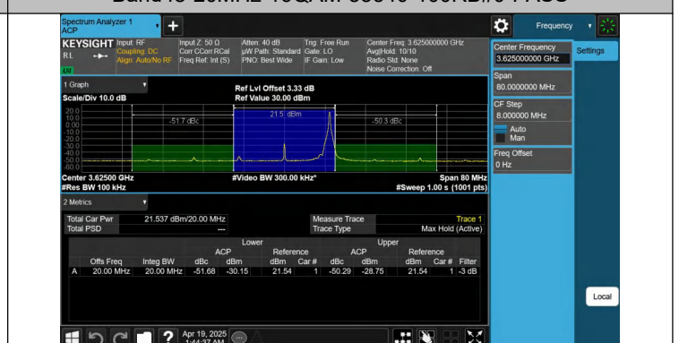
Band48-20MHz-16QAM-55990-1RB#99-PASS
