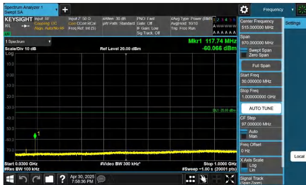
41-41-20MHz-10MHz-QPSK-QPSK-41391-41535-1RB#99-ORB# 0-30~1000MHz-PASS
