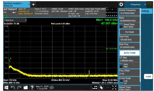
41-41-20MHz-15MHz-QPSK-QPSK-40546-40717-1RB#99-ORB#0 -0.15~30MHz-PASS
