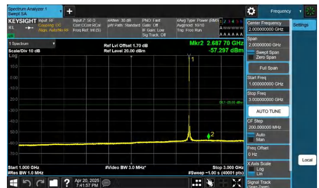
41-41-20MHz-15MHz-QPSK-QPSK-39750-39921-1RB#99-0RB#0 -1000~3000MHz-PASS
