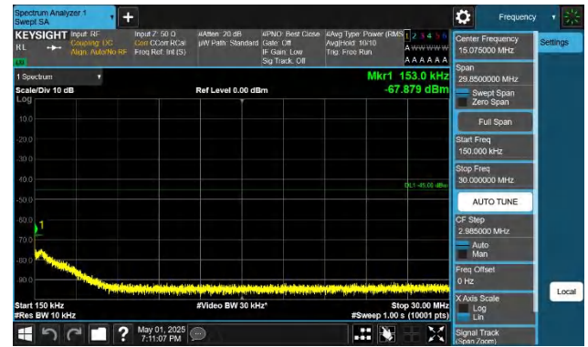
41-41-20MHz-15MHz-QPSK-QPSK-39750-39921-1RB#99-0RB#0 -0.15~30MHz-PASS
