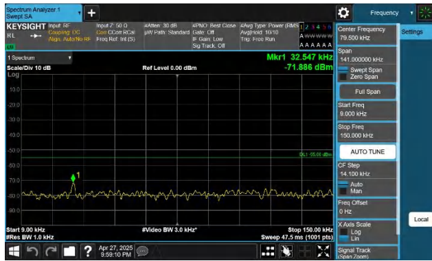
41-41-20MHz-15MHz-QPSK-QPSK-40546-40717-1RB#0-0RB#0 -0.009~0.15MHz-PASS
