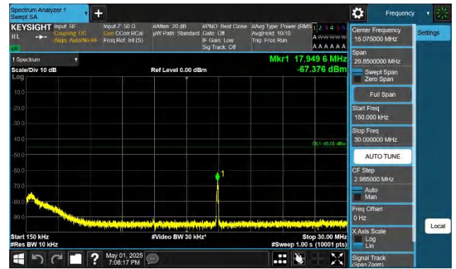
41-41-20MHz-10MHz-QPSK-QPSK-40571-40715-1RB#0-1RB#49 -0.15~30MHz-PASS
