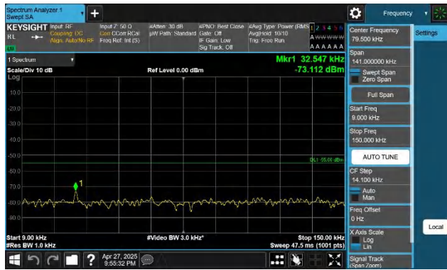
41-41-20MHz-10MHz-QPSK-QPSK-41391-41535-1RB#0-1RB#4 9-0.009~0.15MHz-PASS
