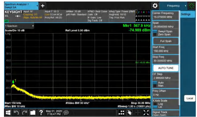
41-41-20MHz-20MHz-QPSK-QPSK-40521-40719-1RB#0-0RB#0 0.15~30MHz-PASS
