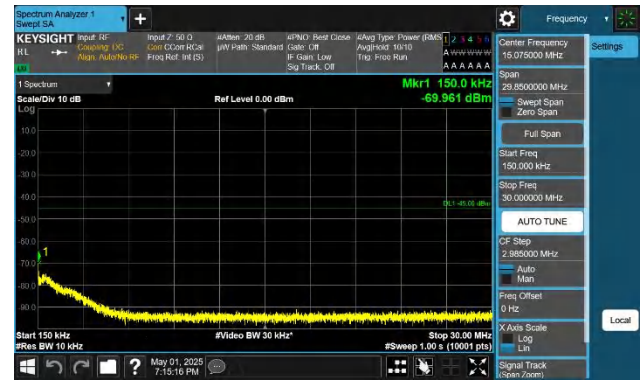
41-41-20MHz-20MHz-QPSK-QPSK-39750-39948-1RB#0-0RB#0 0.15~30MHz-PASS
