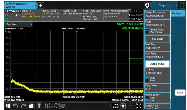
41-41-20MHz-15MHz-QPSK-QPSK-41341-41512-1RB#0-0RB#0 0.15~30MHz-PASS
