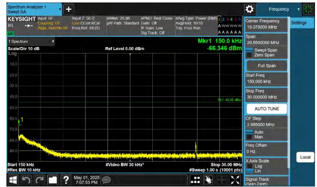
41-41-20MHz-10MHz-QPSK-QPSK-40571-40715-1RB#99-ORB#0 -0.15~30MHz-PASS
