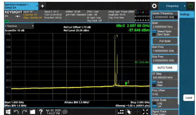
41-41-20MHz-15MHz-QPSK-QPSK-39750-39921-1RB#0-1RB#74 -1000~3000MHz-PASS
