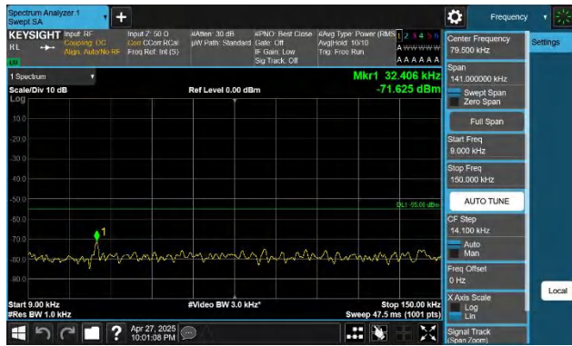
41-41-20MHz-15MHz-QPSK-QPSK-41341-41512-1RB#0-0RB#0 -0.009~0.15MHz-PASS
