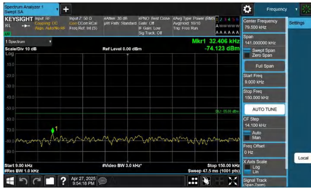
41-41-20MHz-10MHz-QPSK-QPSK-41391-41535-1RB#0-0RB#0 -0.009~0.15MHz-PASS
