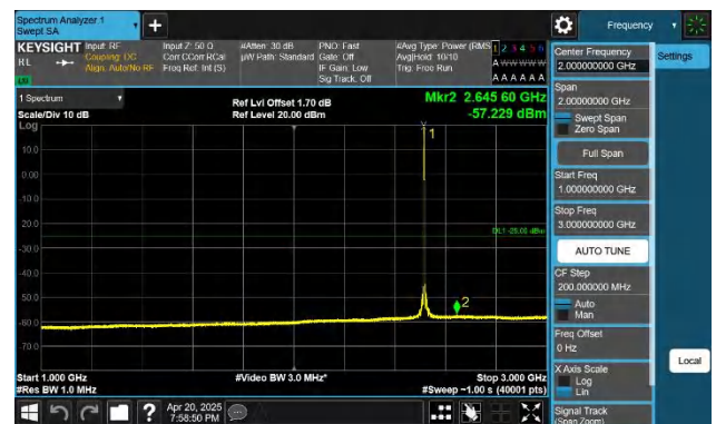
41-41-20MHz-20MHz-QPSK-QPSK-39750-39948-1RB#99-ORB#0 -1000~3000MHz-PASS
