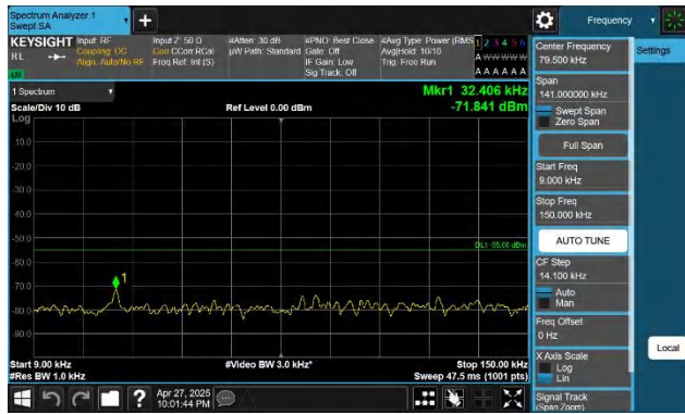
41-41-20MHz-15MHz-QPSK-QPSK-41341-41512-1RB#99-0RB# 0-0.009~0.15MHz-PASS
