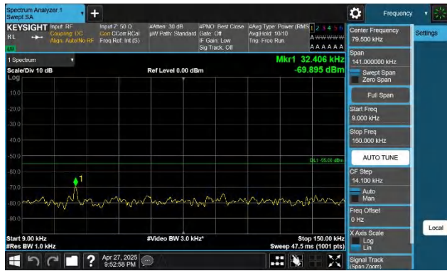
41-41-20MHz-10MHz-QPSK-QPSK-40571-40715-1RB#99-ORB# 0-0.009~0.15MHz-PASS
