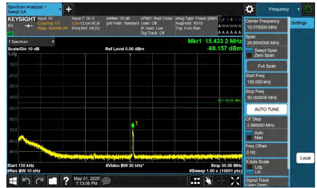
41-41-20MHz-15MHz-QPSK-QPSK-40546-40717-1RB#0-1RB#74 -0.15~30MHz-PASS
