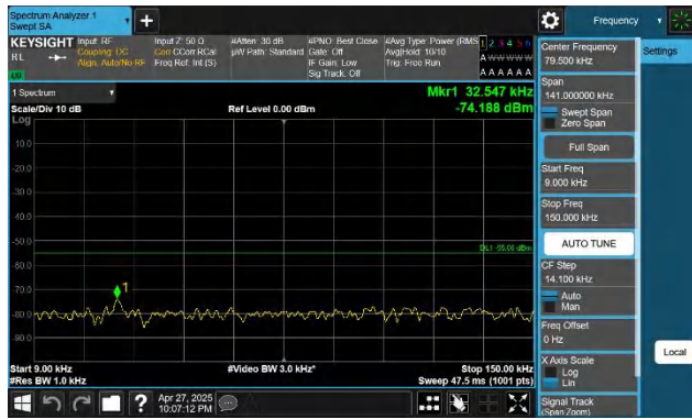
41-41-20MHz-20MHz-QPSK-QPSK-40521-40719-1RB#0-1RB#9 9-0.009~0.15MHz-PASS
