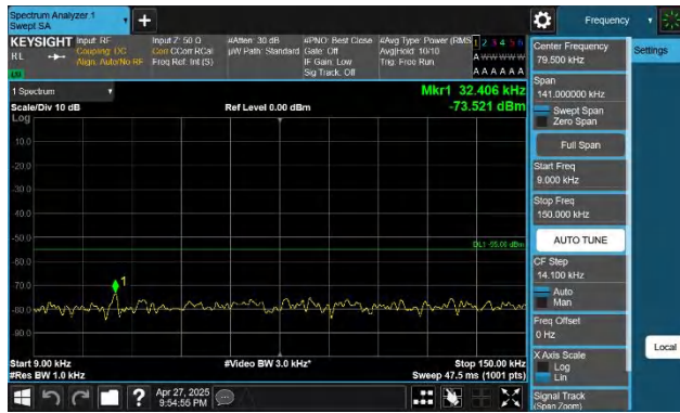
41-41-20MHz-10MHz-QPSK-QPSK-41391-41535-1RB#99-ORB# 0-0.009~0.15MHz-PASS
