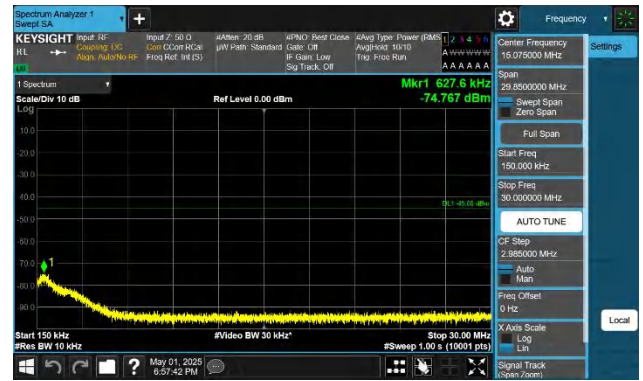
41-41-15MHz-20MHz-QPSK-QPSK-40523-40694-1RB#74-0RB#0 -0.15~30MHz-PASS
