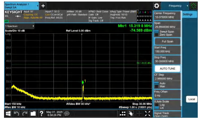
41-41-15MHz-20MHz-QPSK-QPSK-40523-40694-1RB#0-1RB#99 -0.15~30MHz-PASS
