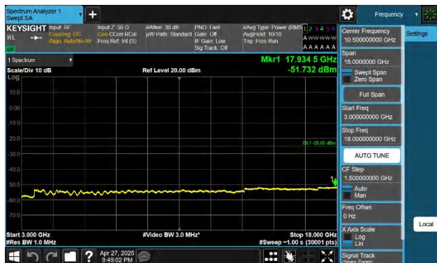
41-41-20MHz-5MHz-QPSK-QPSK-41440-41557-1RB#99-0RB#0 -3000~18000MHz-PASS
