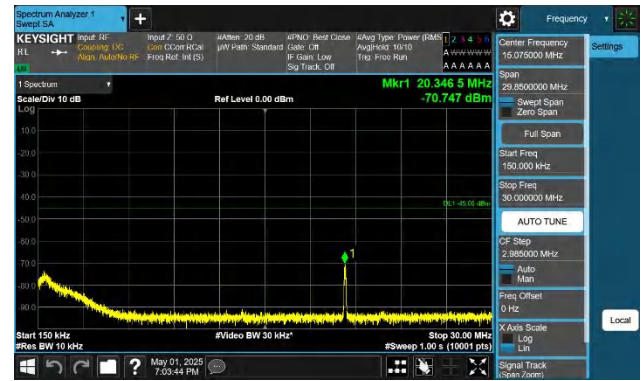
41-41-20MHz-5MHz-QPSK-QPSK-40595-40712-1RB#0-1RB#24- 0.15~30MHz-PASS
