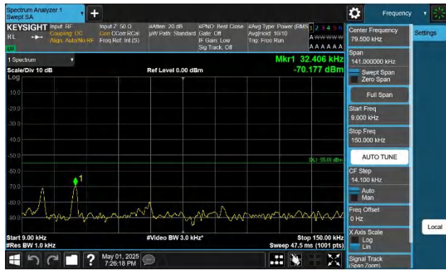
41-41-15MHz-20MHz-QPSK-QPSK-39728-39899-1RB#0-1RB#9 9-0.009~0.15MHz-PASS
