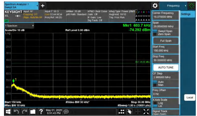
41-41-15MHz-20MHz-QPSK-QPSK-39728-39899-1RB#0-1RB#99 -0.15~30MHz-PASS
