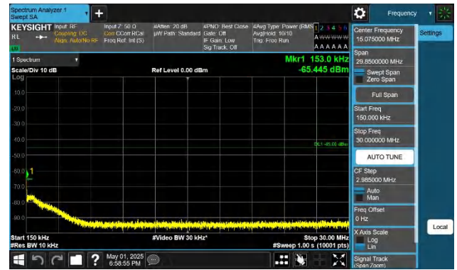
41-41-15MHz-20MHz-QPSK-QPSK-41319-41490-1RB#0-0RB#0 0.15~30MHz-PASS
