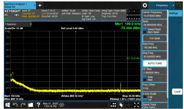
41-41-20MHz-5MHz-QPSK-QPSK-40595-40712-1RB#99-0RB#0 0.15~30MHz-PASS
