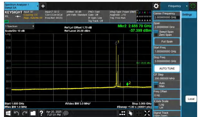
41-41-20MHz-10MHz-QPSK-QPSK-39750-39894-1RB#0-1RB#49 -1000~3000MHz-PASS
