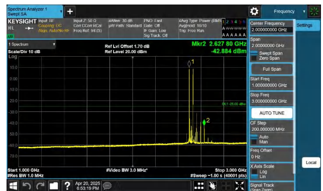
41-41-15MHz-20MHz-QPSK-QPSK-39728-39899-1RB#0-1RB#99 -1000~3000MHz-PASS
