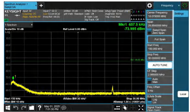
41-41-20MHz-5MHz-QPSK-QPSK-39750-39867-1RB#0-1RB#24- 0.15~30MHz-PASS
