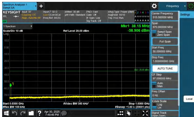
41-41-20MHz-5MHz-QPSK-QPSK-40595-40712-1RB#99-0RB#0 -30~1000MHz-PASS
