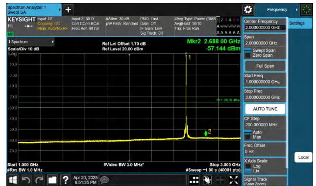
41-41-15MHz-20MHz-QPSK-QPSK-39728-39899-1RB#74-0RB#0 -1000~3000MHz-PASS
