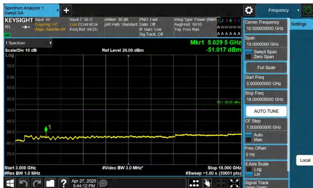
41-41-20MHz-5MHz-QPSK-QPSK-39750-39867-1RB#99-0RB#0 -3000~18000MHz-PASS
