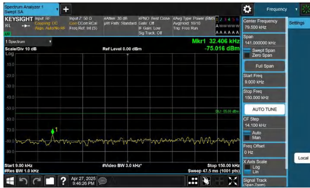
41-41-20MHz-5MHz-QPSK-QPSK-40595-40712-1RB#0-1RB#24 -0.009~0.15MHz-PASS
