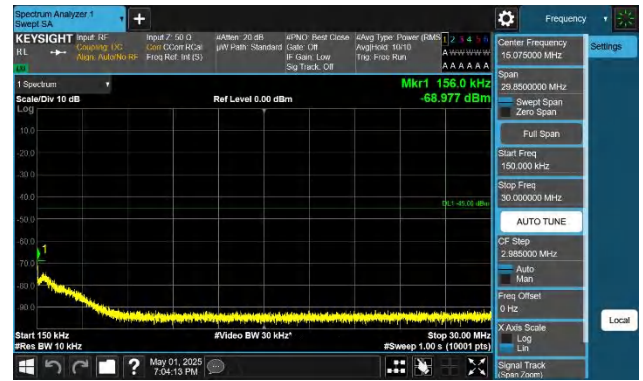
41-41-20MHz-5MHz-QPSK-QPSK-41440-41557-1RB#0-0RB#0-0. 15~30MHz-PASS
