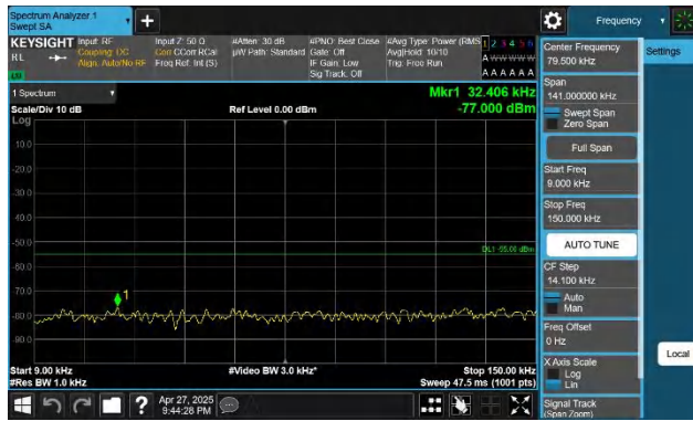
41-41-20MHz-5MHz-QPSK-QPSK-39750-39867-1RB#0-1RB#24 -0.009~0.15MHz-PASS
