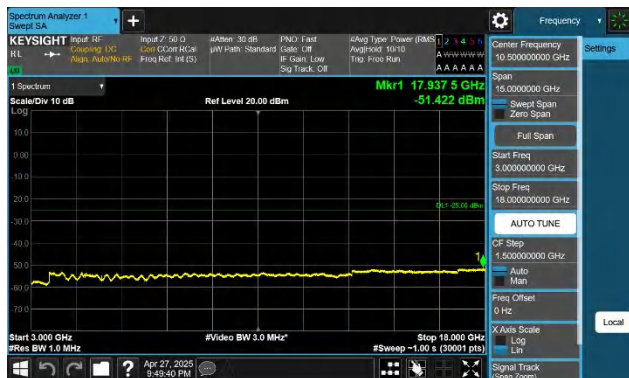
41-41-20MHz-5MHz-QPSK-QPSK-41440-41557-1RB#0-1RB#24 -3000~18000MHz-PASS
