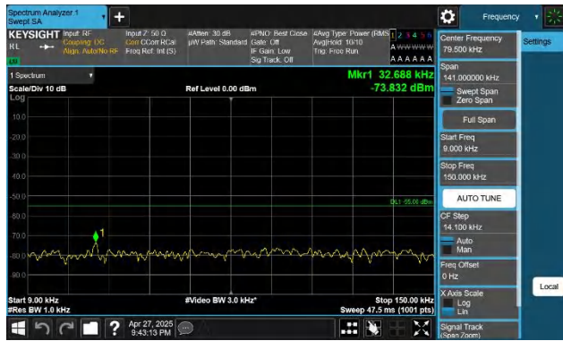
41-41-20MHz-5MHz-QPSK-QPSK-39750-39867-1RB#0-0RB#0- 0.009~0.15MHz-PASS
