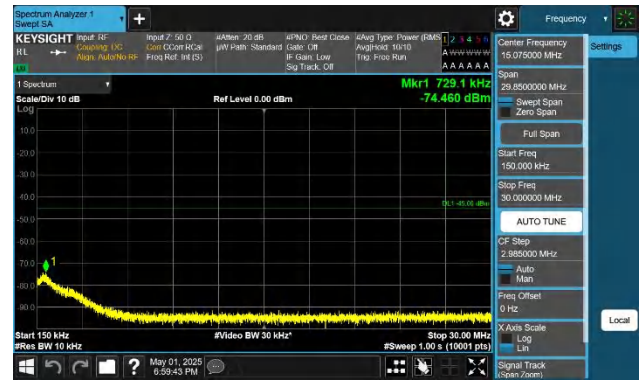
41-41-15MHz-20MHz-QPSK-QPSK-41319-41490-1RB#0-1RB#99 -0.15~30MHz-PASS
