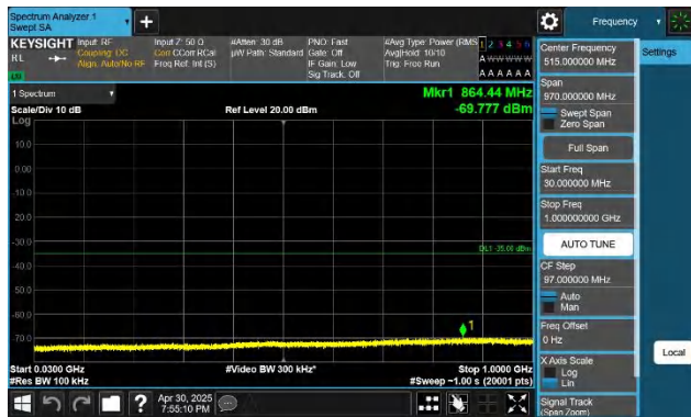
41-41-20MHz-10MHz-QPSK-QPSK-39750-39894-1RB#0-1RB#4 9-30~1000MHz-PASS
