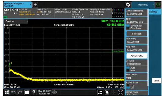
41-41-20MHz-5MHz-QPSK-QPSK-41440-41557-1RB#99-0RB#0- 0.15~30MHz-PASS
