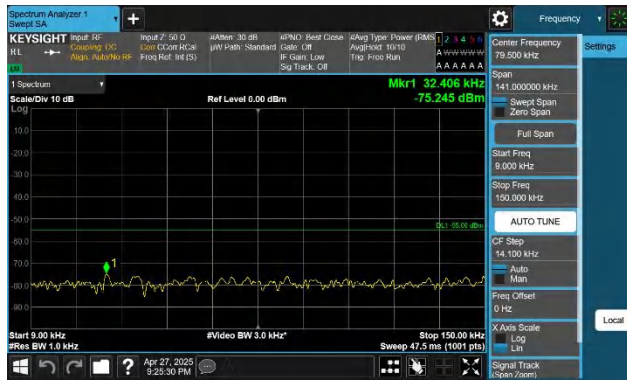
41-41-15MHz-10MHz-QPSK-QPSK-40571-40691-1RB#0-0RB#0 -0.009~0.15MHz-PASS
