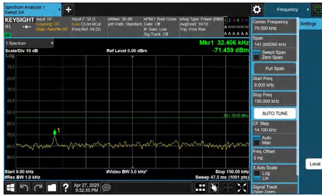
41-41-15MHz-15MHz-QPSK-QPSK-40545-40695-1RB#74-0RB# 0-0.009~0.15MHz-PASS
