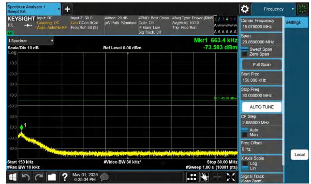
41-41-15MHz-10MHz-QPSK-QPSK-40571-40691-1RB#0-0RB#0 0.15~30MHz-PASS
