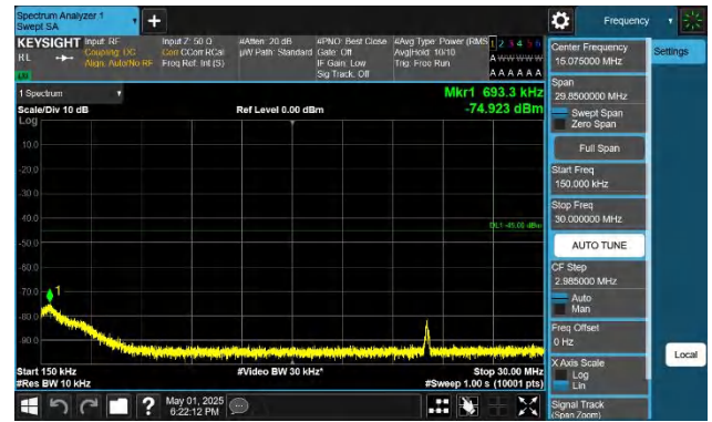
41-41-15MHz-10MHz-QPSK-QPSK-39725-39845-1RB#0-1RB#49 -0.15~30MHz-PASS
