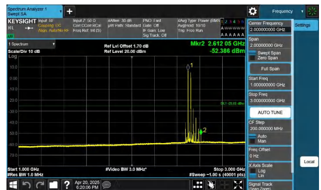
41-41-15MHz-10MHz-QPSK-QPSK-39725-39845-1RB#0-1RB#49 -1000~3000MHz-PASS
