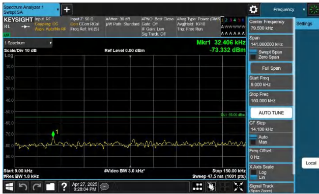
41-41-15MHz-10MHz-QPSK-QPSK-41417-41537-1RB#74-0RB# 0-0.009~0.15MHz-PASS
