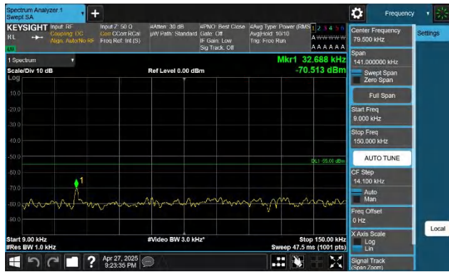
41-41-15MHz-10MHz-QPSK-QPSK-39725-39845-1RB#0-0RB#0 -0.009~0.15MHz-PASS
