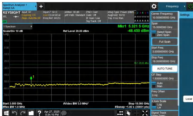
41-41-15MHz-15MHz-QPSK-QPSK-41365-41515-1RB#0-0RB#0 -3000~18000MHz-PASS
