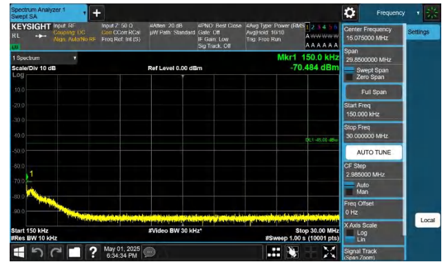
41-41-15MHz-15MHz-QPSK-QPSK-41365-41515-1RB#0-0RB#0 0.15~30MHz-PASS
