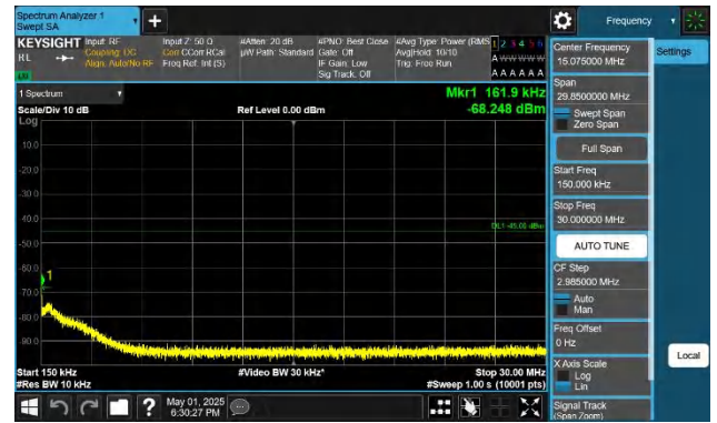
41-41-15MHz-15MHz-QPSK-QPSK-39725-39875-1RB#0-0RB#0 0.15~30MHz-PASS
