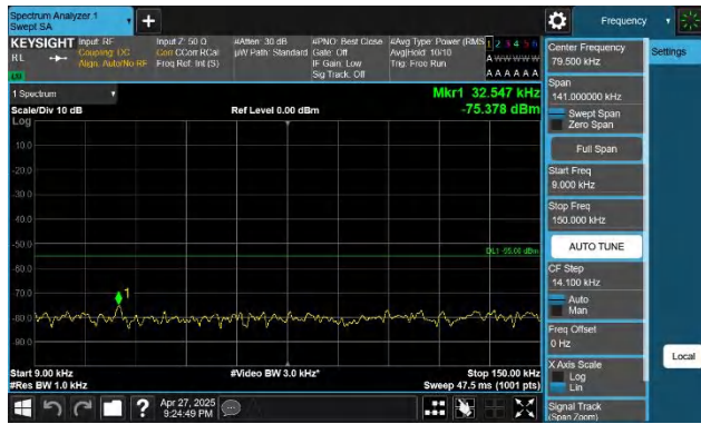
41-41-15MHz-10MHz-QPSK-QPSK-39725-39845-1RB#0-1RB#4 9-0.009~0.15MHz-PASS
