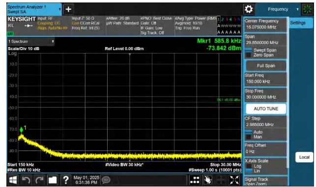
41-41-15MHz-15MHz-QPSK-QPSK-39725-39875-1RB#0-1RB#74 -0.15~30MHz-PASS
