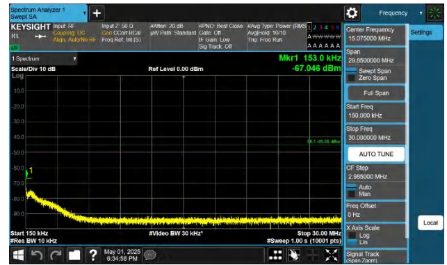
41-41-15MHz-15MHz-QPSK-QPSK-41365-41515-1RB#74-0RB#0 -0.15~30MHz-PASS
