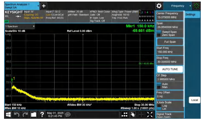
41-41-15MHz-10MHz-QPSK-QPSK-39725-39845-1RB#74-0RB#0 -0.15~30MHz-PASS
