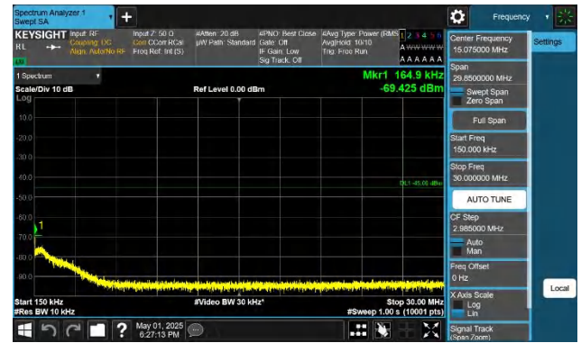
41-41-15MHz-10MHz-QPSK-QPSK-41417-41537-1RB#0-0RB#0 0.15~30MHz-PASS
