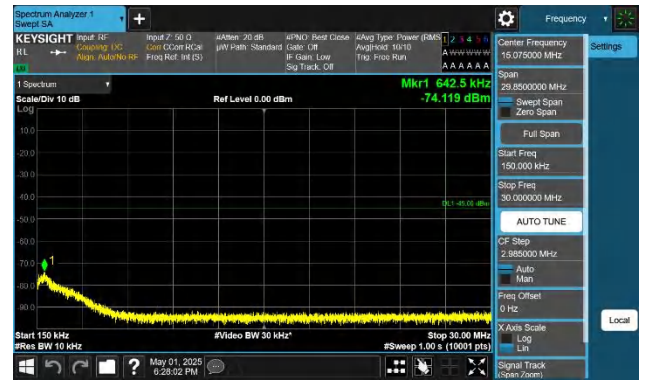
41-41-15MHz-10MHz-QPSK-QPSK-41417-41537-1RB#0-1RB#49 -0.15~30MHz-PASS
