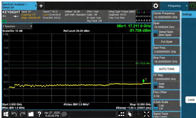
41-41-15MHz-10MHz-QPSK-QPSK-41417-41537-1RB#74-0RB# 0-3000~18000MHz-PASS
