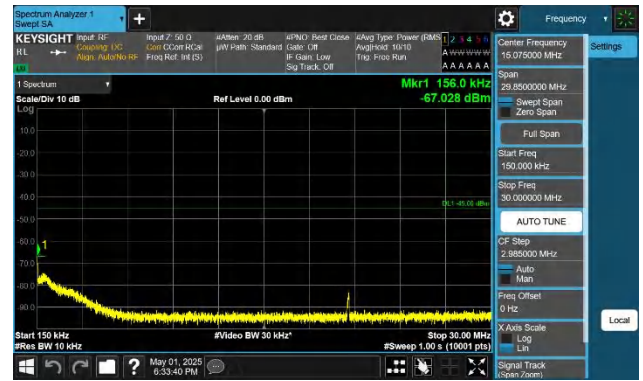
41-41-15MHz-15MHz-QPSK-QPSK-40545-40695-1RB#74-0RB#0 -0.15~30MHz-PASS
