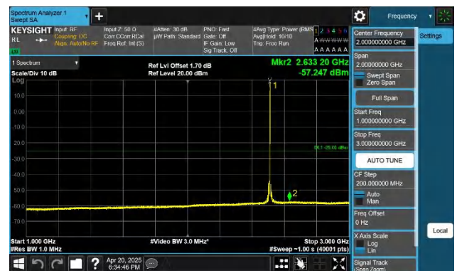
41-41-15MHz-15MHz-QPSK-QPSK-39725-39875-1RB#74-0RB#0 -1000~3000MHz-PASS
