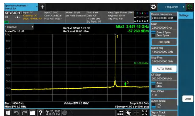
41-41-15MHz-10MHz-QPSK-QPSK-39725-39845-1RB#74-0RB#0 -1000~3000MHz-PASS
