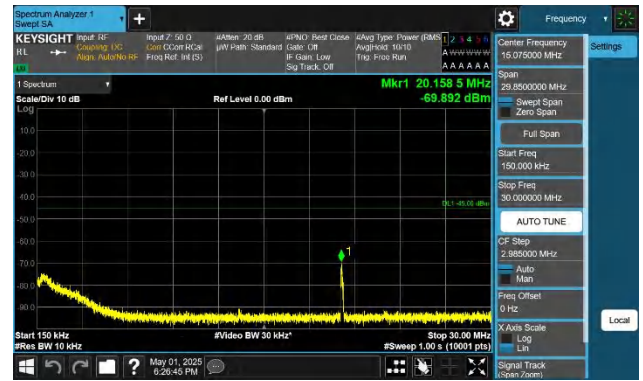
41-41-15MHz-10MHz-QPSK-QPSK-40571-40691-1RB#0-1RB#49 -0.15~30MHz-PASS
