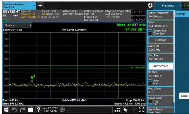
41-41-5MHz-20MHz-QPSK-QPSK-41373-41490-1RB#24-0RB#0 -0.009~0.15MHz-PASS
