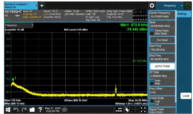
41-41-10MHz-15MHz-QPSK-QPSK-39703-39823-1RB#0-1RB#74 -0.15~30MHz-PASS
