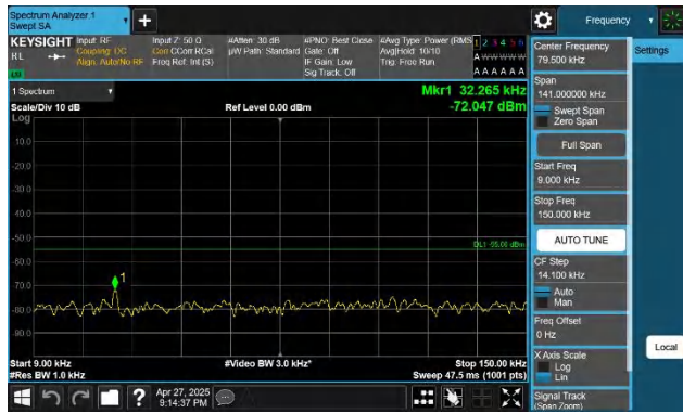
41-41-10MHz-15MHz-QPSK-QPSK-41395-41515-1RB#0-0RB#0 -0.009~0.15MHz-PASS
