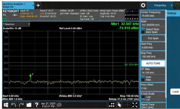
41-41-10MHz-20MHz-QPSK-QPSK-40526-40670-1RB#0-1RB#9 9-0.009~0.15MHz-PASS
