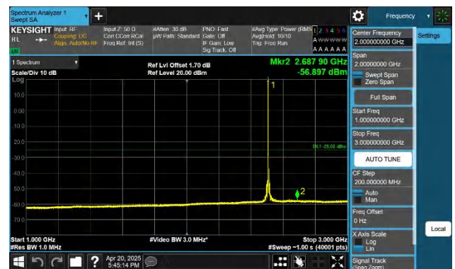
41-41-10MHz-15MHz-QPSK-QPSK-39703-39823-1RB#49-ORB#0 -1000~3000MHz-PASS
