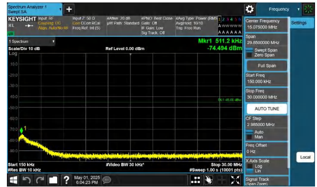
41-41-10MHz-15MHz-QPSK-QPSK-40549-40669-1RB#0-0RB#0 0.15~30MHz-PASS
