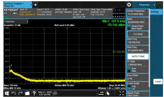
41-41-10MHz-15MHz-QPSK-QPSK-41395-41515-1RB#49-ORB#0 -0.15~30MHz-PASS
