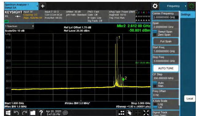
41-41-10MHz-15MHz-QPSK-QPSK-39703-39823-1RB#0-1RB#74 -1000~3000MHz-PASS
