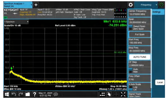
41-41-10MHz-15MHz-QPSK-QPSK-41395-41515-1RB#0-1RB#74 -0.15~30MHz-PASS
