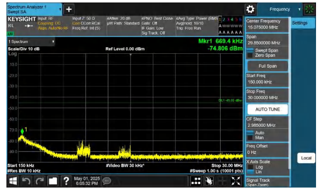
41-41-10MHz-15MHz-QPSK-QPSK-40549-40669-1RB#49-ORB#0 -0.15~30MHz-PASS
