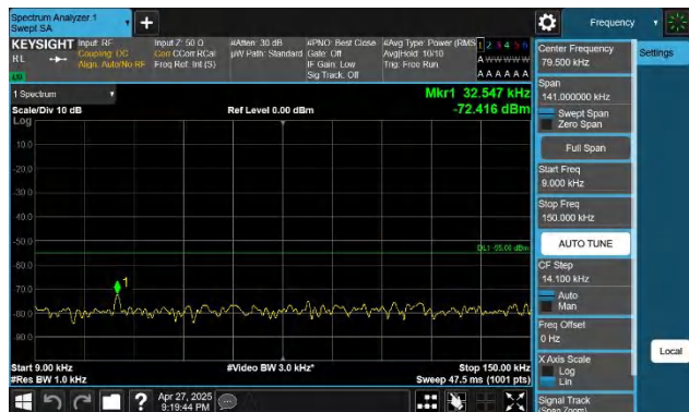
41-41-10MHz-20MHz-QPSK-QPSK-40526-40670-1RB#49-ORB# 0-0.009~0.15MHz-PASS
