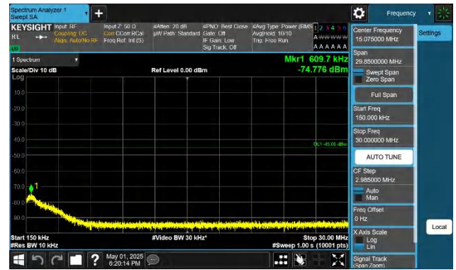
41-41-10MHz-20MHz-QPSK-QPSK-41346-41490-1RB#0-1RB#99 -0.15~30MHz-PASS
