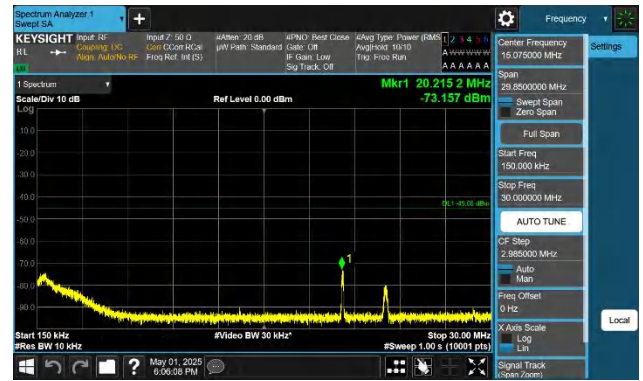
41-41-10MHz-15MHz-QPSK-QPSK-40549-40669-1RB#0-1RB#74 -0.15~30MHz-PASS
