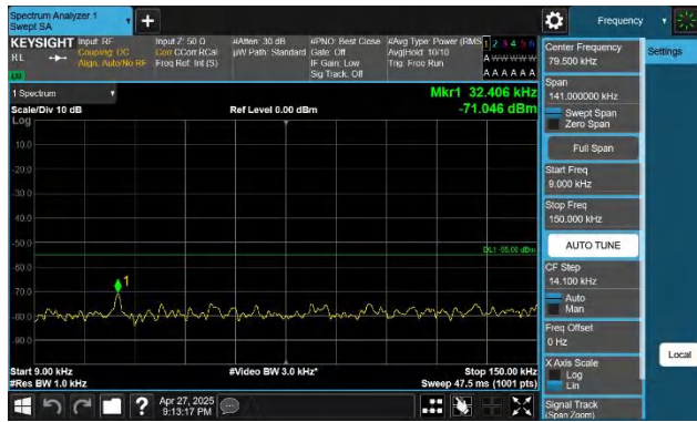
41-41-10MHz-15MHz-QPSK-QPSK-40549-40669-1RB#49-ORB# 0-0.009~0.15MHz-PASS
