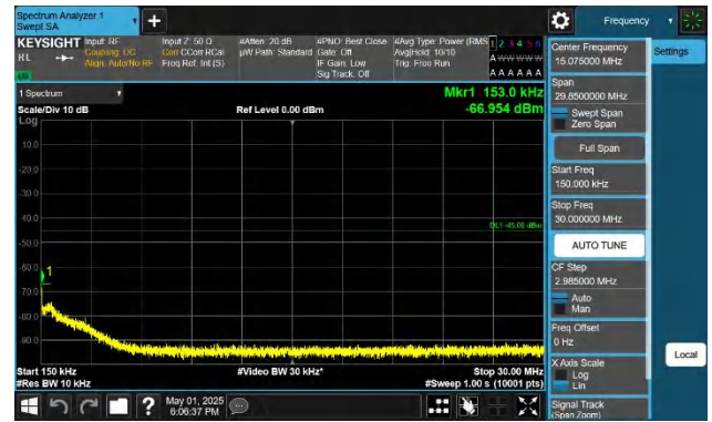
41-41-10MHz-15MHz-QPSK-QPSK-41395-41515-1RB#0-0RB#0 0.15~30MHz-PASS
