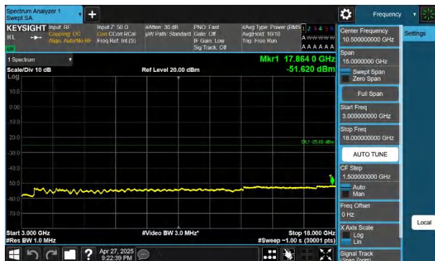
41-41-10MHz-20MHz-QPSK-QPSK-41346-41490-1RB#0-1RB#9 9-3000~18000MHz-PASS
