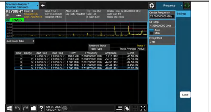
41-41-20MHz-5MHz-QPSK@QPSK-QPSK@QPSK-41440-41557- 1RB#0@100RB#0-1RB#24@25RB#0-PASS
