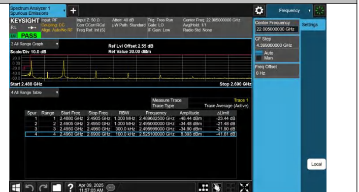
41-41-15MHz-15MHz-QPSK@QPSK-QPSK@QPSK-39725-39875 -1RB#0@75RB#0-1RB#74@75RB#0-PASS
