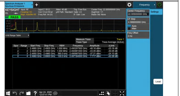
41-41-20MHz-20MHz-QPSK@QPSK-QPSK@QPSK-39750-39948 -1RB#0@100RB#0-1RB#99@100RB#0-PASS
