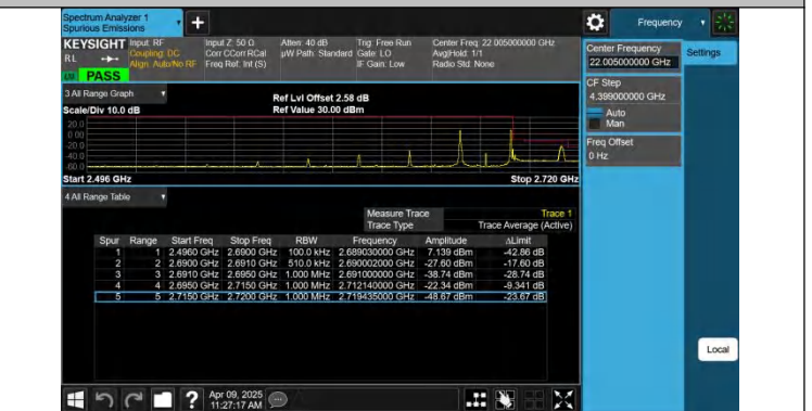
41-41-15MHz-10MHz-QPSK@QPSK-QPSK-41417-41537 -1RB#0@75RB#0-1RB#49@50RB#0-PASS
