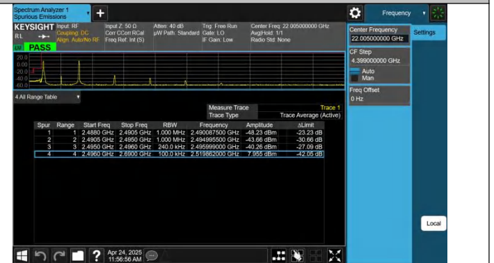
41-41-20MHz-5MHz-QPSK@QPSK-QPSK@QPSK-39750-39867- 1RB#0@100RB#0-1RB#24@25RB#0-PASS
