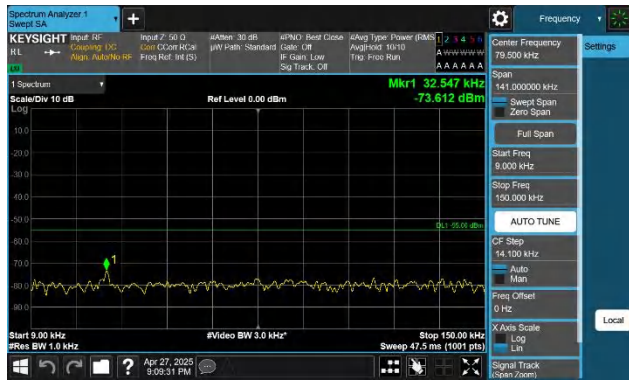
41-41-5MHz-20MHz-QPSK-QPSK-41373-41490-1RB#0-1RB#99 -0.009~0.15MHz-PASS
