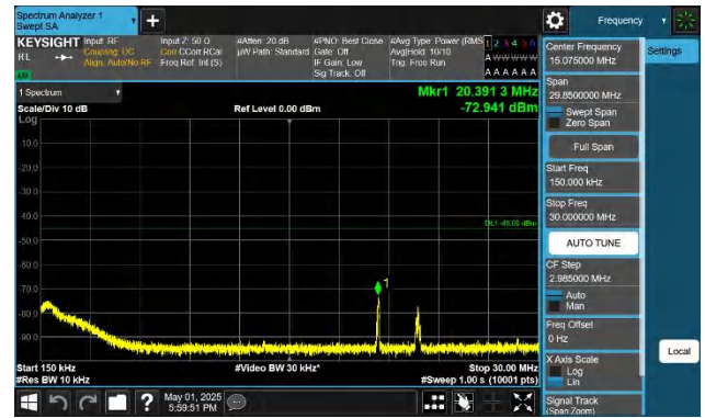
41-41-5MHz-20MHz-QPSK-QPSK-40528-40645-1RB#0-1RB#99- 0.15~30MHz-PASS
