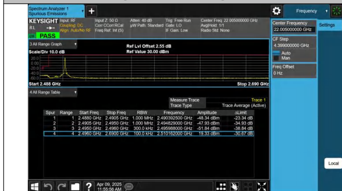
41-41-15MHz-15MHz-QPSK@QPSK-QPSK@QPSK-39725-398 75-1RB#74@75RB#0-0RB#0@75RB#0-PASS
