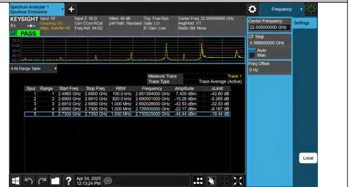
41-41-20MHz-20MHz-QPSK@QPSK-QPSK@QPSK-41292-41490 -1RB#0@100RB#0-1RB#99@100RB#0-PASS
