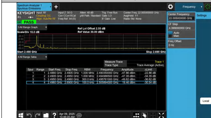
41-41-10MHz-20MHz-QPSK@QPSK-QPSK@QPSK-39705-398 49-1RB#49@50RB#0-0RB#0@100RB#0-PASS
