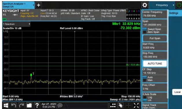
41-41-5MHz-20MHz-QPSK-QPSK-39683-39800-1RB#0-0RB#0-0.009~0.15MHz-PASS
