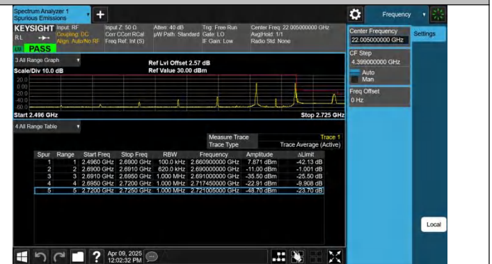
41-41-15MHz-15MHz-QPSK@QPSK-QPSK@QPSK-41365-41515 -1RB#0@75RB#0-1RB#74@75RB#0-PASS
