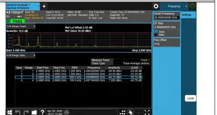
41-41-10MHz-20MHz-QPSK@QPSK-QPSK@QPSK-39705-39849 -1RB#0@50RB#0-1RB#99@100RB#0-PASS
