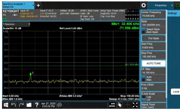
41-41-5MHz-20MHz-QPSK-QPSK-39683-39800-1RB#24-0RB#0 -0.009~0.15MHz-PASS
