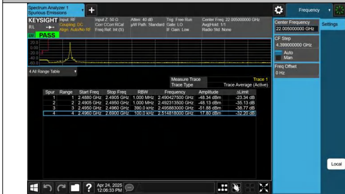
41-41-20MHz-20MHz-QPSK@QPSK-QPSK@QPSK-39750-399 48-1RB#99@100RB#0-0RB#0@100RB#0-PASS
