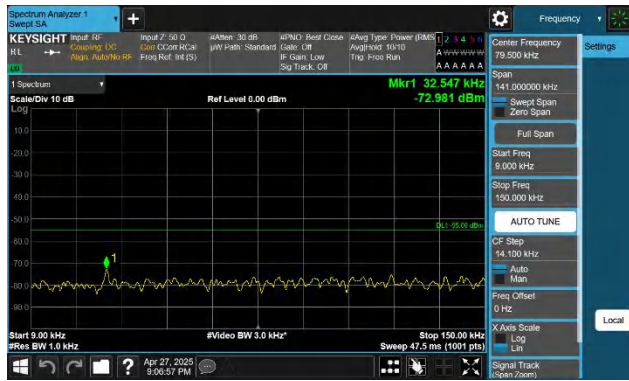
41-41-5MHz-20MHz-QPSK-QPSK-40528-40645-1RB#24-0RB#0 -0.009~0.15MHz-PASS
