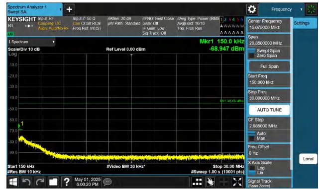
41-41-5MHz-20MHz-QPSK-QPSK-41373-41490-1RB#0-0RB#0-0.15~30MHz-PASS
