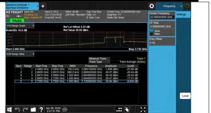
41-41-20MHz-15MHz-QPSK@QPSK-QPSK@QPSK-41341-41512 -100RB#0@100RB#0-75RB#0@75RB#0-PASS
