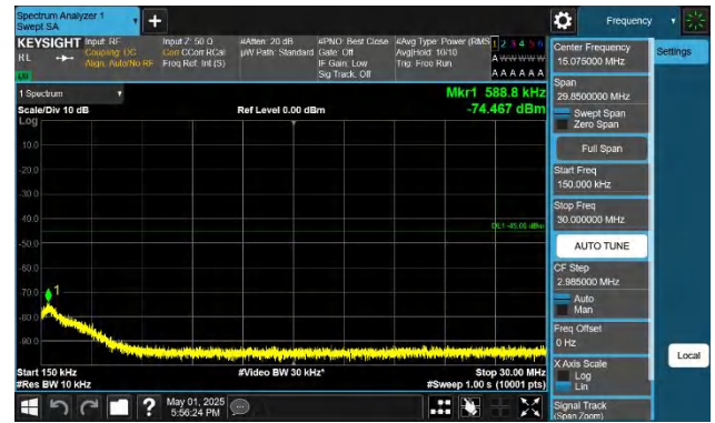
41-41-5MHz-20MHz-QPSK-QPSK-39683-39800-1RB#0-1RB#99- 0.15~30MHz-PASS
