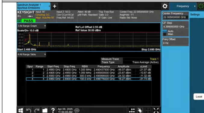
41-41-15MHz-15MHz-QPSK@QPSK-QPSK@QPSK-39725-398 75-1RB#0@75RB#0-0RB#0@75RB#0-PASS
