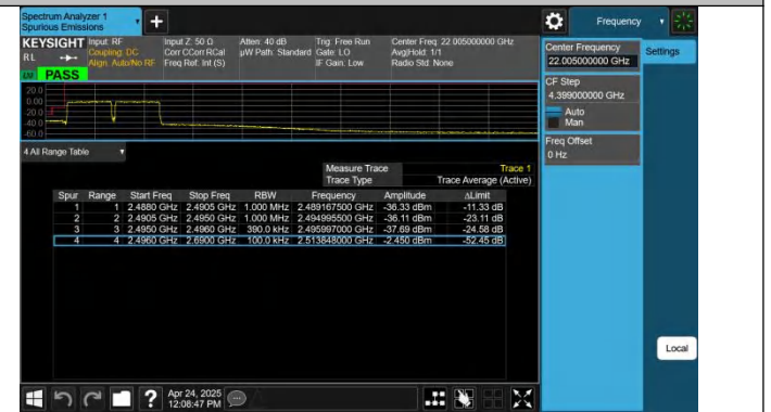
41-41-20MHz-20MHz-QPSK@QPSK-QPSK@QPSK-39750-39948 -100RB#0@100RB#0-100RB#0@100RB#0-PASS
