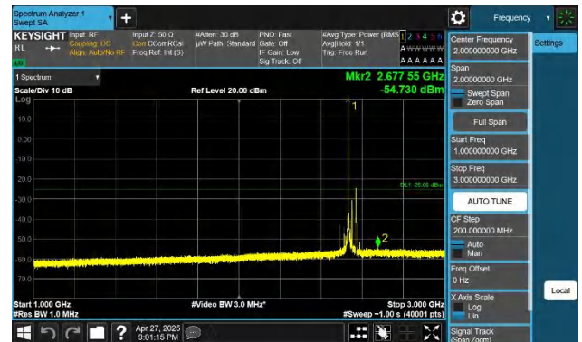
7-7-20MHz-20MHz-QPSK-QPSK-21152-21350-1RB#0-0RB#0-10 00~3000MHz-PASS
