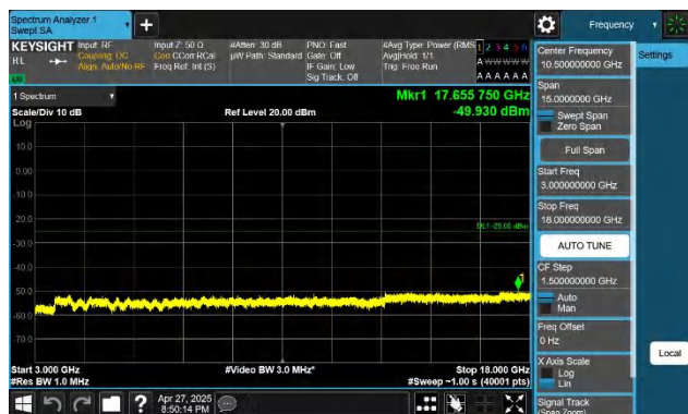
7-7-20MHz-15MHz-QPSK-QPSK-20850-21021-1RB#99-0RB#0- 3000~18000MHz-PASS
