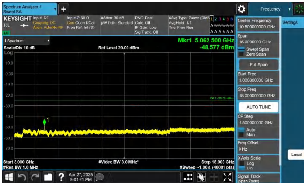
7-7-20MHz-20MHz-QPSK-QPSK-21152-21350-1RB#0-0RB#0-30 00~18000MHz-PASS
