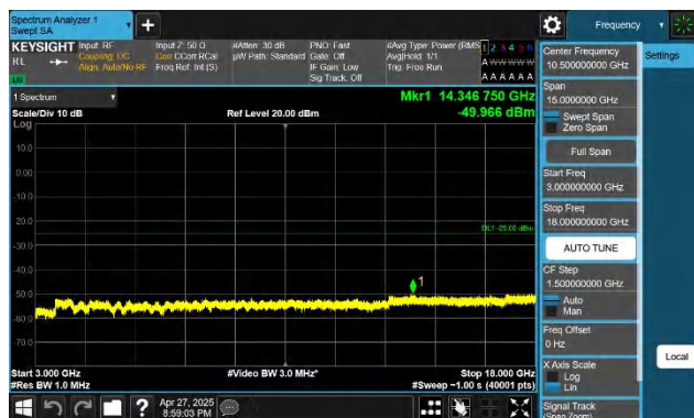
7-7-20MHz-20MHz-QPSK-QPSK-21001-21199-1RB#0-0RB#0-30 00~18000MHz-PASS
