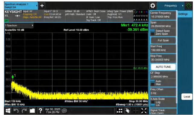
7-7-20MHz-20MHz-QPSK-QPSK-21152-21350-1RB#0-0RB#0-1 5~30MHz-PASS
