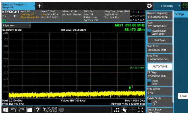
7-7-20MHz-20MHz-QPSK-QPSK-21152-21350-1RB#0-0RB#0-30 ~1000MHz-PASS
