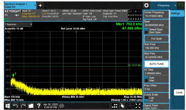
7-7-20MHz-15MHz-QPSK-QPSK-21026-21197-1RB#0-0RB#0-0.1 5~30MHz-PASS
