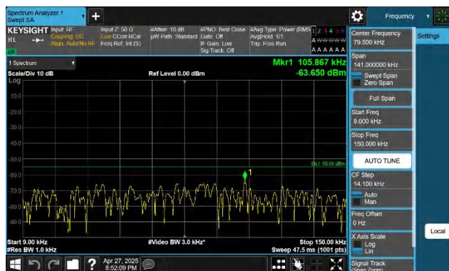
7-7-20MHz-15MHz-QPSK-QPSK-21026-21197-1RB#99-ORB#0-0 .009~0.15MHz-PASS
