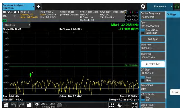
7-7-20MHz-15MHz-QPSK-QPSK-21201-21372-1RB#0-1RB#74- 0.009~0.15MHz-PASS
