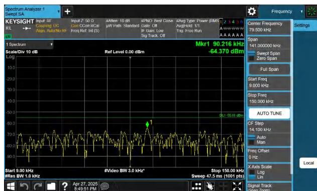
7-7-20MHz-15MHz-QPSK-QPSK-20850-21021-1RB#99-0RB#0- 0.009~0.15MHz-PASS
