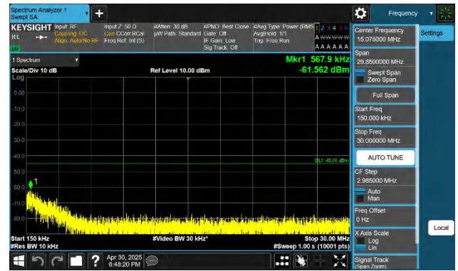
7-7-15MHz-20MHz-QPSK-QPSK-21003-21174-1RB#0-0RB#0-1 5~30MHz-PASS
