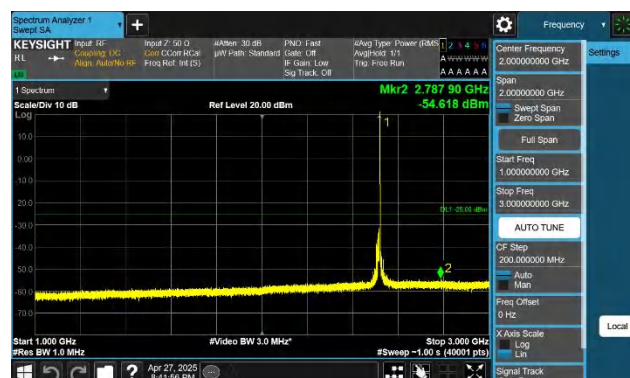
7-7-20MHz-10MHz-QPSK-QPSK-20850-20994-1RB#99-ORB#0-1000~3000MHz-PASS
