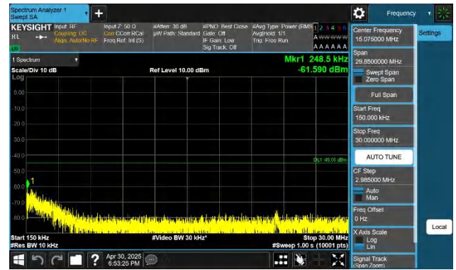
7-7-15MHz-20MHz-QPSK-QPSK-21179-21350-1RB#74-0RB#0-0. 15~30MHz-PASS
