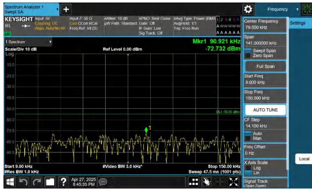
7-7-20MHz-10MHz-QPSK-QPSK-21051-21195-1RB#0-1RB#49-0 .009~0.15MHz-PASS
