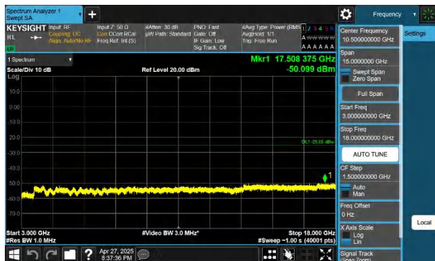
7-7-15MHz-20MHz-QPSK-QPSK-21003-21174-1RB#0-1RB#99-3 000~18000MHz-PASS
