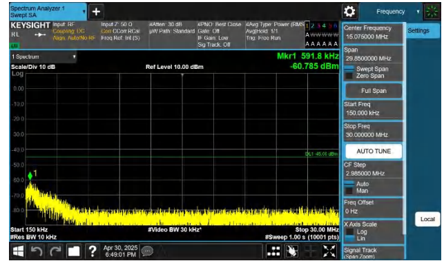
7-7-15MHz-20MHz-QPSK-QPSK-21003-21174-1RB#0-1RB#99-0 15~30MHz-PASS
