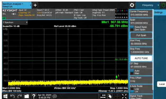
7-7-15MHz-20MHz-QPSK-QPSK-21003-21174-1RB#0-0RB#0-30 ~1000MHz-PASS
