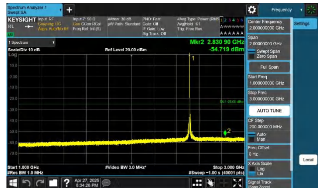
7-7-15MHz-20MHz-QPSK-QPSK-20828-20999-1RB#74-0RB#0-1000~3000MHz-PASS
