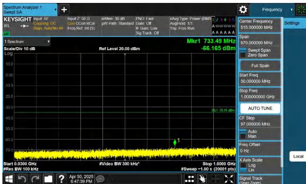
7-7-15MHz-20MHz-QPSK-QPSK-20828-20999-1RB#74-0RB#0-30~1000MHz-PASS
