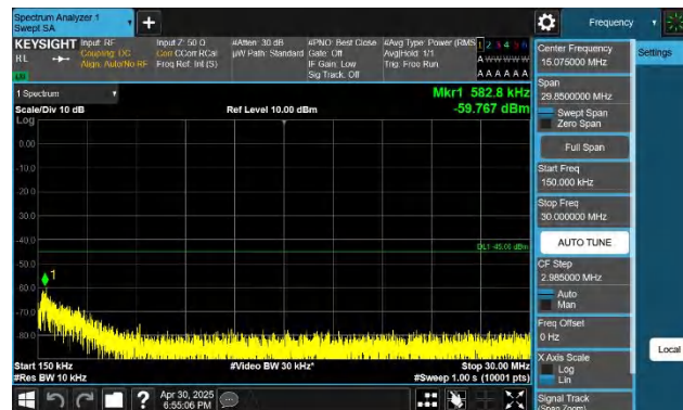
7-7-20MHz-10MHz-QPSK-QPSK-20850-20994-1RB#99-ORB#0-0.15~30MHz-PASS
