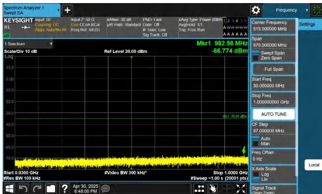
7-7-15MHz-20MHz-QPSK-QPSK-20828-20999-1RB#0-1RB#99- 30~1000MHz-PASS
