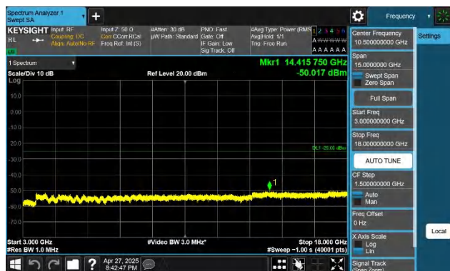
7-7-20MHz-10MHz-QPSK-QPSK-20850-20994-1RB#0-1RB#49- 3000~18000MHz-PASS
