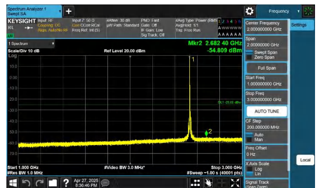
7-7-15MHz-20MHz-QPSK-QPSK-21003-21174-1RB#74-0RB#0-1 000~3000MHz-PASS
