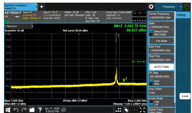
7-7-15MHz-20MHz-QPSK-QPSK-21179-21350-1RB#74-0RB#0-1 000~3000MHz-PASS
