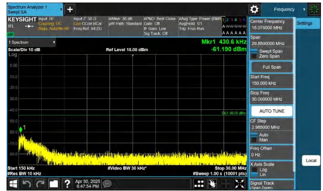
7-7-15MHz-20MHz-QPSK-QPSK-20828-20999-1RB#0-1RB#99-0. 15~30MHz-PASS
