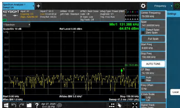
7-7-20MHz-10MHz-QPSK-QPSK-20850-20994-1RB#99-ORB#0-0.009~0.15MHz-PASS
