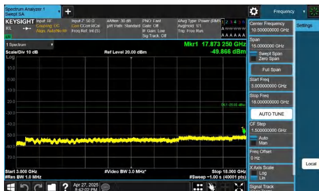
7-7-20MHz-10MHz-QPSK-QPSK-20850-20994-1RB#99-ORB#0-3000~18000MHz-PASS
