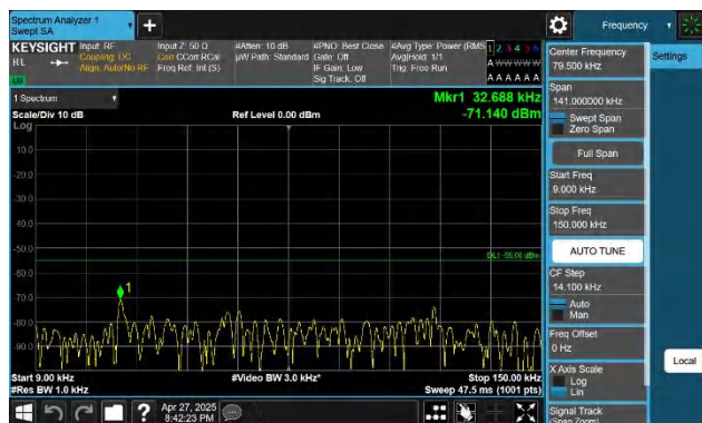
7-7-20MHz-10MHz-QPSK-QPSK-20850-20994-1RB#0-1RB#49- 0.009~0.15MHz-PASS
