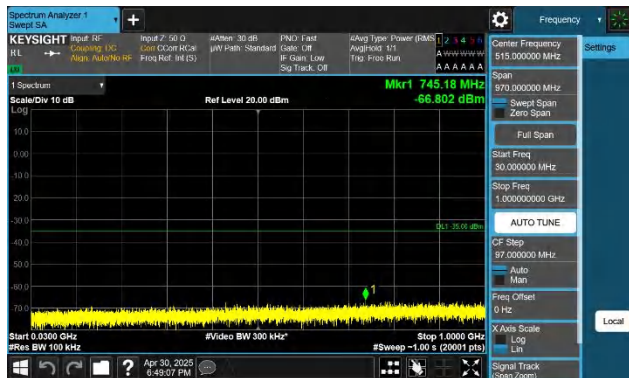
7-7-15MHz-20MHz-QPSK-QPSK-21003-21174-1RB#0-1RB#99-3 0~1000MHz-PASS
