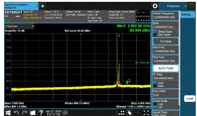
7-7-15MHz-20MHz-QPSK-QPSK-21003-21174-1RB#0-1RB#99-1 000~3000MHz-PASS
