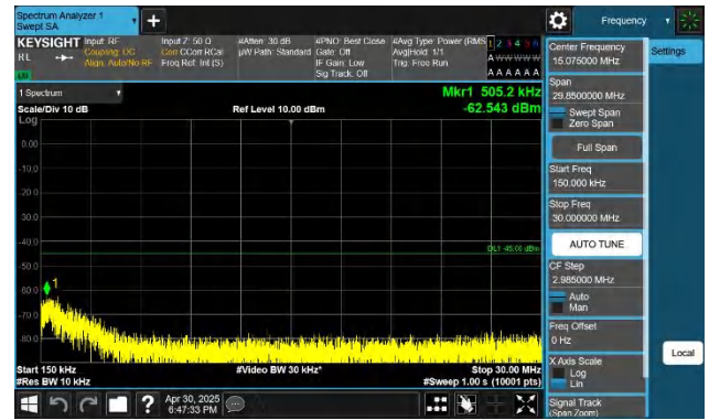
7-7-15MHz-20MHz-QPSK-QPSK-20828-20999-1RB#74-0RB#0-0.15~30MHz-PASS
