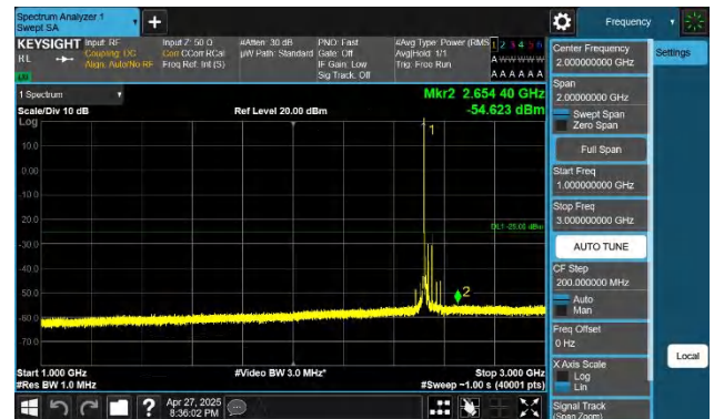
7-7-15MHz-20MHz-QPSK-QPSK-21003-21174-1RB#0-0RB#0-10 00~3000MHz-PASS
