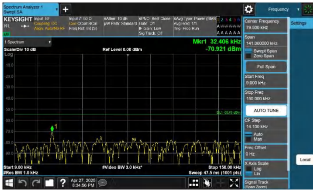
7-7-15MHz-20MHz-QPSK-QPSK-20828-20999-1RB#0-1RB#99- 0.009~0.15MHz-PASS
