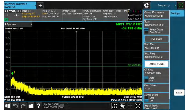
7-7-15MHz-15MHz-QPSK-QPSK-20825-20975-1RB#74-0RB#0-0. 15~30MHz-PASS
