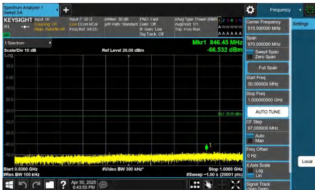
7-7-15MHz-15MHz-QPSK-QPSK-20825-20975-1RB#74-0RB#0- 30~1000MHz-PASS
