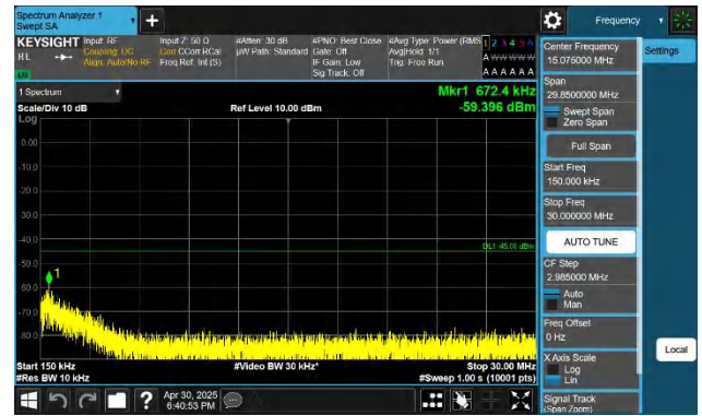
7-7-15MHz-10MHz-QPSK-QPSK-21051-21171-1RB#0-0RB#0-1 5~30MHz-PASS
