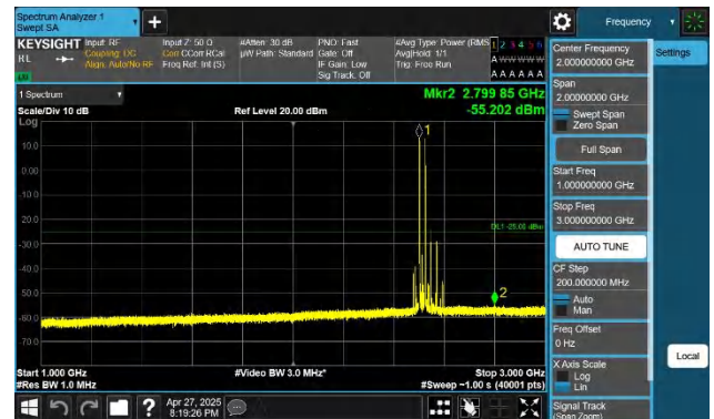
7-7-15MHz-10MHz-QPSK-QPSK-20825-20945-1RB#0-1RB#49-1 000~3000MHz-PASS
