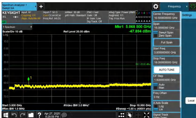
7-7-15MHz-15MHz-QPSK-QPSK-21025-21175-1RB#74-0RB#0-3 000~18000MHz-PASS
