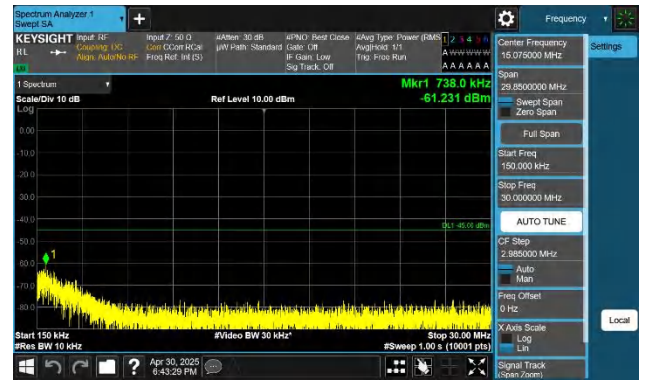
7-7-15MHz-15MHz-QPSK-QPSK-20825-20975-1RB#0-0RB#0-1 5~30MHz-PASS
