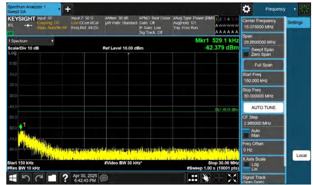
7-7-15MHz-10MHz-QPSK-QPSK-21277-21397-1RB#0-1RB#49-0. 15~30MHz-PASS
