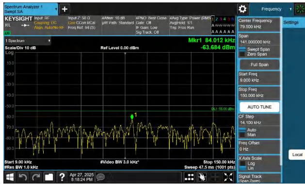
7-7-15MHz-10MHz-QPSK-QPSK-20825-20945-1RB#74-0RB#0-0.009~0.15MHz-PASS
