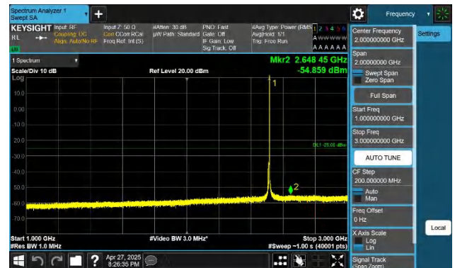
7-7-15MHz-15MHz-QPSK-QPSK-20825-20975-1RB#74-0RB#0-1 000~3000MHz-PASS
