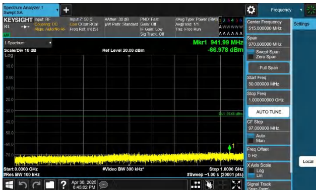
7-7-15MHz-15MHz-QPSK-QPSK-21025-21175-1RB#74-0RB#0-3 0~1000MHz-PASS
