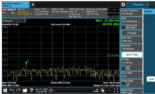
7-7-15MHz-10MHz-QPSK-QPSK-21277-21397-1RB#0-1RB#49- 0.009~0.15MHz-PASS
