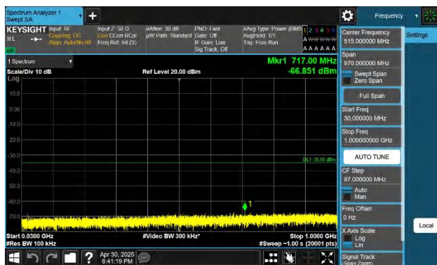
7-7-15MHz-10MHz-QPSK-QPSK-21051-21171-1RB#74-0RB#0-3 0~1000MHz-PASS
