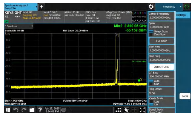
7-7-15MHz-10MHz-QPSK-QPSK-21277-21397-1RB#0-1RB#49-1 000~3000MHz-PASS
