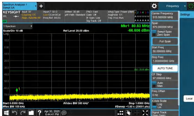
7-7-15MHz-15MHz-QPSK-QPSK-21025-21175-1RB#0-0RB#0-30 ~1000MHz-PASS
