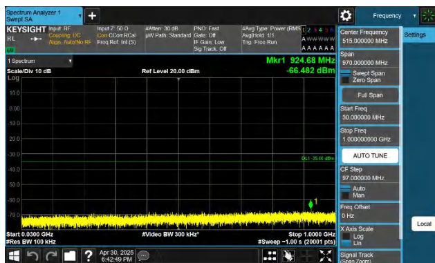
7-7-15MHz-10MHz-QPSK-QPSK-21277-21397-1RB#0-1RB#49- 30~1000MHz-PASS
