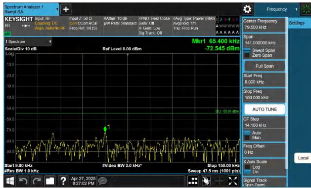
7-7-15MHz-15MHz-QPSK-QPSK-20825-20975-1RB#0-1RB#74- 0.009~0.15MHz-PASS
