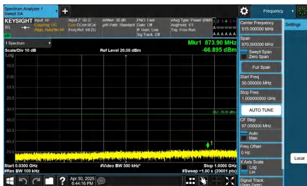
7-7-15MHz-15MHz-QPSK-QPSK-20825-20975-1RB#0-1RB#74- 30~1000MHz-PASS
