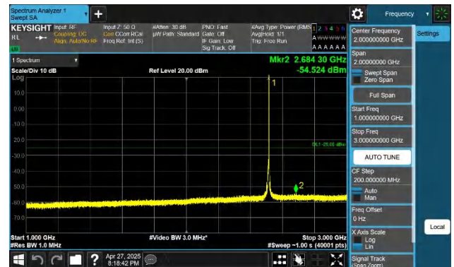
7-7-15MHz-10MHz-QPSK-QPSK-20825-20945-1RB#74-0RB#0-1.000~3000MHz-PASS
