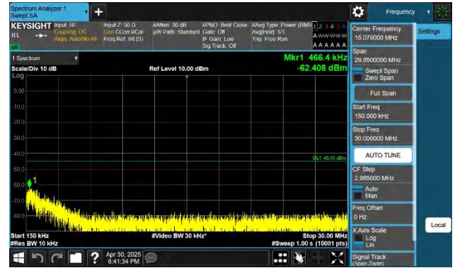
7-7-15MHz-10MHz-QPSK-QPSK-21051-21171-1RB#0-1RB#49-0 15~30MHz-PASS
