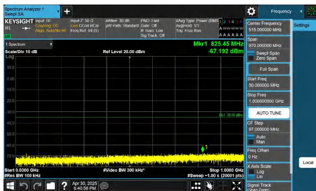
7-7-15MHz-10MHz-QPSK-QPSK-21051-21171-1RB#0-0RB#0-30 ~1000MHz-PASS
