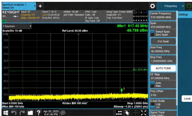
7-7-15MHz-10MHz-QPSK-QPSK-21051-21171-1RB#0-1RB#49-3 0~1000MHz-PASS
