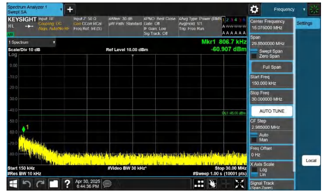
7-7-15MHz-15MHz-QPSK-QPSK-21025-21175-1RB#0-0RB#0-0.1 5~30MHz-PASS
