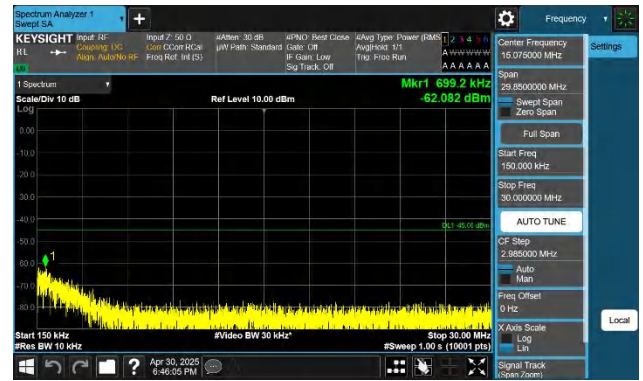
7-7-15MHz-15MHz-QPSK-QPSK-21225-21375-1RB#74-0RB#0-0. 15~30MHz-PASS
