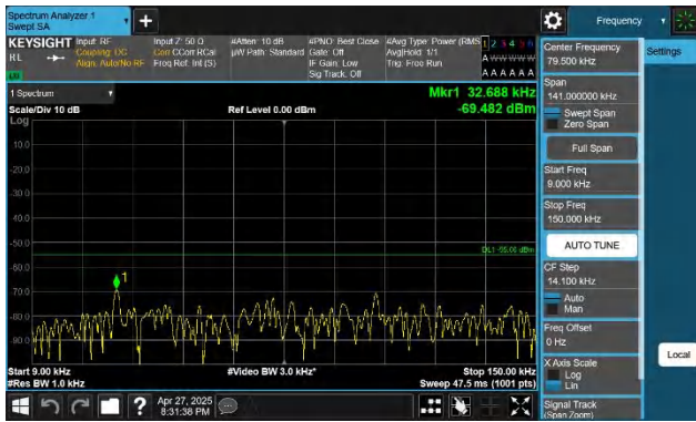
7-7-15MHz-15MHz-QPSK-QPSK-21225-21375-1RB#0-1RB#74- 0.009~0.15MHz-PASS
