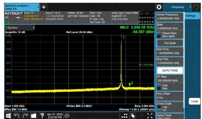
7-7-15MHz-10MHz-QPSK-QPSK-21051-21171-1RB#74-0RB#0-1 000~3000MHz-PASS
