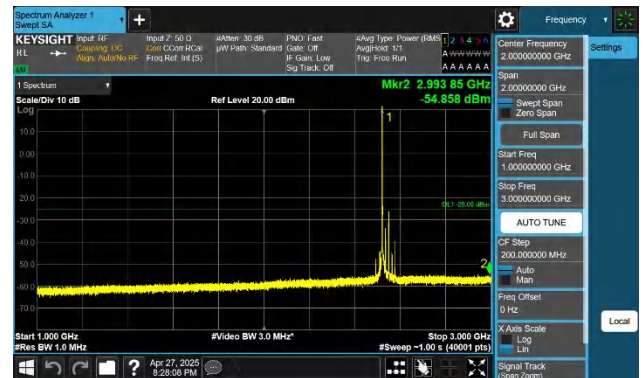
7-7-15MHz-15MHz-QPSK-QPSK-21025-21175-1RB#0-0RB#0-10 00~3000MHz-PASS
