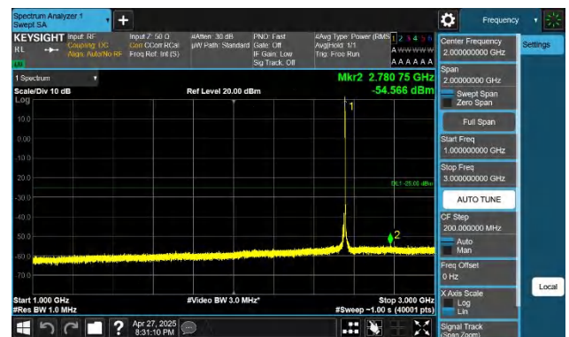
7-7-15MHz-15MHz-QPSK-QPSK-21225-21375-1RB#74-0RB#0-1 000~3000MHz-PASS
