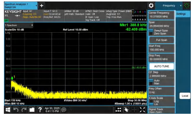
7-7-15MHz-10MHz-QPSK-QPSK-21051-21171-1RB#74-0RB#0-0. 15~30MHz-PASS
