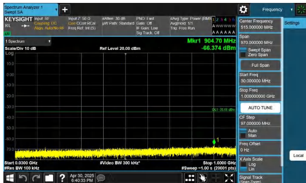
7-7-15MHz-10MHz-QPSK-QPSK-20825-20945-1RB#0-1RB#49- 30~1000MHz-PASS
