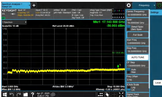
7-7-15MHz-15MHz-QPSK-QPSK-20825-20975-1RB#74-0RB#0- 3000~18000MHz-PASS
