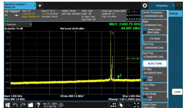
7-7-15MHz-15MHz-QPSK-QPSK-21225-21375-1RB#0-1RB#74-1 000~3000MHz-PASS
