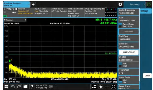
7-7-15MHz-15MHz-QPSK-QPSK-20825-20975-1RB#0-1RB#74-0. 15~30MHz-PASS
