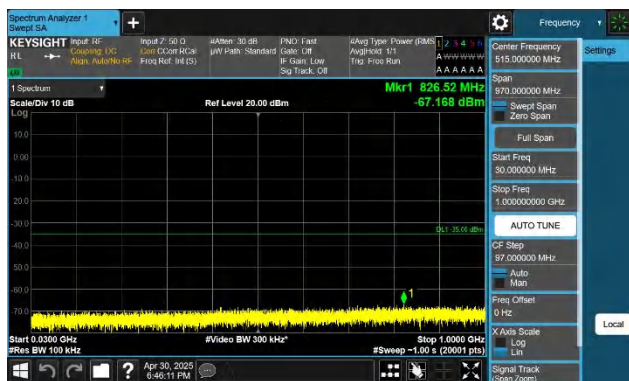
7-7-15MHz-15MHz-QPSK-QPSK-21225-21375-1RB#74-0RB#0- 30~1000MHz-PASS
