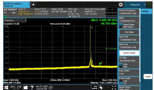
7-7-15MHz-15MHz-QPSK-QPSK-20825-20975-1RB#0-0RB#0-10 00~3000MHz-PASS
