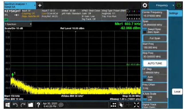
7-7-15MHz-10MHz-QPSK-QPSK-20825-20945-1RB#0-1RB#49-0. 15~30MHz-PASS
