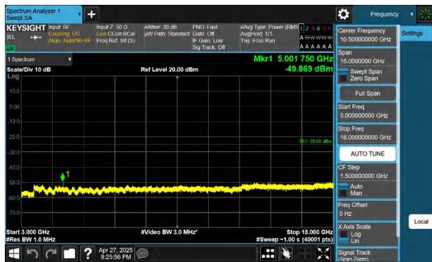
7-7-15MHz-15MHz-QPSK-QPSK-20825-20975-1RB#0-0RB#0-3 000~18000MHz-PASS
