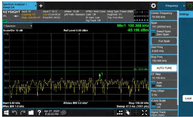
7-7-15MHz-15MHz-QPSK-QPSK-21225-21375-1RB#74-0RB#0- 0.009~0.15MHz-PASS
