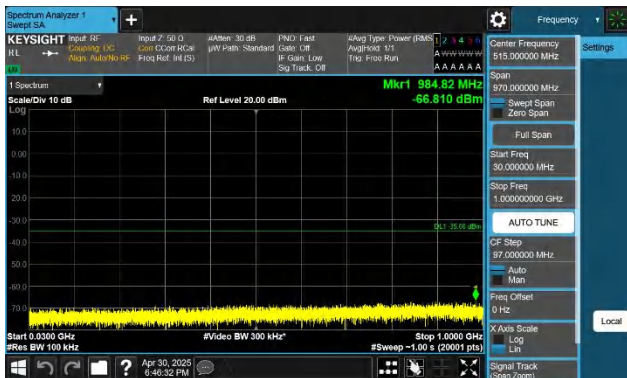
7-7-15MHz-15MHz-QPSK-QPSK-21225-21375-1RB#0-1RB#74- 30~1000MHz-PASS
