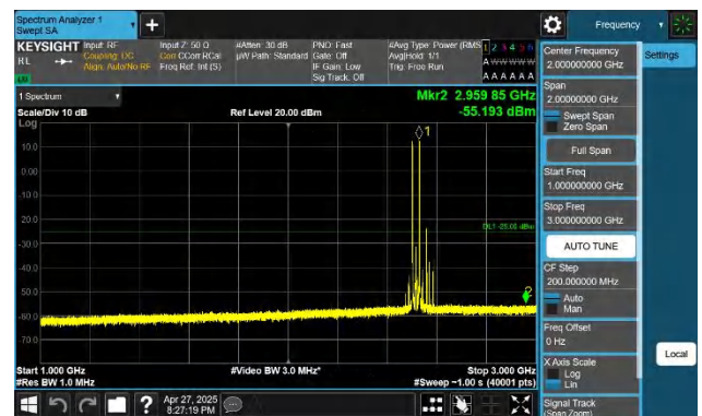
7-7-15MHz-15MHz-QPSK-QPSK-20825-20975-1RB#0-1RB#74-1 000~3000MHz-PASS
