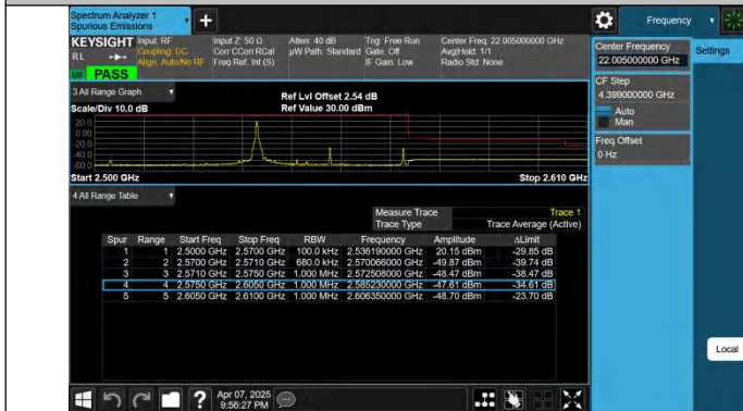
7-7-20MHz-15MHz-QPSK@QPSK-QPSK@QPSK-21201-21372-1 RB#0@100RB#0-0RB#0@75RB#0-PASS
