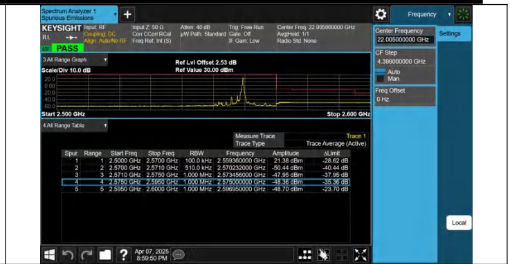
7-7-15MHz-10MHz-QPSK@QPSK-QPSK@QPSK-21277-21397-1 RB#74@75RB#0-0RB#0@50RB#0-PASS
