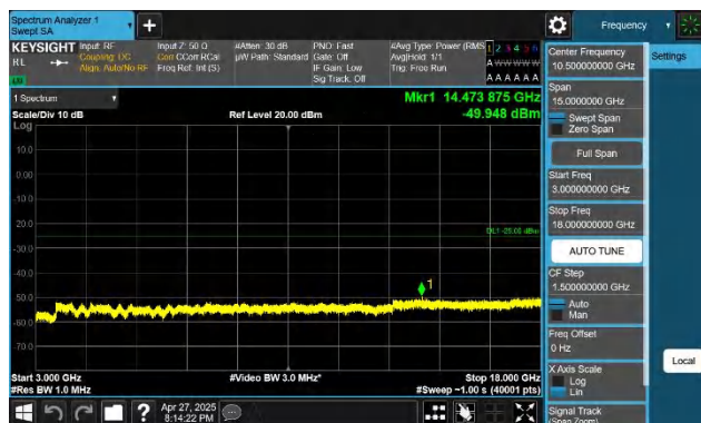
7-7-10MHz-20MHz-QPSK-QPSK-21006-21150-1RB#0-1RB#99-3 000~18000MHz-PASS
