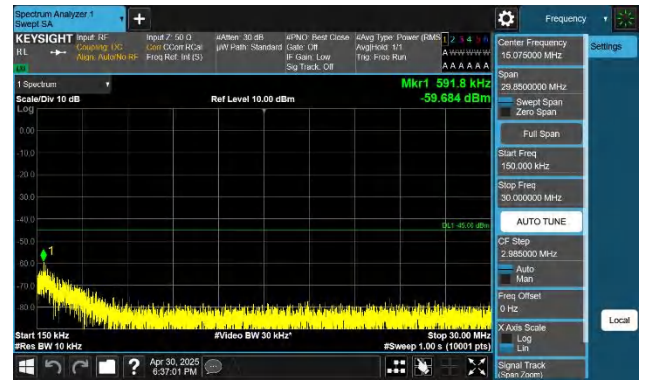
7-7-10MHz-20MHz-QPSK-QPSK-21006-21150-1RB#0-0RB#0-1 5~30MHz-PASS
