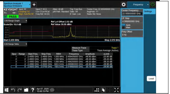
7-7-20MHz-20MHz-QPSK@QPSK-QPSK@QPSK-20850-21048-1 1RB#99@100RB#0-0RB#0@100RB#0-PASS
