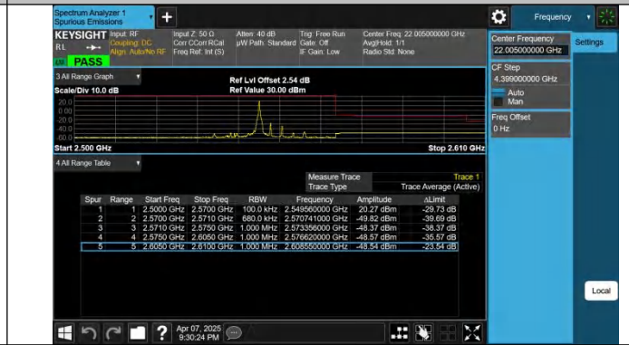
7-7-15MHz-20MHz-QPSK@QPSK-QPSK@QPSK-21179-21350-1 1RB#74@75RB#0-0RB#0@100RB#0-PASS
