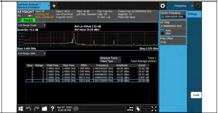
7-7-15MHz-20MHz-QPSK@QPSK-QPSK-20828-20999- 1RB#0@75RB#0-0RB#0@100RB#0-PASS
