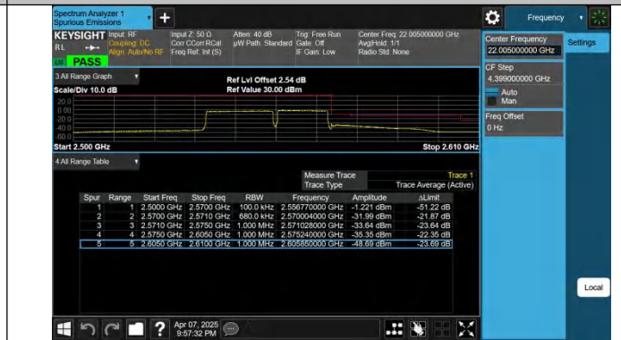
7-7-20MHz-15MHz-QPSK@QPSK-QPSK@QPSK-21201-21372-100RB#0@100RB#0-75RB#0@75RB#0-PASS
