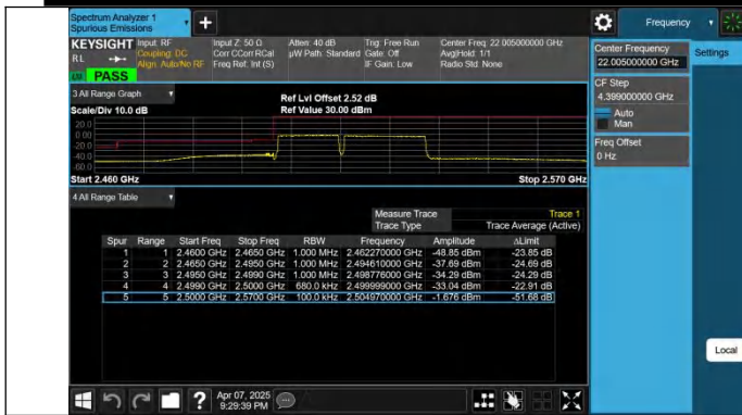
7-7-15MHz-20MHz-QPSK@QPSK-QPSK@QPSK-20828-20999-7 5RB#0@75RB#0-100RB#0@100RB#0-PASS
