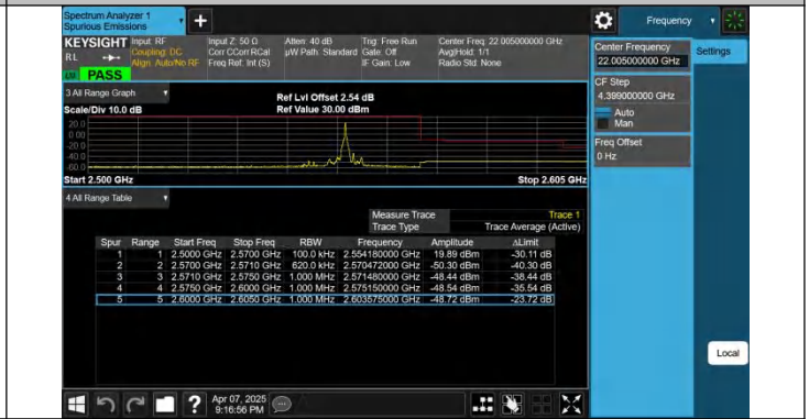
7-7-15MHz-15MHz-QPSK@QPSK-QPSK-21225-21375- 1RB#74@75RB#0-0RB#0@75RB#0-PASS
