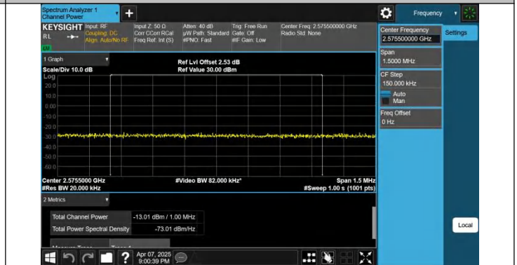
7-7-15MHz-10MHz-QPSK@QPSK-QPSK@QPSK-21277-21397-7 75RB#0@75RB#0-50RB#0@50RB#0-PASS
