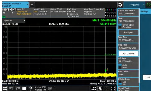
7-7-10MHz-20MHz-QPSK-QPSK-21206-21350-1RB#49-ORB#0- 30~1000MHz-PASS
