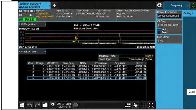
7-7-20MHz-20MHz-QPSK@QPSK-QPSK@QPSK-20850-21048-1 RB#0@100RB#0-1RB#99@100RB#0-PASS
