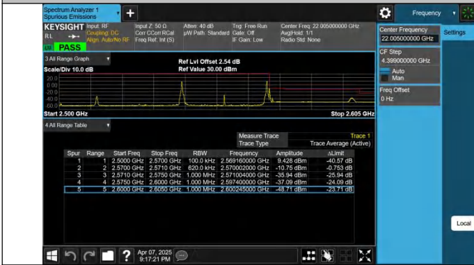
7-7-15MHz-15MHz-QPSK@QPSK-QPSK-21225-21375-1 RB#0@75RB#0-1RB#74@75RB#0-PASS
