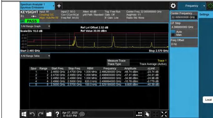
7-7-15MHz-15MHz-QPSK@QPSK-QPSK@QPSK-20825-20975-1 RB#0@75RB#0-1RB#74@75RB#0-PASS
