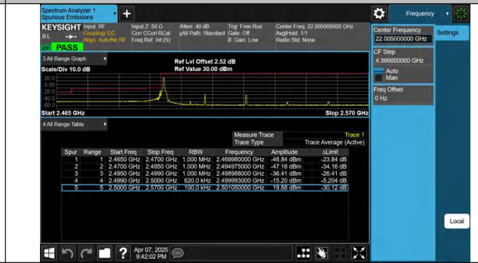
7-7-20MHz-10MHz-QPSK@QPSK-QPSK@QPSK-20850-20994-1 1RB#0@100RB#0-0RB#0@50RB#0-PASS
