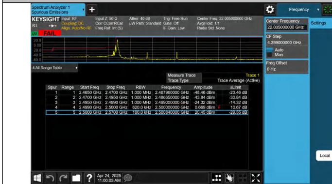
7-7-15MHz-15MHz-QPSK@QPSK-QPSK@QPSK-20825-20975-1 RB#0@75RB#0-0RB#0@75RB#0
