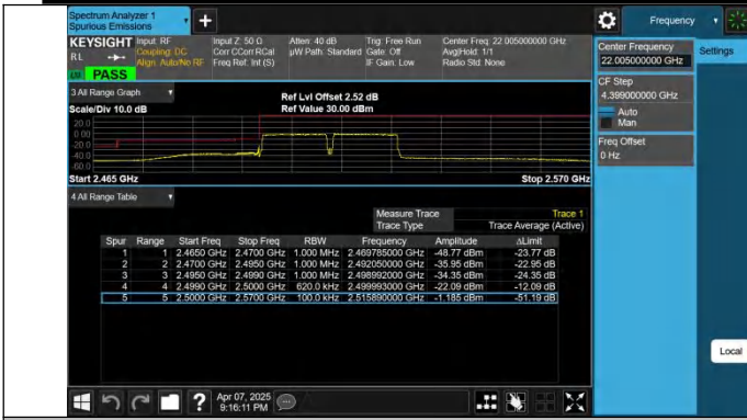
7-7-15MHz-15MHz-QPSK@QPSK-QPSK-20825-20975-7 5RB#0@75RB#0-75RB#0-PASS
