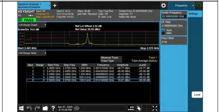
7-7-15MHz-15MHz-QPSK@QPSK-QPSK@QPSK-20825-20975-1 RB#74@75RB#0-0RB#0@75RB#0-PASS
