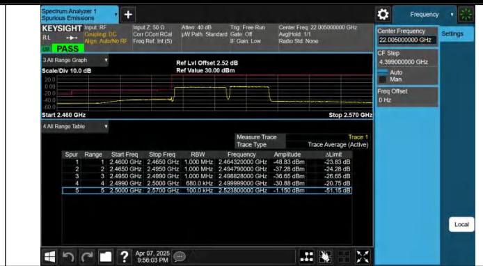
7-7-20MHz-15MHz-QPSK@QPSK-QPSK@QPSK-20850-21021-100RB#0@100RB#0-75RB#0@75RB#0-PASS
