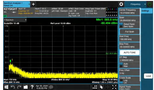
7-7-10MHz-20MHz-QPSK-QPSK-20805-20949-1RB#0-ORB#0-1 5~30MHz-PASS
