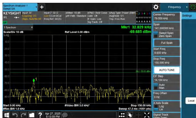
7-7-10MHz-20MHz-QPSK-QPSK-21006-21150-1RB#0-1RB#99-0 .009~0.15MHz-PASS
