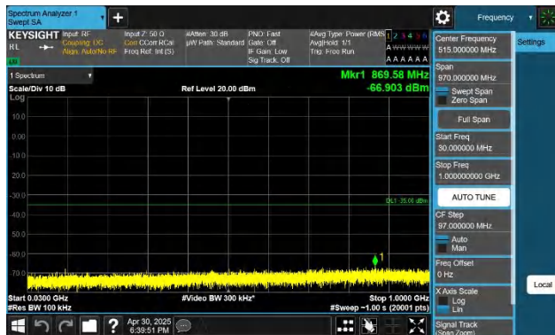
7-7-15MHz-10MHz-QPSK-QPSK-20825-20945-1RB#0-0RB#0-3 0~1000MHz-PASS
