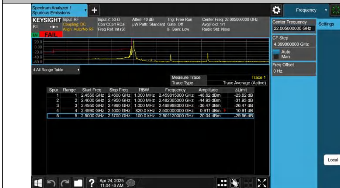
7-7-20MHz-20MHz-QPSK@QPSK-QPSK@QPSK-20850-21048-1 RB#0@100RB#0-0RB#0@100RB#0
