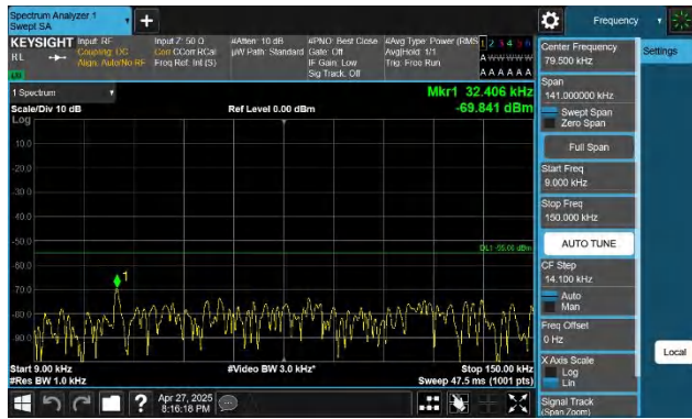
7-7-10MHz-20MHz-QPSK-QPSK-21206-21350-1RB#0-1RB#99- 0.009~0.15MHz-PASS
