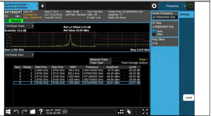
7-7-20MHz-20MHz-QPSK@QPSK-QPSK@QPSK-21152-21350-1 1RB#99@100RB#0-0RB#0@100RB#0-PASS
