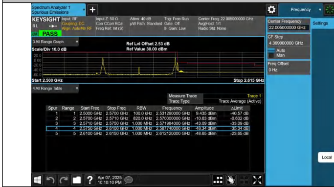
7-7-20MHz-20MHz-QPSK@QPSK-QPSK@QPSK-21152-21350-1 RB#0@100RB#0-1RB#99@100RB#0-PASS
