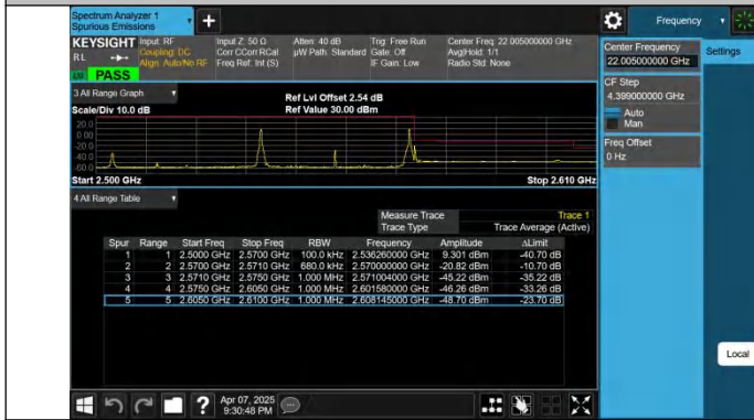
7-7-15MHz-20MHz-QPSK@QPSK-QPSK@QPSK-21179-21350-1 RB#0@75RB#0-1RB#99@100RB#0-PASS
