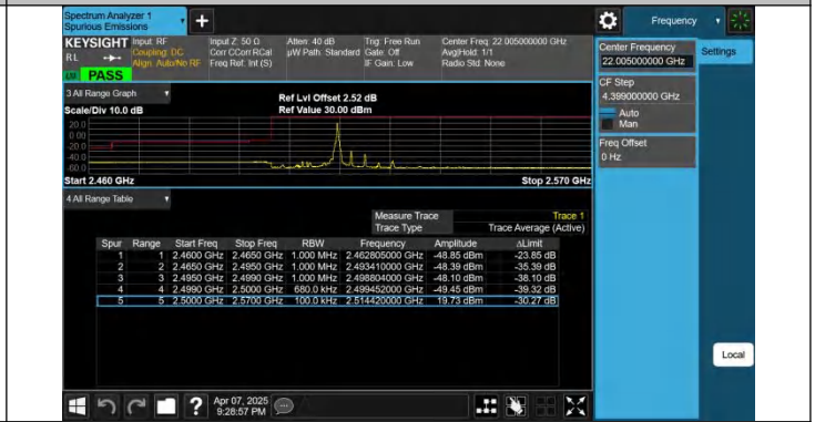
7-7-15MHz-20MHz-QPSK@QPSK-QPSK-20828-20999- 1RB#74@75RB#0-0RB#0@100RB#0-PASS
