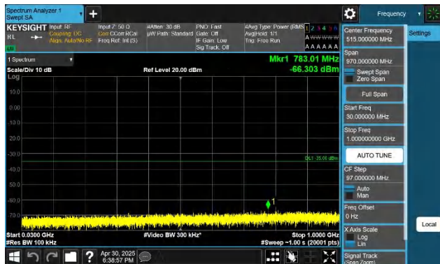
7-7-10MHz-20MHz-QPSK-QPSK-21206-21350-1RB#0-1RB#99- 30~1000MHz-PASS
