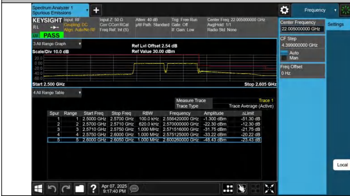
7-7-15MHz-15MHz-QPSK@QPSK-QPSK-21225-21375-7 5RB#0@75RB#0-75RB#0@75RB#0-PASS
