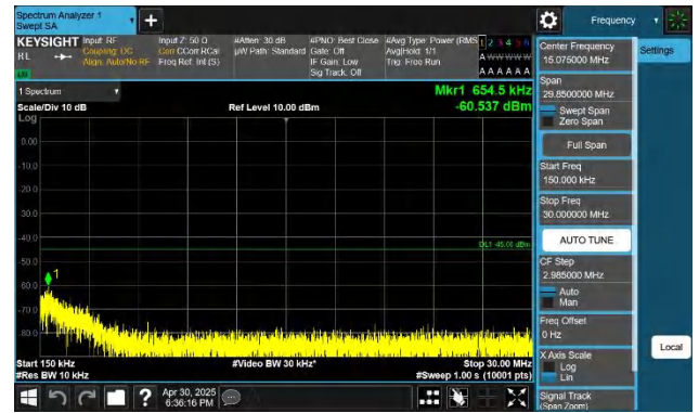
7-7-10MHz-20MHz-QPSK-QPSK-20805-20949-1RB#49-ORB#0-0.15~30MHz-PASS
