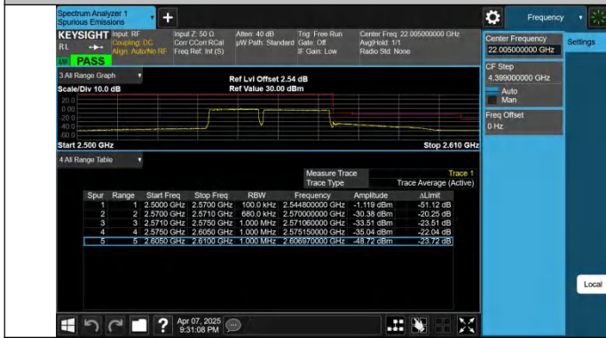
7-7-15MHz-20MHz-QPSK@QPSK-QPSK@QPSK-21179-21350-7 5RB#0@75RB#0-100RB#0@100RB#0-PASS
