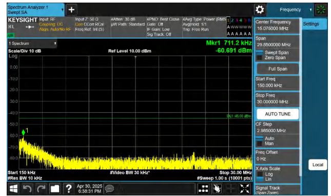
7-7-10MHz-20MHz-QPSK-QPSK-21206-21350-1RB#49-ORB#0-0. 15~30MHz-PASS
