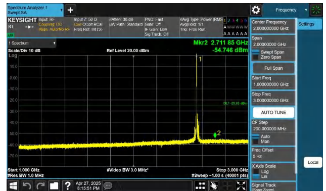
7-7-10MHz-20MHz-QPSK-QPSK-21206-21350-1RB#49-ORB#0-1 000~3000MHz-PASS
