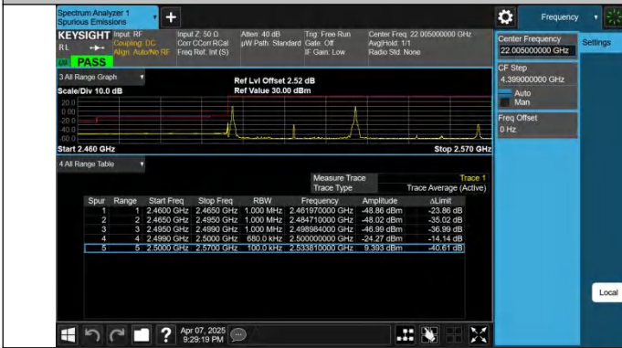
7-7-15MHz-20MHz-QPSK@QPSK-QPSK-20828-20999-1 RB#0@75RB#0-1RB#99@100RB#0-PASS
