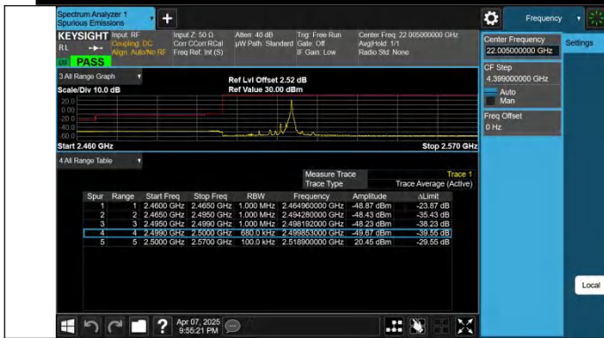
7-7-20MHz-15MHz-QPSK@QPSK-QPSK@QPSK-20850-21021-1 RB#99@100RB#0-0RB#0@75RB#0-PASS
