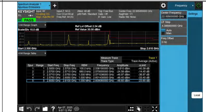
7-7-20MHz-15MHz-QPSK@QPSK-QPSK@QPSK-21201-21372-1RB#0@100RB#0-1RB#74@75RB#0-PASS
