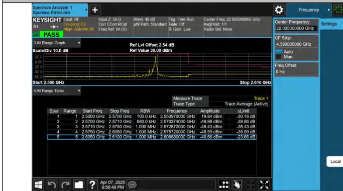
7-7-20MHz-15MHz-QPSK@QPSK-QPSK@QPSK-21201-21372-1 RB#99@100RB#0-0RB#0@75RB#0-PASS
