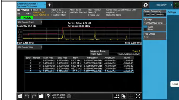
7-7-20MHz-10MHz-QPSK@QPSK-QPSK@QPSK-20850-20994-1 RB#0@100RB#0-1RB#49@50RB#0-PASS
