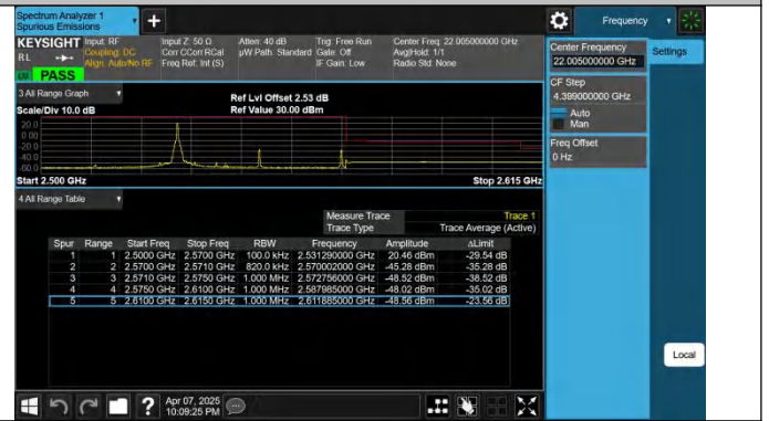
7-7-20MHz-20MHz-QPSK@QPSK-QPSK@QPSK-21152-21350-1 1RB#0@100RB#0-0RB#0@100RB#0-PASS
