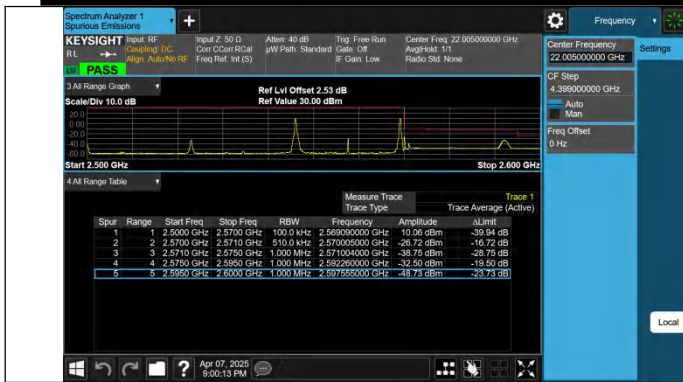
7-7-15MHz-10MHz-QPSK@QPSK-QPSK@QPSK-21277-21397-1 RB#0@75RB#0-1RB#49@50RB#0-PASS
