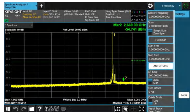
7-7-15MHz-10MHz-QPSK-QPSK-20825-20945-1RB#0-0RB#0-10 00~3000MHz-PASS
