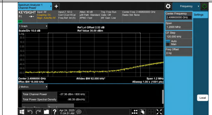
7-7-20MHz-20MHz-QPSK@QPSK-QPSK@QPSK-20850-21048-1RB#0@100RB#0-0RB#0@100RB#0-PASS
