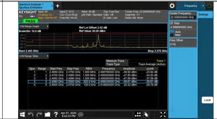
7-7-20MHz-10MHz-QPSK@QPSK-QPSK@QPSK-20850-20994-1 1RB#99@100RB#0-0RB#0@50RB#0-PASS
