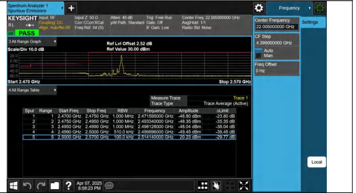
7-7-15MHz-10MHz-QPSK@QPSK-QPSK@QPSK-20825-20945-1 1RB#74@75RB#0-0RB#0@50RB#0-PASS
