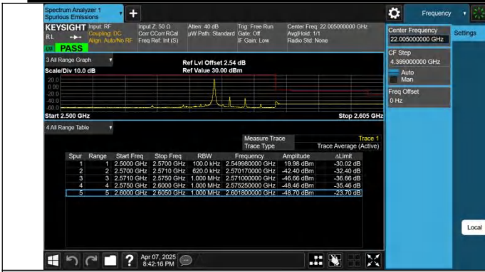
7-7-10MHz-20MHz-QPSK@QPSK-QPSK@QPSK-21206-21350-1 RB#49@50RB#0-0RB#0@100RB#0-PASS
