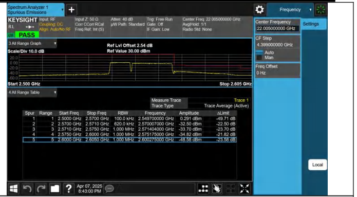
7-7-10MHz-20MHz-QPSK@QPSK-QPSK@QPSK-21206-21350-1 50RB#0@50RB#0-100RB#0@100RB#0-PASS
