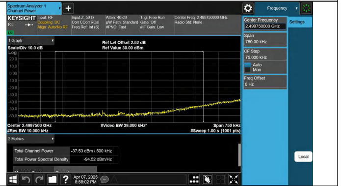
7-7-15MHz-10MHz-QPSK@QPSK-QPSK@QPSK-20825-20945-1 1RB#0@75RB#0-0RB#0@50RB#0-PASS
