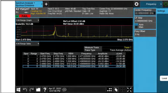
7-7-15MHz-10MHz-QPSK@QPSK-QPSK@QPSK-20825-20945-1 RB#0@75RB#0-0RB#0@50RB#0
