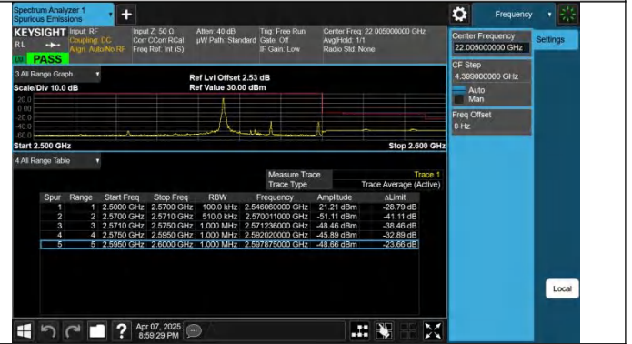
7-7-15MHz-10MHz-QPSK@QPSK-QPSK@QPSK-21277-21397-1 1RB#0@75RB#0-0RB#0@50RB#0-PASS
