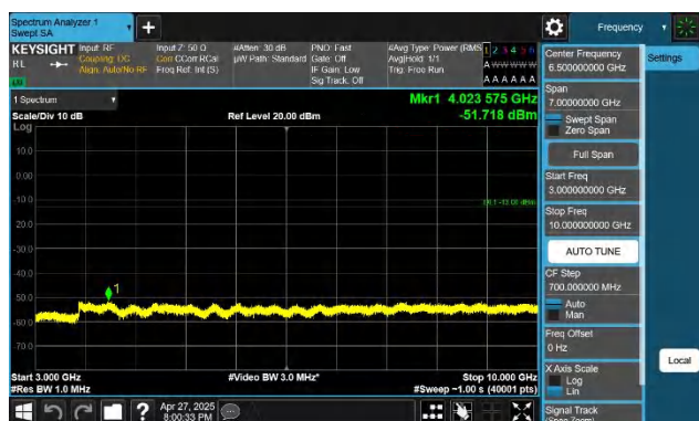
5-5-10MHz-10MHz-QPSK-QPSK-20450-20549-1RB#49-0RB#0-3 000~10000MHz-PASS
