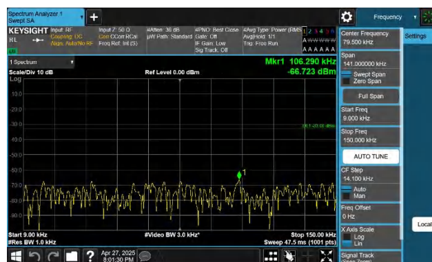
5-5-10MHz-10MHz-QPSK-QPSK-20476-20575-1RB#0-0RB#0-0. 009~0.15MHz-PASS
