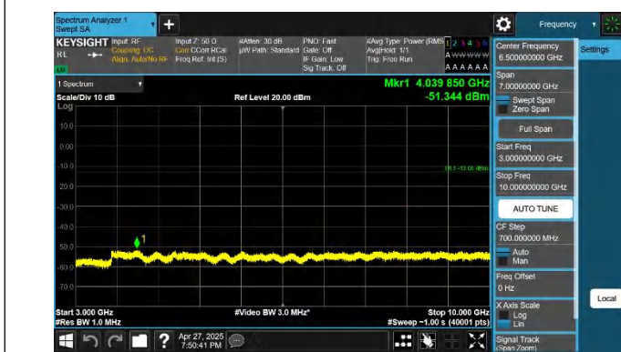
5-5-5MHz-10MHz-QPSK-QPSK-20528-20600-1RB#24-ORB#0-30 00~10000MHz-PASS
