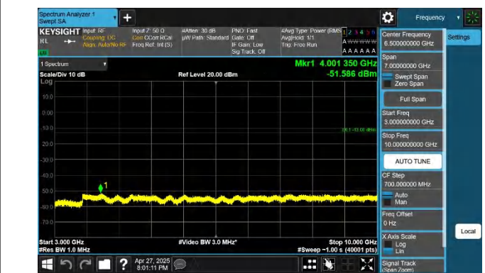
5-5-10MHz-10MHz-QPSK-QPSK-20450-20549-1RB#0-1RB#49-3 000~10000MHz-PASS
