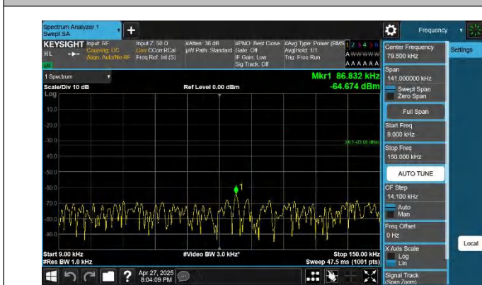
5-5-10MHz-10MHz-QPSK-QPSK-20501-20600-1RB#49-0RB#0-0 .009~0.15MHz-PASS
