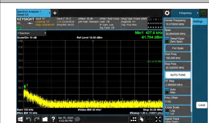
5-5-10MHz-10MHz-QPSK-QPSK-20501-20600-1RB#49-0RB#0-0 .15~30MHz-PASS
