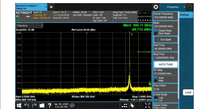
5-5-10MHz-10MHz-QPSK-QPSK-20476-20575-1RB#49-0RB#0-3 0~1000MHz-PASS
