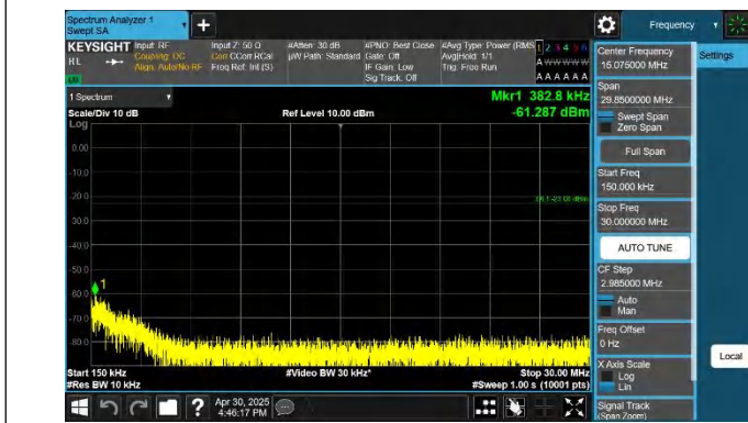
5-5-10MHz-5MHz-QPSK-QPSK-20450-20522-1RB#0-ORB#0-0.1 5~30MHz-PASS
