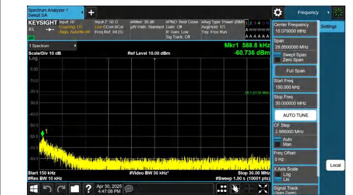
5-5-10MHz-5MHz-QPSK-QPSK-20450-20522-1RB#0-1RB#24-0. 15~30MHz-PASS
