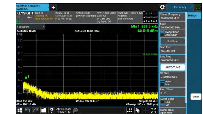
5-5-10MHz-5MHz-QPSK-QPSK-20550-20622-1RB#0-1RB#24-0. 15~30MHz-PASS
