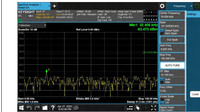
5-5-10MHz-10MHz-QPSK-QPSK-20450-20549-1RB#49-0RB#0-0 .009~0.15MHz-PASS
