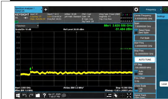
5-5-10MHz-5MHz-QPSK-QPSK-20550-20622-1RB#0-1RB#24-30 00~10000MHz-PASS
