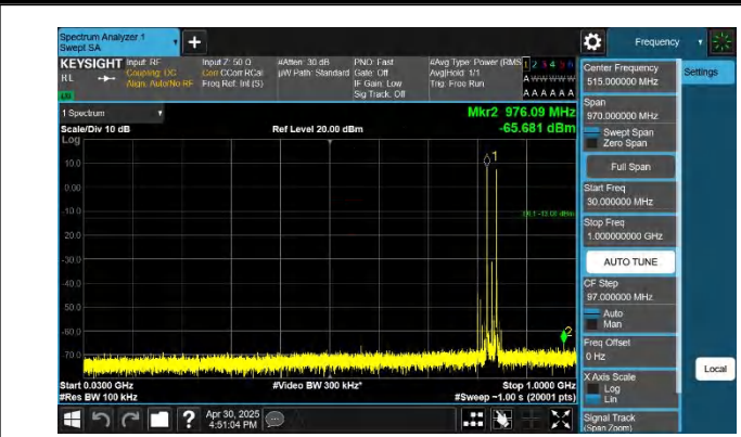
5-5-10MHz-10MHz-QPSK-QPSK-20450-20549-1RB#0-1RB#49-3 0~1000MHz-PASS
