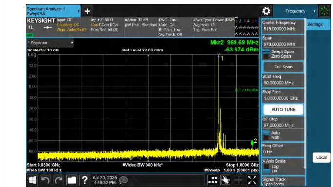
5-5-10MHz-5MHz-QPSK-QPSK-20450-20522-1RB#0-ORB#0-30~ 1000MHz-PASS
