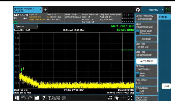
5-5-10MHz-5MHz-QPSK-QPSK-20500-20572-1RB#0-ORB#0-0.1 5~30MHz-PASS
