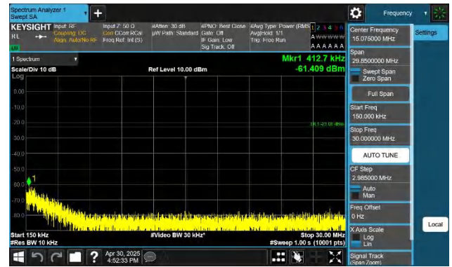
5-5-10MHz-10MHz-QPSK-QPSK-20501-20600-1RB#0-0RB#0-0. 15~30MHz-PASS
