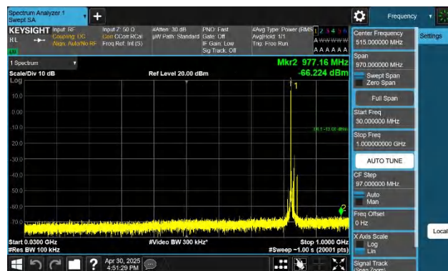
5-5-10MHz-10MHz-QPSK-QPSK-20476-20575-1RB#0-0RB#0-30 ~1000MHz-PASS
