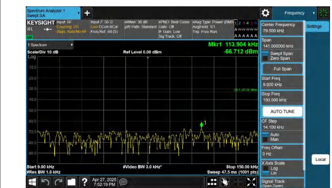
5-5-10MHz-5MHz-QPSK-QPSK-20450-20522-1RB#0-ORB#0-0.0 09~0.15MHz-PASS
