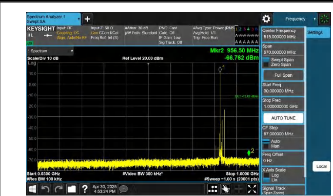
5-5-10MHz-10MHz-QPSK-QPSK-20501-20600-1RB#0-1RB#49-3 0~1000MHz-PASS
