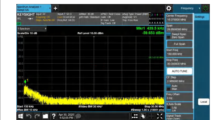
5-5-10MHz-10MHz-QPSK-QPSK-20476-20575-1RB#0-1RB#49-0 .15~30MHz-PASS
