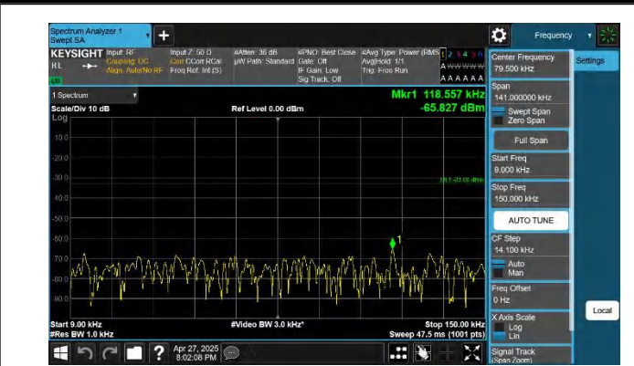
5-5-10MHz-10MHz-QPSK-QPSK-20476-20575-1RB#49-0RB#0-0 .009~0.15MHz-PASS
