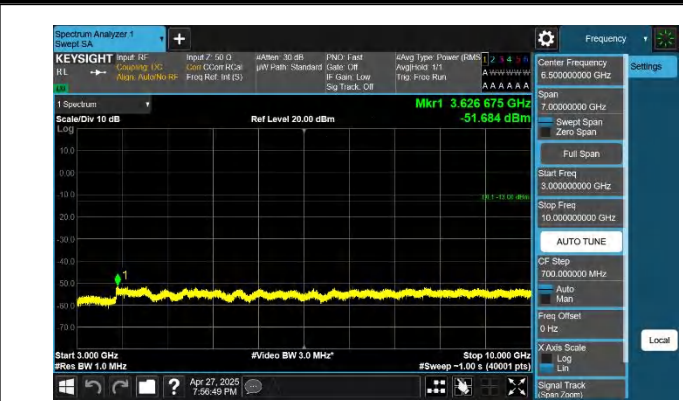
5-5-10MHz-5MHz-QPSK-QPSK-20550-20622-1RB#0-0RB#0-300 0~10000MHz-PASS
