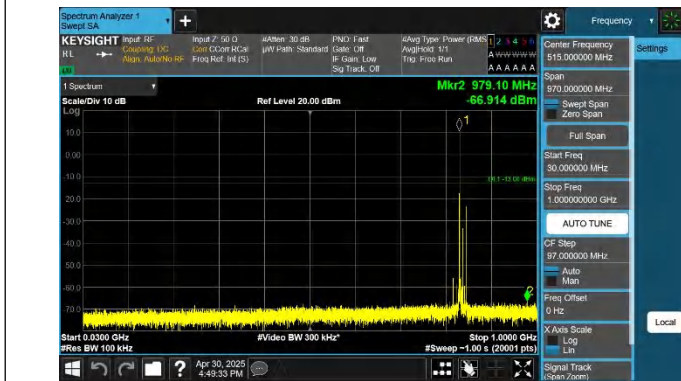
5-5-10MHz-5MHz-QPSK-QPSK-20550-20622-1RB#0-1RB#24-30 ~1000MHz-PASS
