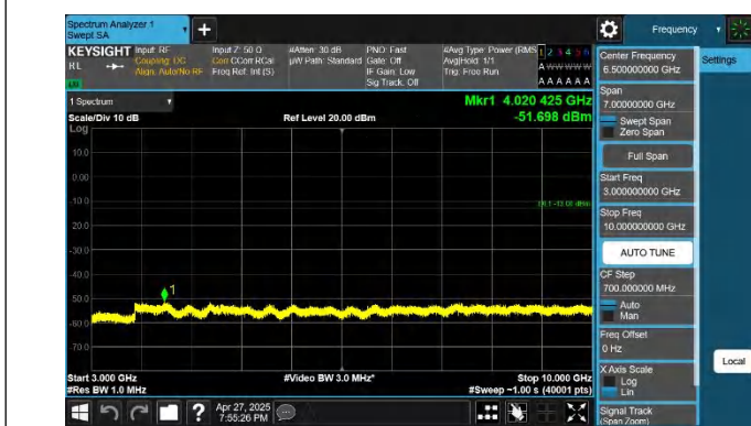
5-5-10MHz-5MHz-QPSK-QPSK-20500-20572-1RB#49-ORB#0-30 00~10000MHz-PASS
