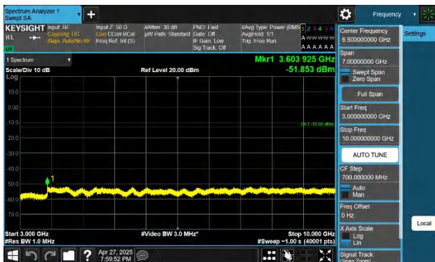
5-5-10MHz-10MHz-QPSK-QPSK-20450-20549-1RB#0-0RB#0-30 00~10000MHz-PASS
