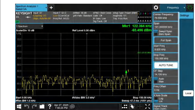
5-5-10MHz-5MHz-QPSK-QPSK-20550-20622-1RB#0-ORB#0-0.0 09~0.15MHz-PASS
