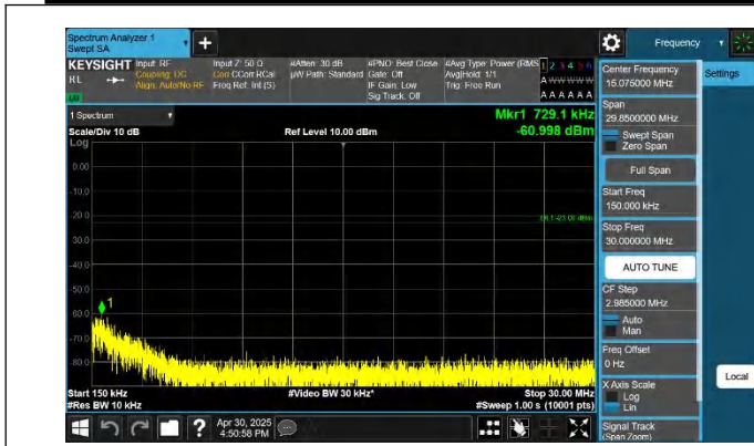
5-5-10MHz-10MHz-QPSK-QPSK-20450-20549-1RB#0-1RB#49-0 .15~30MHz-PASS
