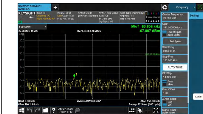
5-5-10MHz-5MHz-QPSK-QPSK-20550-20622-1RB#0-1RB#24-0. 009~0.15MHz-PASS
