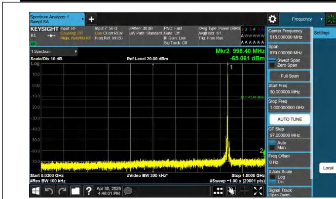
5-5-10MHz-5MHz-QPSK-QPSK-20500-20572-1RB#49-ORB#0-30 ~1000MHz-PASS
