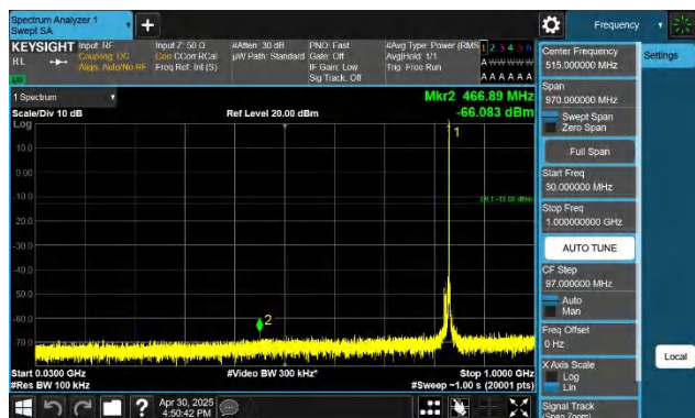
5-5-10MHz-10MHz-QPSK-QPSK-20450-20549-1RB#49-0RB#0-3 0~1000MHz-PASS
