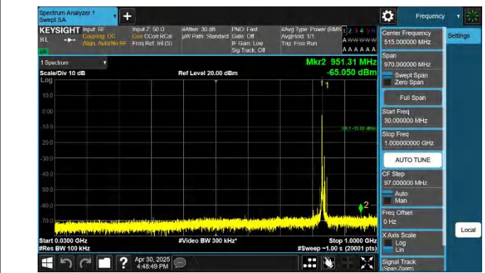
5-5-10MHz-5MHz-QPSK-QPSK-20550-20622-1RB#0-ORB#0-30~ 1000MHz-PASS
