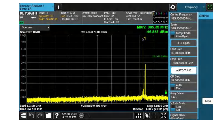
5-5-10MHz-10MHz-QPSK-QPSK-20476-20575-1RB#0-1RB#49-3 0~1000MHz-PASS
