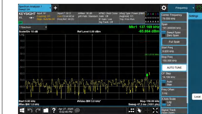
5-5-10MHz-10MHz-QPSK-QPSK-20476-20575-1RB#0-1RB#49-0 .009~0.15MHz-PASS
