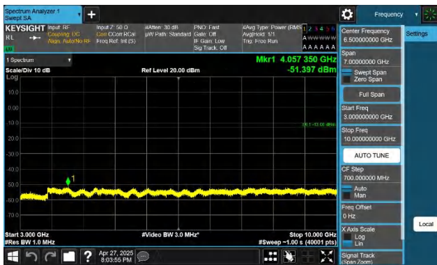
5-5-10MHz-10MHz-QPSK-QPSK-20501-20600-1RB#0-0RB#0-30 00~10000MHz-PASS
