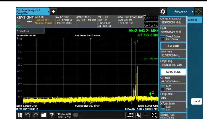
5-5-5MHz-10MHz-QPSK-QPSK-20528-20600-1RB#0-1RB#49-30 ~1000MHz-PASS
