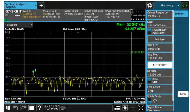
5-5-5MHz-10MHz-QPSK-QPSK-20478-20550-1RB#24-0RB#0-0. 009~0.15MHz-PASS
