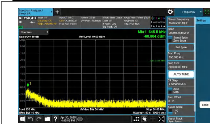
5-5-5MHz-10MHz-QPSK-QPSK-20528-20600-1RB#0-1RB#49-0. 15~30MHz-PASS
