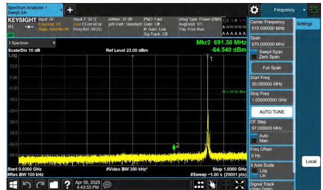
5-5-5MHz-10MHz-QPSK-QPSK-20478-20550-1RB#24-0RB#0-30 ~1000MHz-PASS
