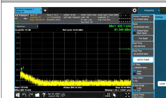
5-5-5MHz-10MHz-QPSK-QPSK-20478-20550-1RB#0-ORB#0-0.1 5~30MHz-PASS
