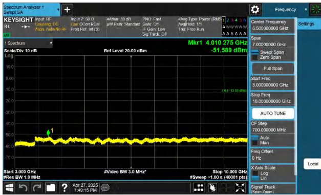
5-5-5MHz-10MHz-QPSK-QPSK-20478-20550-1RB#0-1RB#49-30 00~10000MHz-PASS
