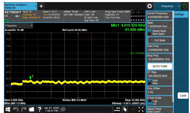
5-5-5MHz-10MHz-QPSK-QPSK-20478-20550-1RB#24-0RB#0-30 00~10000MHz-PASS
