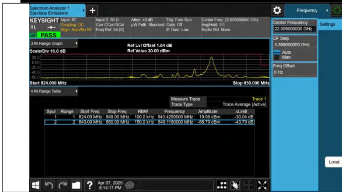
5-5-10MHz-5MHz-QPSK@QPSK-QPSK@QPSK-20550-20622-1 RB#49@50RB#0-0RB#0@25RB#0-PASS
