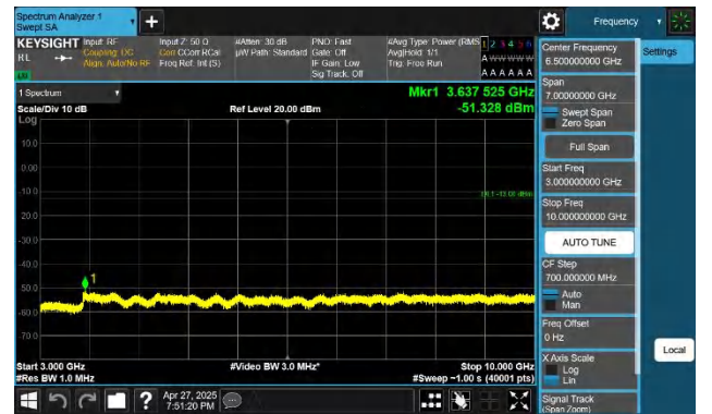
5-5-5MHz-10MHz-QPSK-QPSK-20528-20600-1RB#0-1RB#49-30 00~10000MHz-PASS
