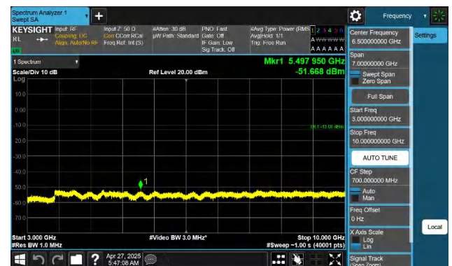
Band71-15MHz-QPSK-133197-1RB#74-3000~10000-PASS
