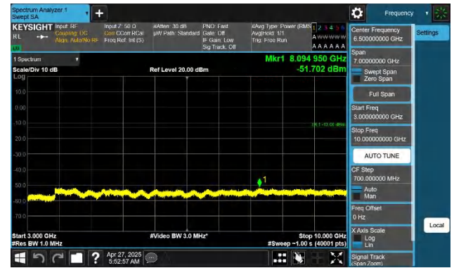
Band71-20MHz-QPSK-133322-1RB#99-3000~10000-PASS
