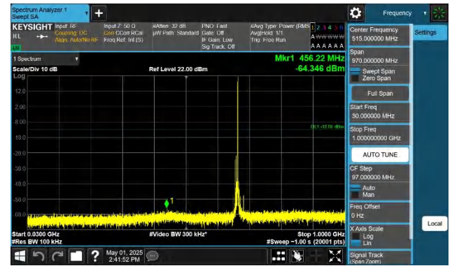
Band71-10MHz-QPSK-133172-1RB#49-30~1000-PASS
