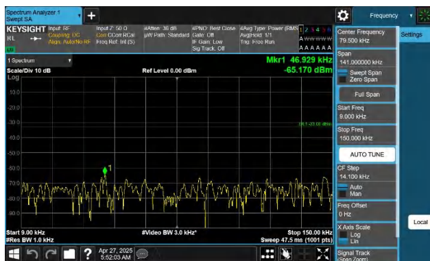
Band71-20MHz-QPSK-133322-1RB#0-0.009~0.15-PASS
