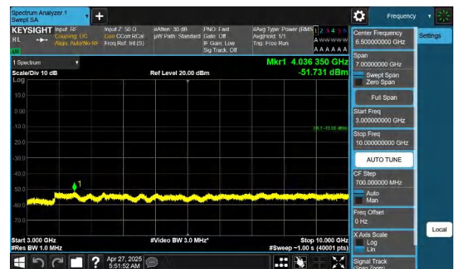
Band71-20MHz-QPSK-133222-1RB#99-3000~10000-PASS
