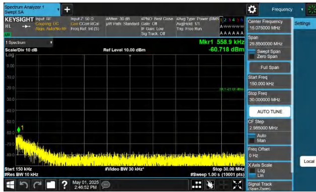
Band71-10MHz-QPSK-133172-1RB#49-0.15~30-PASS
