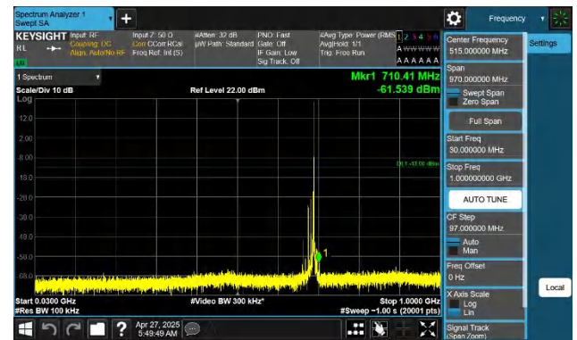
Band71-15MHz-QPSK-133397-1RB#74-30~1000-PASS
