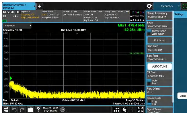
Band71-20MHz-QPSK-133222-1RB#99-0.15~30-PASS
