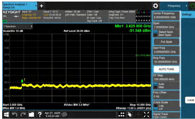
Band71-15MHz-QPSK-133397-1RB#0-3000~10000-PASS
