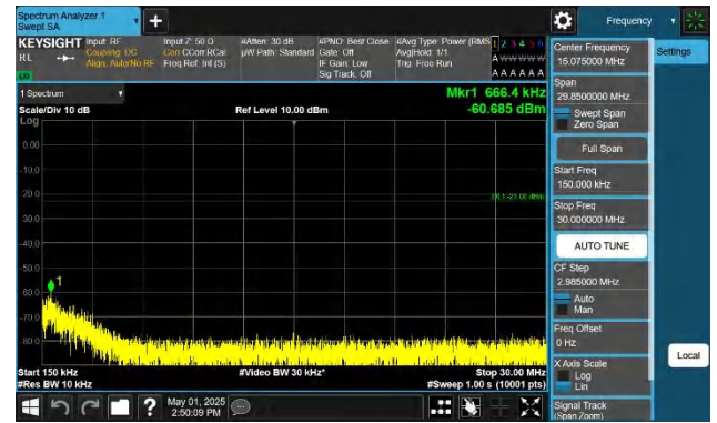
Band71-20MHz-QPSK-133222-1RB#0-0.15~30-PASS
