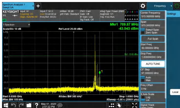
Band71-20MHz-QPSK-133322-1RB#0-30~1000-PASS
