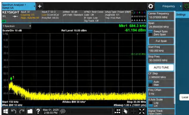
Band71-15MHz-QPSK-133297-1RB#74-0.15~30-PASS
