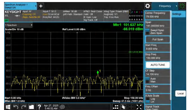
Band71-15MHz-QPSK-133197-1RB#74-0.009~0.15-PASS
