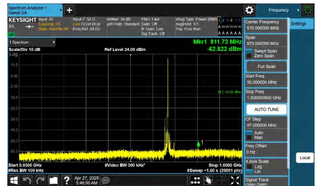
Band71-15MHz-QPSK-133197-1RB#74-30~1000-PASS
