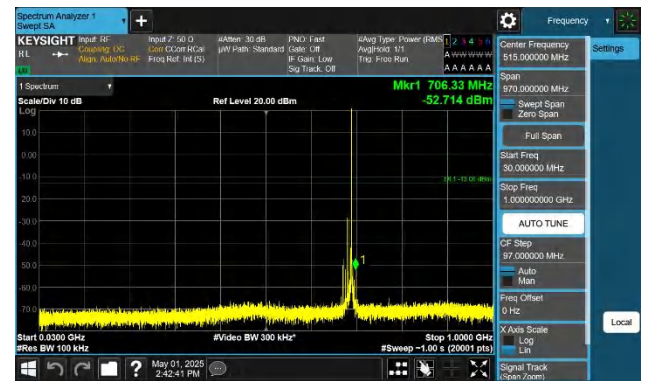
Band71-10MHz-QPSK-133422-1RB#49-30~1000-PASS
