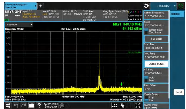
Band71-15MHz-QPSK-133297-1RB#74-30~1000-PASS
