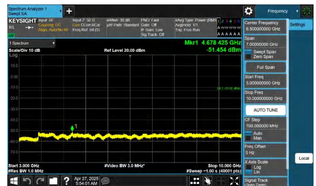
Band71-20MHz-QPSK-133372-1RB#99-3000~10000-PASS
