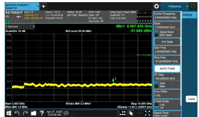
Band71-15MHz-QPSK-133397-1RB#74-3000~10000-PASS
