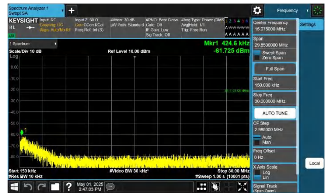
Band71-10MHz-QPSK-133297-1RB#0-0.15~30-PASS
