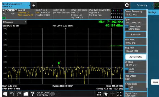
Band71-10MHz-QPSK-133297-1RB#0-0.009~0.15-PASS
