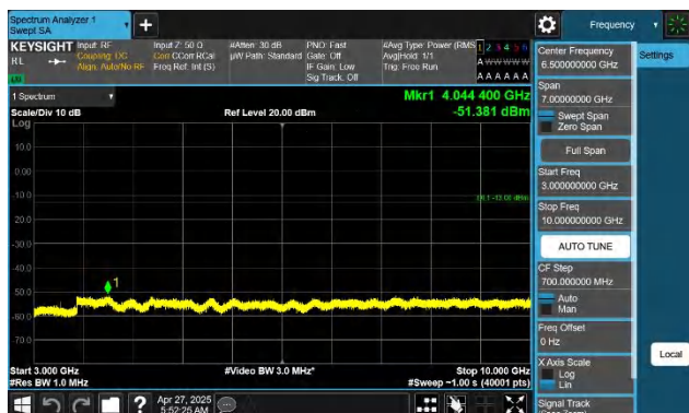
Band71-20MHz-QPSK-133322-1RB#0-3000~10000-PASS
