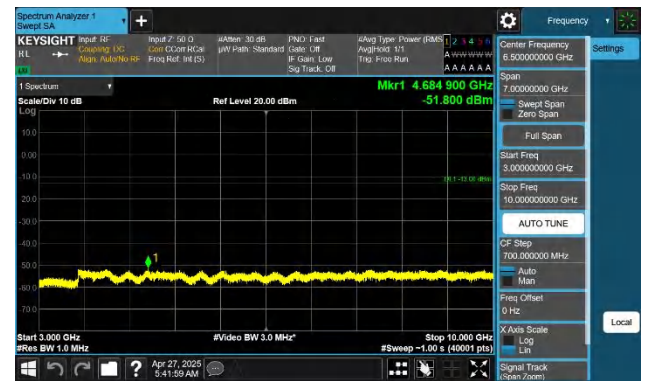
Band71-10MHz-QPSK-133172-1RB#49-3000~10000-PASS
