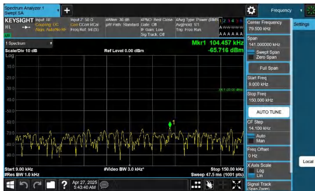
Band71-10MHz-QPSK-133422-1RB#0-0.009~0.15-PASS
