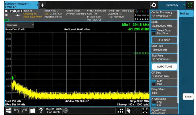
Band71-15MHz-QPSK-133197-1RB#0-0.15~30-PASS
