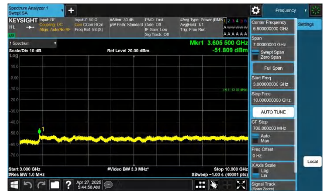
Band71-10MHz-QPSK-133422-1RB#49-3000~10000-PASS
