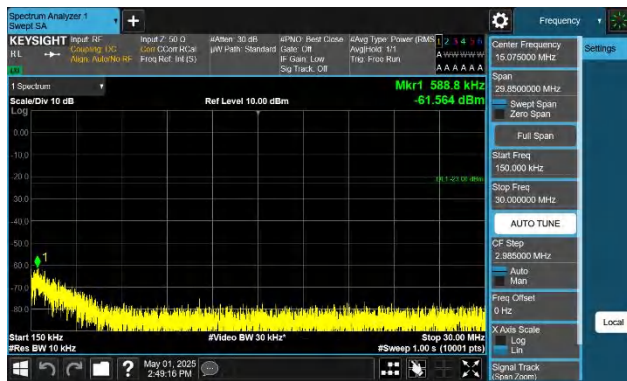
Band71-15MHz-QPSK-133397-1RB#74-0.15~30-PASS
