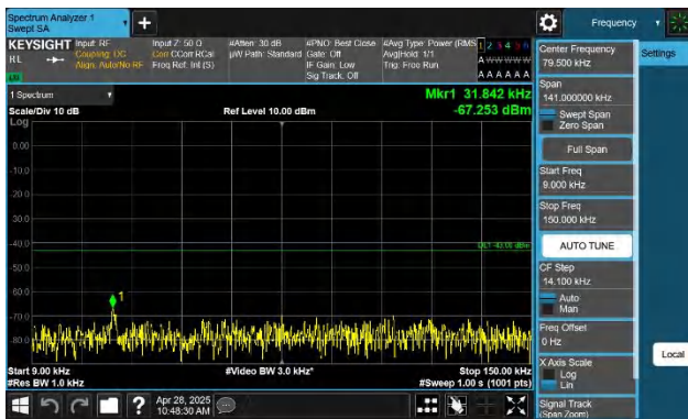
Band66-10MHz-QPSK-132622-1RB#0-0.009~0.15-PASS
