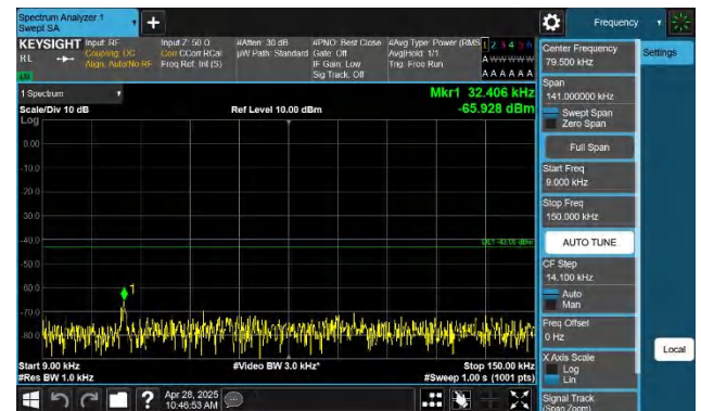
Band66-5MHz-QPSK-131997-1RB#24-0.009~0.15-PASS
