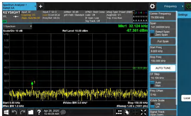
Band66-10MHz-QPSK-132322-1RB#0-0.009~0.15-PASS
