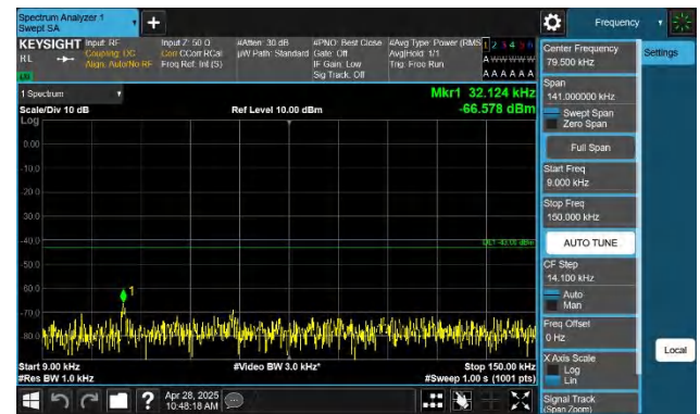
Band66-10MHz-QPSK-132322-1RB#49-0.009~0.15-PASS
