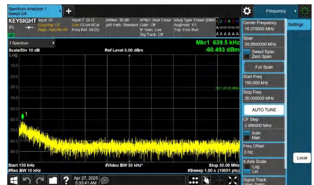
Band66-20MHz-QPSK-132572-1RB#0-0.15~30-PASS
