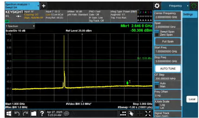
Band66-10MHz-QPSK-132322-1RB#0-1000~3000-PASS
