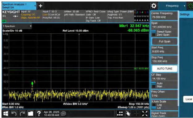
Band66-20MHz-QPSK-132072-1RB#0-0.009~0.15-PASS
