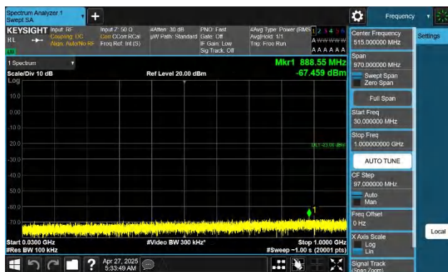
Band66-20MHz-QPSK-132572-1RB#0-30~1000-PASS
