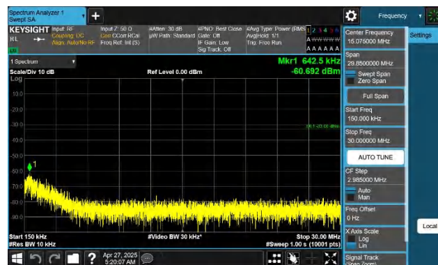
Band66-5MHz-QPSK-132647-1RB#0-0.15~30-PASS
