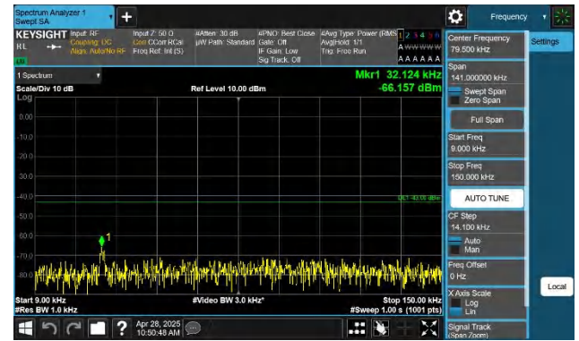
Band66-20MHz-QPSK-132572-1RB#99-0.009~0.15-PASS
