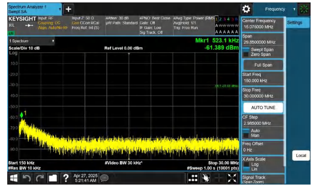
Band66-10MHz-QPSK-132022-1RB#0-0.15~30-PASS
