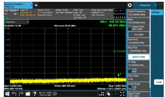
Band66-20MHz-QPSK-132572-1RB#99-30~1000-PASS
