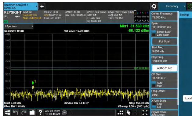
Band66-15MHz-QPSK-132597-1RB#74-0.009~0.15-PASS
