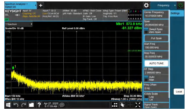
Band66-5MHz-QPSK-131997-1RB#0-0.15~30-PASS
