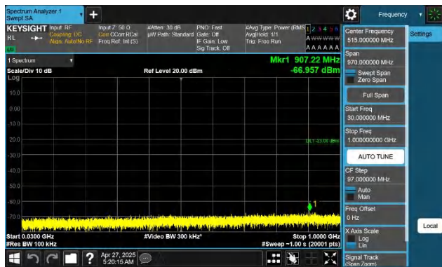
Band66-5MHz-QPSK-132647-1RB#0-30~1000-PASS
