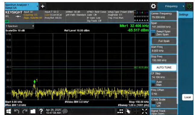
Band66-10MHz-QPSK-132022-1RB#49-0.009~0.15-PASS
