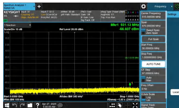
Band66-15MHz-QPSK-132597-1RB#74-30~1000-PASS
