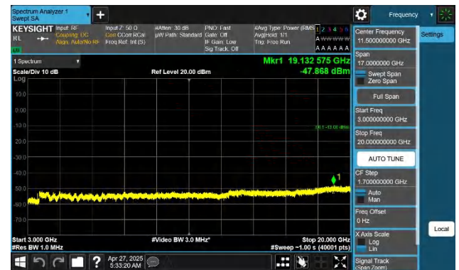
Band66-20MHz-QPSK-132322-1RB#99-3000~20000-PASS
