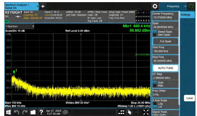
Band66-15MHz-QPSK-132322-1RB#0-0.15~30-PASS
