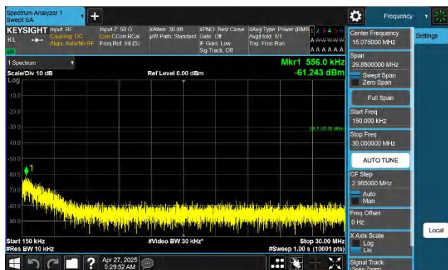
Band66-15MHz-QPSK-132597-1RB#74-0.15~30-PASS
