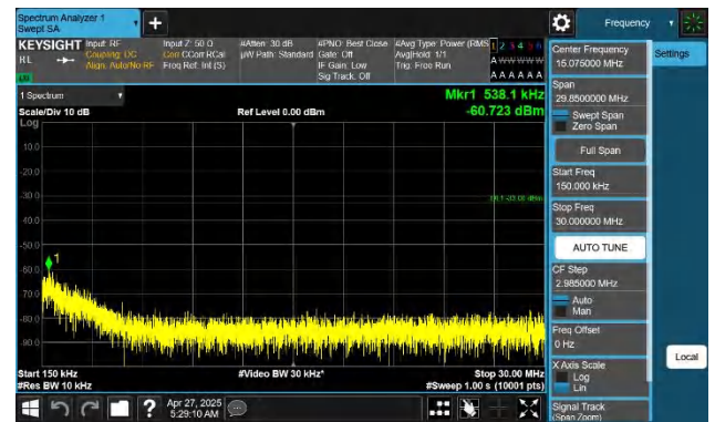
Band66-15MHz-QPSK-132597-1RB#0-0.15~30-PASS
