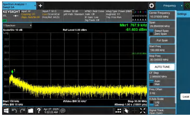
Band66-10MHz-QPSK-132022-1RB#49-0.15~30-PASS
