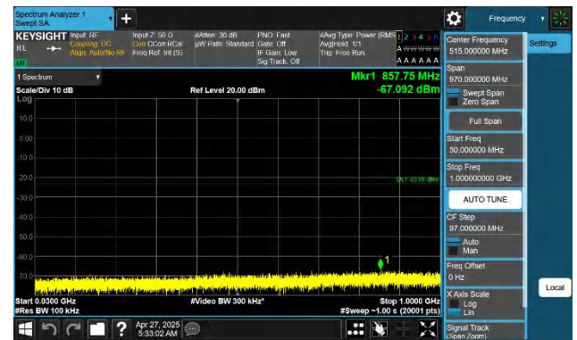
Band66-20MHz-QPSK-132322-1RB#99-30~1000-PASS
