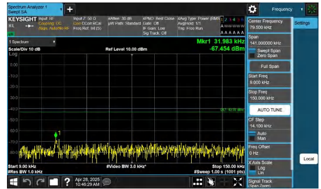
Band66-3MHz-QPSK-132657-1RB#14-0.009~0.15-PASS
