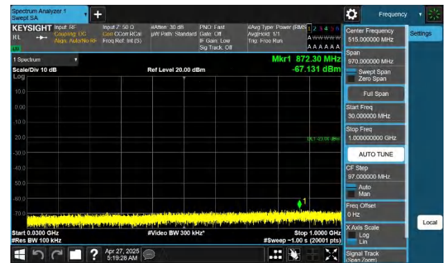
Band66-5MHz-QPSK-132322-1RB#24-30~1000-PASS
