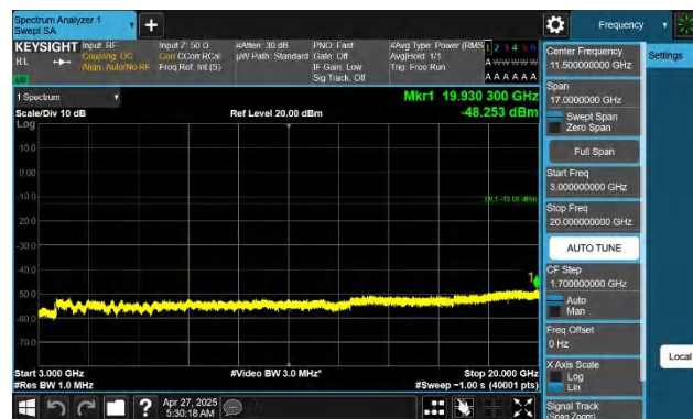
Band66-15MHz-QPSK-132597-1RB#74-3000~20000-PASS
