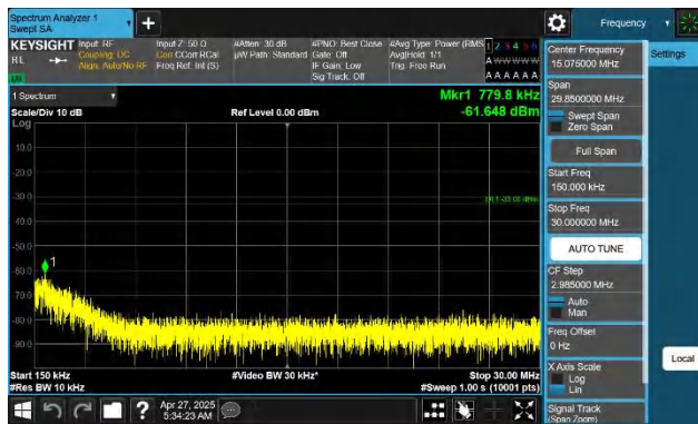
Band66-20MHz-QPSK-132572-1RB#99-0.15~30-PASS
