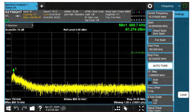
Band66-10MHz-QPSK-132322-1RB#0-0.15~30-PASS
