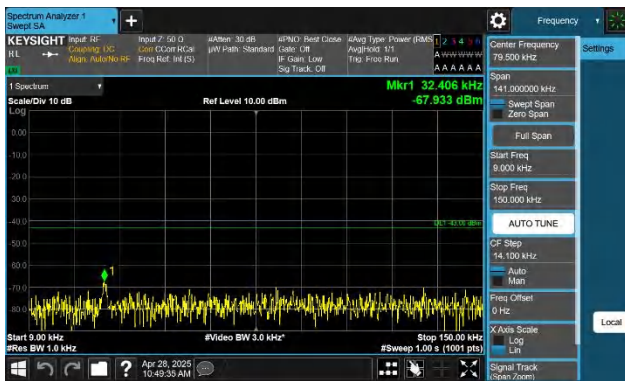
Band66-15MHz-QPSK-132597-1RB#0-0.009~0.15-PASS
