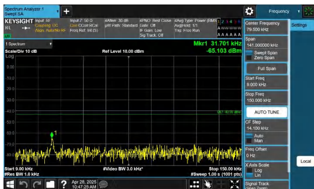
Band66-5MHz-QPSK-132647-1RB#0-0.009~0.15-PASS
