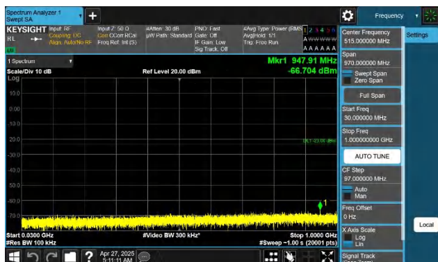
Band66-1.4MHz-QPSK-132665-1RB#0-30~1000-PASS
