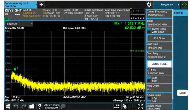
Band66-1.4MHz-QPSK-131979-1RB#0-0.15~30-PASS
