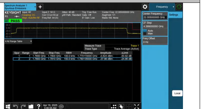
Band66-15MHz-QPSK-132597-75RB#0-PASS
