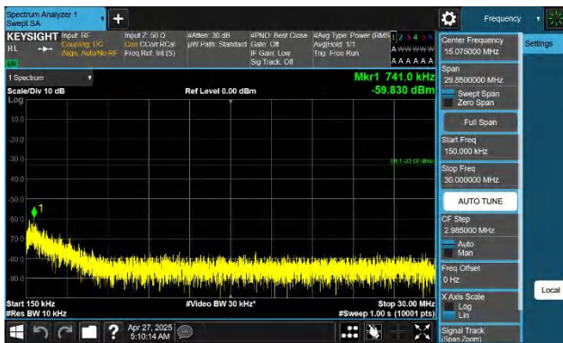
Band66-1.4MHz-QPSK-132322-1RB#5-0.15~30-PASS
