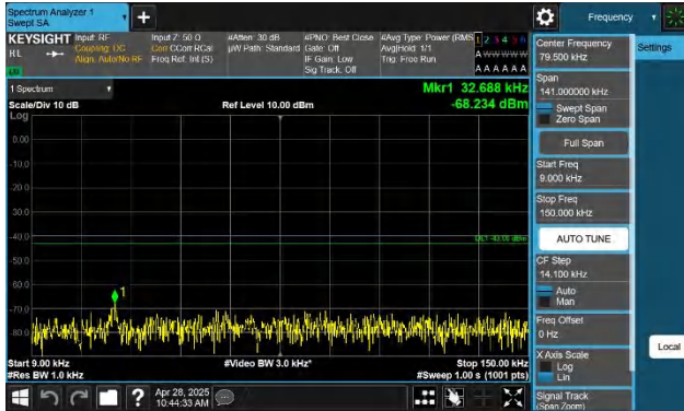
Band66-1.4MHz-QPSK-131979-1RB#0-0.009~0.15-PASS
