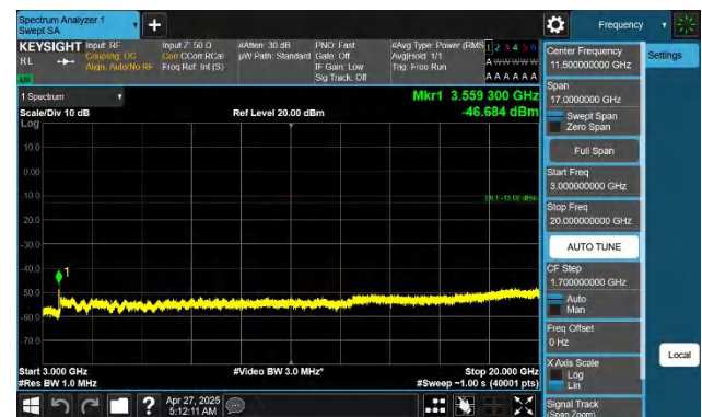
Band66-1.4MHz-QPSK-132665-1RB#5-3000~20000-PASS
