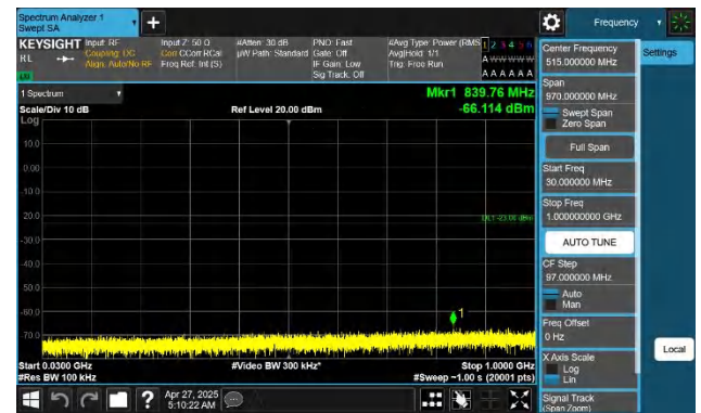
Band66-1.4MHz-QPSK-132322-1RB#5-30~1000-PASS
