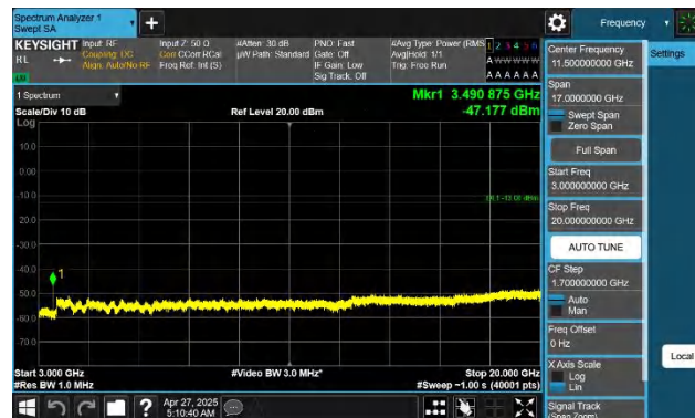
Band66-1.4MHz-QPSK-132322-1RB#5-3000~20000-PASS
