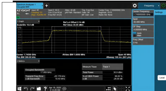
Band66-20MHz-64QAM-132322-100RB#0-PASS
