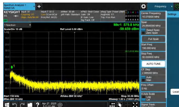
Band66-1.4MHz-QPSK-132665-1RB#0-0.15~30-PASS
