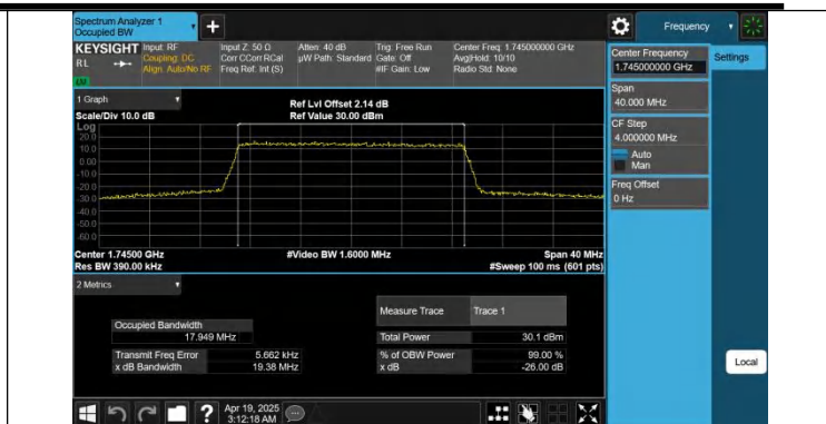
Band66-20MHz-16QAM-132322-100RB#0-PASS
