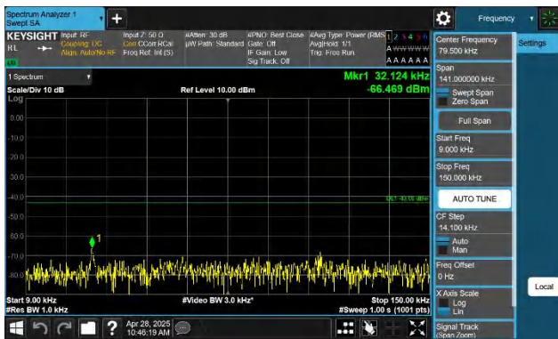
Band66-3MHz-QPSK-132657-1RB#0-0.009~0.15-PASS
