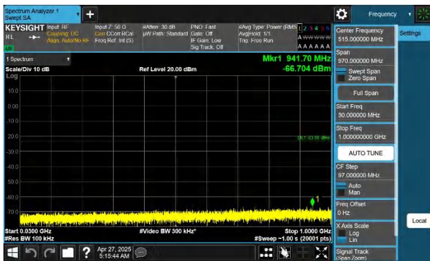
Band66-3MHz-QPSK-132657-1RB#0-30~1000-PASS
