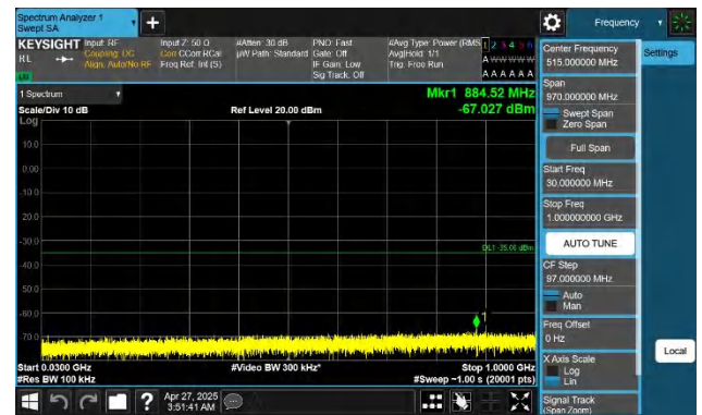
Band41-10MHz-QPSK-40620-1RB#49-30~1000-PASS
