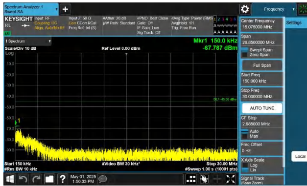
Band41-10MHz-QPSK-39700-1RB#49-0.15~30-PASS
