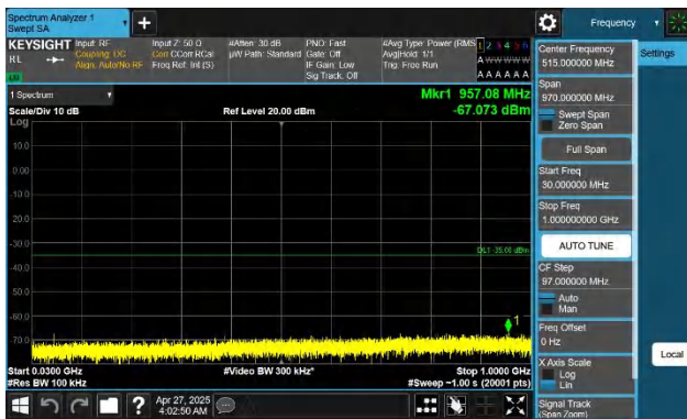
Band41-20MHz-QPSK-41490-1RB#0-30~1000-PASS
