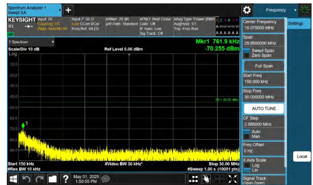
Band41-10MHz-QPSK-40620-1RB#0-0.15~30-PASS
