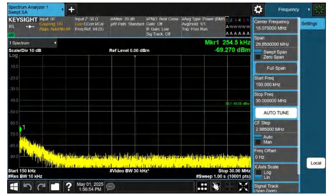
Band41-15MHz-QPSK-39725-1RB#0-0.15~30-PASS
