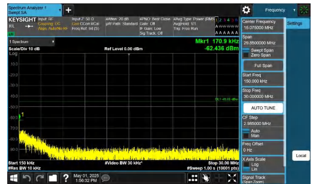
Band41-10MHz-QPSK-41540-1RB#0-0.15~30-PASS
