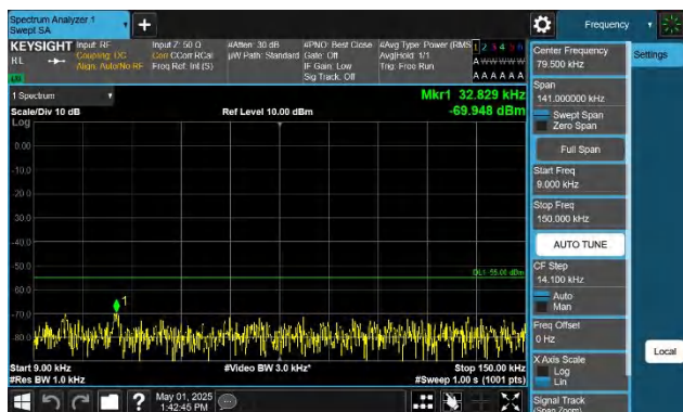
Band41-15MHz-QPSK-41515-1RB#0-0.009~0.15-PASS
