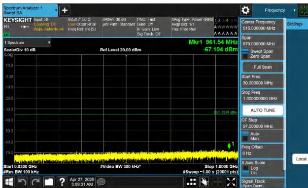
Band41-20MHz-QPSK-39750-1RB#0-30~1000-PASS
