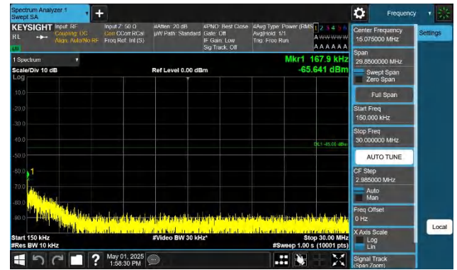
Band41-20MHz-QPSK-39750-1RB#0-0.15~30-PASS
