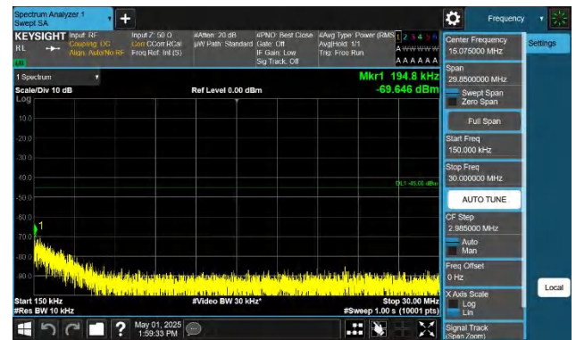
Band41-20MHz-QPSK-41490-1RB#0-0.15~30-PASS
