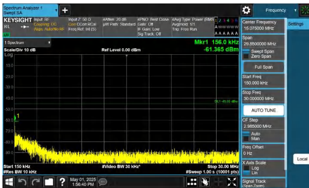
Band41-10MHz-QPSK-41540-1RB#49-0.15~30-PASS
