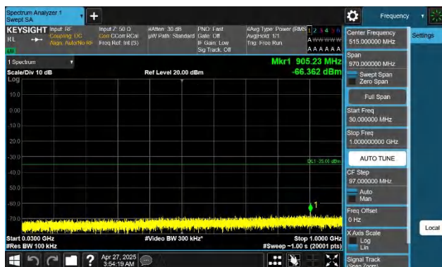
Band41-15MHz-QPSK-39725-1RB#0-30~1000-PASS
