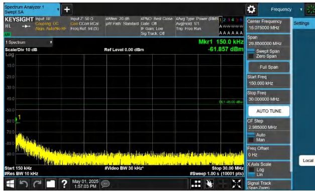
Band41-15MHz-QPSK-39725-1RB#74-0.15~30-PASS
