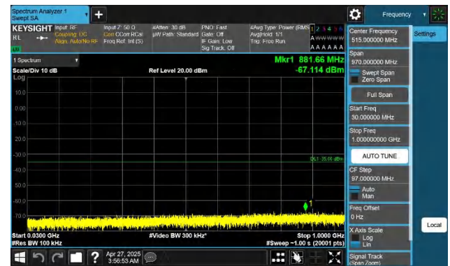
Band41-15MHz-QPSK-40620-1RB#74-30~1000-PASS
