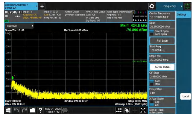
Band41-20MHz-QPSK-40620-1RB#0-0.15~30-PASS
