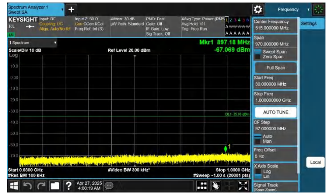
Band41-20MHz-QPSK-39750-1RB#99-30~1000-PASS
