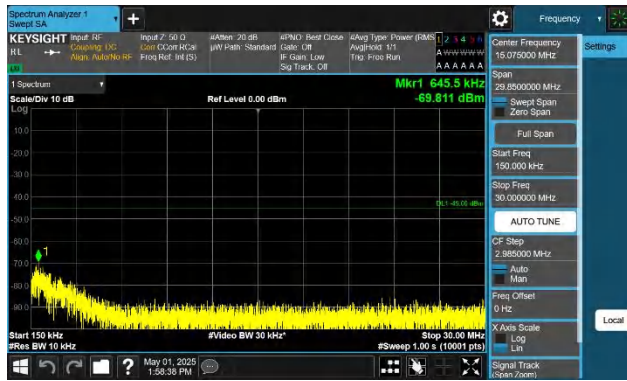
Band41-20MHz-QPSK-39750-1RB#99-0.15~30-PASS
