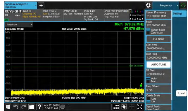
Band41-10MHz-QPSK-39700-1RB#49-30~1000-PASS
