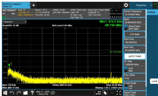
Band41-20MHz-QPSK-40620-1RB#99-0.15~30-PASS
