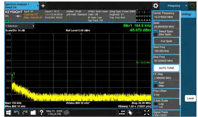
Band41-10MHz-QPSK-39700-1RB#0-0.15~30-PASS
