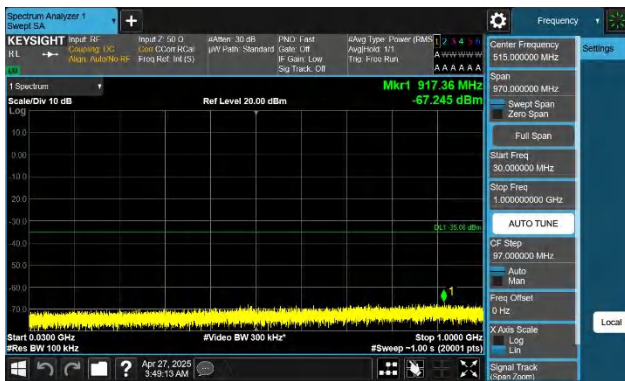
Band41-10MHz-QPSK-39700-1RB#0-30~1000-PASS
