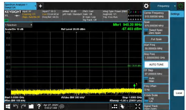
Band41-10MHz-QPSK-41540-1RB#49-30~1000-PASS
