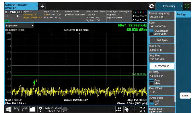
Band41-15MHz-QPSK-40620-1RB#74-0.009~0.15-PASS
