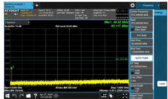
Band41-20MHz-QPSK-40620-1RB#99-30~1000-PASS
