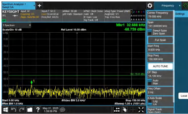
Band41-10MHz-QPSK-39700-1RB#0-0.009~0.15-PASS
