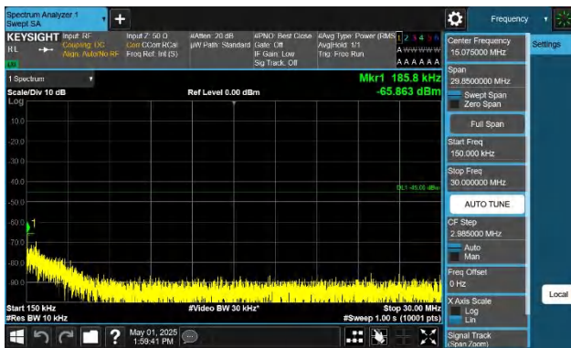
Band41-20MHz-QPSK-41490-1RB#99-0.15~30-PASS
