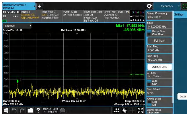
Band41-20MHz-QPSK-40620-1RB#0-0.009~0.15-PASS
