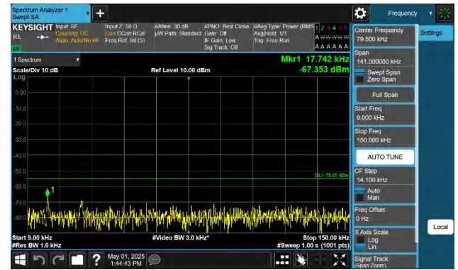
Band41-20MHz-QPSK-41490-1RB#99-0.009~0.15-PASS
