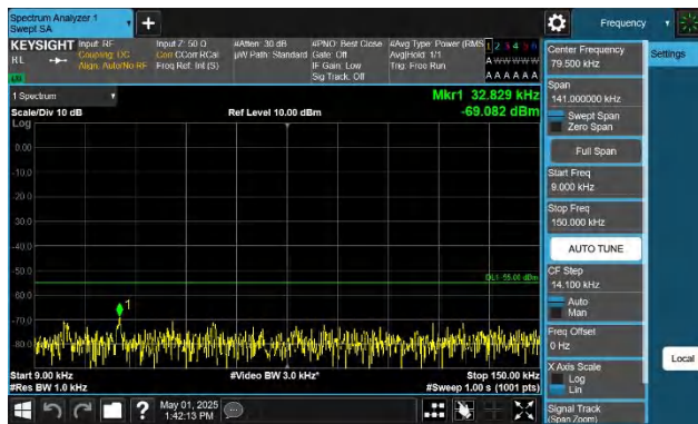
Band41-15MHz-QPSK-40620-1RB#0-0.009~0.15-PASS
