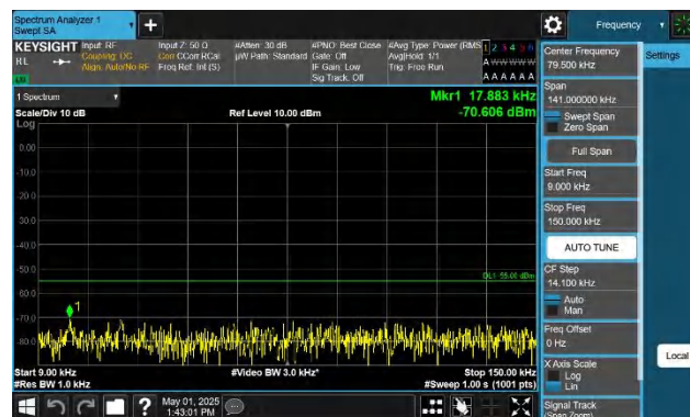
Band41-15MHz-QPSK-41515-1RB#74-0.009~0.15-PASS
