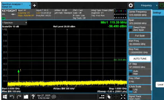
Band41-10MHz-QPSK-41540-1RB#0-30~1000-PASS
