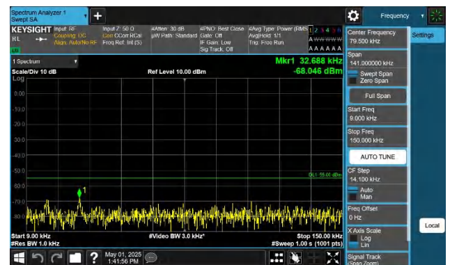
Band41-15MHz-QPSK-39725-1RB#74-0.009~0.15-PASS
