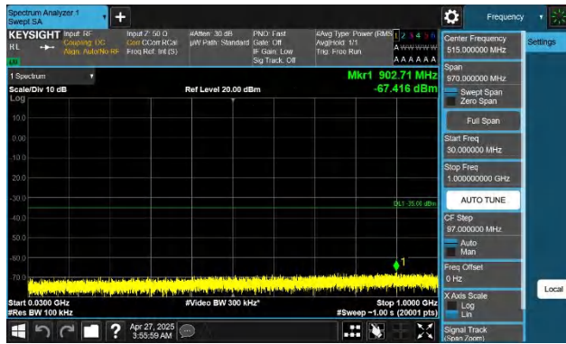
Band41-15MHz-QPSK-40620-1RB#0-30~1000-PASS
