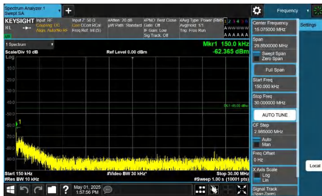
Band41-15MHz-QPSK-40620-1RB#74-0.15~30-PASS
