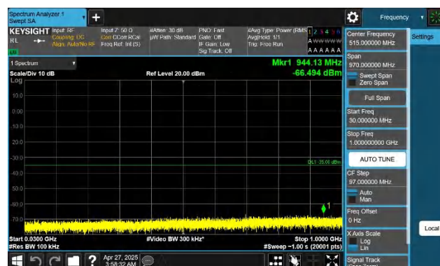
Band41-15MHz-QPSK-41515-1RB#74-30~1000-PASS
