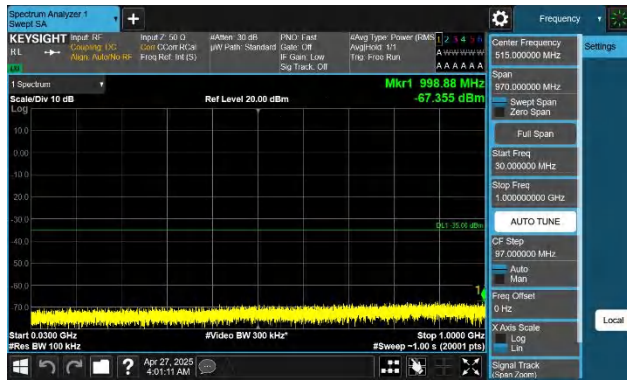
Band41-20MHz-QPSK-40620-1RB#0-30~1000-PASS
