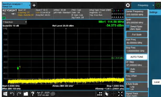
Band41-15MHz-QPSK-41515-1RB#0-30~1000-PASS
