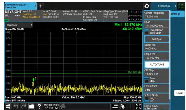
Band41-20MHz-QPSK-40620-1RB#99-0.009~0.15-PASS
