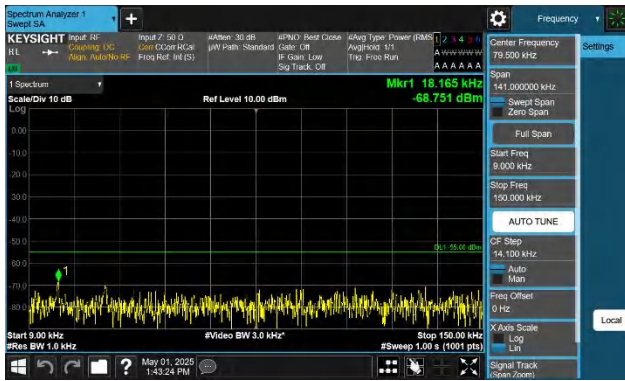
Band41-20MHz-QPSK-39750-1RB#0-0.009~0.15-PASS
