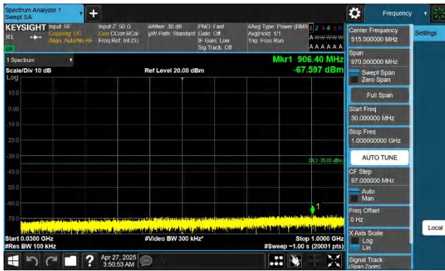
Band41-10MHz-QPSK-40620-1RB#0-30~1000-PASS
