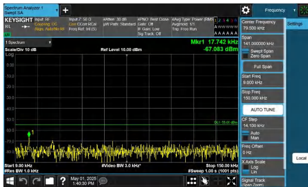
Band41-10MHz-QPSK-40620-1RB#0-0.009~0.15-PASS
