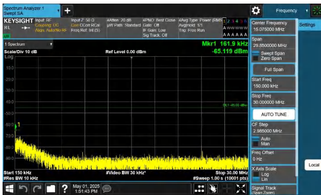
Band41-10MHz-QPSK-40620-1RB#49-0.15~30-PASS
