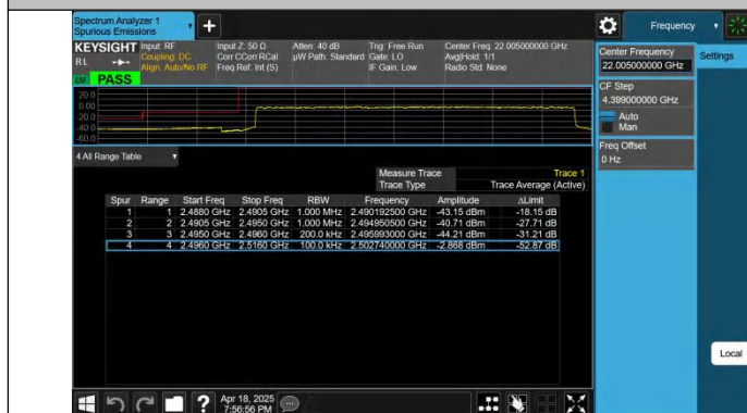
Band41-20MHz-QPSK-39750-100RB#0-PASS
