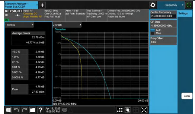
Band41-20MHz-QPSK-40620-1RB#0-PASS
