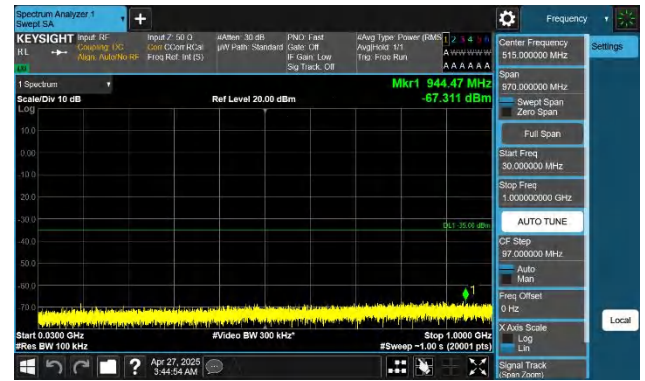
Band41-5MHz-QPSK-39675-1RB#24-30~1000-PASS
