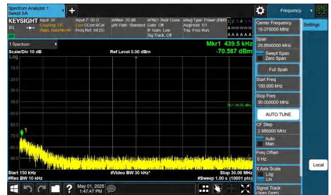
Band41-5MHz-QPSK-40620-1RB#0-0.15~30-PASS
