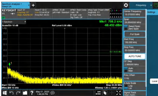
Band41-5MHz-QPSK-41565-1RB#24-0.15~30-PASS
