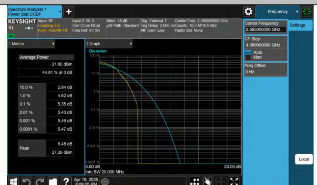
Band41-20MHz-16QAM-40620-1RB#0-PASS
