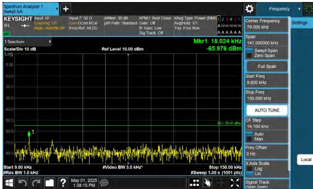
Band41-5MHz-QPSK-39675-1RB#0-0.009~0.15-PASS
