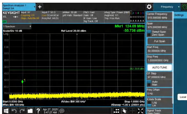
Band41-5MHz-QPSK-41565-1RB#0-30~1000-PASS
