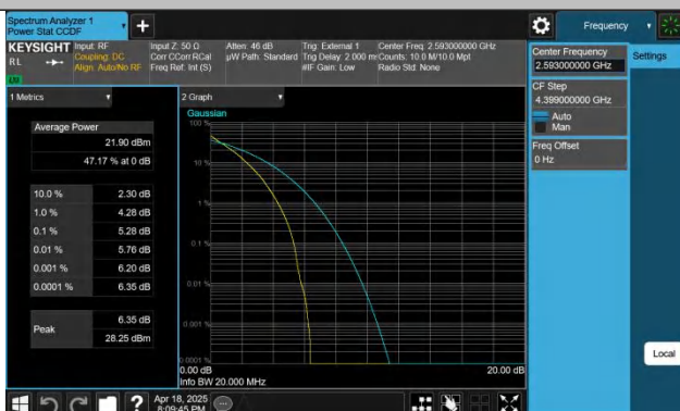
Band41-20MHz-64QAM-40620-100RB#0-PASS
