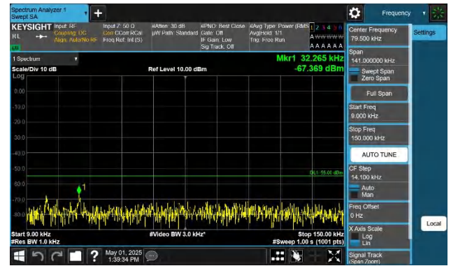
Band41-5MHz-QPSK-41565-1RB#24-0.009~0.15-PASS
