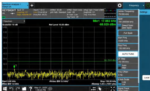
Band41-5MHz-QPSK-41565-1RB#0-0.009~0.15-PASS
