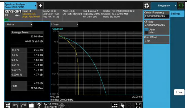
Band41-20MHz-64QAM-40620-1RB#0-PASS
