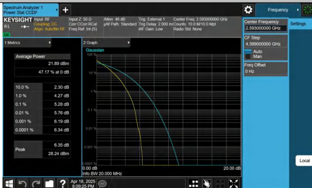
Band41-20MHz-QPSK-40620-100RB#0-PASS
