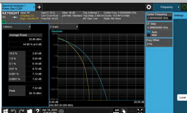
Band41-20MHz-16QAM-40620-100RB#0-PASS
