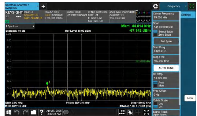
Band26(824-849)-15MHz-QPSK-26915-1RB#0-1000~3000-PASS
