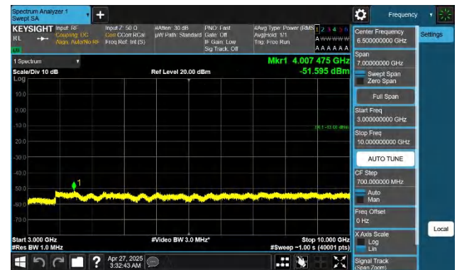
Band26(824-849)-15MHz-QPSK-26965-1RB#74-3000~10000-PAS S
