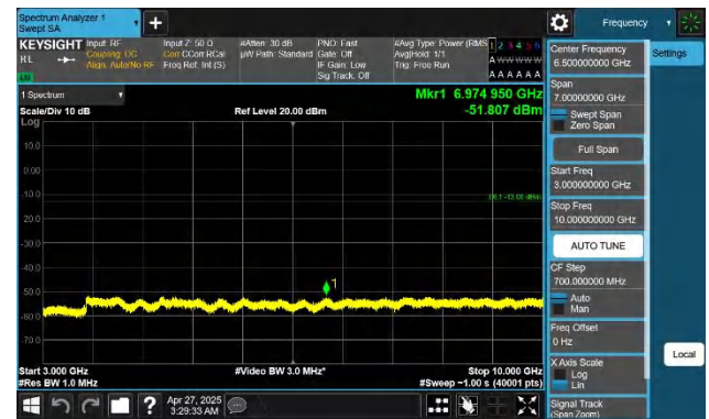
Band26(824-849)-15MHz-QPSK-26865-1RB#74-3000~10000-PAS
