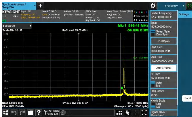
Band26(824-849)-15MHz-QPSK-26915-1RB#0-30~1000-PASS
