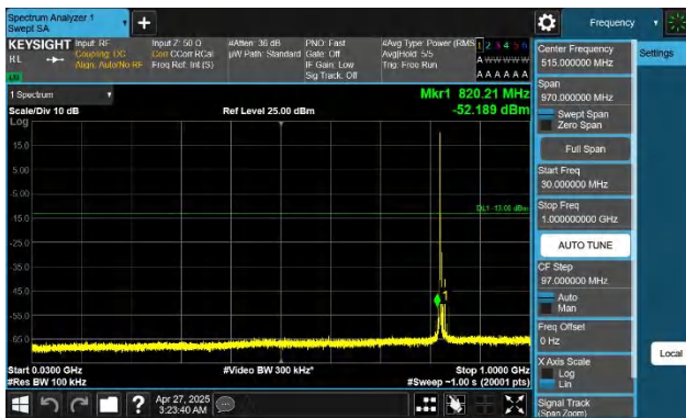
Band26(824-849)-10MHz-QPSK-26840-1RB#0-30~1000-PASS
