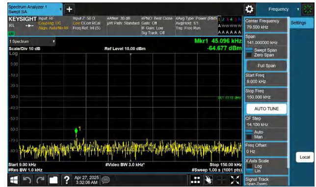
Band26(824-849)-15MHz-QPSK-26965-1RB#74-0.009~0.15-PASS
