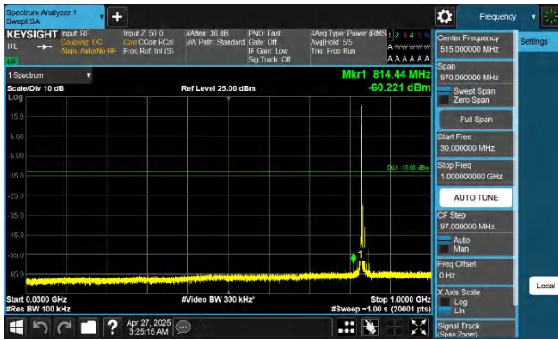
Band26(824-849)-10MHz-QPSK-26915-1RB#0-30~1000-PASS
