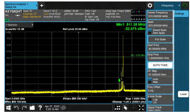
Band26(824-849)-15MHz-QPSK-26865-1RB#74-30~1000-PASS
