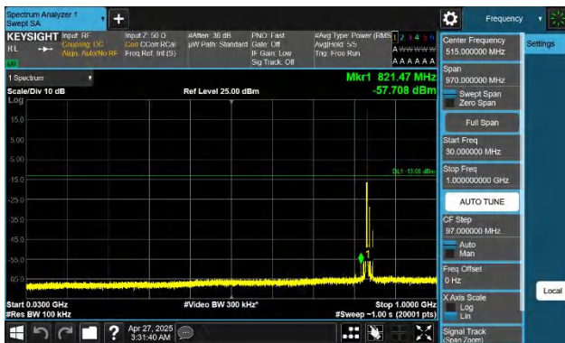
Band26(824-849)-15MHz-QPSK-26965-1RB#0-30~1000-PASS
