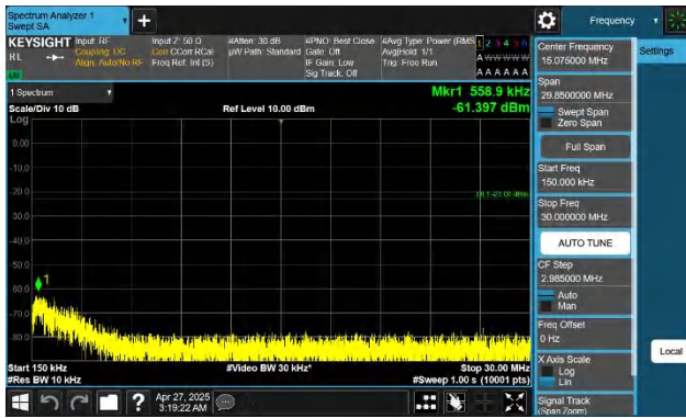
Band26(824-849)-5MHz-QPSK-26815-1RB#24-0.15~30-PASS
