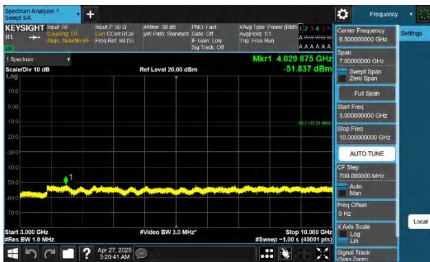
Band26(824-849)-5MHz-QPSK-26915-1RB#0-3000~10000-PASS
