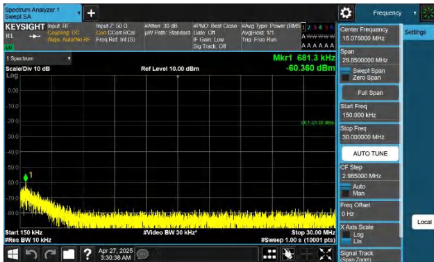
Band26(824-849)-15MHz-QPSK-26915-1RB#74-0.15~30-PASS
