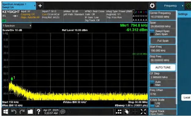
Band26(824-849)-5MHz-QPSK-26915-1RB#24-0.15~30-PASS
