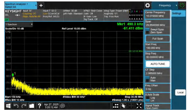
Band26(824-849)-5MHz-QPSK-26915-1RB#0-0.15~30-PASS
