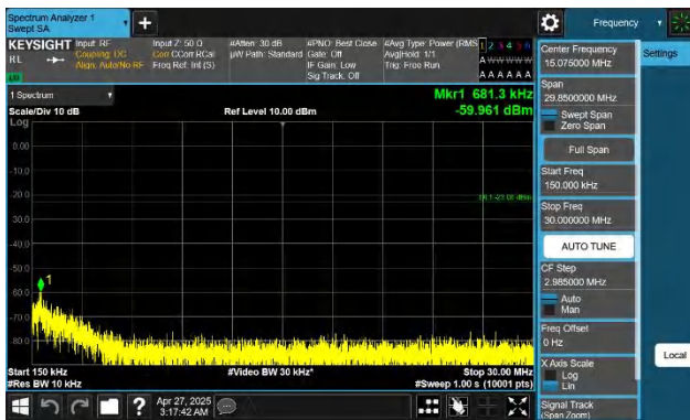
Band26(824-849)-3MHz-QPSK-27025-1RB#14-0.15~30-PASS
