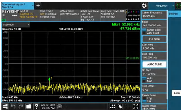
Band26(824-849)-15MHz-QPSK-26965-1RB#0-0.009~0.15-PASS
