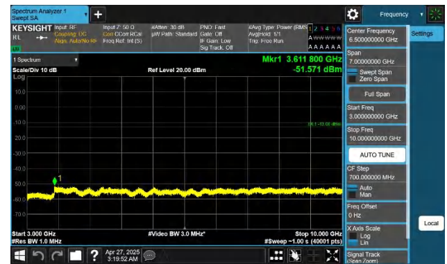
Band26(824-849)-5MHz-QPSK-26815-1RB#24-3000~10000-PASS
