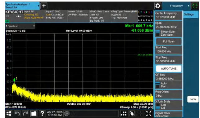
Band26(824-849)-5MHz-QPSK-26815-1RB#0-0.15~30-PASS
