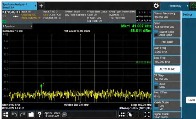
Band26(824-849)-5MHz-QPSK-26915-1RB#0-0.009~0.15-PASS
