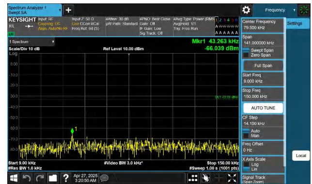
Band26(824-849)-5MHz-QPSK-26915-1RB#24-0.009~0.15-PASS
