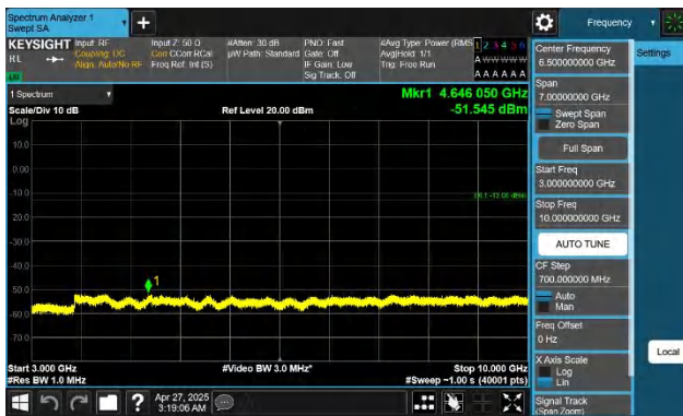
Band26(824-849)-5MHz-QPSK-26815-1RB#0-3000~10000-PASS
