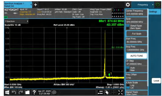
Band26(824-849)-5MHz-QPSK-26915-1RB#24-30~1000-PASS
