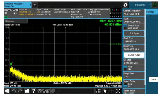
Band26(824-849)-15MHz-QPSK-26965-1RB#0-0.15~30-PASS
