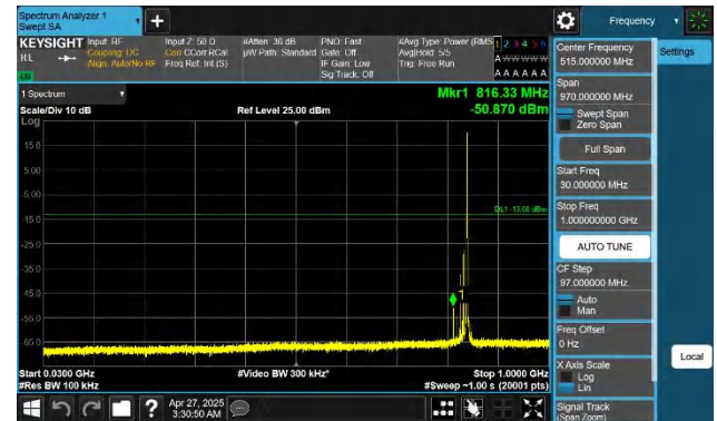
Band26(824-849)-15MHz-QPSK-26915-1RB#74-30~1000-PASS
