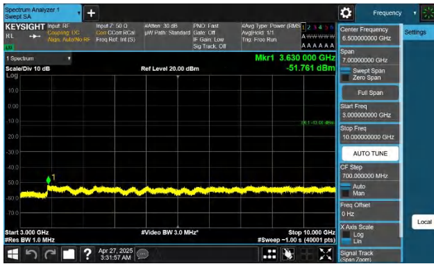
Band26(824-849)-15MHz-QPSK-26965-1RB#0-3000~10000-PAS S
