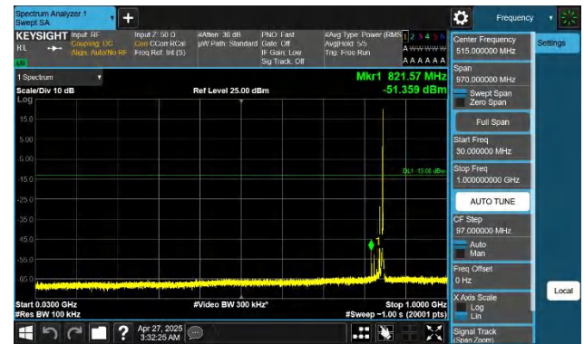
Band26(824-849)-15MHz-QPSK-26965-1RB#74-30~1000-PASS
