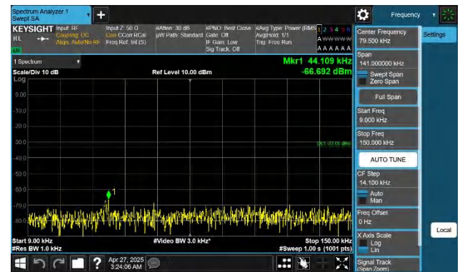
Band26(824-849)-10MHz-QPSK-26840-1RB#49-0.009~0.15-PASS
