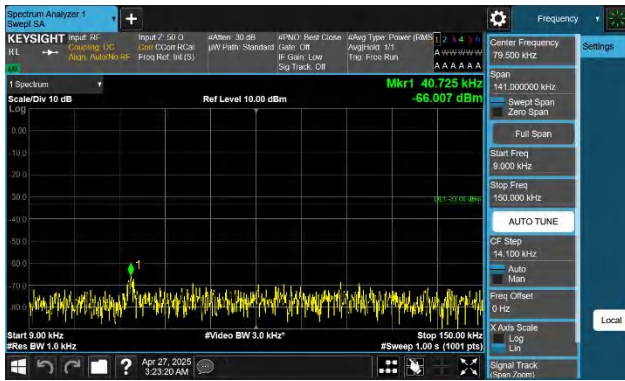
Band26(824-849)-10MHz-QPSK-26840-1RB#0-0.009~0.15-PASS
