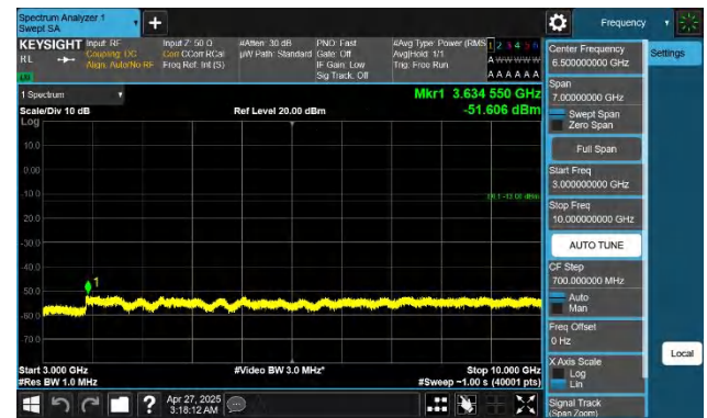
Band26(824-849)-3MHz-QPSK-27025-1RB#14-3000~10000-PASS
