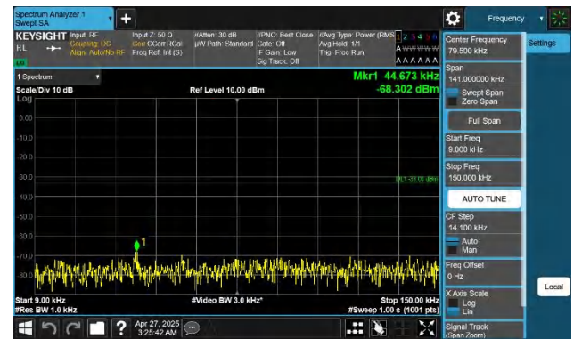
Band26(824-849)-10MHz-QPSK-26915-1RB#49-0.009~0.15-PASS
