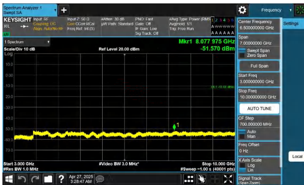
Band26(824-849)-15MHz-QPSK-26865-1RB#0-3000~10000-PASS
