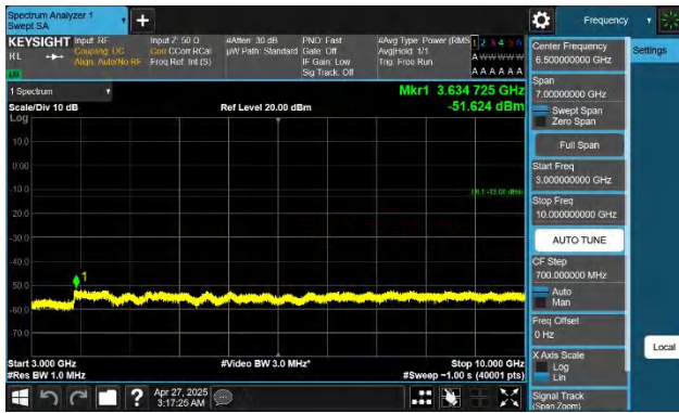
Band26(824-849)-3MHz-QPSK-27025-1RB#0-3000~10000-PASS
