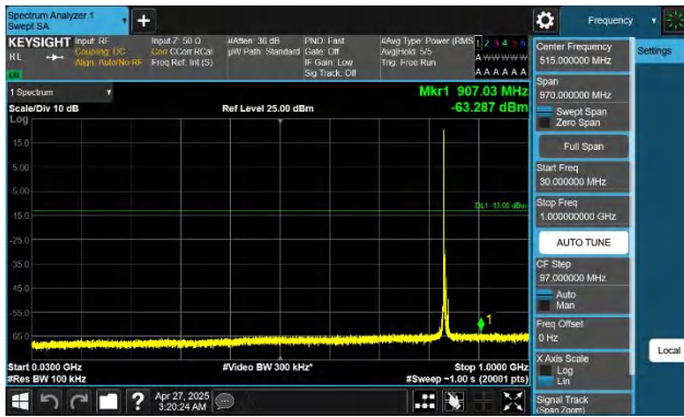
Band26(824-849)-5MHz-QPSK-26915-1RB#0-30~1000-PASS
