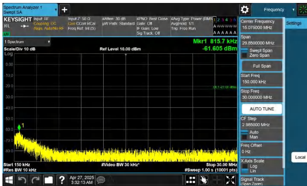
Band26(824-849)-15MHz-QPSK-26965-1RB#74-0.15~30-PASS
