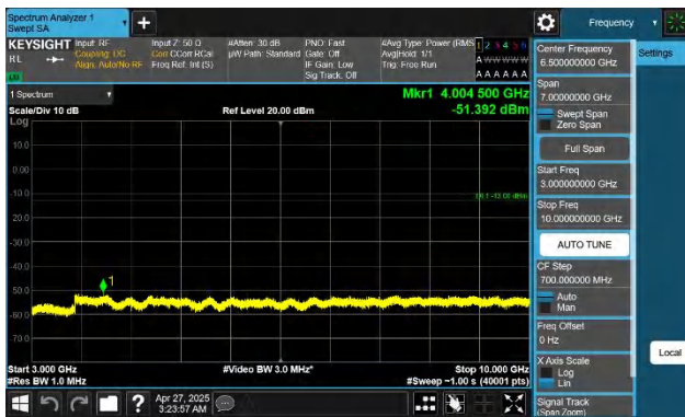
Band26(824-849)-10MHz-QPSK-26840-1RB#0-3000~10000-PAS
