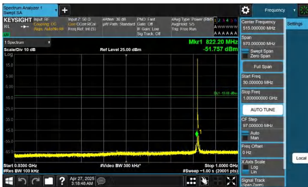
Band26(824-849)-5MHz-QPSK-26815-1RB#0-30~1000-PASS
