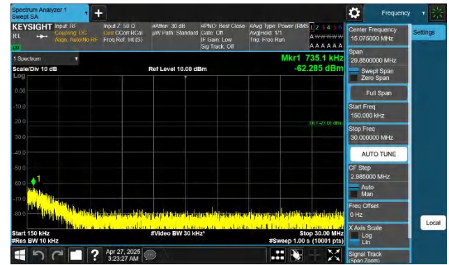
Band26(824-849)-10MHz-QPSK-26840-1RB#0-0.15~30-PASS
