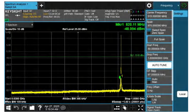
Band26(824-849)-5MHz-QPSK-26815-1RB#24-30~1000-PASS
