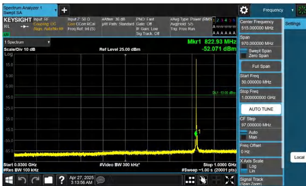
Band26(824-849)-3MHz-QPSK-26805-1RB#0-30~1000-PASS
