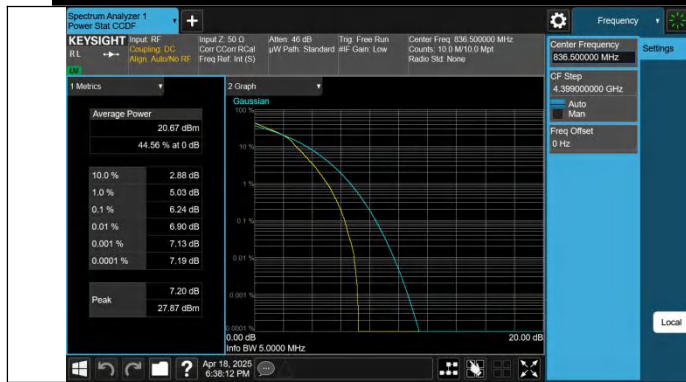
Band26(824-849)-5MHz-16QAM-26915-25RB#0-PASS
