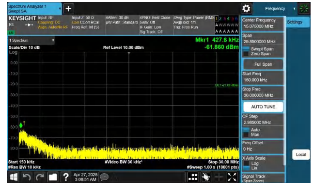
Band26(824-849)-1.4MHz-QPSK-26797-1RB#0-0.15~30-PASS
