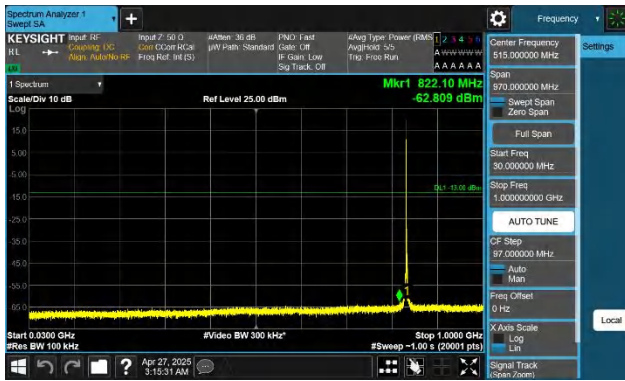
Band26(824-849)-3MHz-QPSK-26915-1RB#0-30~1000-PASS
