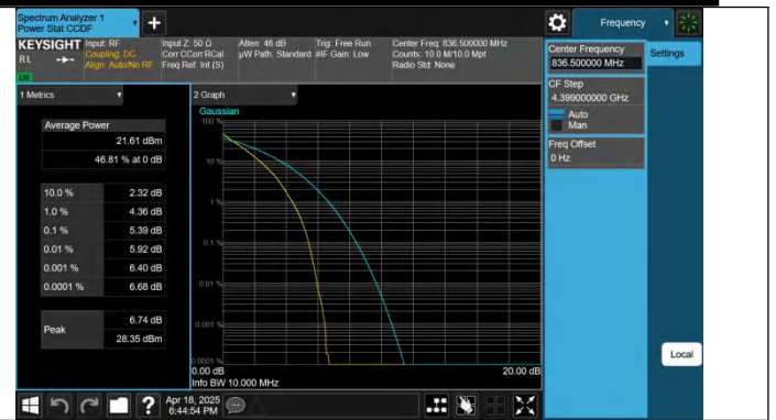
Band26(824-849)-10MHz-QPSK-26915-50RB#0-PASS
