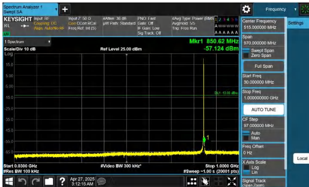
Band26(824-849)-1.4MHz-QPSK-27033-1RB#0-30~1000-PASS
