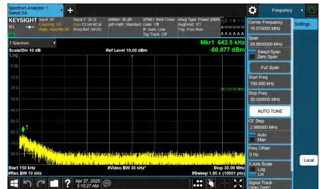
Band26(824-849)-1.4MHz-QPSK-26915-1RB#0-0.15~30-PASS
