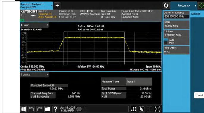
Band26(824-849)-5MHz-16QAM-26915-25RB#0-PASS
