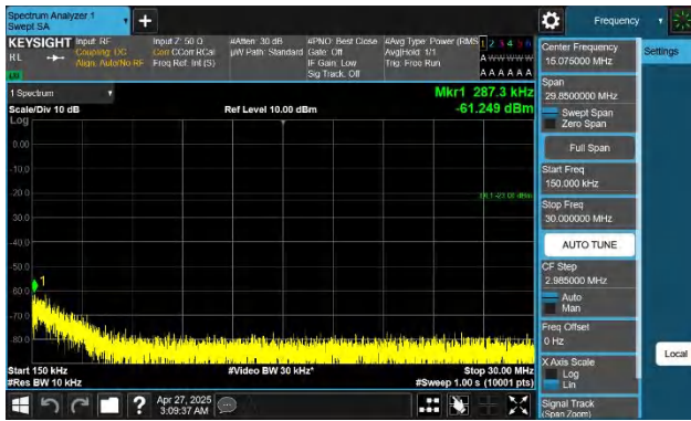
Band26(824-849)-1.4MHz-QPSK-26797-1RB#5-0.15~30-PASS
