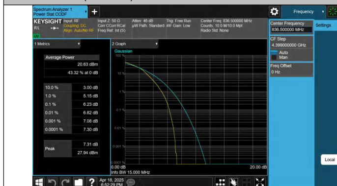
Band26(824-849)-15MHz-16QAM-26915-75RB#0-PASS
