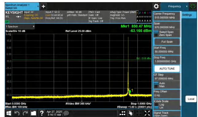
Band26(824-849)-3MHz-QPSK-26915-1RB#14-30~1000-PASS
