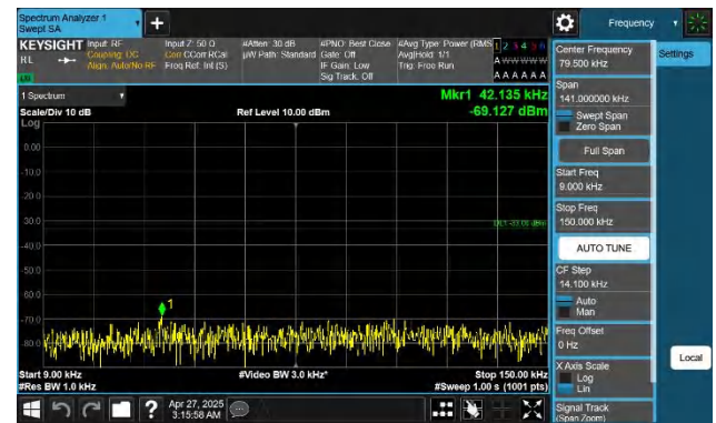
Band26(824-849)-3MHz-QPSK-26915-1RB#14-0.009~0.15-PASS
