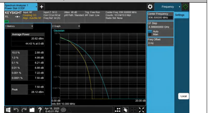
Band26(824-849)-10MHz-16QAM-26915-50RB#0-PASS
