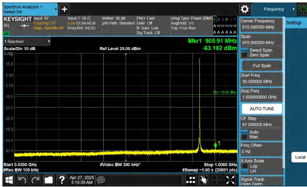
Band26(824-849)-1.4MHz-QPSK-26915-1RB#0-30~1000-PASS
