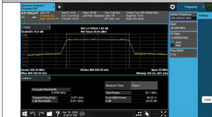
Band26(824-849)-10MHz-64QAM-26915-50RB#0-PASS
