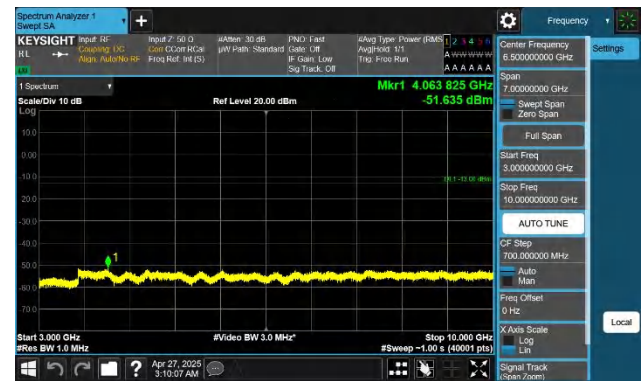
Band26(824-849)-1.4MHz-QPSK-26797-1RB#5-3000~10000-PASS
