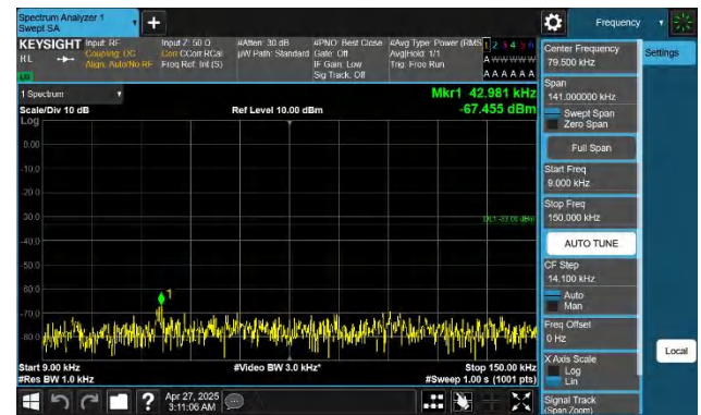
Band26(824-849)-1.4MHz-QPSK-26915-1RB#5-0.009~0.15-PASS
