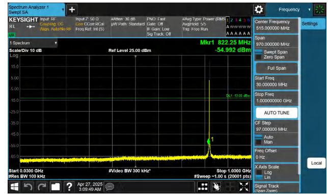
Band26(824-849)-1.4MHz-QPSK-26797-1RB#5-30~1000-PASS
