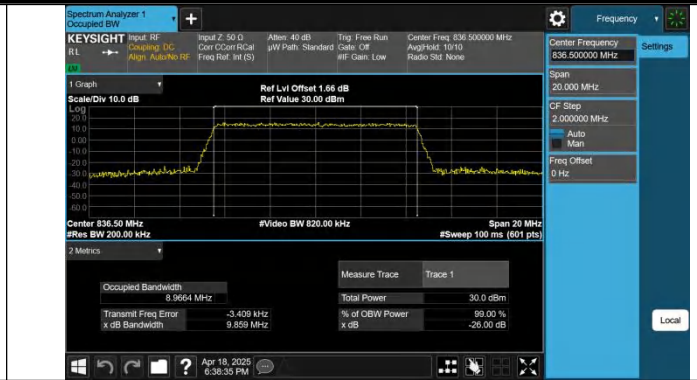
Band26(824-849)-10MHz-QPSK-26915-50RB#0-PASS
