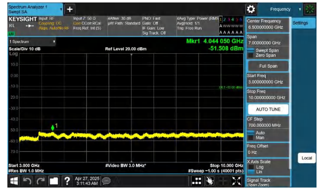
Band26(824-849)-1.4MHz-QPSK-26915-1RB#5-3000~10000-PASS S
