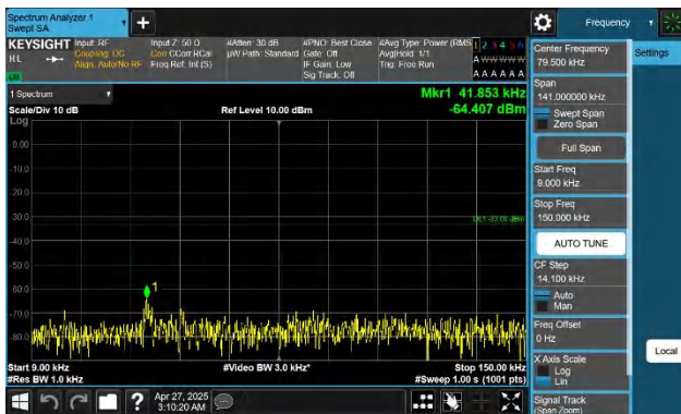
Band26(824-849)-1.4MHz-QPSK-26915-1RB#0-0.009~0.15-PASS
