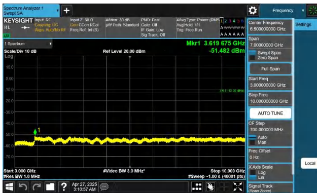
Band26(824-849)-1.4MHz-QPSK-26915-1RB#0-3000~10000-PAS
