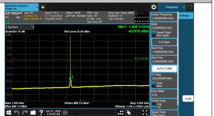
Band25-10MHz-QPSK-26090-1RB#0-1000~3000-PASS
