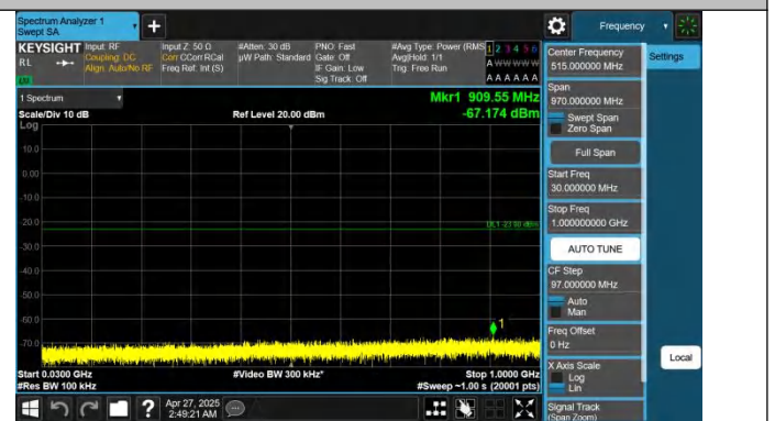
Band25-20MHz-QPSK-26140-1RB#99-30~1000-PASS
