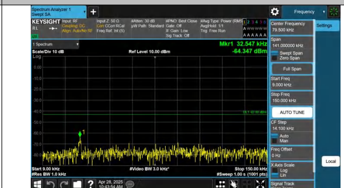
Band25-20MHz-QPSK-26590-1RB#99-0.009~0.15-PASS
