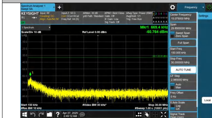
Band25-20MHz-QPSK-26140-1RB#99-0.15~30-PASS
