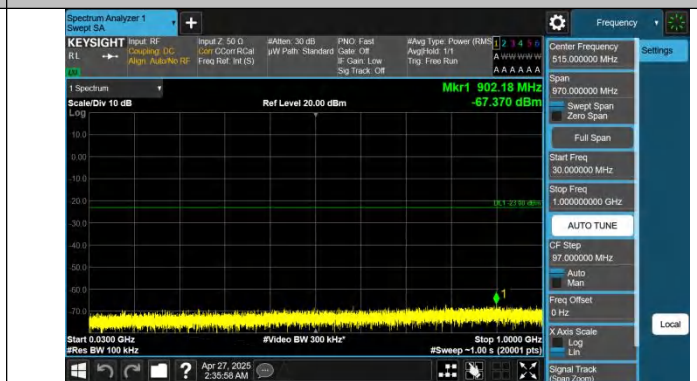
Band25-5MHz-QPSK-26065-1RB#24-30~1000-PASS
