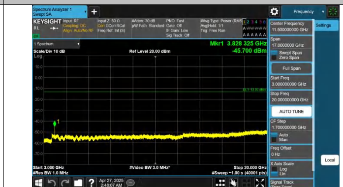
Band25-15MHz-QPSK-26615-1RB#74-3000~20000-PASS
