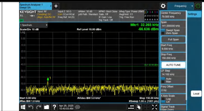
Band25-5MHz-QPSK-26065-1RB#24-0.009~0.15-PASS
