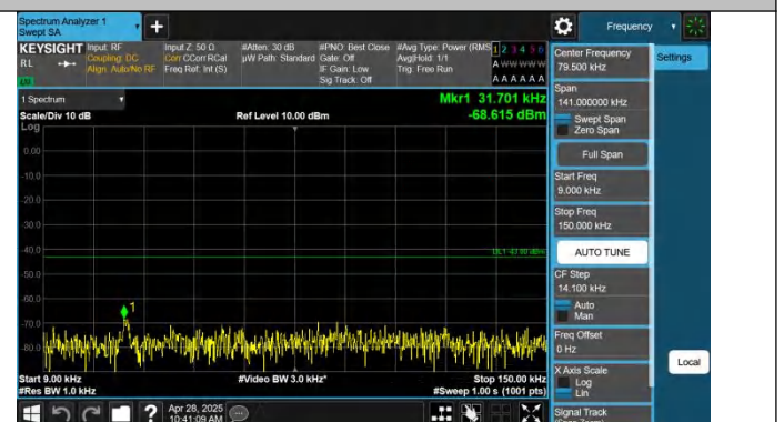
Band25-10MHz-QPSK-26090-1RB#49-0.009~0.15-PASS
