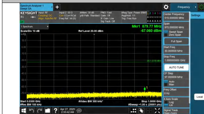
Band25-3MHz-QPSK-26675-1RB#0-30~1000-PASS
