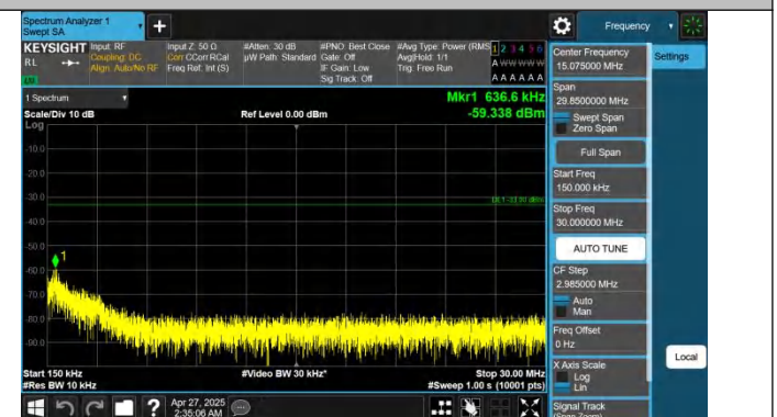
Band25-5MHz-QPSK-26065-1RB#0-0.15~30-PASS
