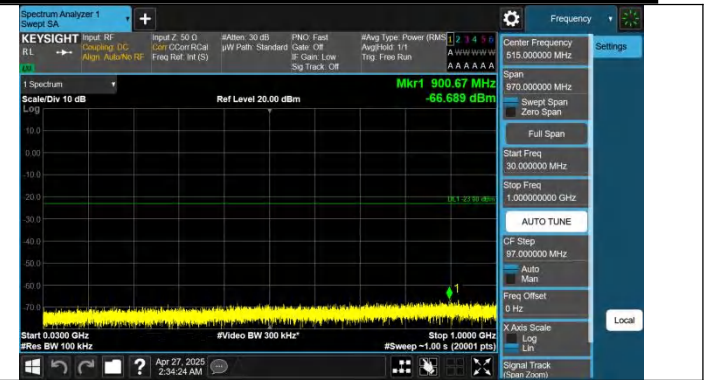
Band25-3MHz-QPSK-26675-1RB#14-30~1000-PASS
