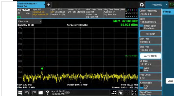
Band25-15MHz-QPSK-26115-1RB#0-0.009~0.15-PASS
