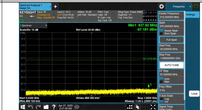
Band25-15MHz-QPSK-26615-1RB#74-30~1000-PASS
