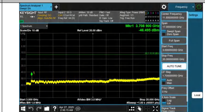
Band25-5MHz-QPSK-26065-1RB#24-3000~20000-PASS
