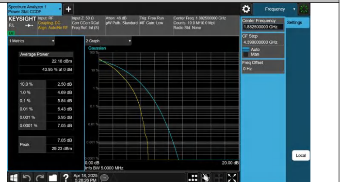
Band25-5MHz-64QAM-26365-25RB#0-PASS
