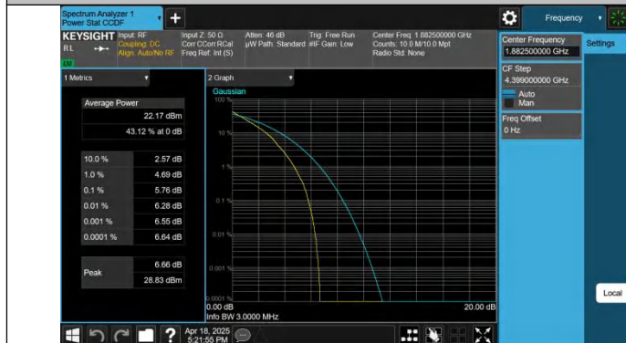
Band25-3MHz-16QAM-26365-15RB#0-PASS
