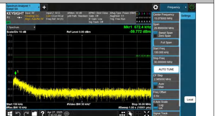
Band25-3MHz-QPSK-26055-1RB#0-0.15~30-PASS
