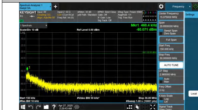
Band25-1.4MHz-QPSK-26683-1RB#5-0.15~30-PASS
