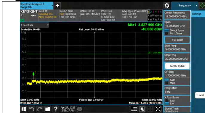
Band25-1.4MHz-QPSK-26683-1RB#0-3000~20000-PASS
