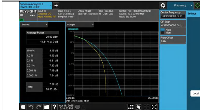
Band25-1.4MHz-16QAM-26365-6RB#0-PASS
