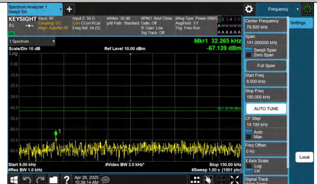
Band25-1.4MHz-QPSK-26365-1RB#5-0.009~0.15-PASS
