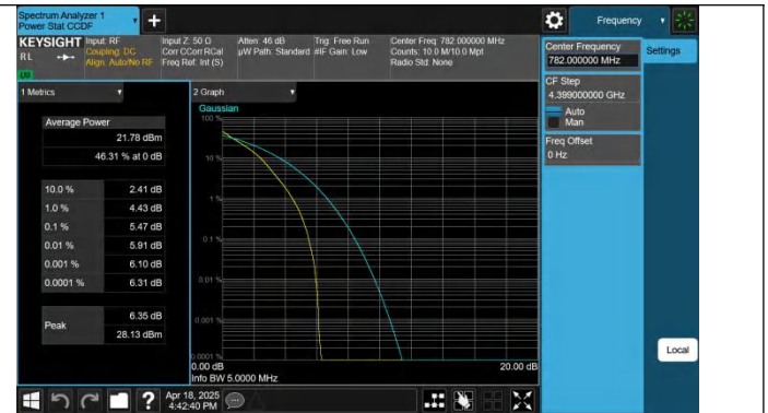
Band13-5MHz-64QAM-23230-25RB#0-PASS
