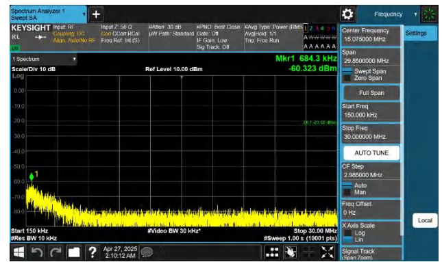
Band13-5MHz-QPSK-23205-1RB#24-0.15~30-PASS
