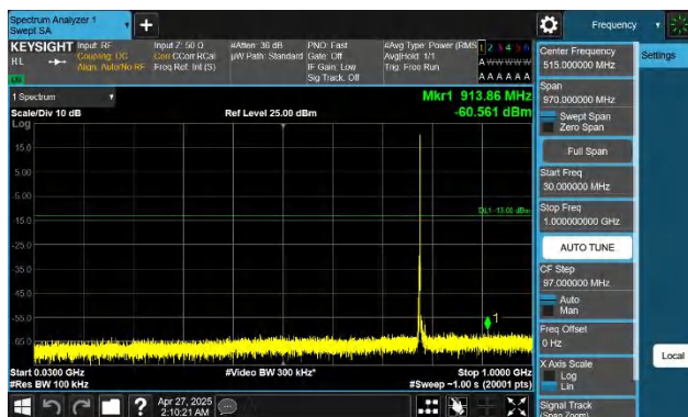
Band13-5MHz-QPSK-23205-1RB#24-30~1000-PASS
