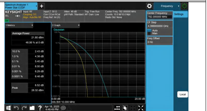
Band13-10MHz-QPSK-23230-50RB#0-PASS
