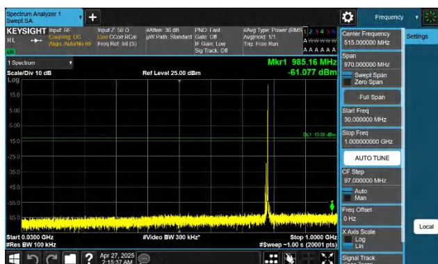
Band13-10MHz-QPSK-23230-1RB#49-30~1000-PASS
