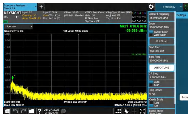
Band13-10MHz-QPSK-23230-1RB#49-0.15~30-PASS
