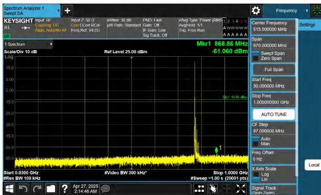
Band13-10MHz-QPSK-23230-1RB#0-30~1000-PASS
