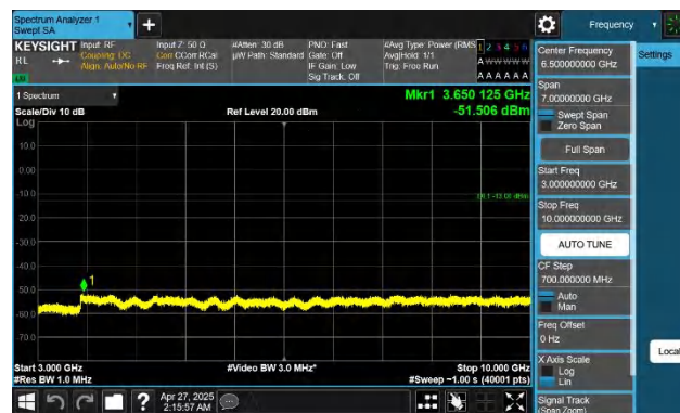
Band13-10MHz-QPSK-23230-1RB#49-3000~10000-PASS
