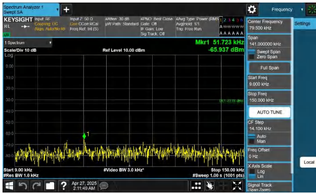
Band13-5MHz-QPSK-23230-1RB#24-0.009~0.15-PASS
