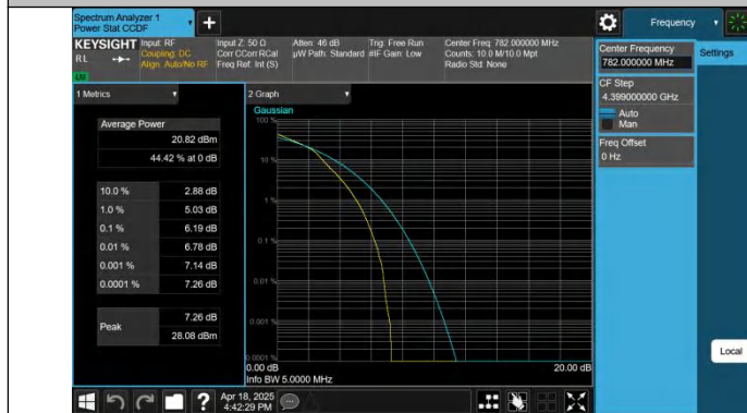
Band13-5MHz-16QAM-23230-25RB#0-PASS
