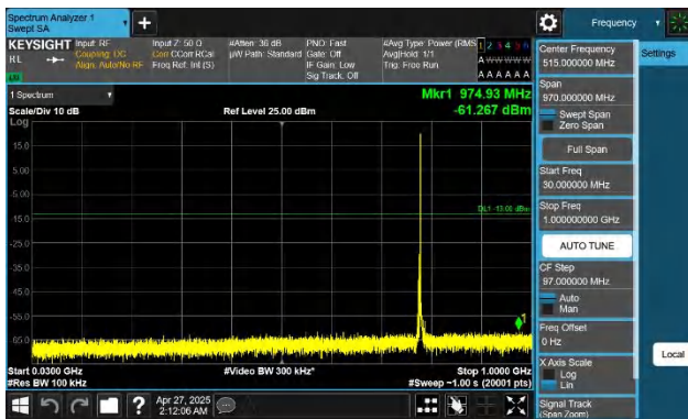
Band13-5MHz-QPSK-23230-1RB#24-30~1000-PASS
