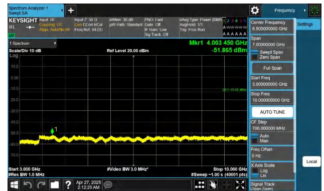
Band13-5MHz-QPSK-23230-1RB#24-3000~10000-PASS
