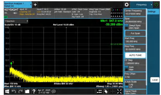
Band13-5MHz-QPSK-23230-1RB#24-0.15~30-PASS
