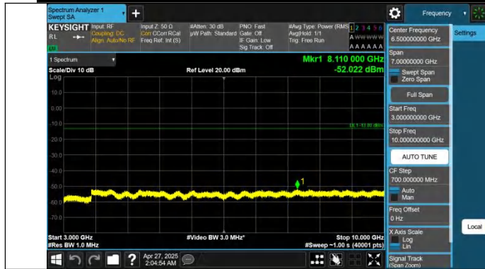
Band12-10MHz-QPSK-23095-1RB#0-3000~10000-PASS
