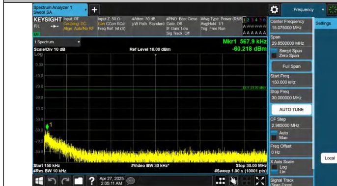
Band12-10MHz-QPSK-23095-1RB#49-0.15~30-PASS
