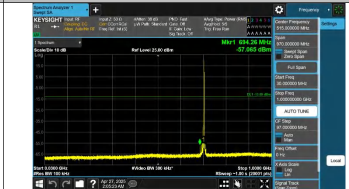
Band12-10MHz-QPSK-23095-1RB#49-30~1000-PASS
