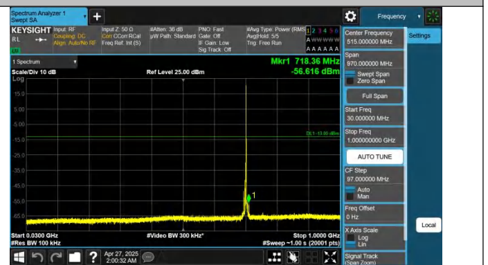
Band12-5MHz-QPSK-23095-1RB#24-30~1000-PASS
