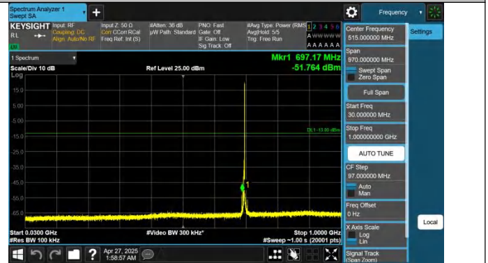
Band12-5MHz-QPSK-23035-1RB#24-30~1000-PASS
