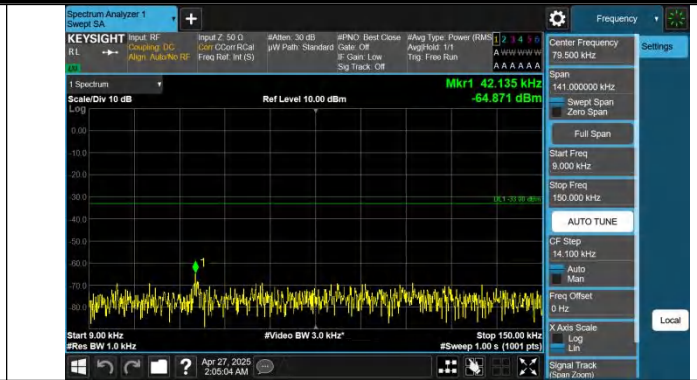
Band12-10MHz-QPSK-23095-1RB#49-0.009~0.15-PASS
