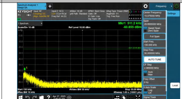
Band12-10MHz-QPSK-23130-1RB#0-0.15~30-PASS
