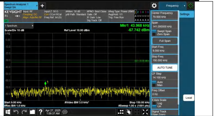
Band12-5MHz-QPSK-23035-1RB#24-0.009~0.15-PASS
