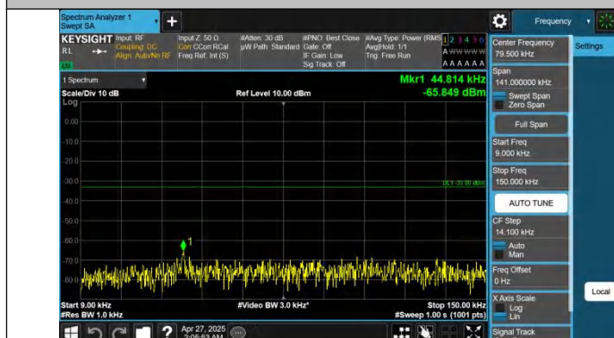
Band12-10MHz-QPSK-23130-1RB#0-0.009~0.15-PASS
