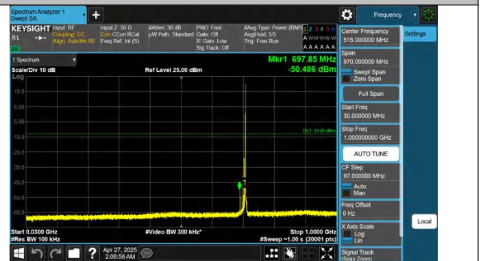
Band12-10MHz-QPSK-23130-1RB#49-30~1000-PASS
