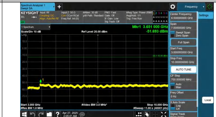
Band12-10MHz-QPSK-23095-1RB#49-3000~10000-PASS
