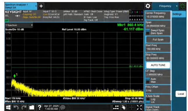
Band7-15MHz-QPSK-21375-1RB#0-0.15~30-PASS
