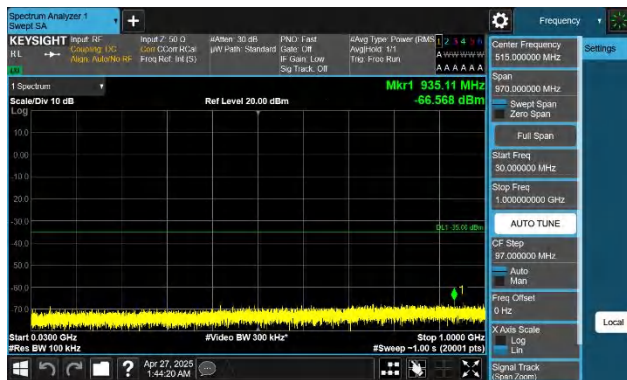
Band7-20MHz-QPSK-21100-1RB#0-30~1000-PASS
