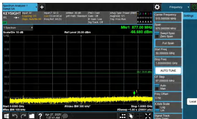
Band7-15MHz-QPSK-20825-1RB#0-30~1000-PASS
