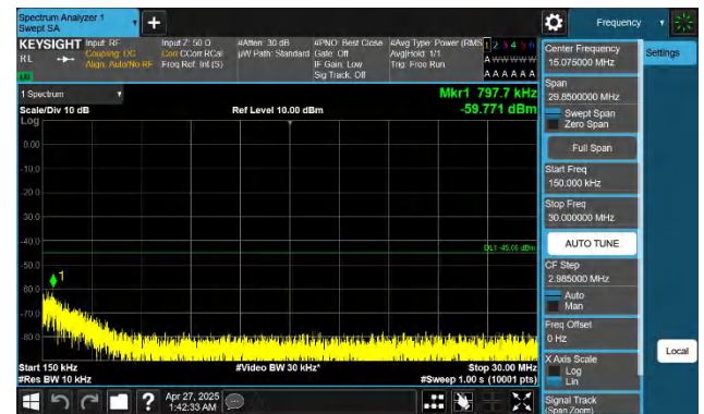
Band7-20MHz-QPSK-20850-1RB#0-0.15~30-PASS
