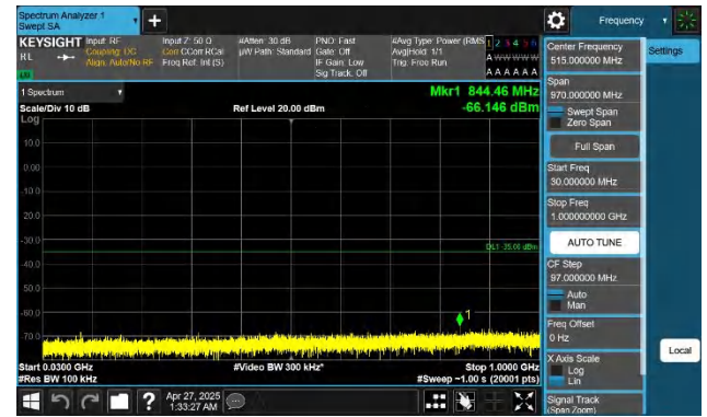
Band7-10MHz-QPSK-20800-1RB#49-30~1000-PASS
