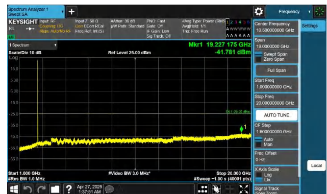
Band7-15MHz-QPSK-20825-1RB#0-1000~20000-PASS
