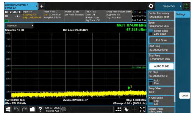
Band7-10MHz-QPSK-21100-1RB#49-30~1000-PASS
