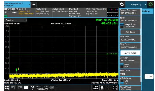
Band7-15MHz-QPSK-20825-1RB#74-30~1000-PASS
