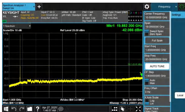
Band7-20MHz-QPSK-21350-1RB#99-1000~20000-PASS
