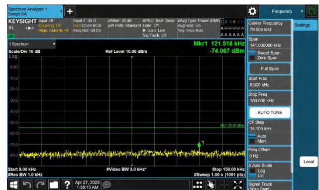
Band7-15MHz-QPSK-20825-1RB#74-0.009~0.15-PASS
