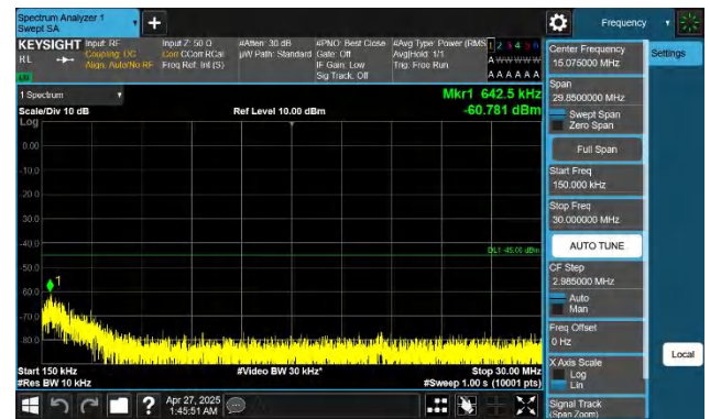
Band7-20MHz-QPSK-21350-1RB#0-0.15~30-PASS
