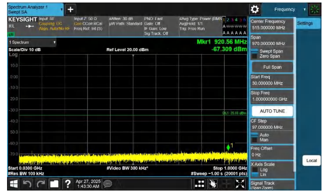
Band7-20MHz-QPSK-20850-1RB#99-30~1000-PASS
