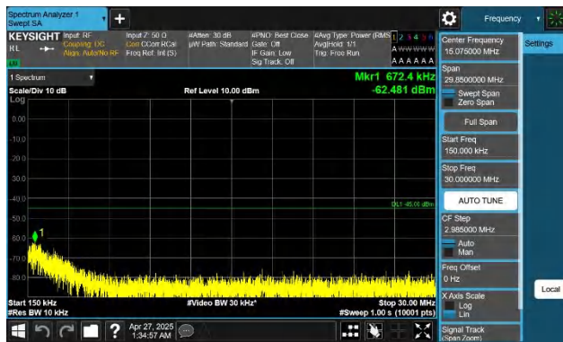
Band7-10MHz-QPSK-21100-1RB#49-0.15~30-PASS
