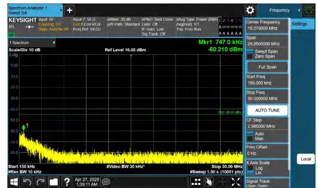
Band7-15MHz-QPSK-21100-1RB#0-0.15~30-PASS
