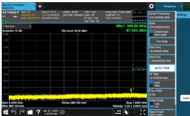
Band7-20MHz-QPSK-21350-1RB#0-30~1000-PASS
