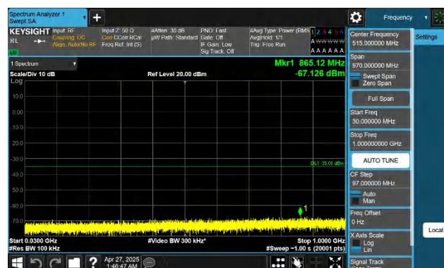
Band7-20MHz-QPSK-21350-1RB#99-30~1000-PASS
