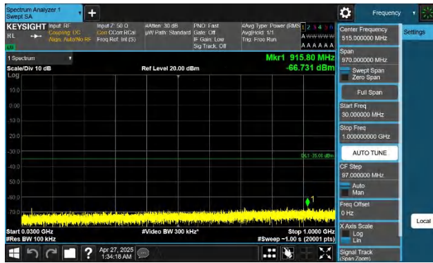
Band7-10MHz-QPSK-21100-1RB#0-30~1000-PASS
