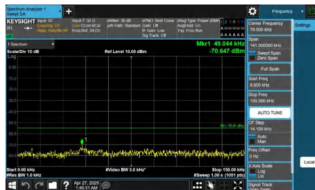
Band7-20MHz-QPSK-21350-1RB#99-0.009~0.15-PASS
