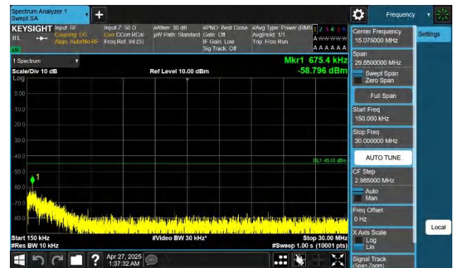
Band7-15MHz-QPSK-20825-1RB#0-0.15~30-PASS
