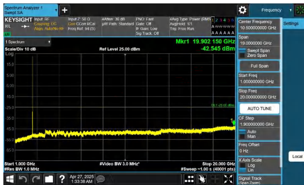
Band7-10MHz-QPSK-20800-1RB#49-1000~20000-PASS
