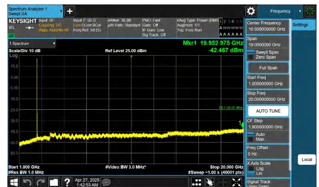
Band7-20MHz-QPSK-20850-1RB#0-1000~20000-PASS
