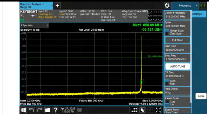
Band5-3MHz-QPSK-20635-1RB#14-30~1000-PASS
