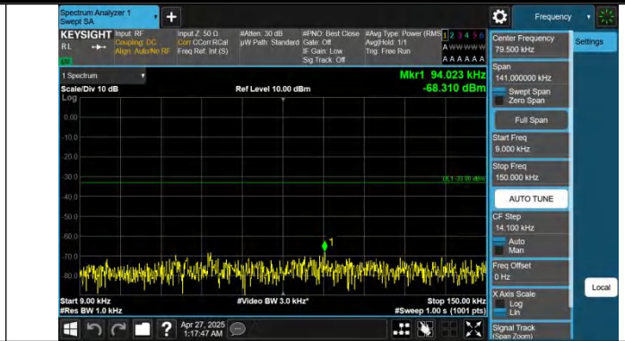
Band5-5MHz-QPSK-20425-1RB#24-0.009~0.15-PASS
