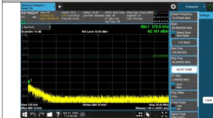
Band5-3MHz-QPSK-20415-1RB#14-0.15~30-PASS
