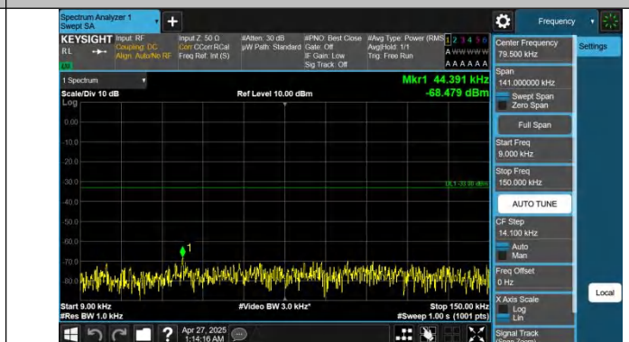
Band5-3MHz-QPSK-20525-1RB#14-0.009~0.15-PASS
