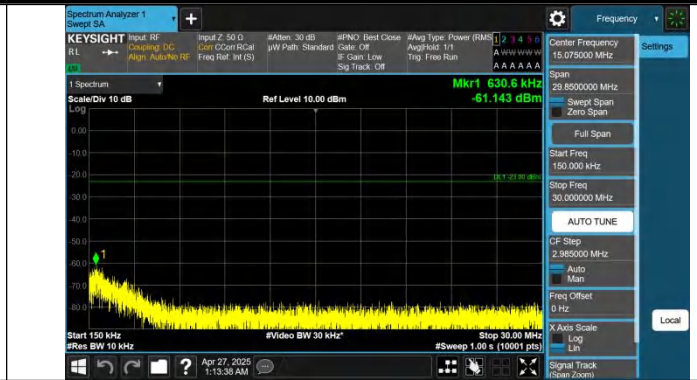
Band5-3MHz-QPSK-20525-1RB#0-0.15~30-PASS
