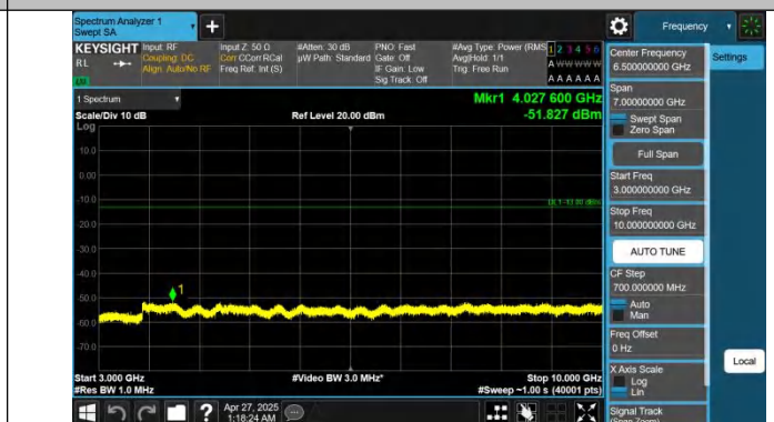
Band5-5MHz-QPSK-20425-1RB#24-3000~10000-PASS
