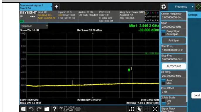
Band5-3MHz-QPSK-20635-1RB#14-1000~3000-PASS
