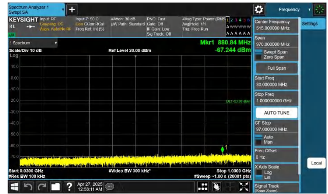
Band4-10MHz-QPSK-20000-1RB#49-30~1000-PASS
