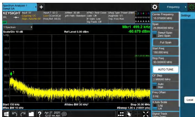
Band4-15MHz-QPSK-20025-1RB#74-0.15~30-PASS
