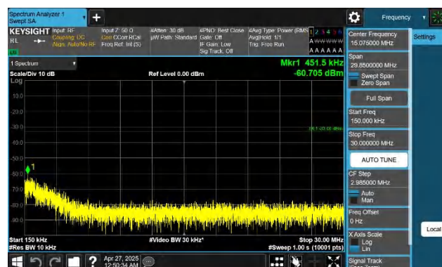
Band4-5MHz-QPSK-20375-1RB#0-0.15~30-PASS
