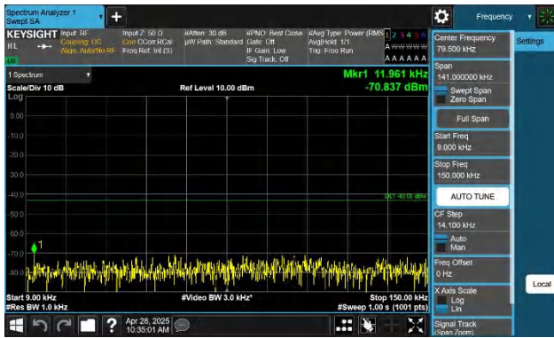
Band4-10MHz-QPSK-20000-1RB#0-0.009~0.15-PASS
