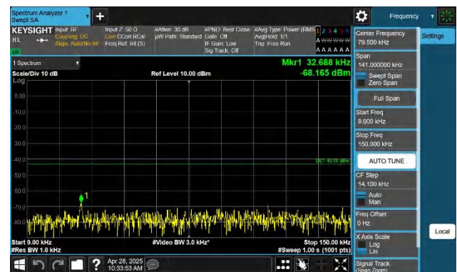
Band4-5MHz-QPSK-19975-1RB#24-0.009~0.15-PASS
