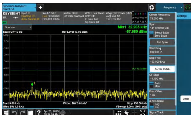
Band4-5MHz-QPSK-20375-1RB#0-0.009~0.15-PASS
