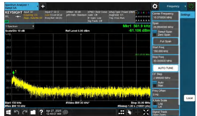
Band4-5MHz-QPSK-20175-1RB#0-0.15~30-PASS
