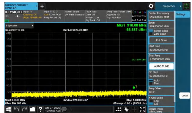
Band4-5MHz-QPSK-20175-1RB#24-30~1000-PASS
