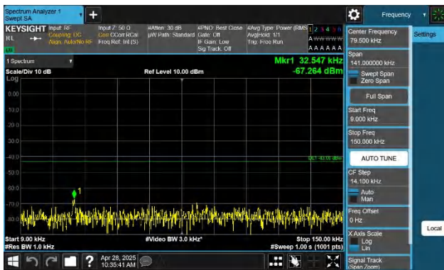
Band4-10MHz-QPSK-20350-1RB#0-0.009~0.15-PASS
