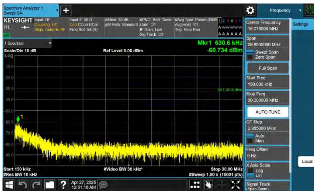
Band4-5MHz-QPSK-20375-1RB#24-0.15~30-PASS
