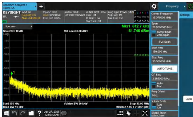
Band4-15MHz-QPSK-20175-1RB#74-0.15~30-PASS
