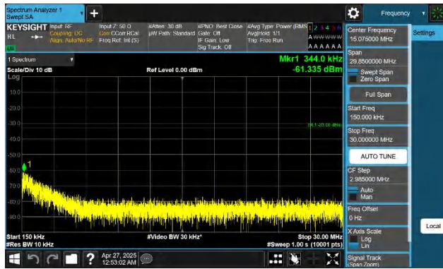
Band4-10MHz-QPSK-20000-1RB#49-0.15~30-PASS
