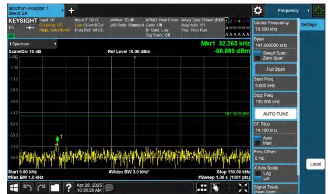
Band4-15MHz-QPSK-20025-1RB#74-0.009~0.15-PASS
