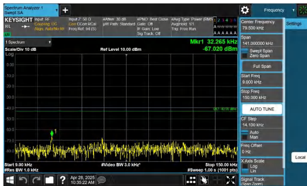
Band4-10MHz-QPSK-20175-1RB#0-0.009~0.15-PASS
