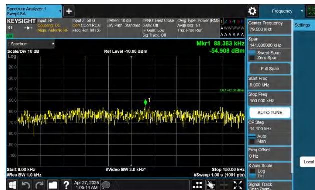
Band4-20MHz-QPSK-20300-1RB#99-0.009~0.15-PASS
