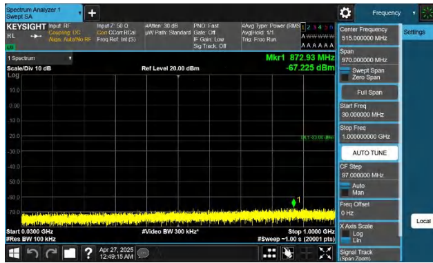
Band4-5MHz-QPSK-20175-1RB#0-30~1000-PASS
