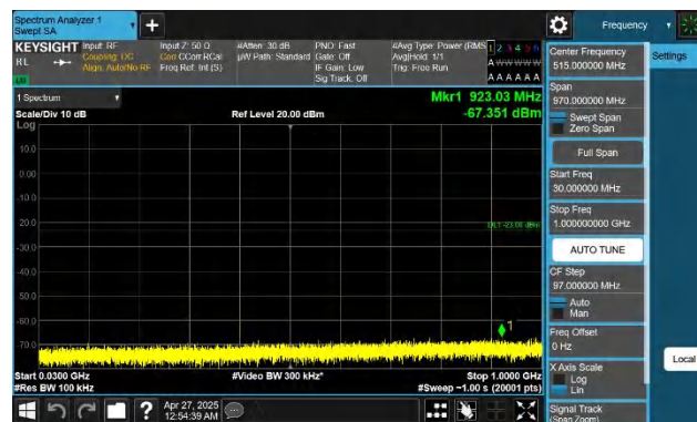
Band4-10MHz-QPSK-20175-1RB#49-30~1000-PASS
