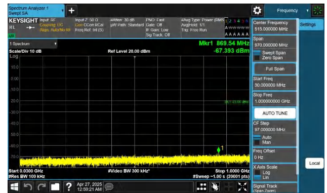
Band4-15MHz-QPSK-20175-1RB#74-30~1000-PASS
