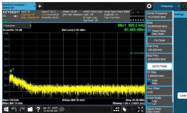
Band4-5MHz-QPSK-20175-1RB#24-0.15~30-PASS
