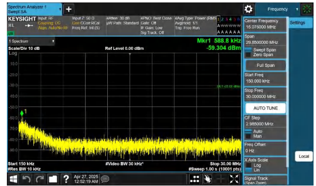
Band4-10MHz-QPSK-20000-1RB#0-0.15~30-PASS
