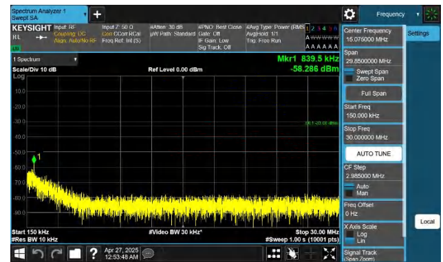
Band4-10MHz-QPSK-20175-1RB#0-0.15~30-PASS
