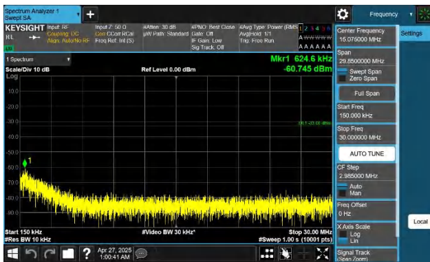
Band4-15MHz-QPSK-20325-1RB#74-0.15~30-PASS
