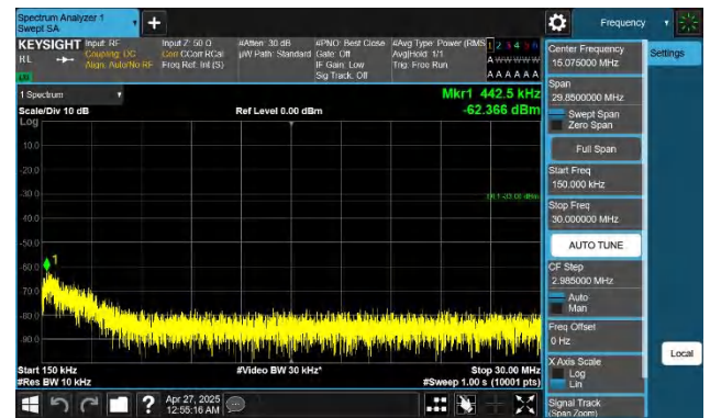
Band4-10MHz-QPSK-20350-1RB#0-0.15~30-PASS
