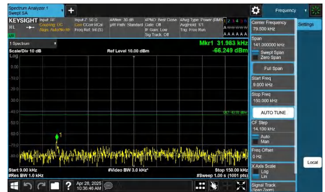
Band4-15MHz-QPSK-20175-1RB#74-0.009~0.15-PASS
