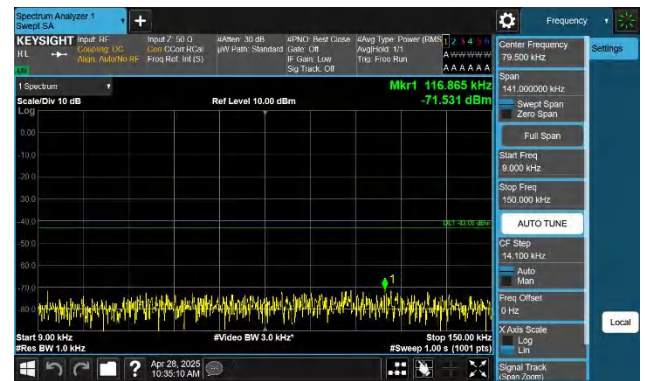
Band4-10MHz-QPSK-20000-1RB#49-0.009~0.15-PASS
