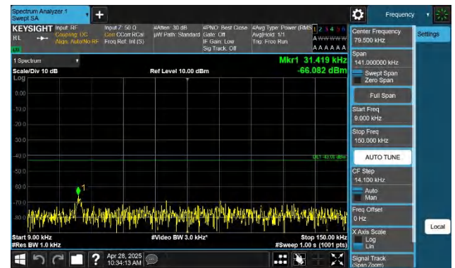
Band4-5MHz-QPSK-20175-1RB#24-0.009~0.15-PASS
