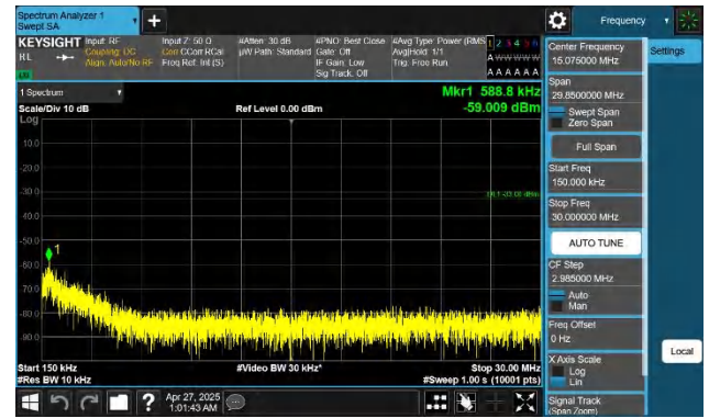
Band4-20MHz-QPSK-20050-1RB#0-0.15~30-PASS
