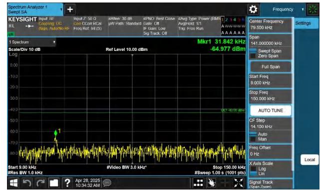
Band4-5MHz-QPSK-20375-1RB#24-0.009~0.15-PASS
