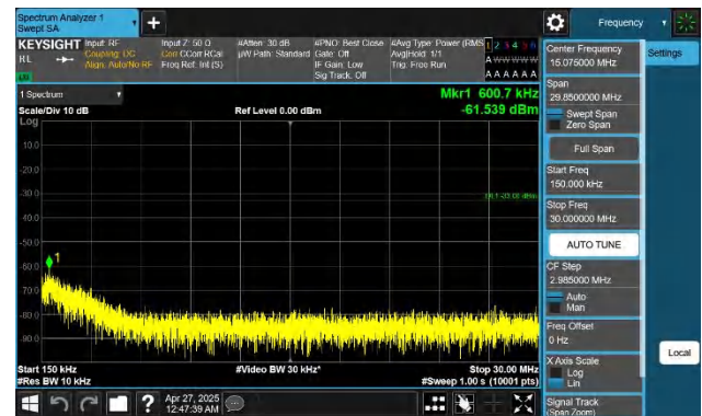
Band4-5MHz-QPSK-19975-1RB#0-0.15~30-PASS
