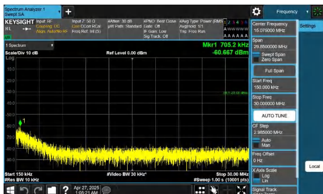
Band4-20MHz-QPSK-20300-1RB#99-0.15~30-PASS
