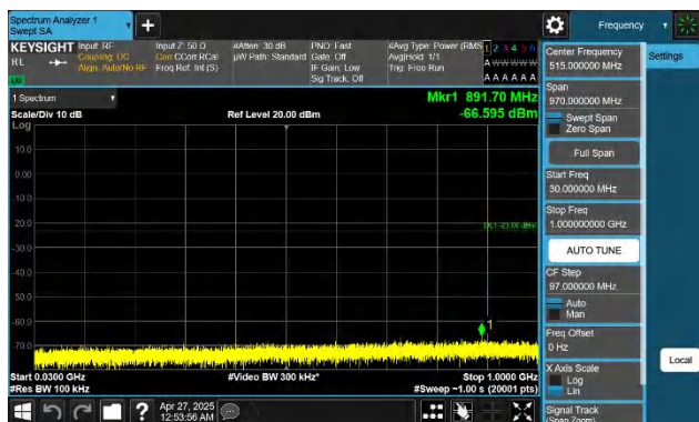
Band4-10MHz-QPSK-20175-1RB#0-30~1000-PASS
