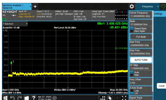
Band4-10MHz-QPSK-20175-1RB#0-3000~20000-PASS
