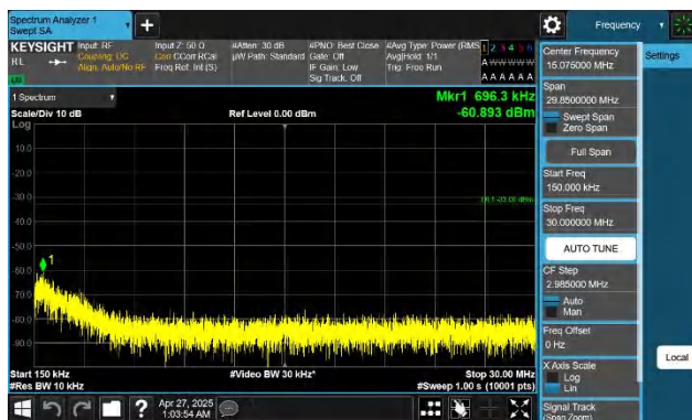
Band4-20MHz-QPSK-20175-1RB#99-0.15~30-PASS
