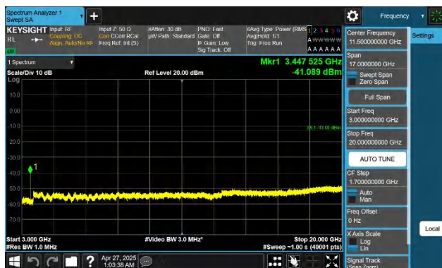
Band4-20MHz-QPSK-20175-1RB#0-3000~20000-PASS
