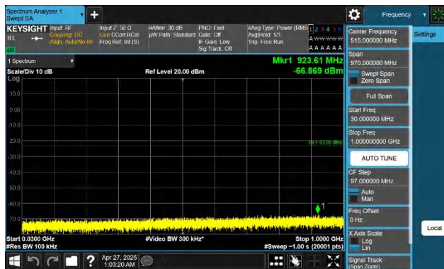
Band4-20MHz-QPSK-20175-1RB#0-30~1000-PASS
