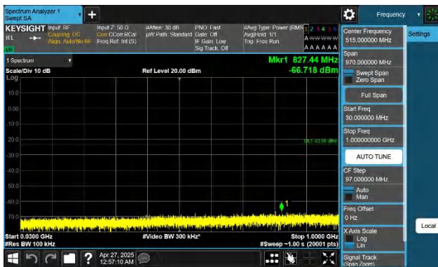
Band4-15MHz-QPSK-20025-1RB#0-30~1000-PASS
