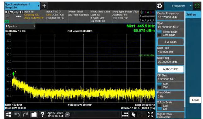
Band4-15MHz-QPSK-20025-1RB#0-0.15~30-PASS
