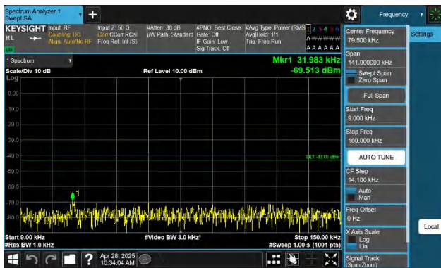
Band4-5MHz-QPSK-20175-1RB#0-0.009~0.15-PASS
