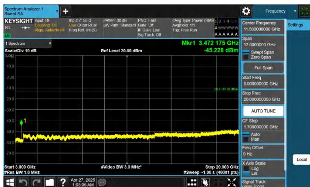
Band4-20MHz-QPSK-20300-1RB#0-3000~20000-PASS
