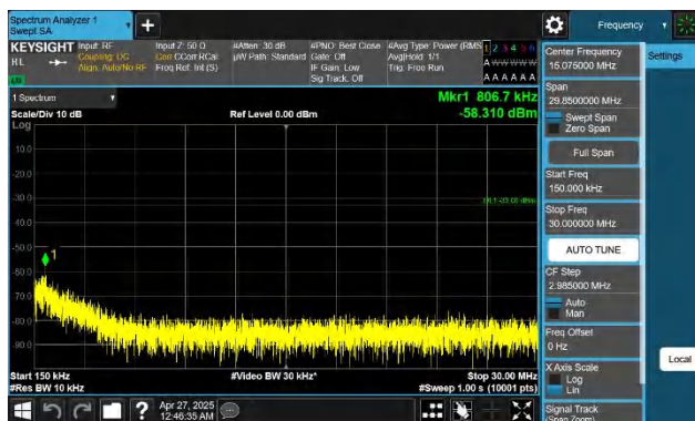
Band4-3MHz-QPSK-20385-1RB#14-0.15~30-PASS
