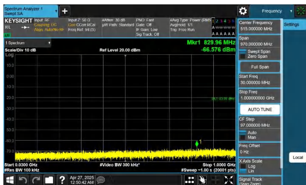
Band4-5MHz-QPSK-20375-1RB#0-30~1000-PASS
