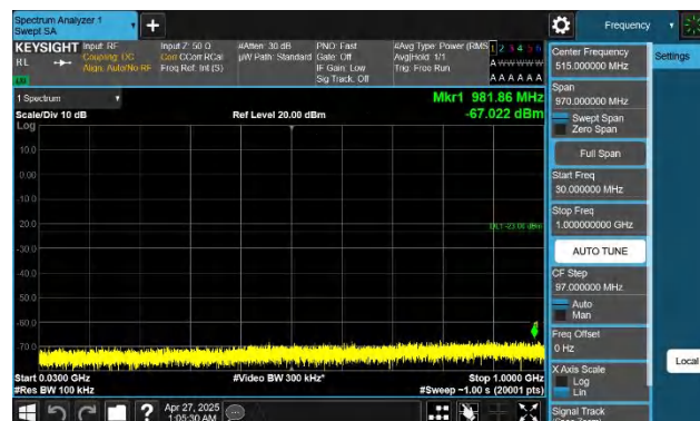
Band4-20MHz-QPSK-20300-1RB#99-30~1000-PASS
