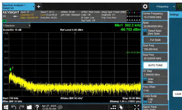
Band4-10MHz-QPSK-20350-1RB#49-0.15~30-PASS
