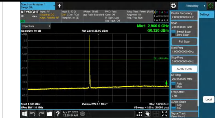
Band2-5MHz-QPSK-18900-1RB#0-1000~3000-PASS
