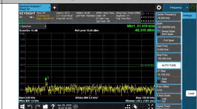
Band2-3MHz-QPSK-18615-1RB#14-0.009~0.15-PASS
