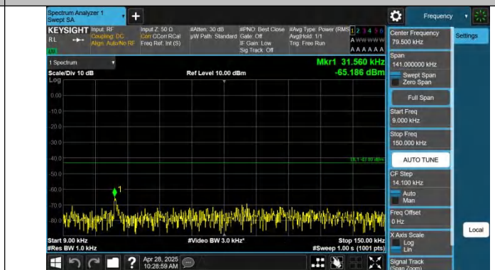
Band2-20MHz-QPSK-18700-1RB#99-0.009~0.15-PASS
