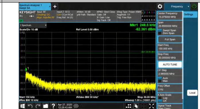
Band2-15MHz-QPSK-18900-1RB#0-0.15~30-PASS
