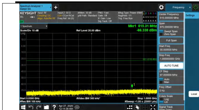
Band2-3MHz-QPSK-18615-1RB#0-30~1000-PASS
