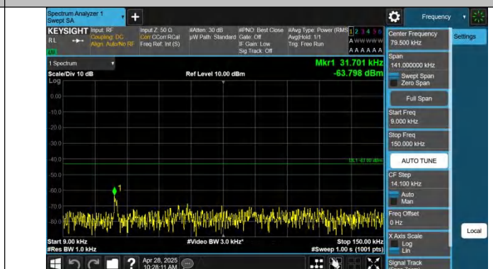
Band2-15MHz-QPSK-18900-1RB#74-0.009~0.15-PASS
