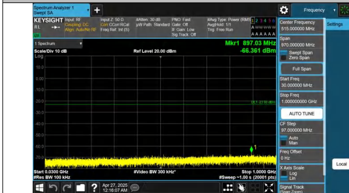
Band2-3MHz-QPSK-18900-1RB#0-30~1000-PASS
