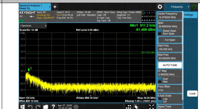
Band2-5MHz-QPSK-18900-1RB#0-0.15~30-PASS
