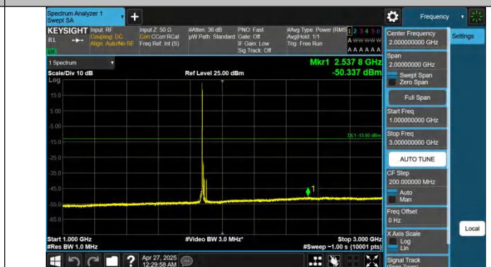
Band2-15MHz-QPSK-18900-1RB#0-1000~3000-PASS
