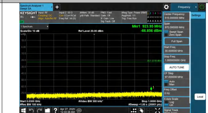
Band2-20MHz-QPSK-18700-1RB#99-30~1000-PASS
