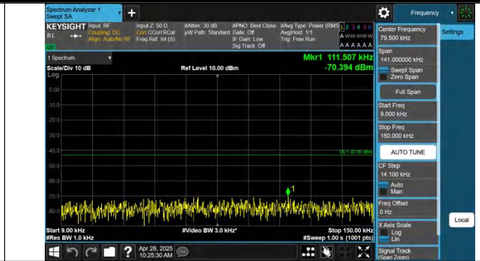
Band2-5MHz-QPSK-18625-1RB#24-0.009~0.15-PASS
