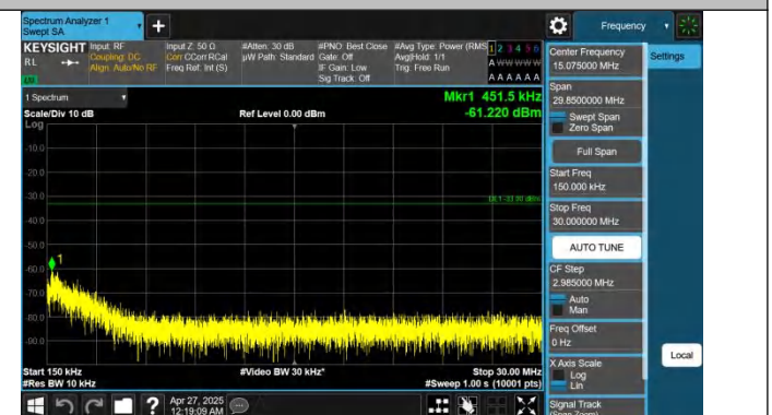
Band2-5MHz-QPSK-18625-1RB#0-0.15~30-PASS
