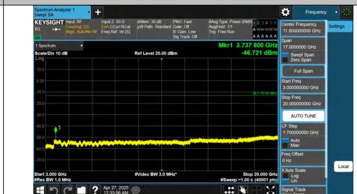
Band2-20MHz-QPSK-18700-1RB#99-3000~20000-PASS
