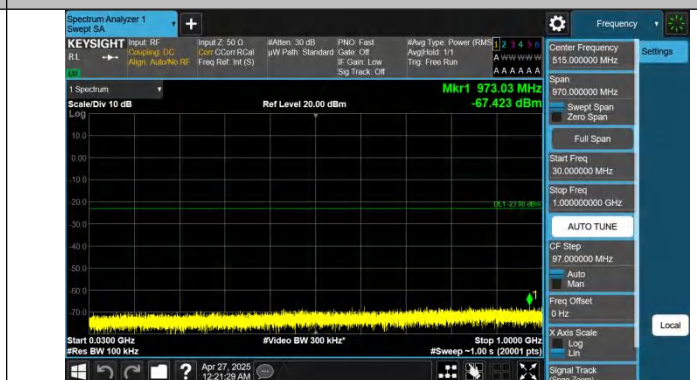
Band2-5MHz-QPSK-18900-1RB#24-30~1000-PASS
