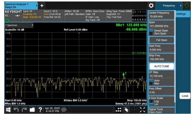
Band71-15MHz-QPSK-133397-1RB#74-0.009~0.15-PASS
