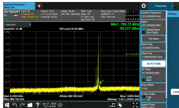
Band71-20MHz-QPSK-133322-1RB#99-30~1000-PASS
