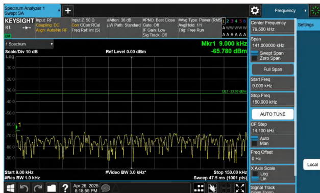
Band71-15MHz-QPSK-133397-1RB#0-0.009~0.15-PASS
