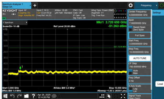
Band71-10MHz-QPSK-133422-1RB#0-3000~10000-PASS
