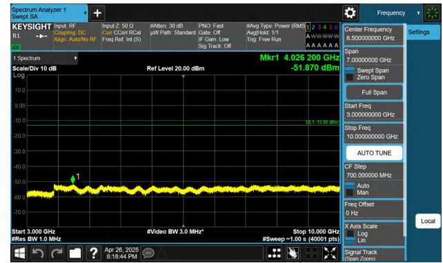
Band71-15MHz-QPSK-133297-1RB#74-3000~10000-PASS
