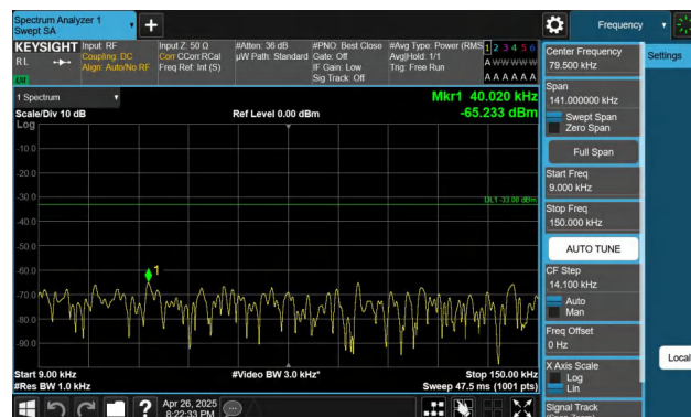
Band71-20MHz-QPSK-133322-1RB#99-0.009~0.15-PASS
