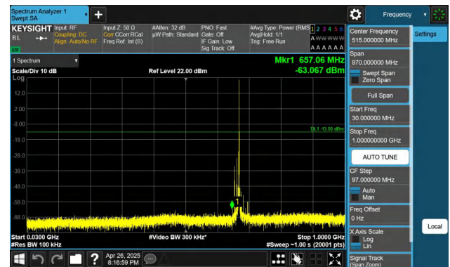
Band71-15MHz-QPSK-133197-1RB#74-30~1000-PASS
