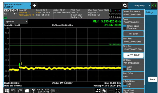
Band71-15MHz-QPSK-133197-1RB#74-3000~10000-PASS
