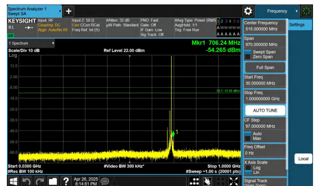
Band71-10MHz-QPSK-133422-1RB#49-30~1000-PASS
