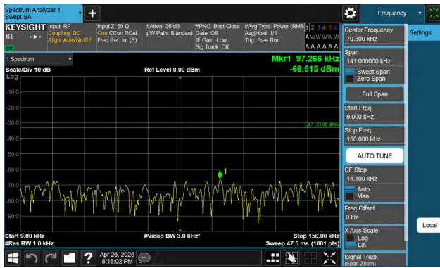
Band71-15MHz-QPSK-133197-1RB#0-0.009~0.15-PASS
