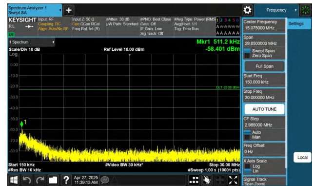
Band71-20MHz-QPSK-133322-1RB#0-0.15~30-PASS
