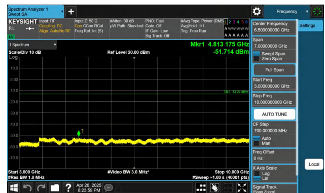
Band71-20MHz-QPSK-133372-1RB#99-3000~10000-PASS
