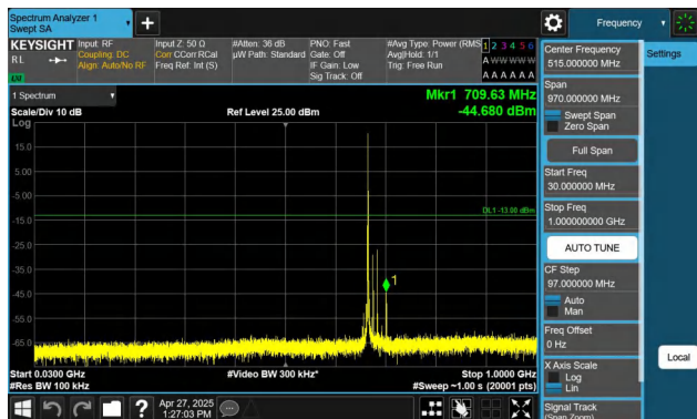
Band71-20MHz-QPSK-133322-1RB#0-30~1000-PASS
