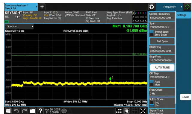
Band71-10MHz-QPSK-133422-1RB#49-3000~10000-PASS
