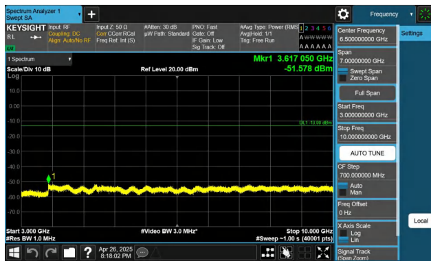
Band71-15MHz-QPSK-133297-1RB#0-3000~10000-PASS
