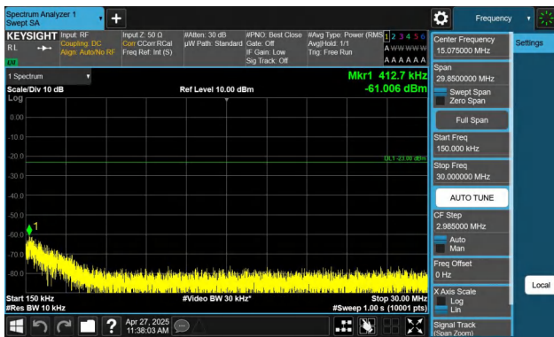
Band71-15MHz-QPSK-133397-1RB#74-0.15~30-PASS
