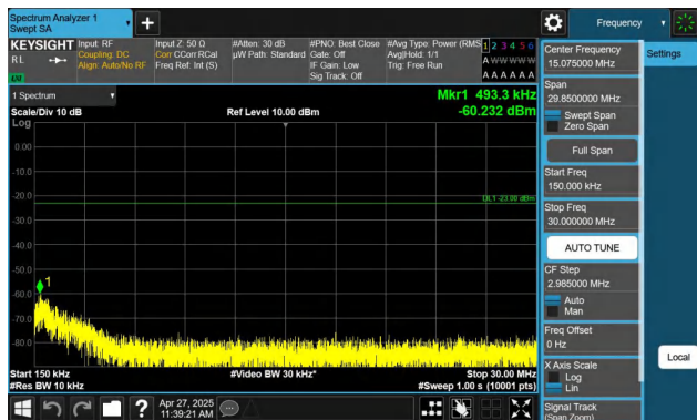
Band71-20MHz-QPSK-133322-1RB#99-0.15~30-PASS
