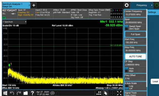
Band71-15MHz-QPSK-133197-1RB#74-0.15~30-PASS
