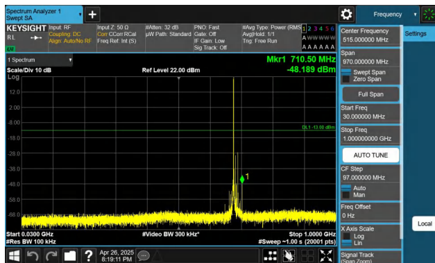
Band71-15MHz-QPSK-133397-1RB#0-30~1000-PASS
