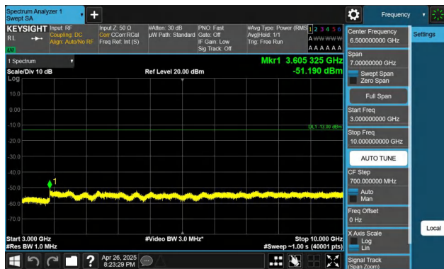
Band71-20MHz-QPSK-133372-1RB#0-3000~10000-PASS
