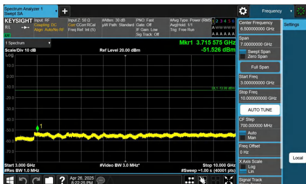
Band71-20MHz-QPSK-133322-1RB#0-3000~10000-PASS
