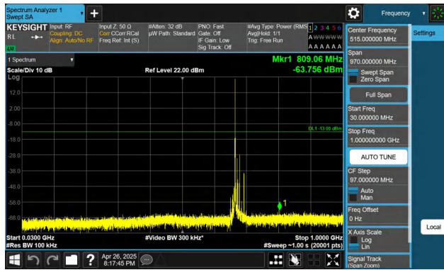
Band71-15MHz-QPSK-133297-1RB#0-30~1000-PASS
