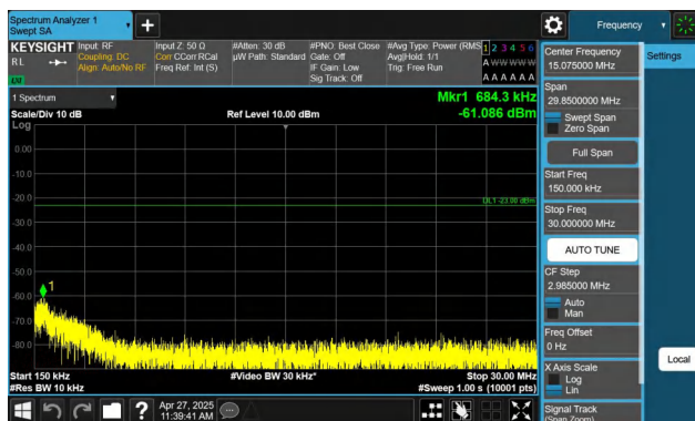
Band71-20MHz-QPSK-133372-1RB#99-0.15~30-PASS
