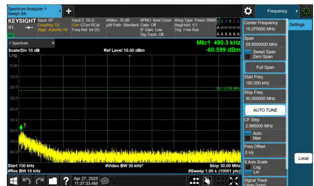
Band71-15MHz-QPSK-133297-1RB#0-0.15~30-PASS
