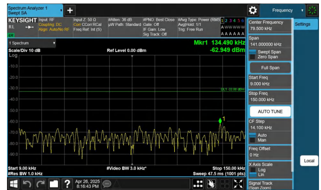
Band71-15MHz-QPSK-133197-1RB#74-0.009~0.15-PASS
