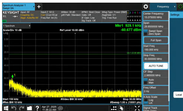
Band71-10MHz-QPSK-133422-1RB#49-0.15~30-PASS
