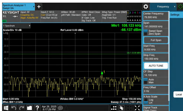
Band71-15MHz-QPSK-133297-1RB#0-0.009~0.15-PASS
