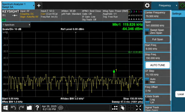
Band71-20MHz-QPSK-133222-1RB#0-0.009~0.15-PASS
