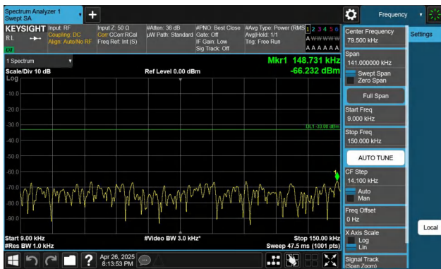
Band71-10MHz-QPSK-133422-1RB#0-0.009~0.15-PASS
