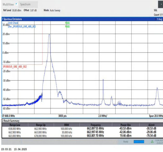
Band71-15MHz-QPSK-133197-1RB#0-PASS
