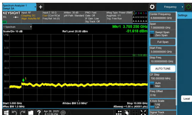
Band71-10MHz-QPSK-133297-1RB#0-3000~10000-PASS
