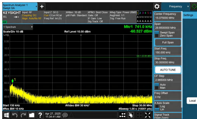
Band71-5MHz-QPSK-133447-1RB#24-0.15~30-PASS
