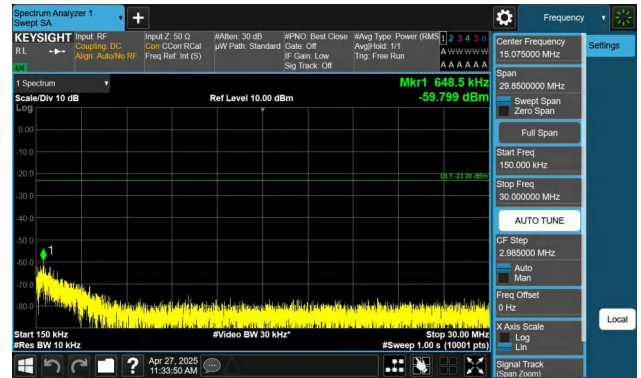
Band71-5MHz-QPSK-133147-1RB#0-0.15~30-PASS
