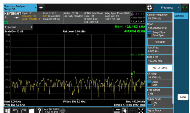
Band71-5MHz-QPSK-133147-1RB#24-0.009~0.15-PASS
