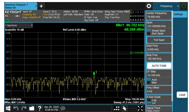
Band71-5MHz-QPSK-133297-1RB#24-0.009~0.15-PASS
