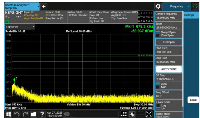
Band71-5MHz-QPSK-133297-1RB#0-0.15~30-PASS
