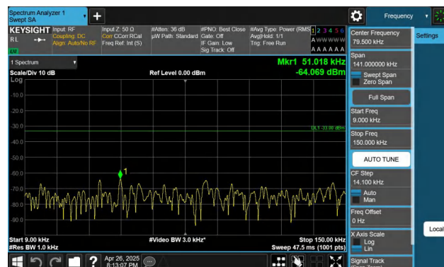
Band71-10MHz-QPSK-133297-1RB#49-0.009~0.15-PASS
