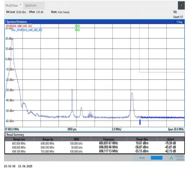
Band71-15MHz-QPSK-133397-1RB#0-PASS
