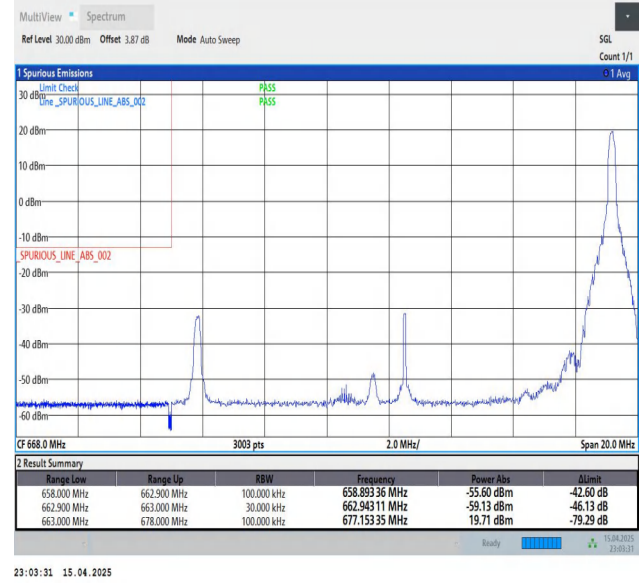
Band71-15MHz-QPSK-133197-1RB#74-PASS
