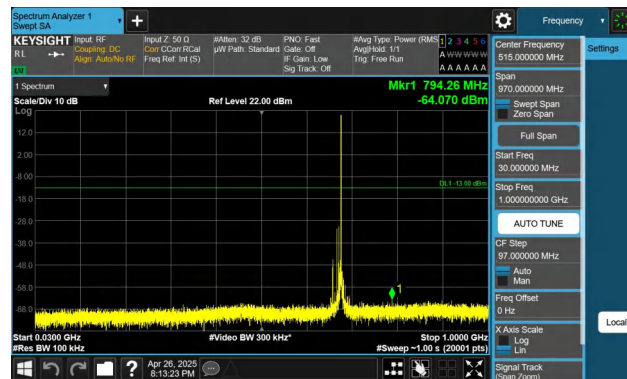
Band71-10MHz-QPSK-133297-1RB#49-30~1000-PASS
