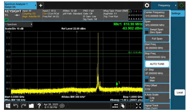
Band71-10MHz-QPSK-133172-1RB#49-30~1000-PASS
