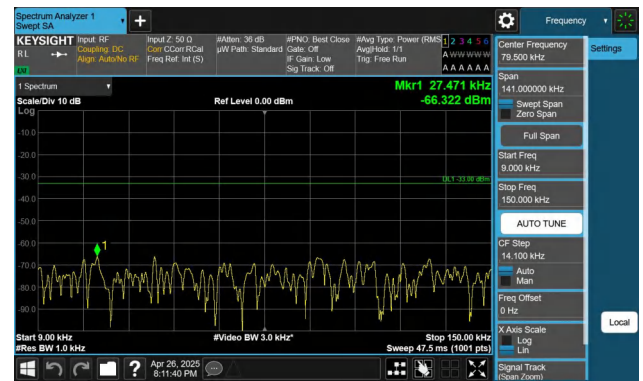
Band71-10MHz-QPSK-133172-1RB#49-0.009~0.15-PASS
