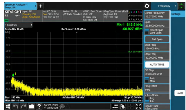
Band71-10MHz-QPSK-133297-1RB#0-0.15~30-PASS
