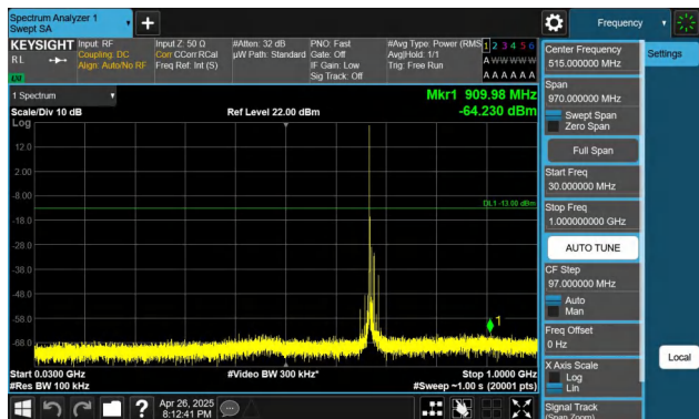
Band71-10MHz-QPSK-133297-1RB#0-30~1000-PASS
