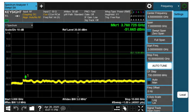
Band71-5MHz-QPSK-133147-1RB#24-3000~10000-PASS
