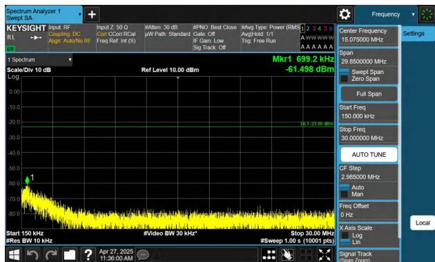
Band71-10MHz-QPSK-133297-1RB#49-0.15~30-PASS
