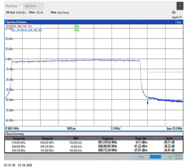
Band71-20MHz-QPSK-133372-100RB#0-PASS
