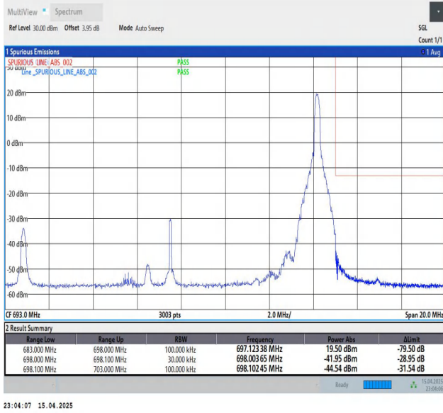
Band71-15MHz-QPSK-133397-1RB#74-PASS
