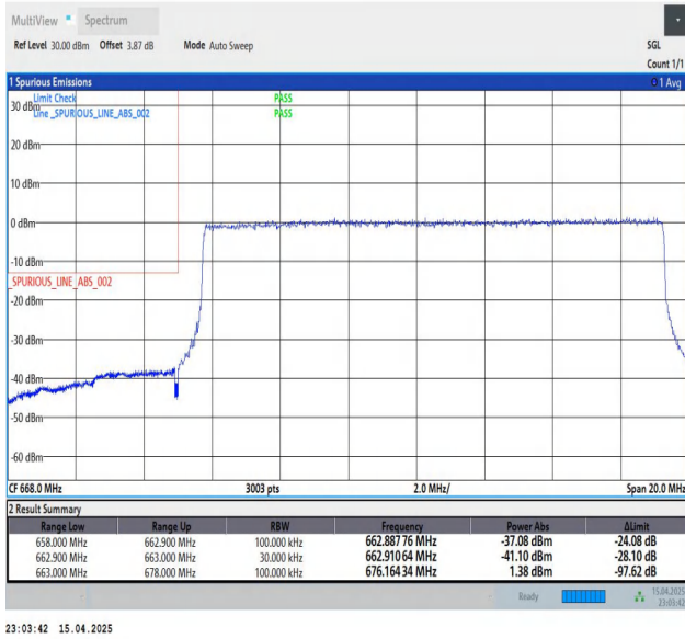
Band71-15MHz-QPSK-133197-75RB#0-PASS
