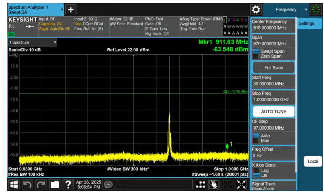
Band71-5MHz-QPSK-133147-1RB#24-30~1000-PASS
