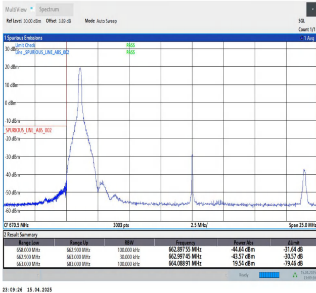
Band71-20MHz-QPSK-133222-1RB#0-PASS
