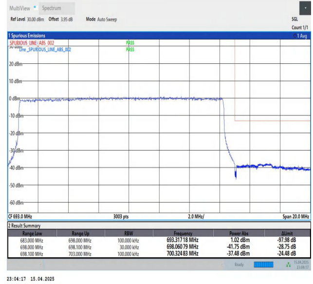
Band71-15MHz-QPSK-133397-75RB#0-PASS
