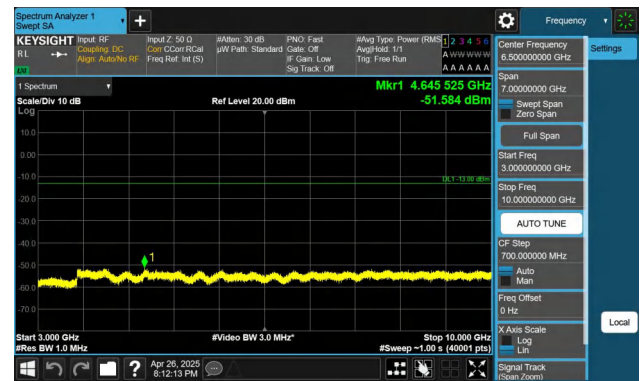
Band71-10MHz-QPSK-133172-1RB#49-3000~10000-PASS
