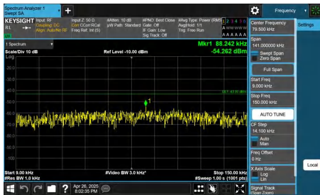
Band66-20MHz-QPSK-132322-1RB#0-0.009~0.15-PASS
