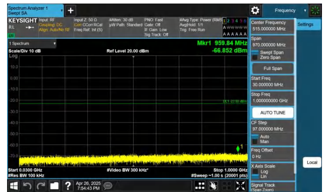
Band66-10MHz-QPSK-132322-1RB#49-30~1000-PASS
