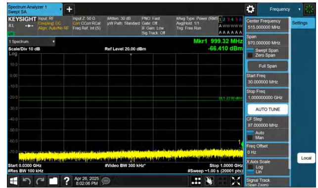
Band66-20MHz-QPSK-132072-1RB#99-30~1000-PASS
