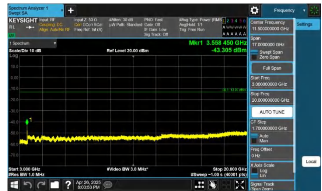
Band66-15MHz-QPSK-132597-1RB#74-3000~20000-PASS
