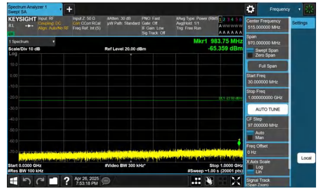
Band66-10MHz-QPSK-132022-1RB#49-30~1000-PASS
