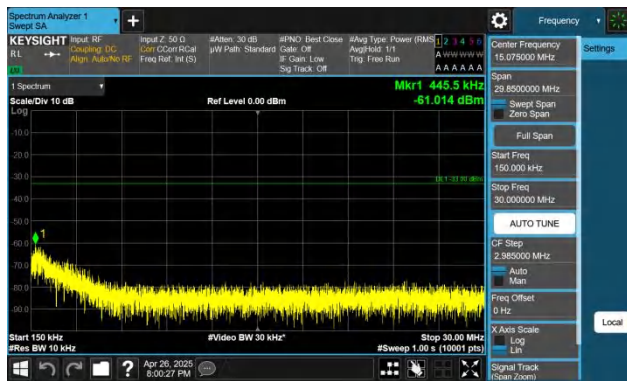
Band66-15MHz-QPSK-132597-1RB#74-0.15~30-PASS
