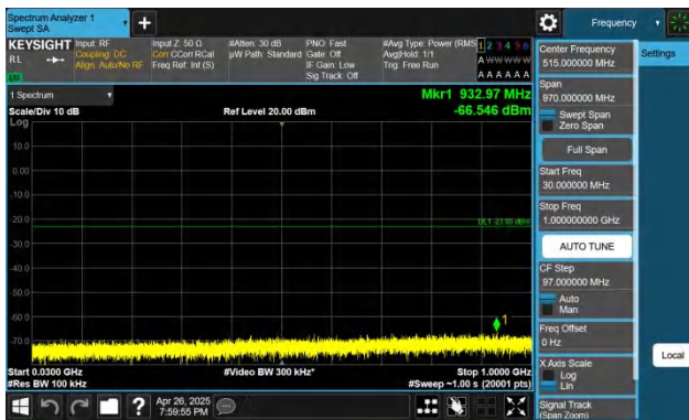
Band66-15MHz-QPSK-132597-1RB#0-30~1000-PASS
