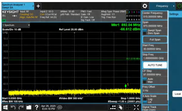
Band66-20MHz-QPSK-132572-1RB#0-30~1000-PASS
