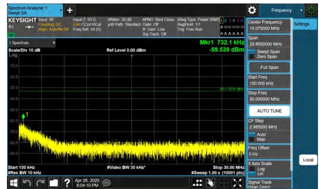
Band66-20MHz-QPSK-132572-1RB#0-0.15~30-PASS
