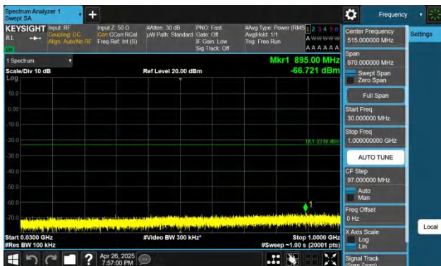
Band66-15MHz-QPSK-132047-1RB#0-30~1000-PASS
