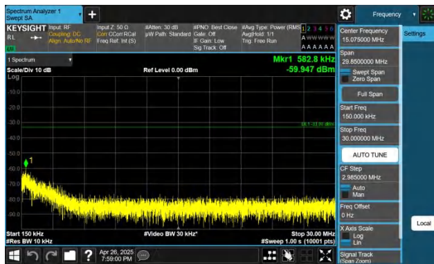
Band66-15MHz-QPSK-132322-1RB#74-0.15~30-PASS
