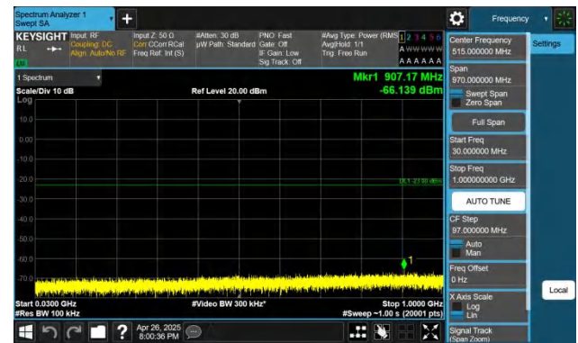
Band66-15MHz-QPSK-132597-1RB#74-30~1000-PASS
