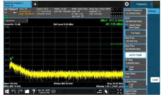
Band66-15MHz-QPSK-132047-1RB#0-0.15~30-PASS
