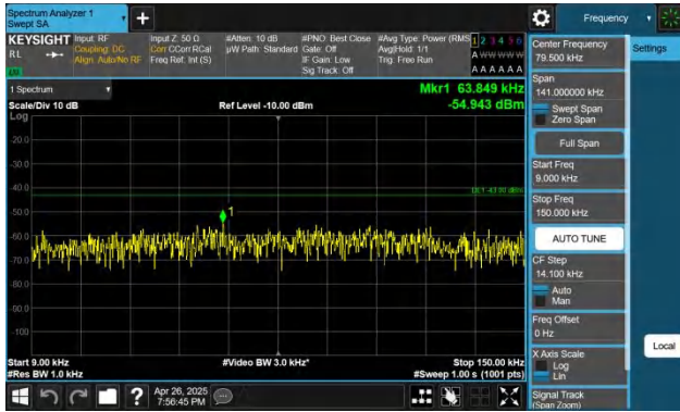
Band66-15MHz-QPSK-132047-1RB#0-0.009~0.15-PASS
