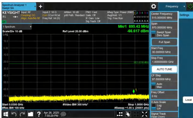
Band66-10MHz-QPSK-132622-1RB#0-30~1000-PASS
