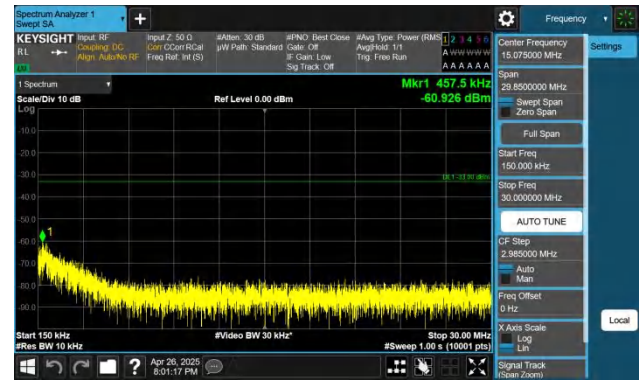
Band66-20MHz-QPSK-132072-1RB#0-0.15~30-PASS
