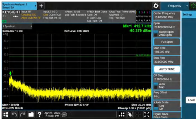
Band66-10MHz-QPSK-132022-1RB#49-0.15~30-PASS
