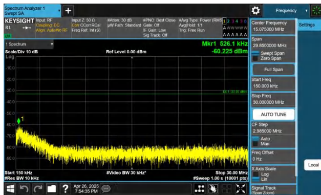
Band66-10MHz-QPSK-132322-1RB#49-0.15~30-PASS
