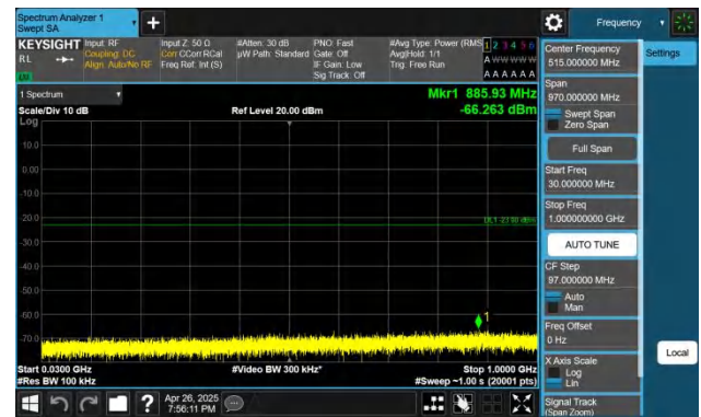
Band66-10MHz-QPSK-132622-1RB#49-30~1000-PASS
