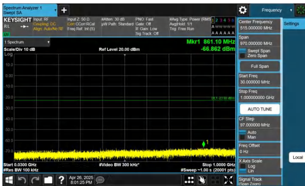
Band66-20MHz-QPSK-132072-1RB#0-30~1000-PASS
