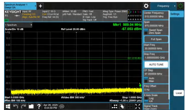
Band66-20MHz-QPSK-132572-1RB#99-30~1000-PASS
