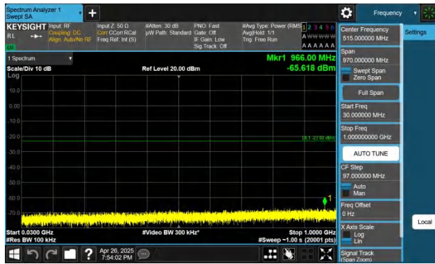
Band66-10MHz-QPSK-132322-1RB#0-30~1000-PASS
