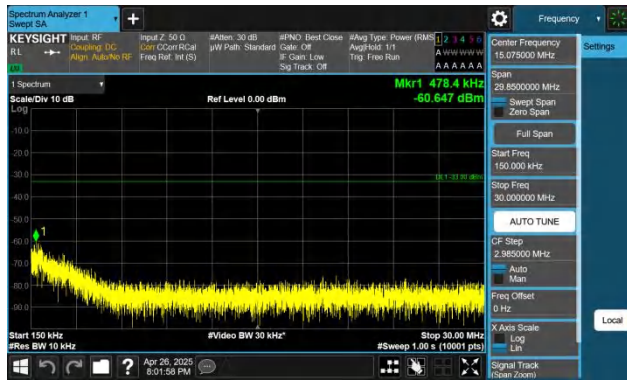
Band66-20MHz-QPSK-132072-1RB#99-0.15~30-PASS
