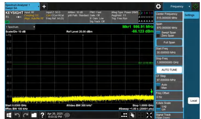
Band66-20MHz-QPSK-132322-1RB#99-30~1000-PASS
