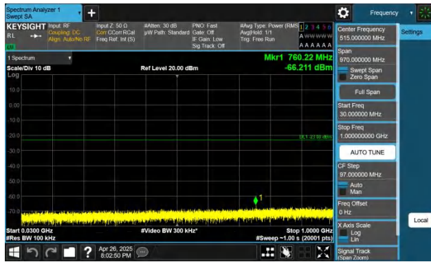
Band66-20MHz-QPSK-132322-1RB#0-30~1000-PASS
