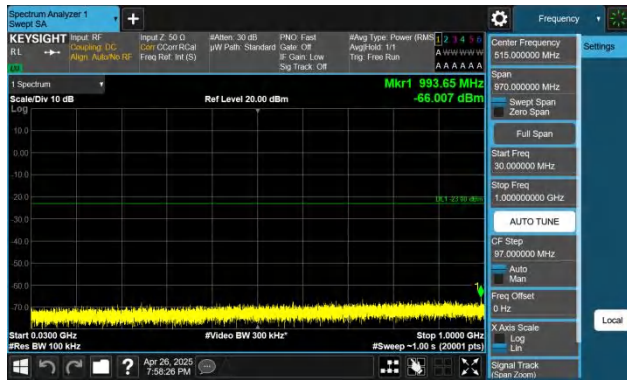
Band66-15MHz-QPSK-132322-1RB#0-30~1000-PASS
