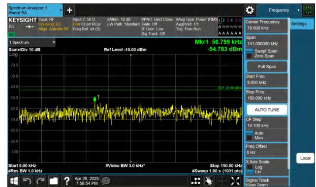
Band66-15MHz-QPSK-132322-1RB#74-0.009~0.15-PASS
