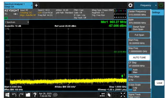
Band66-15MHz-QPSK-132322-1RB#74-30~1000-PASS
