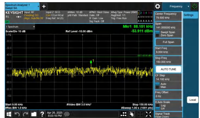
Band66-20MHz-QPSK-132322-1RB#99-0.009~0.15-PASS
