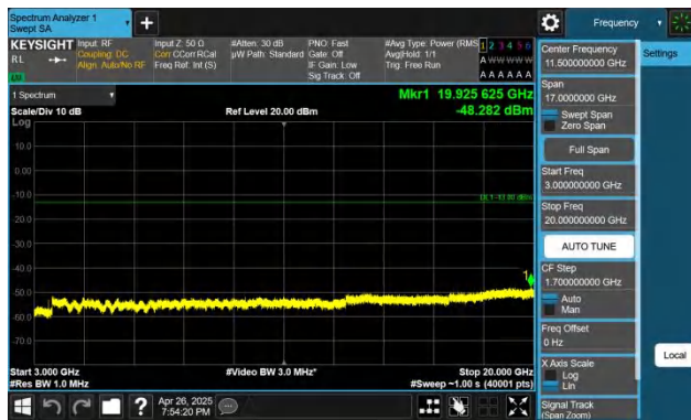
Band66-10MHz-QPSK-132322-1RB#0-3000~20000-PASS
