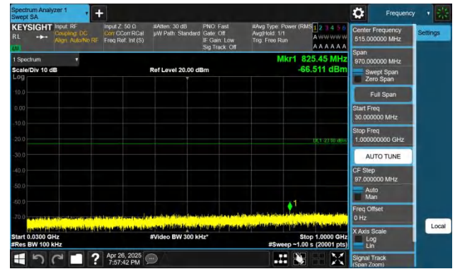
Band66-15MHz-QPSK-132047-1RB#74-30~1000-PASS
