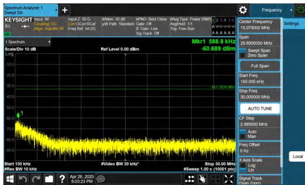
Band66-20MHz-QPSK-132322-1RB#99-0.15~30-PASS
