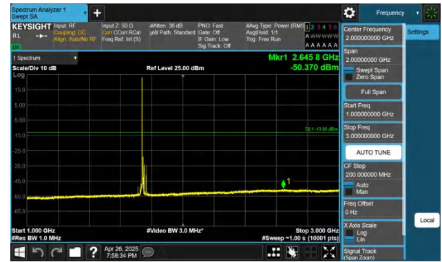
Band66-15MHz-QPSK-132322-1RB#0-1000~3000-PASS
