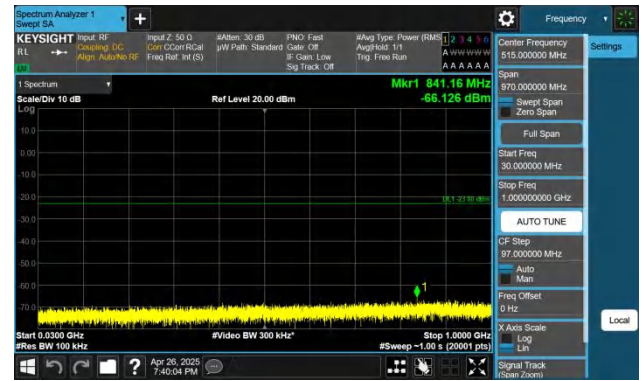
Band66-1.4MHz-QPSK-131979-1RB#5-30~1000-PASS
