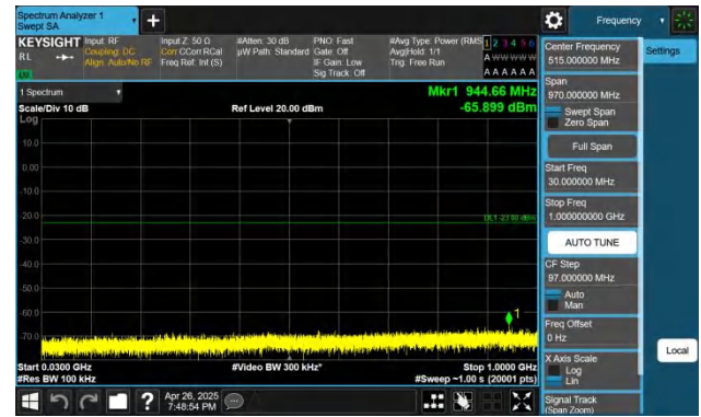
Band66-5MHz-QPSK-131997-1RB#24-30~1000-PASS
