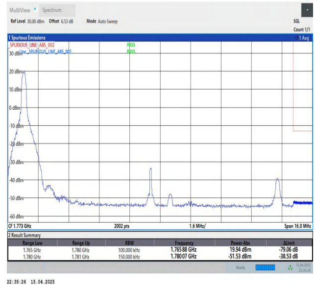
Band66-15MHz-QPSK-132597-1RB#0-PASS
