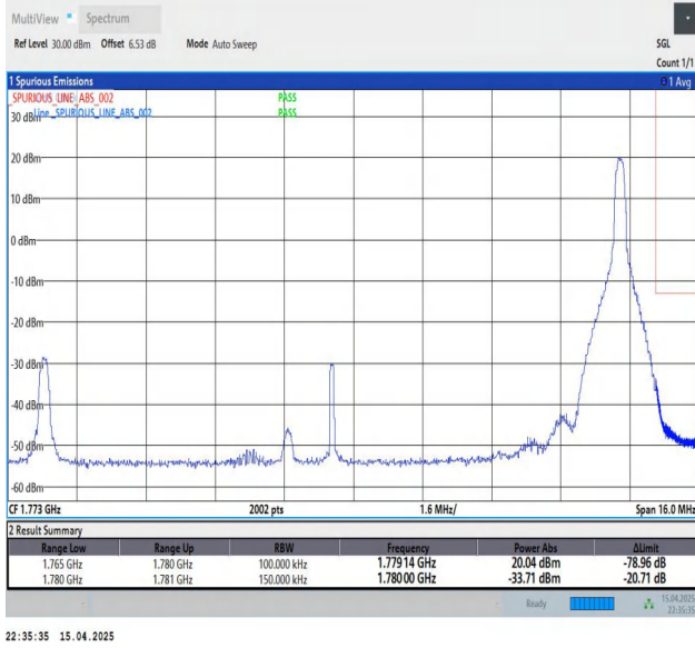
Band66-15MHz-QPSK-132597-1RB#74-PASS
