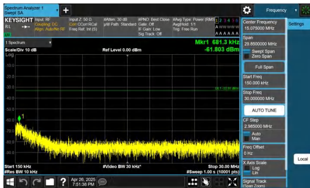
Band66-5MHz-QPSK-132647-1RB#24-0.15~30-PASS
