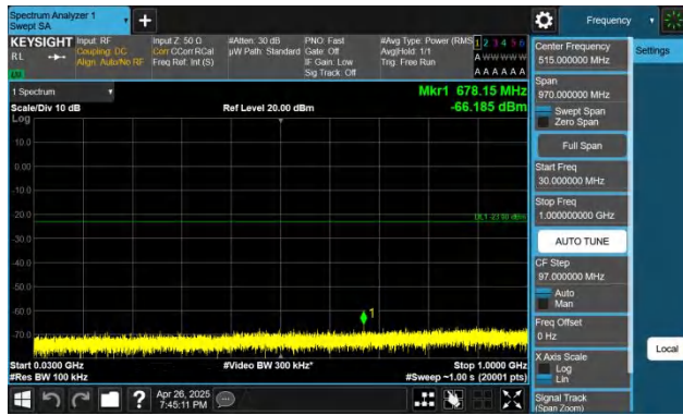
Band66-3MHz-QPSK-132322-1RB#0-30~1000-PASS
