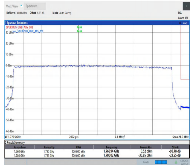
Band66-20MHz-QPSK-132572-100RB#0-PASS
