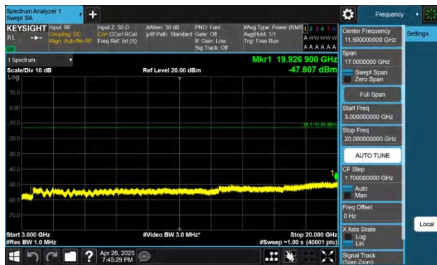
Band66-3MHz-QPSK-132322-1RB#0-3000~20000-PASS
