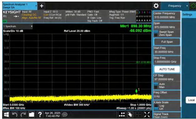
Band66-1.4MHz-QPSK-132322-1RB#0-30~1000-PASS
