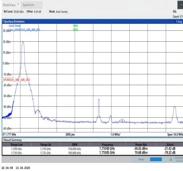
Band66-15MHz-QPSK-132047-1RB#0-PASS
