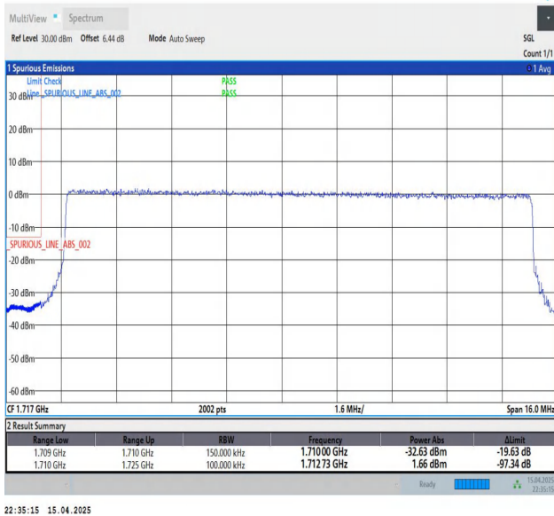
Band66-15MHz-QPSK-132047-75RB#0-PASS
