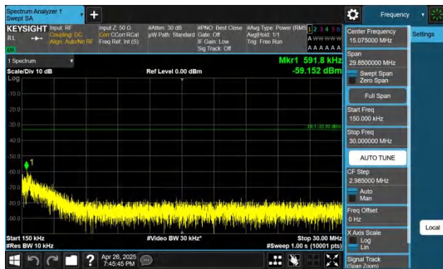
Band66-3MHz-QPSK-132322-1RB#14-0.15~30-PASS
