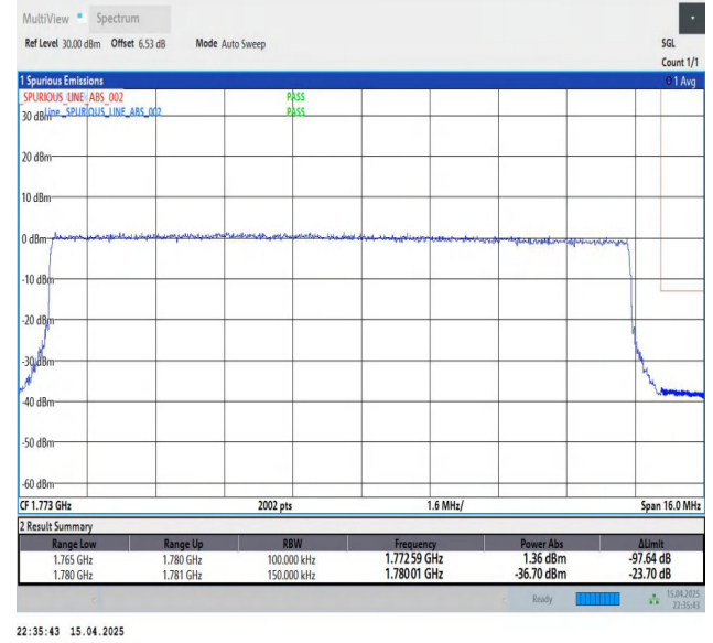
Band66-15MHz-QPSK-132597-75RB#0-PASS
