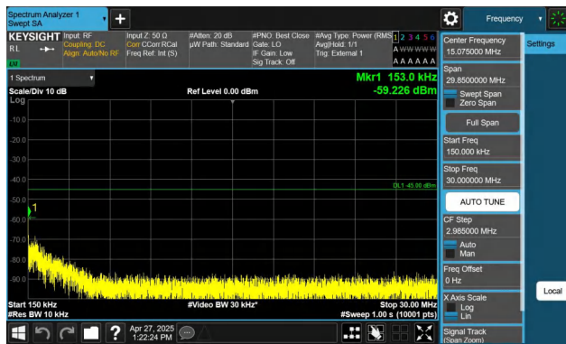
Band41-20MHz-QPSK-41490-1RB#99-0.15~30-PASS
