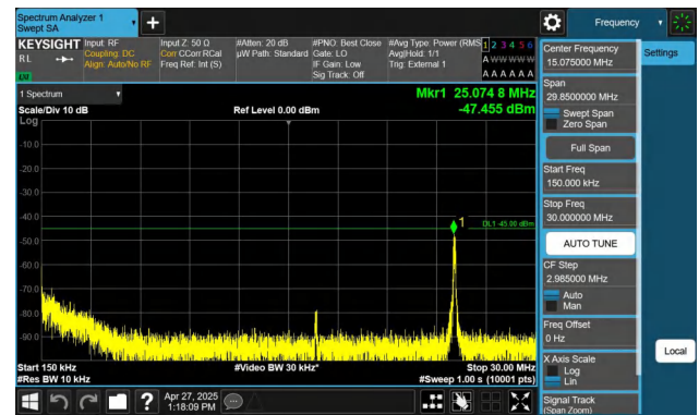
Band41-15MHz-QPSK-40620-1RB#0-0.15~30-PASS
