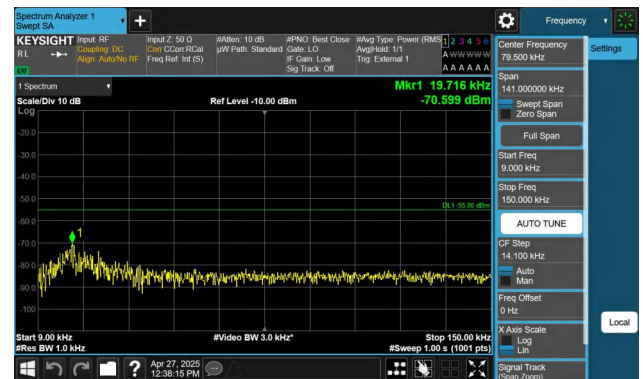
Band41-20MHz-QPSK-39750-1RB#99-0.009~0.15-PASS
