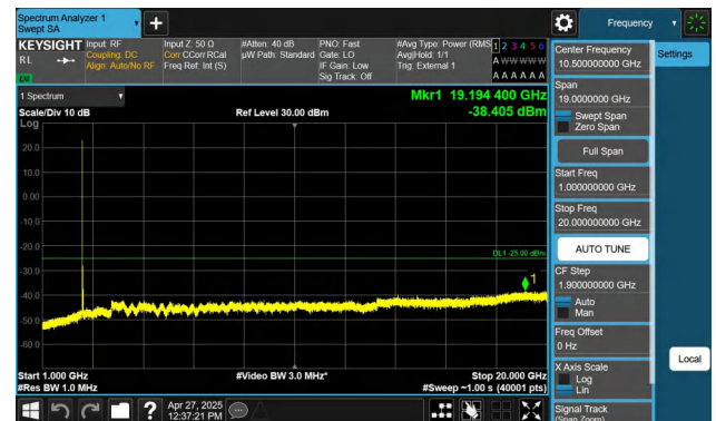
Band41-20MHz-QPSK-39750-1RB#0-1000~20000-PASS
