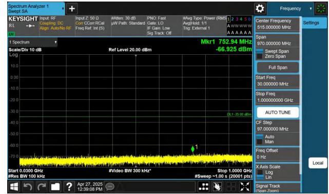
Band41-20MHz-QPSK-39750-1RB#99-30~1000-PASS
