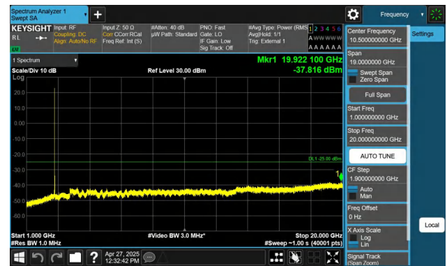
Band41-15MHz-QPSK-41515-1RB#0-1000~20000-PASS
