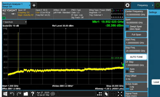
Band41-15MHz-QPSK-41515-1RB#74-1000~20000-PASS
