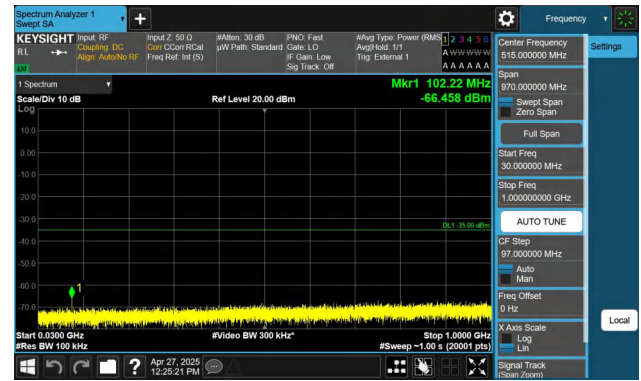
Band41-15MHz-QPSK-39725-1RB#74-30~1000-PASS
