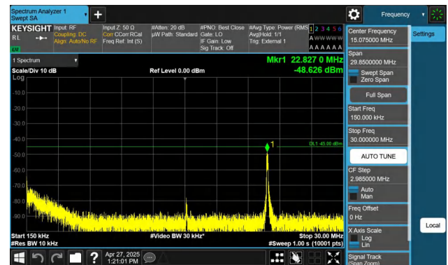
Band41-20MHz-QPSK-40620-1RB#0-0.15~30-PASS
