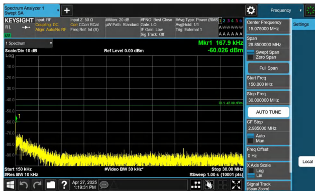
Band41-15MHz-QPSK-41515-1RB#74-0.15~30-PASS
