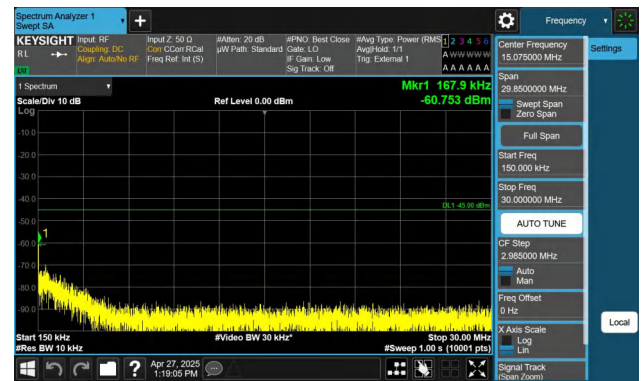
Band41-15MHz-QPSK-41515-1RB#0-0.15~30-PASS
