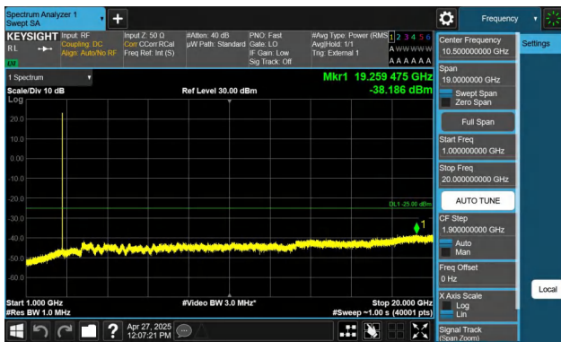
Band41-5MHz-QPSK-41565-1RB#24-1000~20000-PASS
