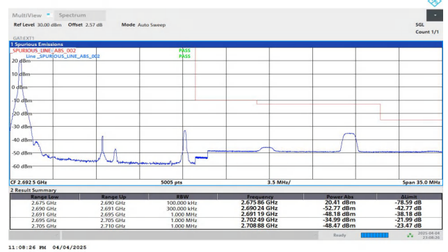
Band41-15MHz-QPSK-41515-1RB#0-PASS
