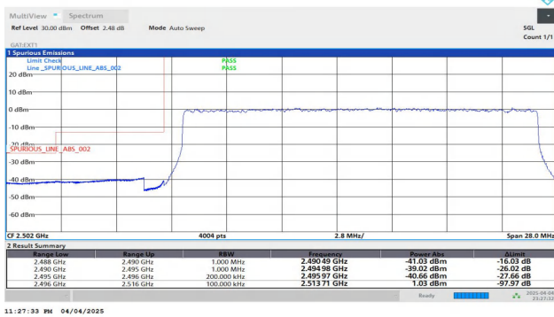
Band41-20MHz-QPSK-39750-100RB#0-PASS
