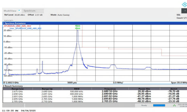
Band41-15MHz-QPSK-41515-1RB#74-PASS
