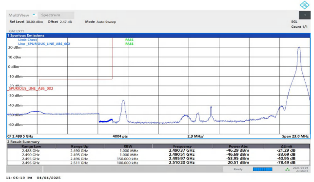
Band41-15MHz-QPSK-39725-1RB#74-PASS
