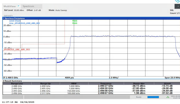
Band41-15MHz-QPSK-39725-75RB#0-PASS
