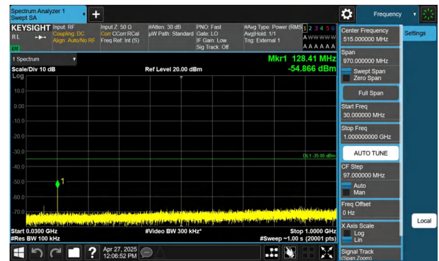
Band41-5MHz-QPSK-41565-1RB#24-30~1000-PASS
