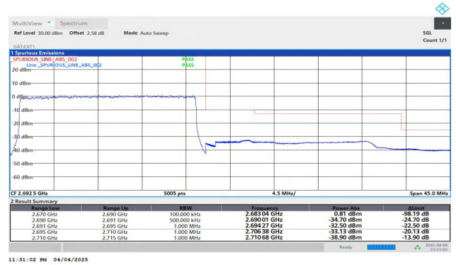
Band41-20MHz-QPSK-41490-100RB#0-PASS
