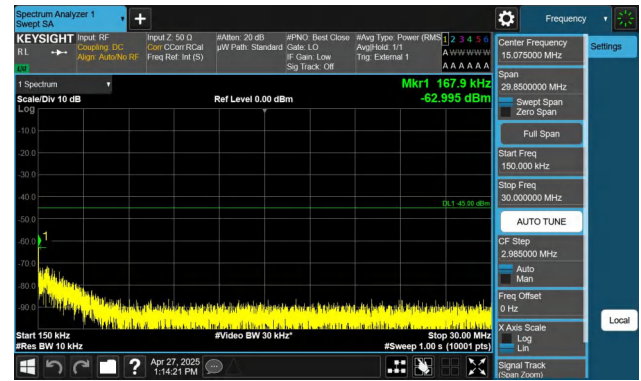
Band41-10MHz-QPSK-39700-1RB#0-0.15~30-PASS
