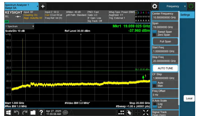
Band41-5MHz-QPSK-39675-1RB#0-1000~20000-PASS
