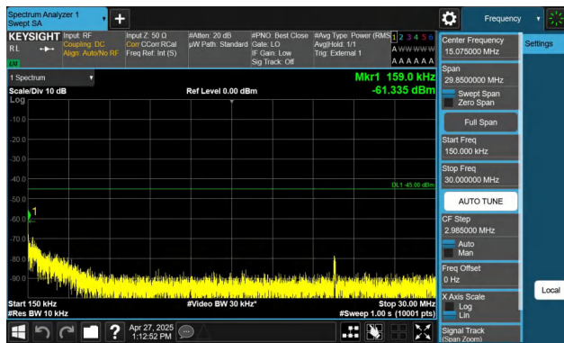
Band41-5MHz-QPSK-40620-1RB#24-0.15~30-PASS
