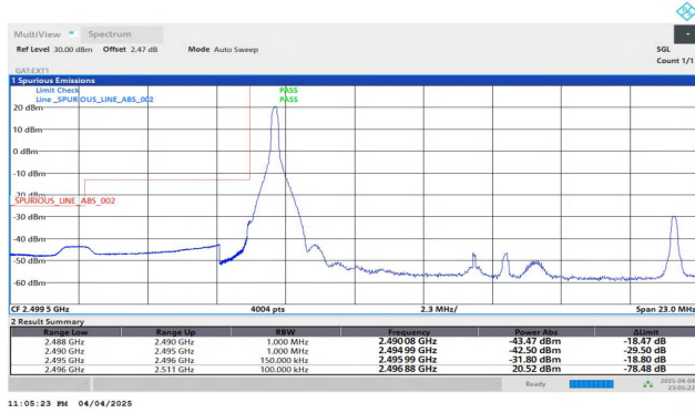
Band41-15MHz-QPSK-39725-1RB#0-PASS
