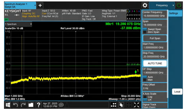
Band41-5MHz-QPSK-40620-1RB#0-1000~20000-PASS
