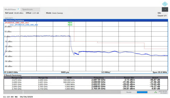
Band41-15MHz-QPSK-41515-75RB#0-PASS
