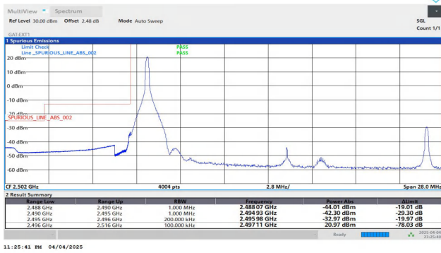
Band41-20MHz-QPSK-39750-1RB#0-PASS
