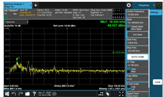
Band41-10MHz-QPSK-39700-1RB#49-0.009~0.15-PASS
