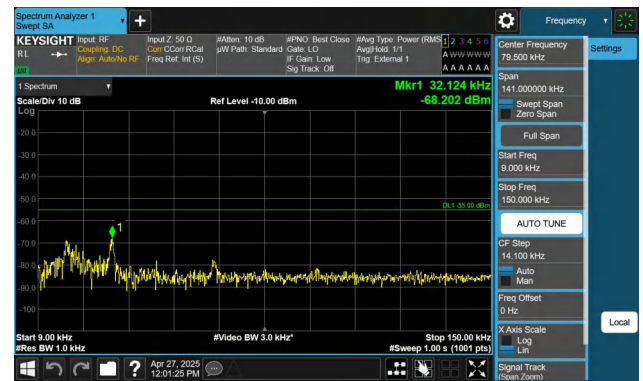
Band41-5MHz-QPSK-40620-1RB#24-0.009~0.15-PASS
