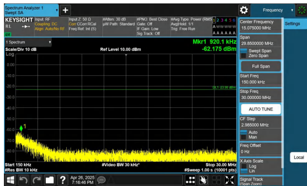
Band26(824-849)-5MHz-QPSK-26915-1RB#24-0.15~30-PASS
