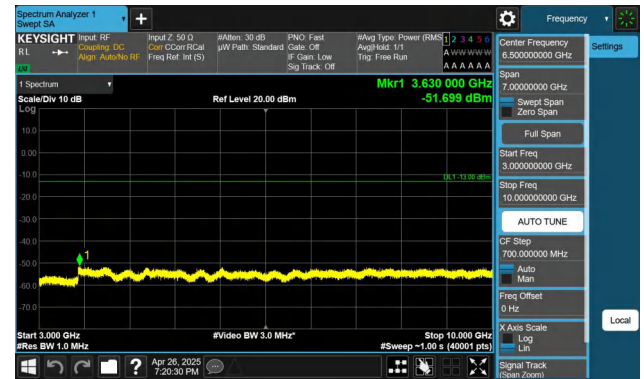
Band26(824-849)-10MHz-QPSK-26840-1RB#49-3000~10000-PAS S
