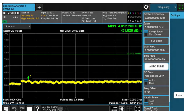
Band26(824-849)-15MHz-QPSK-26915-1RB#0-3000~10000-PAS
