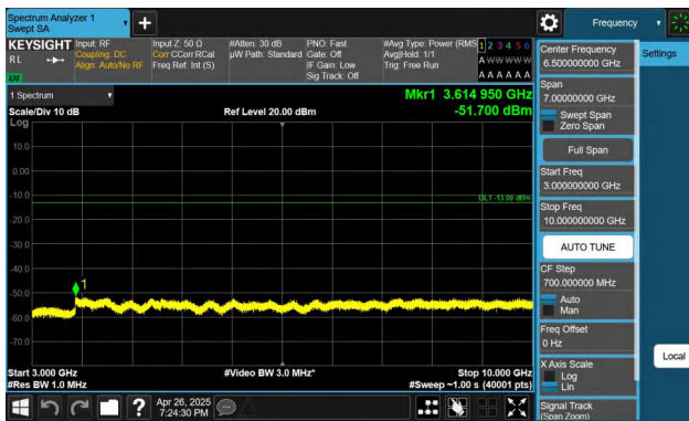
Band26(824-849)-15MHz-QPSK-26865-1RB#0-3000~10000-PAS
