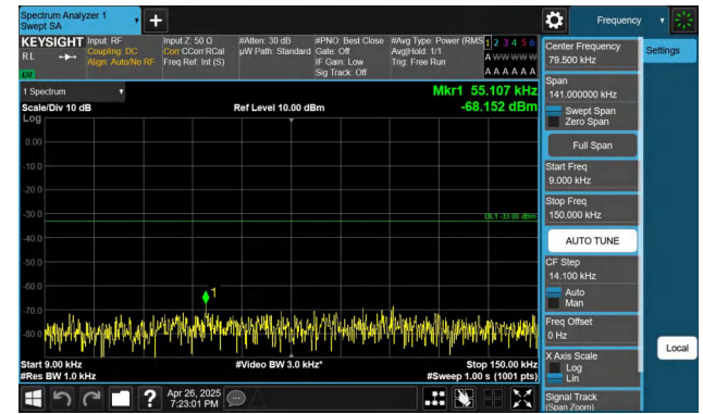
Band26(824-849)-10MHz-QPSK-26990-1RB#49-0.009~0.15-PASS
