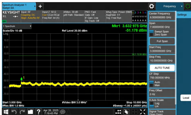
Band26(824-849)-10MHz-QPSK-26840-1RB#0-3000~10000-PAS
