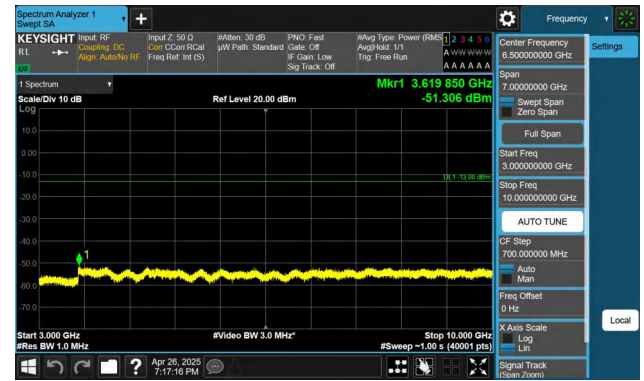
Band26(824-849)-5MHz-QPSK-26915-1RB#24-3000~10000-PASS
