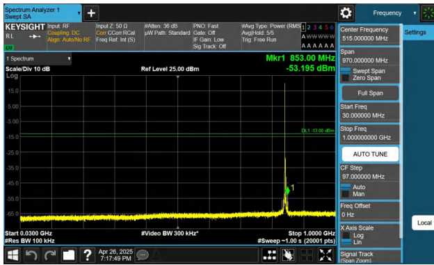
Band26(824-849)-5MHz-QPSK-27015-1RB#0-30~1000-PASS
