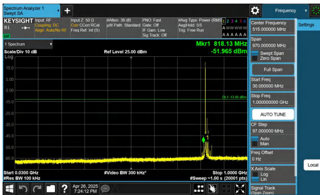
Band26(824-849)-15MHz-QPSK-26865-1RB#0-30~1000-PASS
