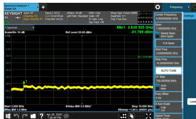
Band26(824-849)-15MHz-QPSK-26915-1RB#74-3000~10000-PAS
