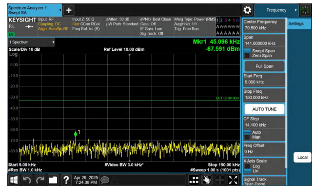
Band26(824-849)-15MHz-QPSK-26865-1RB#74-0.009~0.15-PASS
