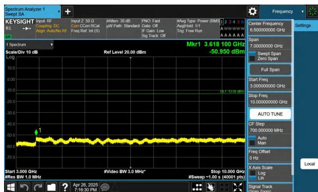
Band26(824-849)-5MHz-QPSK-26915-1RB#0-3000~10000-PASS
