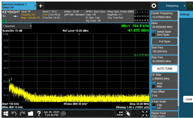
Band26(824-849)-15MHz-QPSK-26865-1RB#74-0.15~30-PASS
