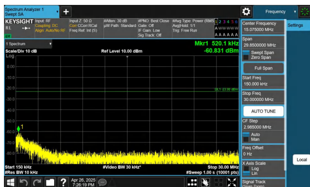
Band26(824-849)-15MHz-QPSK-26915-1RB#74-0.15~30-PASS
