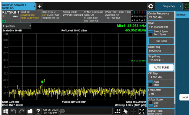
Band26(824-849)-5MHz-QPSK-27015-1RB#0-0.009~0.15-PASS
