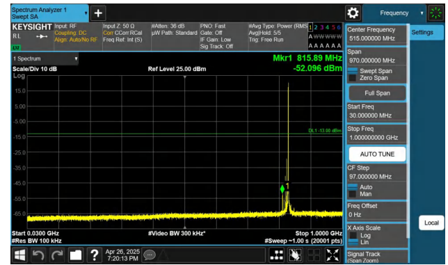
Band26(824-849)-10MHz-QPSK-26840-1RB#49-30~1000-PASS
