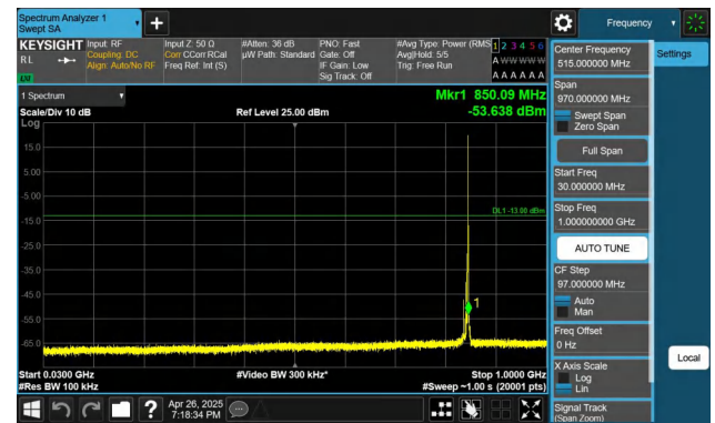
Band26(824-849)-5MHz-QPSK-27015-1RB#24-30~1000-PASS
