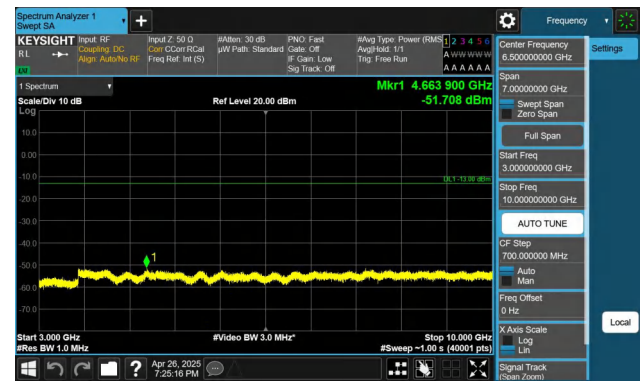
Band26(824-849)-15MHz-QPSK-26865-1RB#74-3000~10000-PAS
