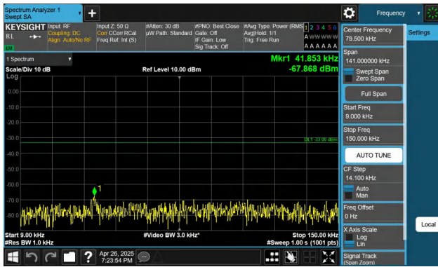
Band26(824-849)-15MHz-QPSK-26865-1RB#0-0.009~0.15-PASS
