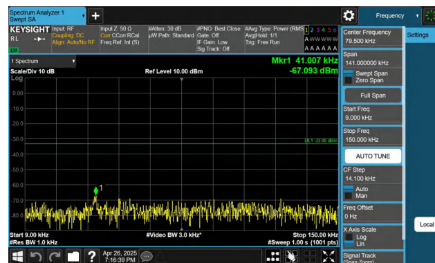
Band26(824-849)-5MHz-QPSK-26915-1RB#24-0.009~0.15-PASS
