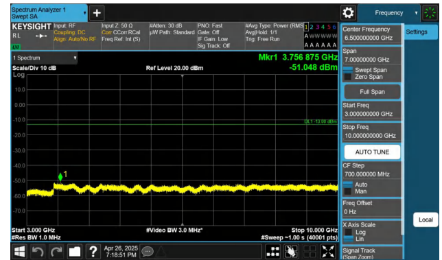
Band26(824-849)-5MHz-QPSK-27015-1RB#24-3000~10000-PASS
