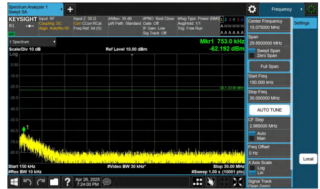
Band26(824-849)-15MHz-QPSK-26865-1RB#0-0.15~30-PASS
