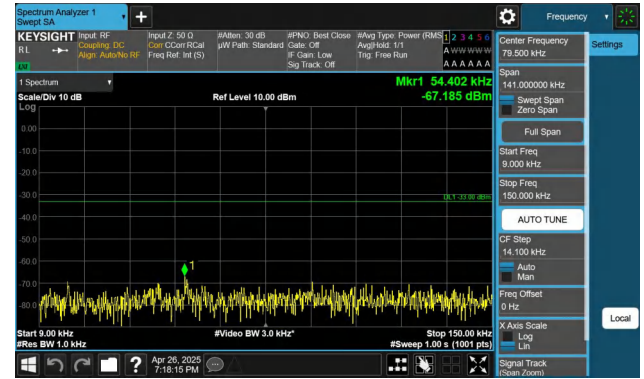
Band26(824-849)-5MHz-QPSK-27015-1RB#24-0.009~0.15-PASS
