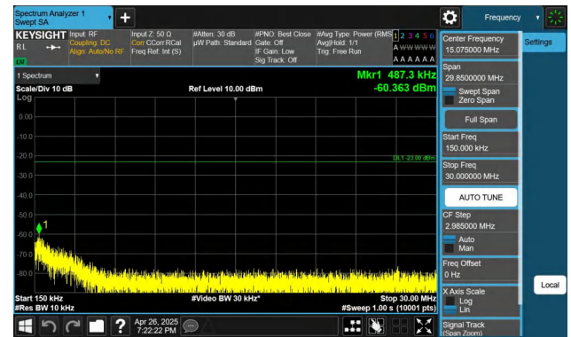
Band26(824-849)-10MHz-QPSK-26990-1RB#0-0.15~30-PASS
