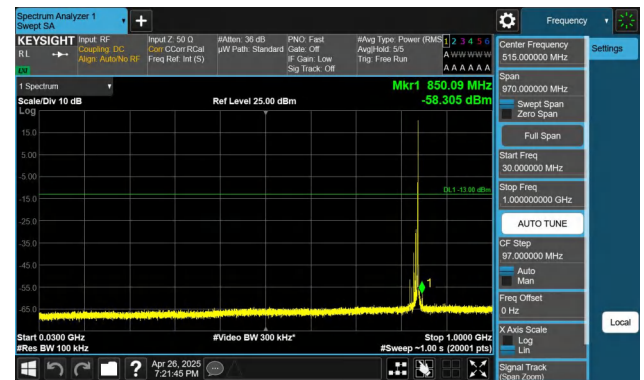
Band26(824-849)-10MHz-QPSK-26915-1RB#49-30~1000-PASS
