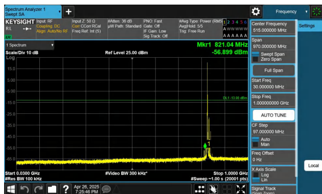
Band26(824-849)-15MHz-QPSK-26915-1RB#0-30~1000-PASS
