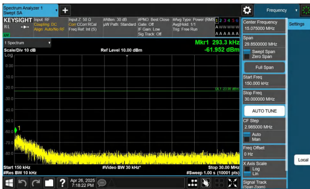
Band26(824-849)-5MHz-QPSK-27015-1RB#24-0.15~30-PASS
