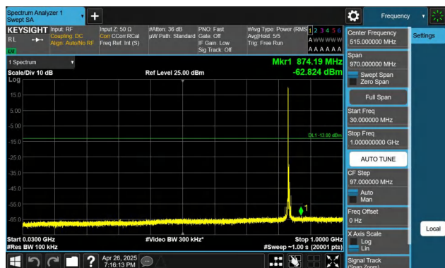
Band26(824-849)-5MHz-QPSK-26915-1RB#0-30~1000-PASS
