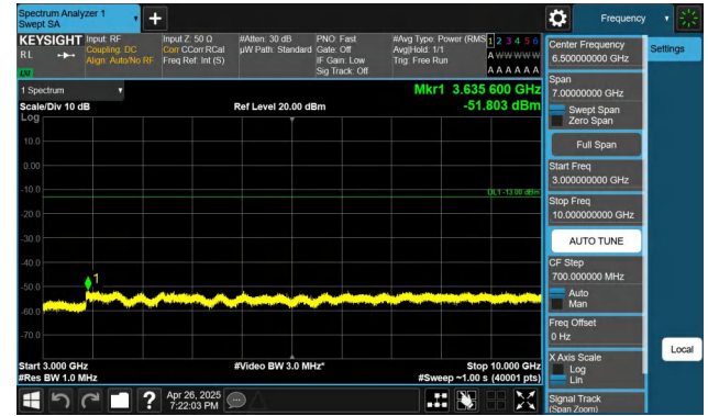
Band26(824-849)-10MHz-QPSK-26915-1RB#49-3000~10000-PAS
