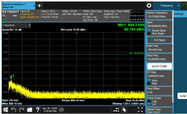
Band26(824-849)-10MHz-QPSK-26840-1RB#49-0.15~30-PASS
