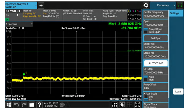
Band26(824-849)-10MHz-QPSK-26990-1RB#49-3000~10000-PAS S
