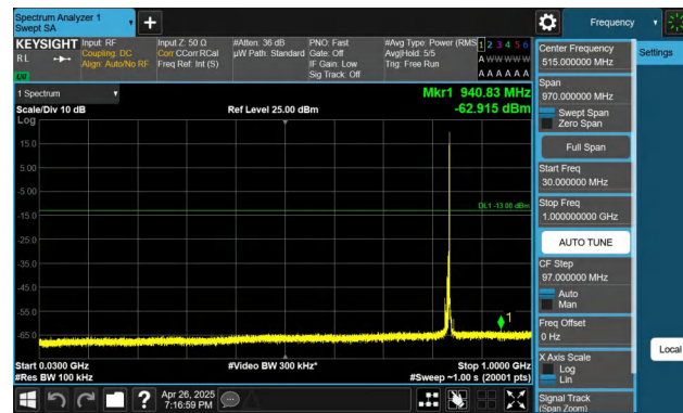
Band26(824-849)-5MHz-QPSK-26915-1RB#24-30~1000-PASS
