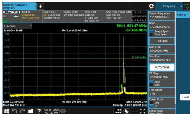
Band26(824-849)-15MHz-QPSK-26965-1RB#0-30~1000-PASS
