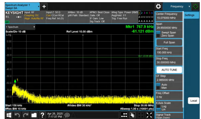
Band26(824-849)-5MHz-QPSK-27015-1RB#0-0.15~30-PASS
