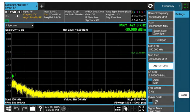
Band26(824-849)-15MHz-QPSK-26915-1RB#0-0.15~30-PASS
