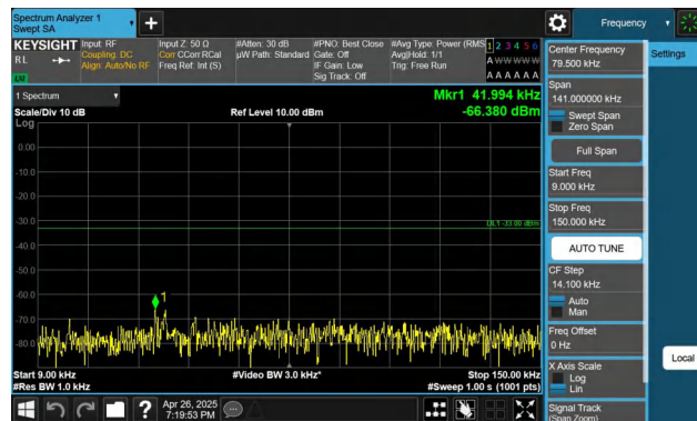
Band26(824-849)-10MHz-QPSK-26840-1RB#49-0.009~0.15-PASS
