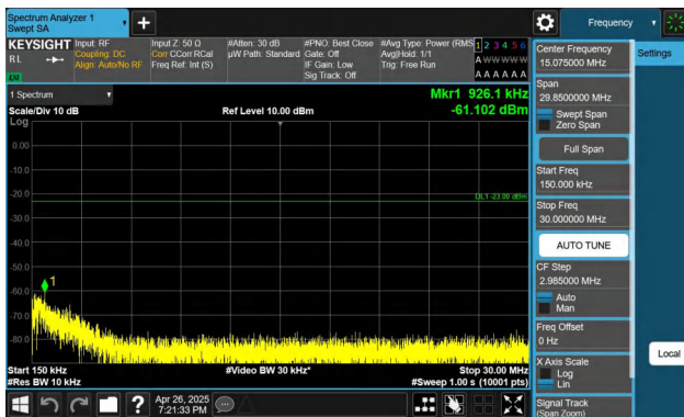
Band26(824-849)-10MHz-QPSK-26915-1RB#49-0.15~30-PASS
