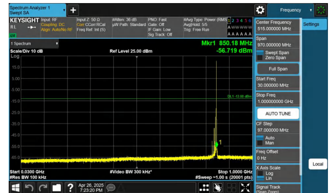
Band26(824-849)-10MHz-QPSK-26990-1RB#49-30~1000-PASS
