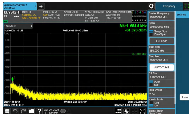
Band26(824-849)-10MHz-QPSK-26840-1RB#0-0.15~30-PASS
