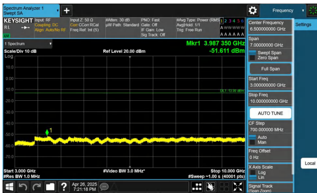
Band26(824-849)-10MHz-QPSK-26915-1RB#0-3000~10000-PASS S
