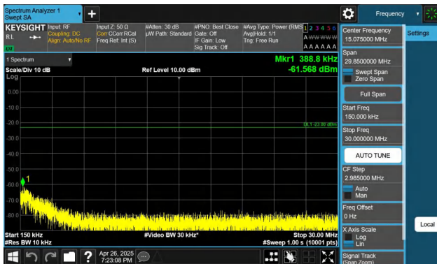
Band26(824-849)-10MHz-QPSK-26990-1RB#49-0.15~30-PASS
