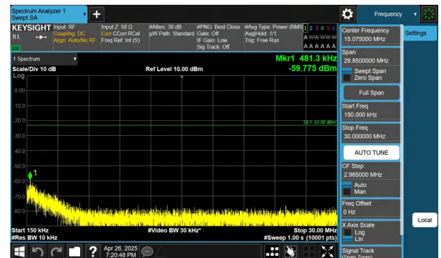
Band26(824-849)-10MHz-QPSK-26915-1RB#0-0.15~30-PASS
