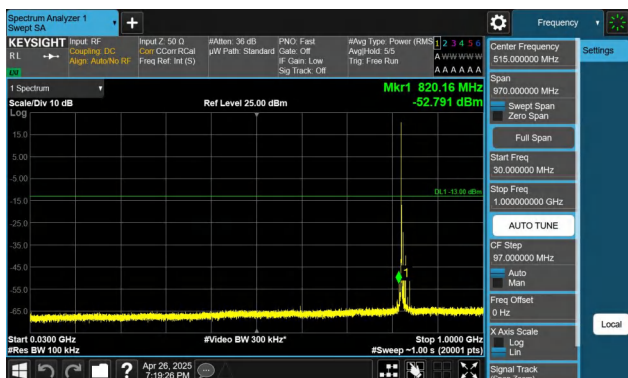
Band26(824-849)-10MHz-QPSK-26840-1RB#0-30~1000-PASS
