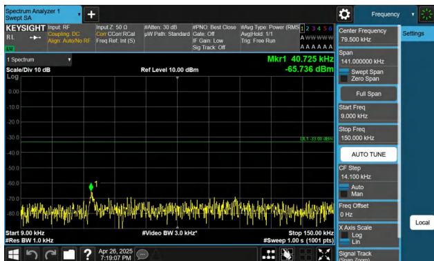
Band26(824-849)-10MHz-QPSK-26840-1RB#0-0.009~0.15-PASS
