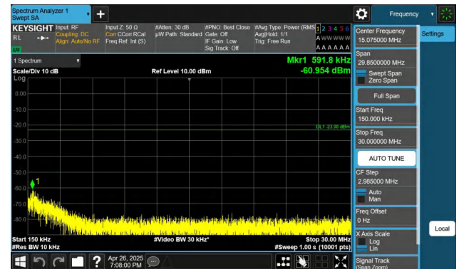
Band26(824-849)-1.4MHz-QPSK-27033-1RB#0-0.15~30-PASS
