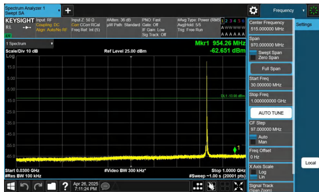
Band26(824-849)-3MHz-QPSK-26915-1RB#0-30~1000-PASS
