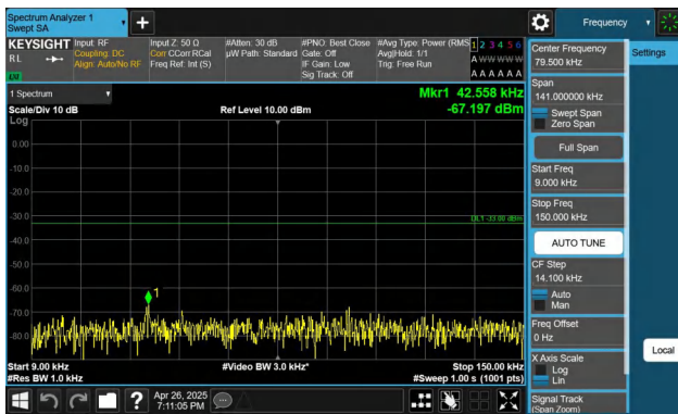
Band26(824-849)-3MHz-QPSK-26915-1RB#0-0.009~0.15-PASS
