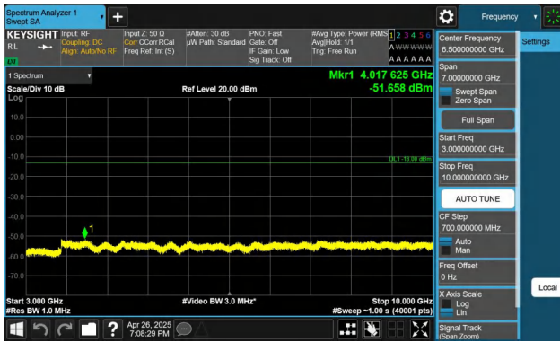
Band26(824-849)-1.4MHz-QPSK-27033-1RB#0-3000~10000-PAS S
