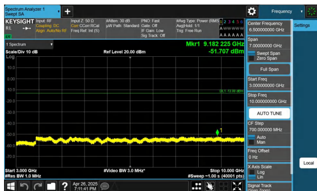
Band26(824-849)-3MHz-QPSK-26915-1RB#0-3000~10000-PASS
