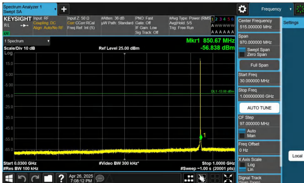
Band26(824-849)-1.4MHz-QPSK-27033-1RB#0-30~1000-PASS
