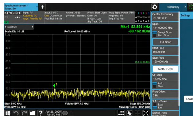
Band26(824-849)-3MHz-QPSK-26915-1RB#14-0.009~0.15-PASS
