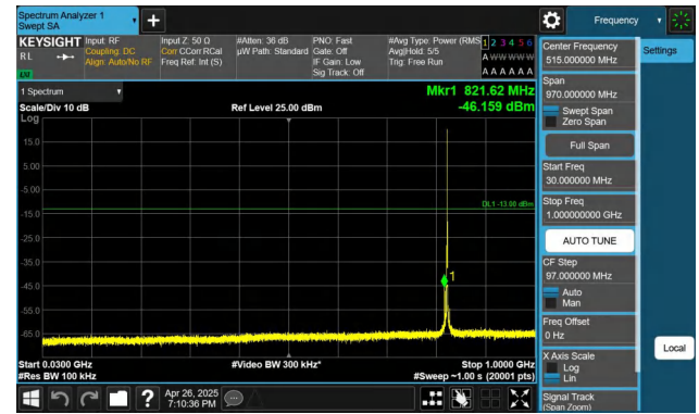
Band26(824-849)-3MHz-QPSK-26805-1RB#14-30~1000-PASS
