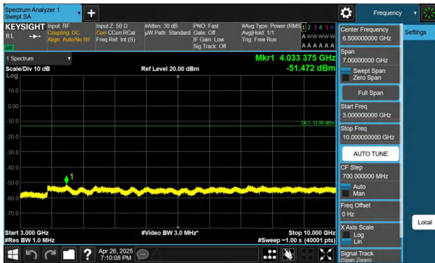
Band26(824-849)-3MHz-QPSK-26805-1RB#0-3000~10000-PASS
