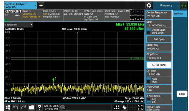
Band26(824-849)-3MHz-QPSK-26805-1RB#14-0.009~0.15-PASS
