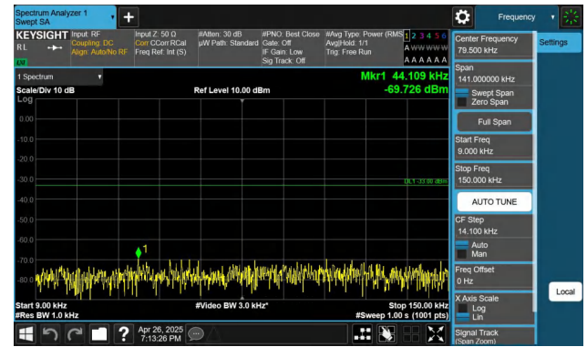
Band26(824-849)-3MHz-QPSK-27025-1RB#14-0.009~0.15-PASS
