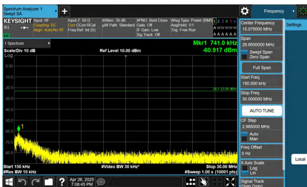
Band26(824-849)-1.4MHz-QPSK-27033-1RB#5-0.15~30-PASS
