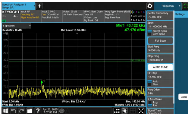
Band26(824-849)-1.4MHz-QPSK-27033-1RB#0-0.009~0.15-PASS
