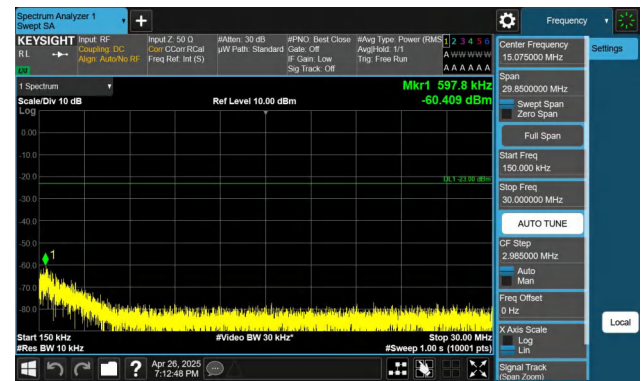
Band26(824-849)-3MHz-QPSK-27025-1RB#0-0.15~30-PASS
