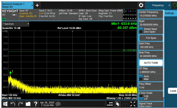
Band26(824-849)-3MHz-QPSK-26805-1RB#14-0.15~30-PASS
