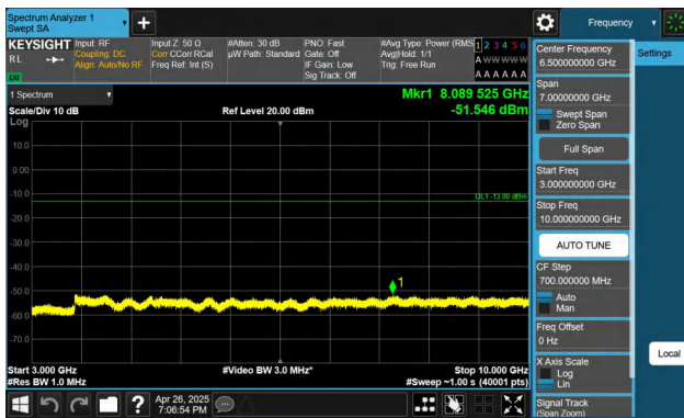
Band26(824-849)-1.4MHz-QPSK-26915-1RB#0-3000~10000-PASS S
