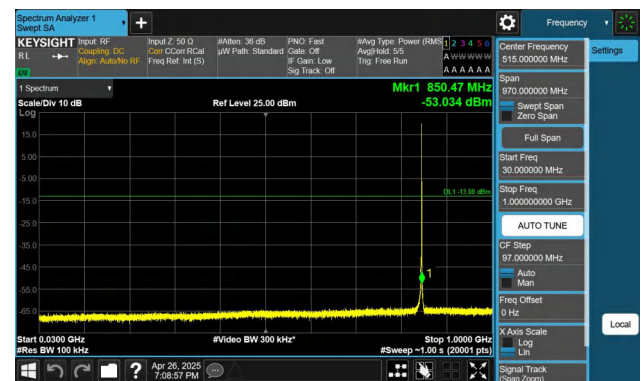
Band26(824-849)-1.4MHz-QPSK-27033-1RB#5-30~1000-PASS
