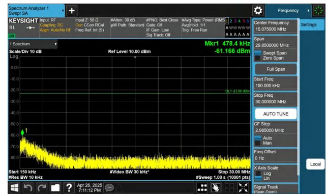
Band26(824-849)-3MHz-QPSK-26915-1RB#0-0.15~30-PASS
