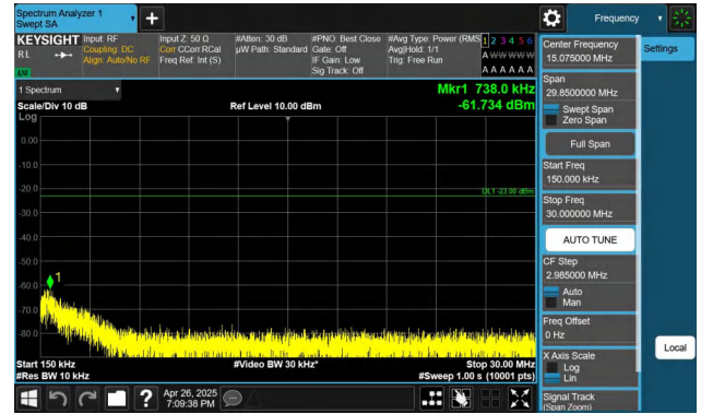
Band26(824-849)-3MHz-QPSK-26805-1RB#0-0.15~30-PASS
