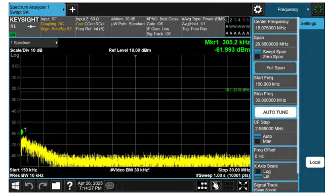
Band26(824-849)-5MHz-QPSK-26815-1RB#0-0.15~30-PASS
