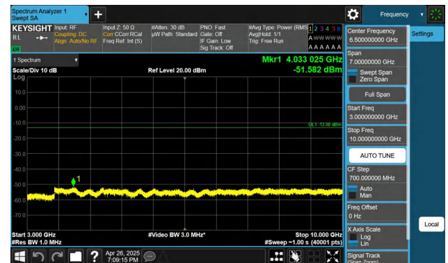
Band26(824-849)-1.4MHz-QPSK-27033-1RB#5-3000~10000-PAS S
