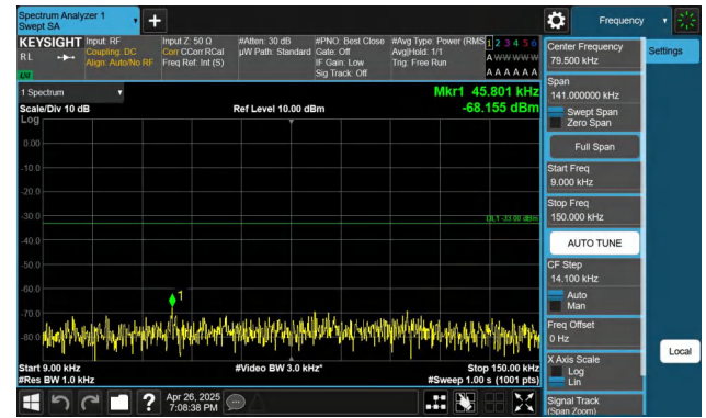
Band26(824-849)-1.4MHz-QPSK-27033-1RB#5-0.009~0.15-PASS
