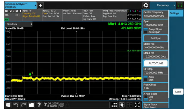
Band26(824-849)-3MHz-QPSK-26915-1RB#14-3000~10000-PASS
