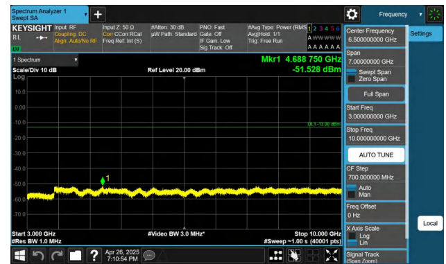
Band26(824-849)-3MHz-QPSK-26805-1RB#14-3000~10000-PASS
