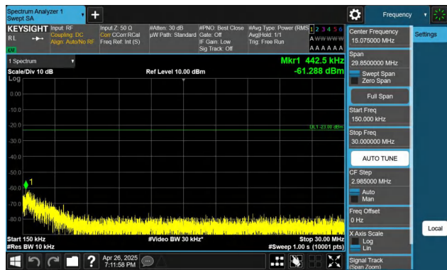
Band26(824-849)-3MHz-QPSK-26915-1RB#14-0.15~30-PASS
