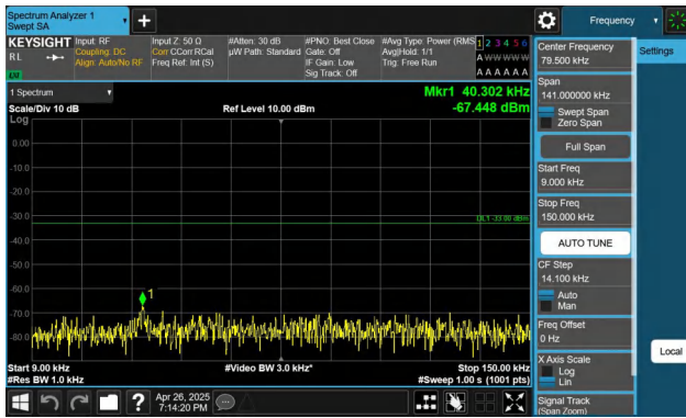
Band26(824-849)-5MHz-QPSK-26815-1RB#0-0.009~0.15-PASS
