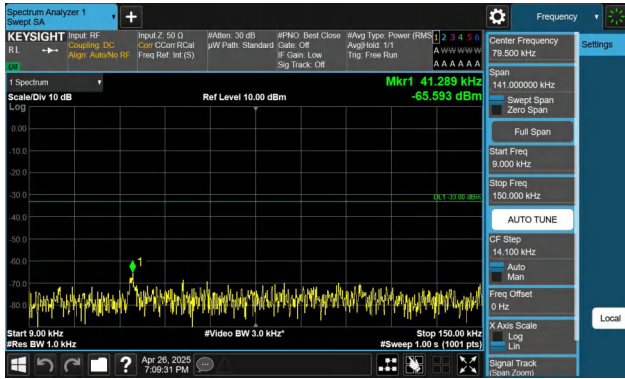
Band26(824-849)-3MHz-QPSK-26805-1RB#0-0.009~0.15-PASS
