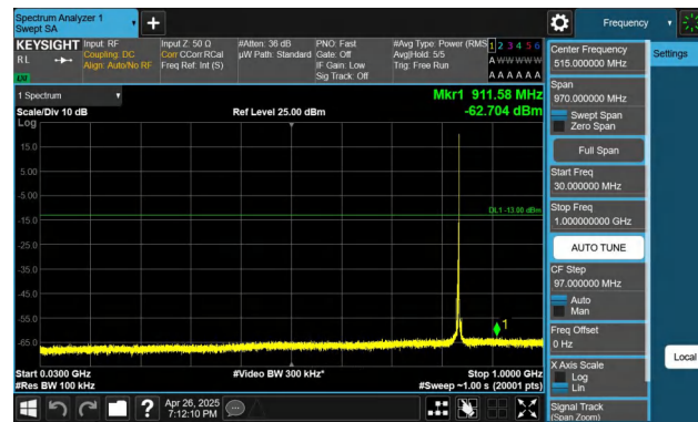
Band26(824-849)-3MHz-QPSK-26915-1RB#14-30~1000-PASS
