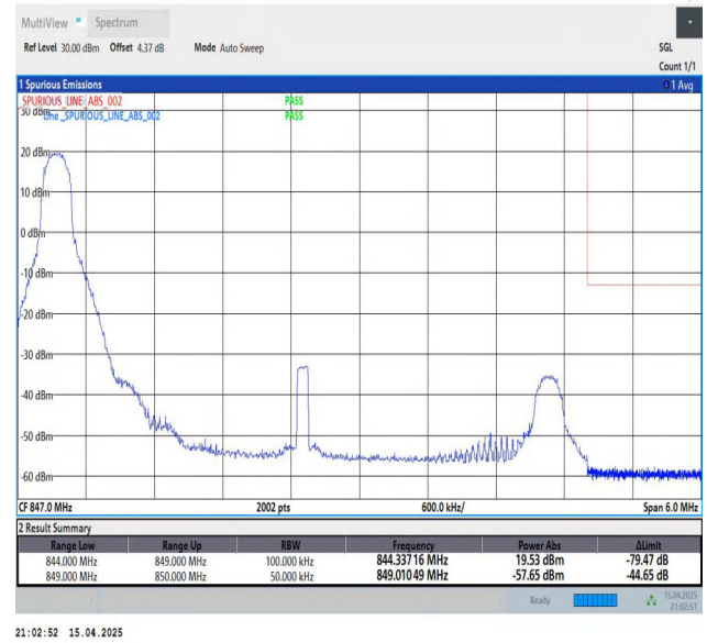
Band26(824-849)-5MHz-QPSK-27015-1RB#0-PASS
