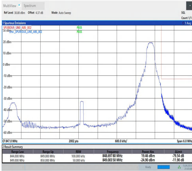
Band26(824-849)-5MHz-QPSK-27015-1RB#24-PASS
