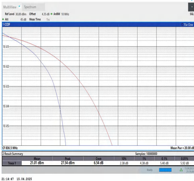
Band26(824-849)-10MHz-QPSK-26915-50RB#0-PASS
