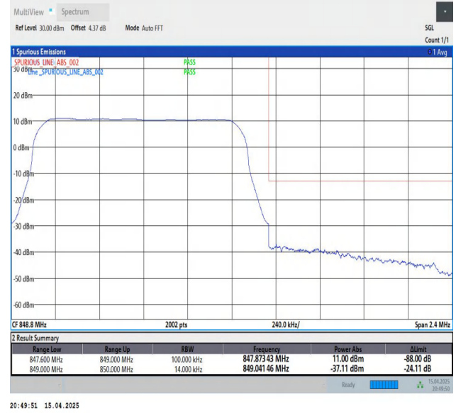
Band26(824-849)-1.4MHz-QPSK-27033-6RB#0-PASS
