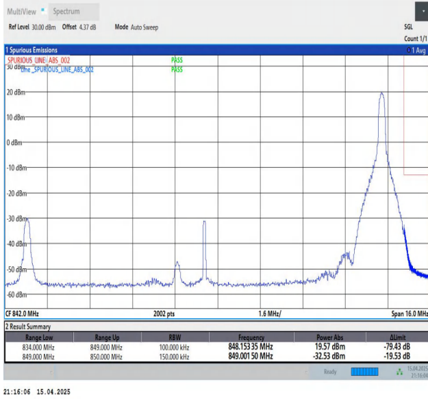
Band26(824-849)-15MHz-QPSK-26965-1RB#74-PASS
