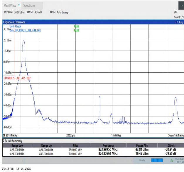
Band26(824-849)-15MHz-QPSK-26865-1RB#0-PASS
