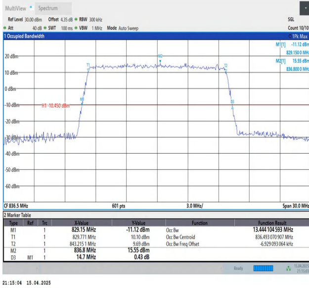
Band26(824-849)-15MHz-QPSK-26915-75RB#0-PASS
