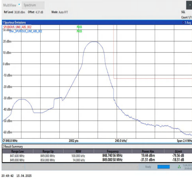
Band26(824-849)-1.4MHz-QPSK-27033-1RB#5-PASS
