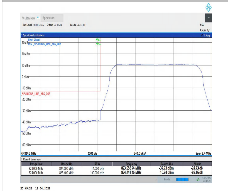
Band26(824-849)-1.4MHz-QPSK-26797-6RB#0-PASS
