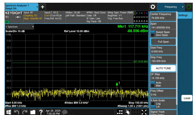
Band26(824-849)-1.4MHz-QPSK-26797-1RB#5-0.009~0.15-PASS
