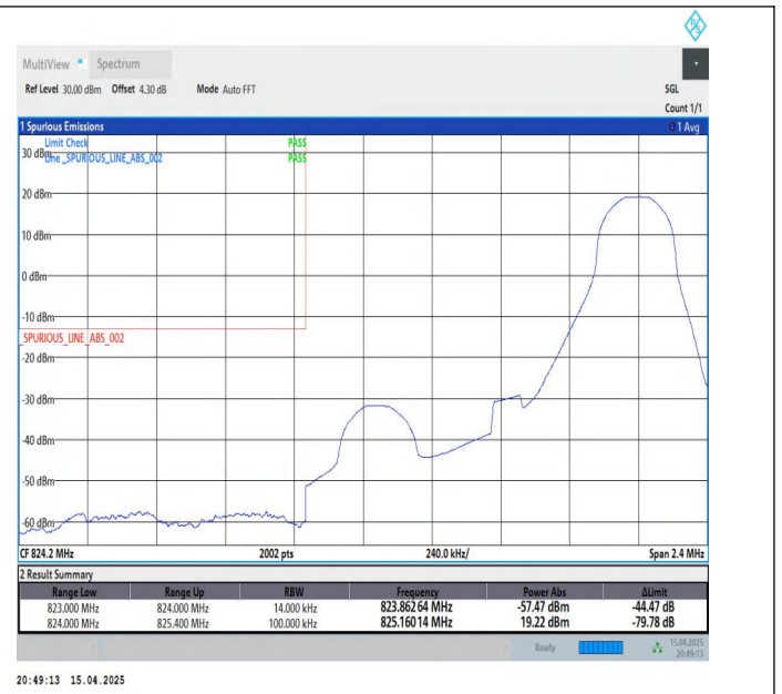
Band26(824-849)-1.4MHz-QPSK-26797-1RB#5-PASS
