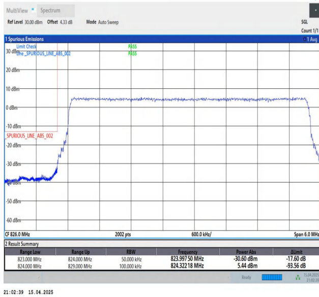
Band26(824-849)-5MHz-QPSK-26815-25RB#0-PASS
