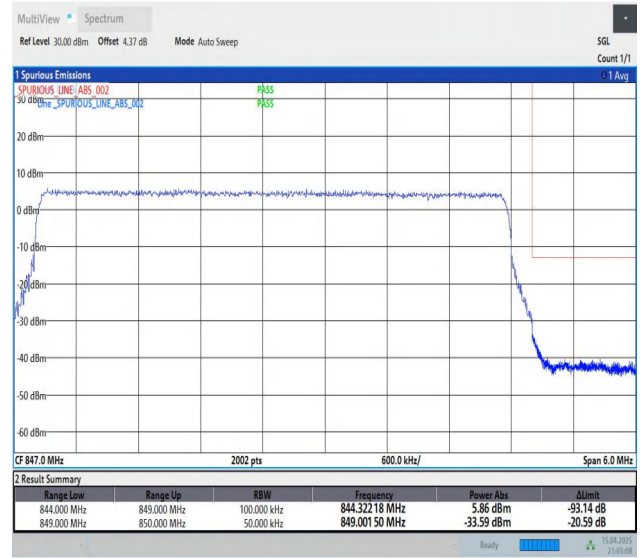
Band26(824-849)-5MHz-QPSK-27015-25RB#0-PASS
