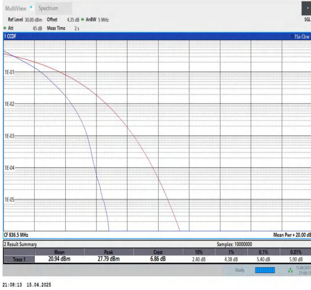
Band26(824-849)-5MHz-QPSK-26915-25RB#0-PASS
