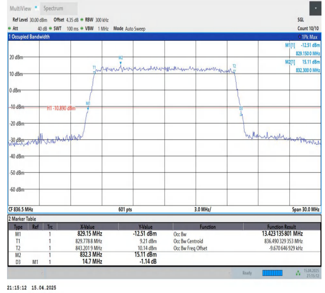
Band26(824-849)-15MHz-16QAM-26915-75RB#0-PASS
