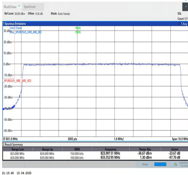
Band26(824-849)-15MHz-QPSK-26865-75RB#0-PASS
