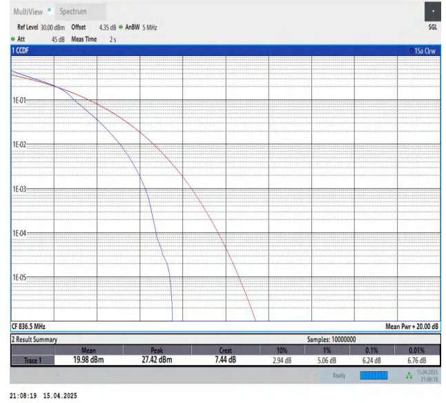
Band26(824-849)-5MHz-16QAM-26915-25RB#0-PASS
