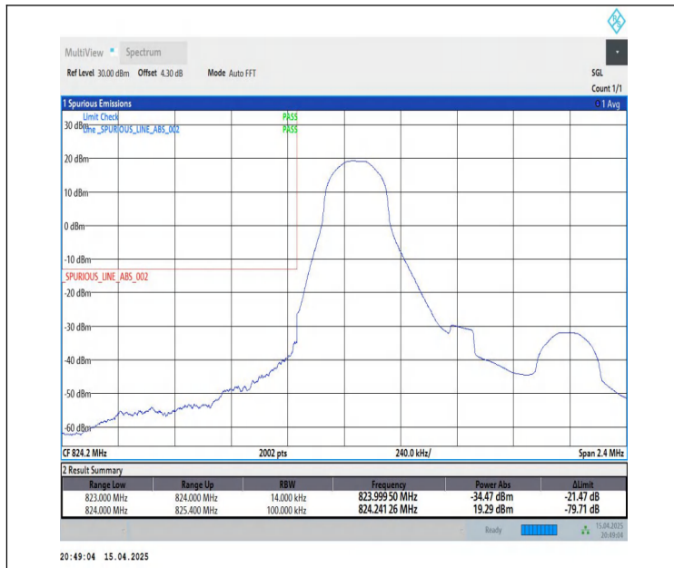
Band26(824-849)-1.4MHz-QPSK-26797-1RB#0-PASS
