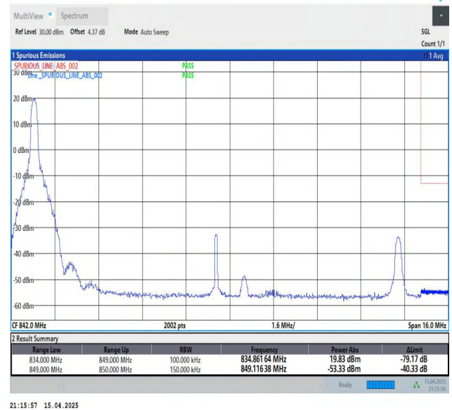
Band26(824-849)-15MHz-QPSK-26965-1RB#0-PASS
