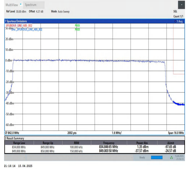
Band26(824-849)-15MHz-QPSK-26965-75RB#0-PASS
