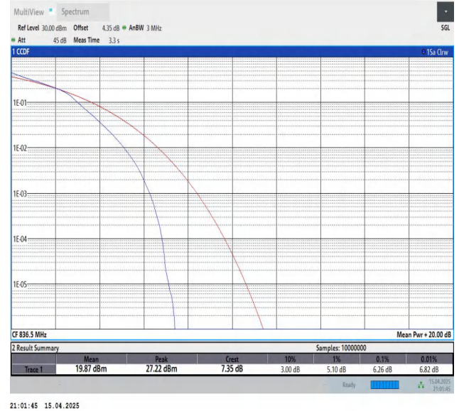
Band26(824-849)-3MHz-16QAM-26915-15RB#0-PASS
