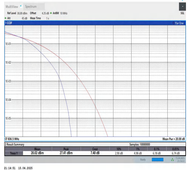
Band26(824-849)-10MHz-16QAM-26915-50RB#0-PASS
