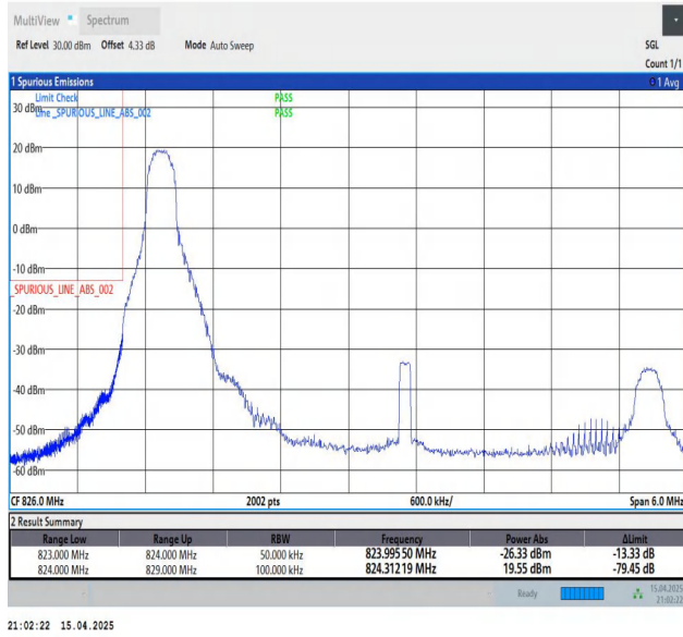
Band26(824-849)-5MHz-QPSK-26815-1RB#0-PASS
