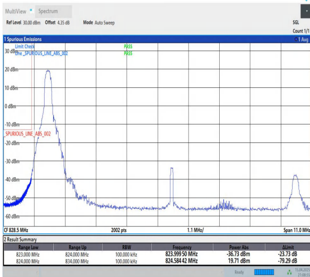
Band26(824-849)-10MHz-QPSK-26840-1RB#0-PASS
