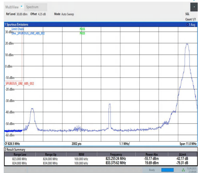
Band26(824-849)-10MHz-QPSK-26840-1RB#49-PASS
