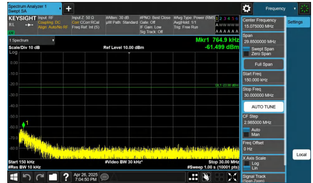
Band26(824-849)-1.4MHz-QPSK-26797-1RB#0-0.15~30-PASS
