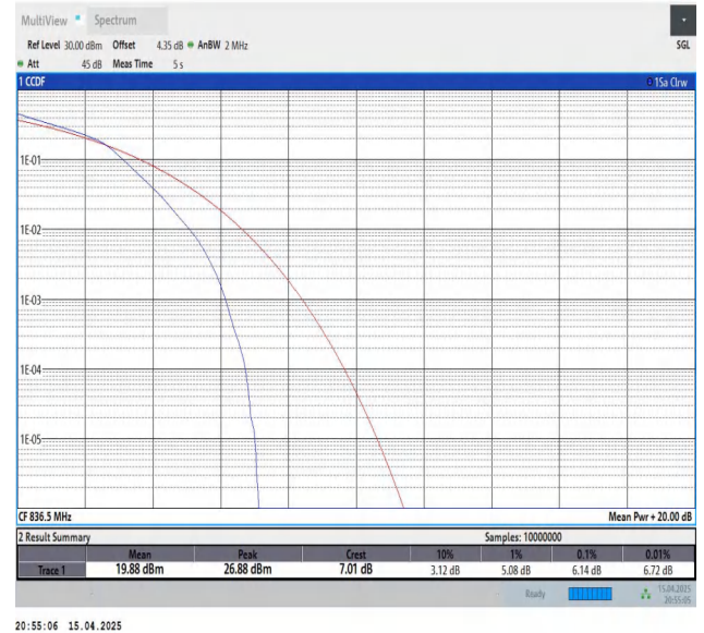
Band26(824-849)-1.4MHz-16QAM-26915-6RB#0-PASS
