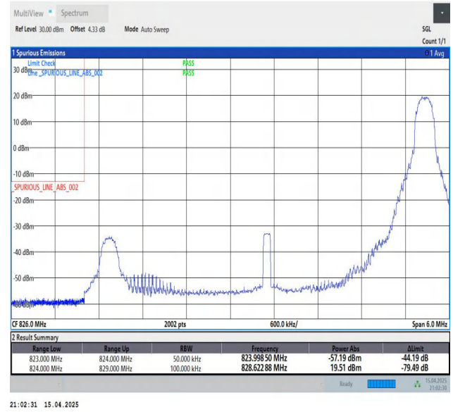
Band26(824-849)-5MHz-QPSK-26815-1RB#24-PASS
