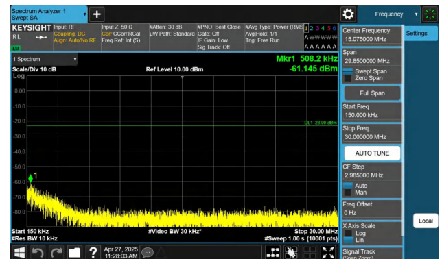
Band26(814-824)-3MHz-QPSK-26775-1RB#0-0.15~30-PASS
