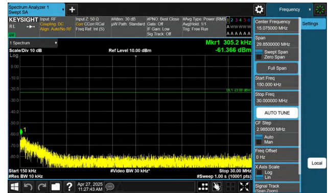
Band26(814-824)-3MHz-QPSK-26740-1RB#0-0.15~30-PASS
