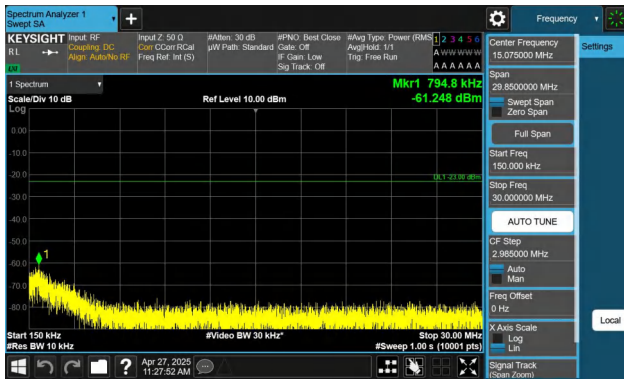
Band26(814-824)-3MHz-QPSK-26740-1RB#14-0.15~30-PASS
