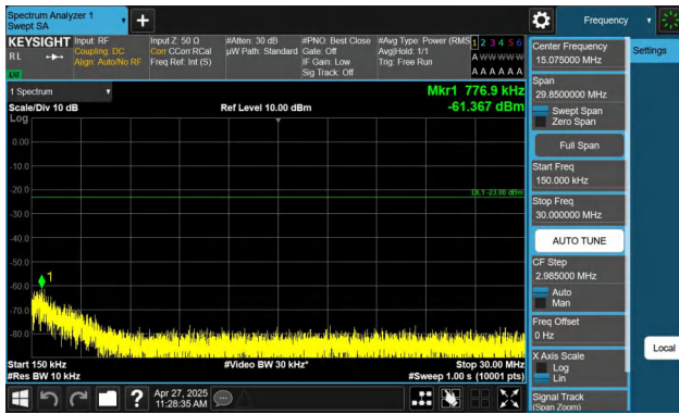
Band26(814-824)-5MHz-QPSK-26715-1RB#24-0.15~30-PASS
