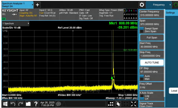
Band26(814-824)-5MHz-QPSK-26740-1RB#0-30~1000-PASS
