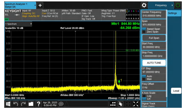
Band26(814-824)-5MHz-QPSK-26715-1RB#24-30~1000-PASS
