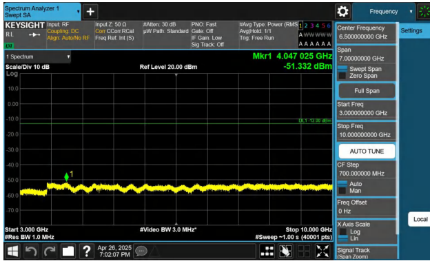
Band26(814-824)-5MHz-QPSK-26765-1RB#0-3000~10000-PASS
