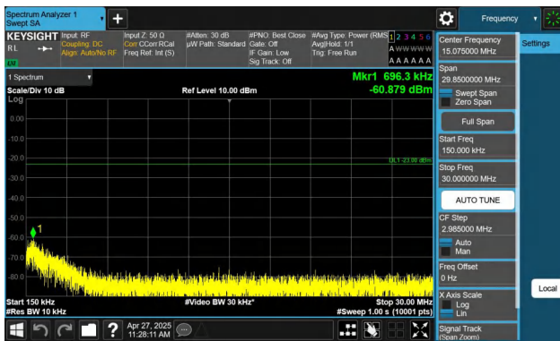
Band26(814-824)-3MHz-QPSK-26775-1RB#14-0.15~30-PASS
