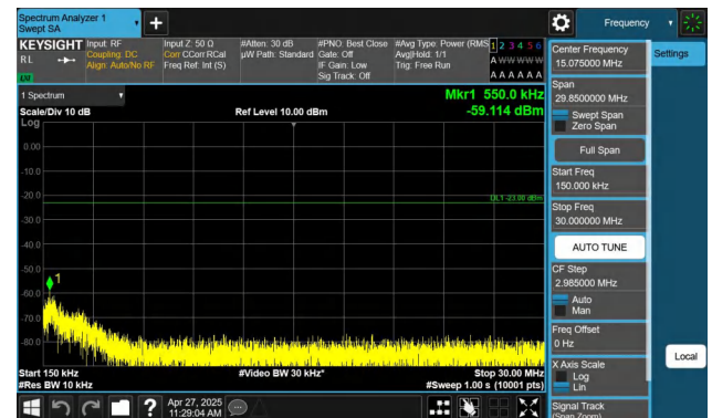
Band26(814-824)-5MHz-QPSK-26765-1RB#0-0.15~30-PASS
