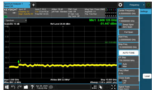
Band26(814-824)-5MHz-QPSK-26715-1RB#24-3000~10000-PASS
