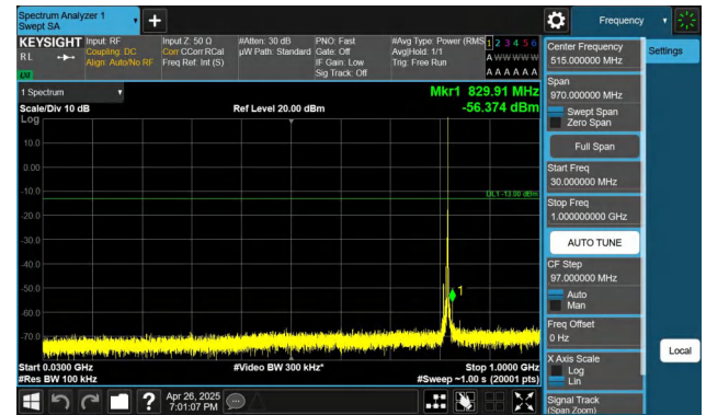
Band26(814-824)-5MHz-QPSK-26740-1RB#24-30~1000-PASS
