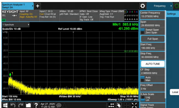
Band26(814-824)-5MHz-QPSK-26765-1RB#24-0.15~30-PASS
