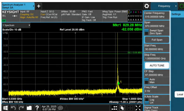
Band26(814-824)-3MHz-QPSK-26775-1RB#0-30~1000-PASS
