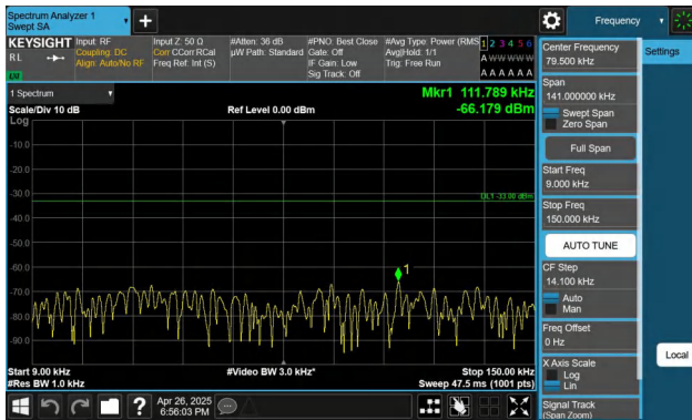
Band26(814-824)-3MHz-QPSK-26740-1RB#0-0.009~0.15-PASS
