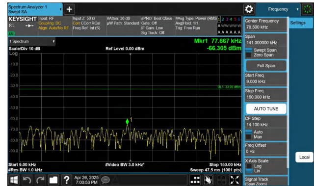
Band26(814-824)-5MHz-QPSK-26740-1RB#24-0.009~0.15-PASS
