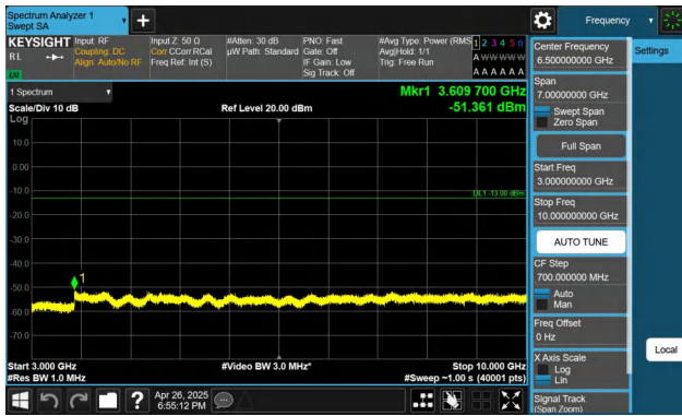
Band26(814-824)-3MHz-QPSK-26705-1RB#0-3000~10000-PASS
