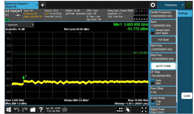
Band26(814-824)-5MHz-QPSK-26740-1RB#24-3000~10000-PASS
