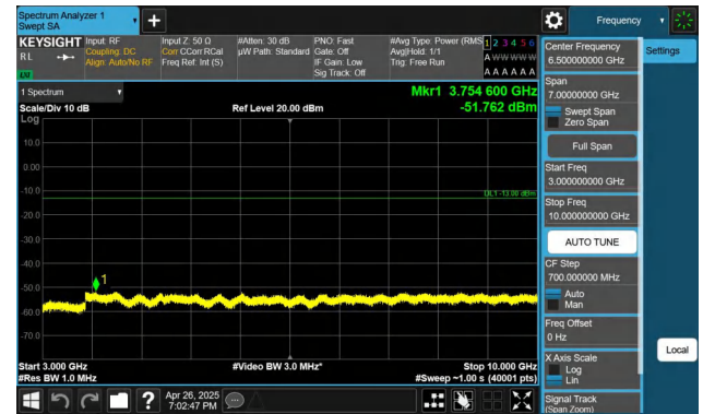
Band26(814-824)-5MHz-QPSK-26765-1RB#24-3000~10000-PASS
