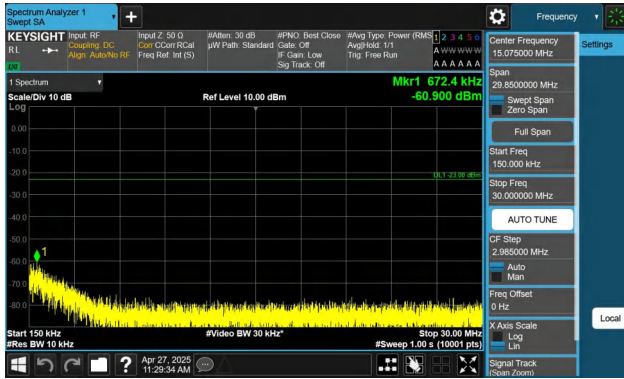
Band26(814-824)-10MHz-QPSK-26740-1RB#49-0.15~30-PASS
