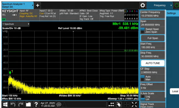
Band26(814-824)-5MHz-QPSK-26740-1RB#24-0.15~30-PASS
