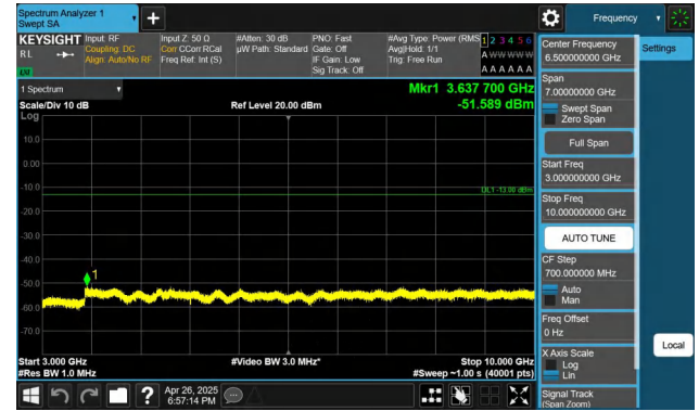
Band26(814-824)-3MHz-QPSK-26740-1RB#14-3000~10000-PASS
