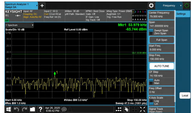
Band26(814-824)-3MHz-QPSK-26740-1RB#14-0.009~0.15-PASS
