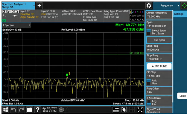
Band26(814-824)-3MHz-QPSK-26705-1RB#0-0.009~0.15-PASS
