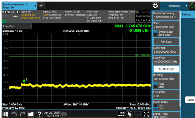
Band26(814-824)-5MHz-QPSK-26740-1RB#0-3000~10000-PASS
