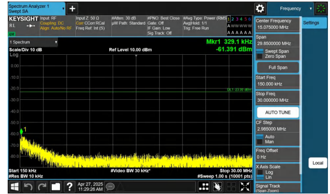
Band26(814-824)-10MHz-QPSK-26740-1RB#0-0.15~30-PASS
