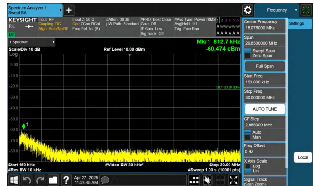
Band26(814-824)-5MHz-QPSK-26740-1RB#0-0.15~30-PASS
