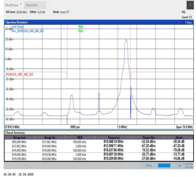
Band26(814-824)-5MHz-QPSK-26715-1RB#24-PASS
