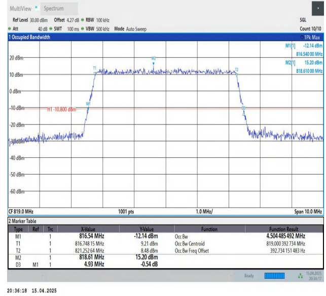
Band26(814-824)-5MHz-16QAM-26740-25RB#0-PASS
