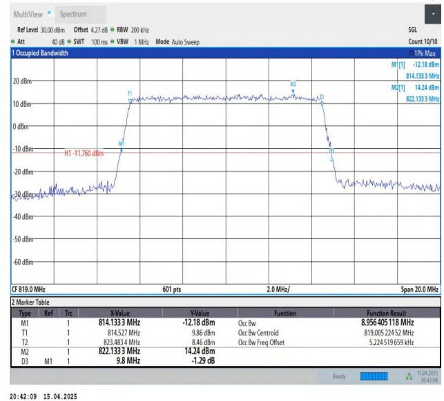
Band26(814-824)-10MHz-16QAM-26740-50RB#0-PASS
