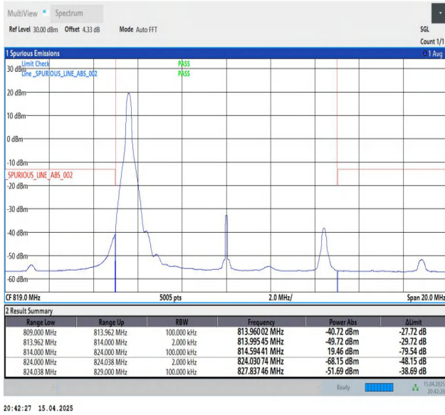
Band26(814-824)-10MHz-QPSK-26740-1RB#0-PASS
