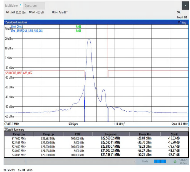
Band26(814-824)-1.4MHz-QPSK-26783-1RB#0-PASS
