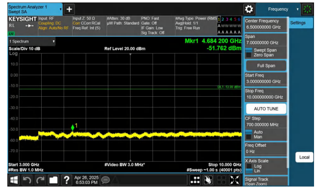
Band26(814-824)-1.4MHz-QPSK-26740-1RB#5-3000~10000-PASS
