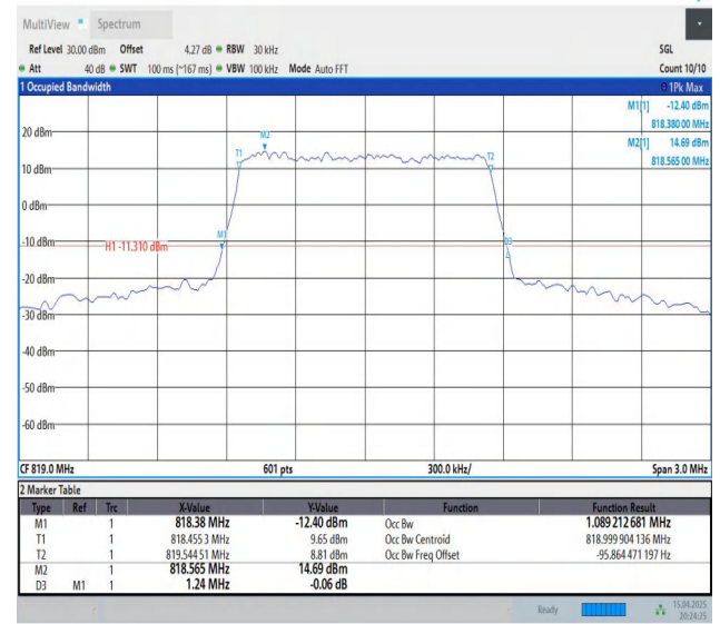
Band26(814-824)-1.4MHz-16QAM-26740-6RB#0-PASS
