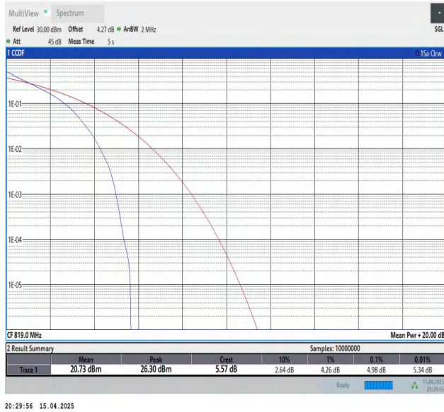
Band26(814-824)-1.4MHz-QPSK-26740-6RB#0-PASS
