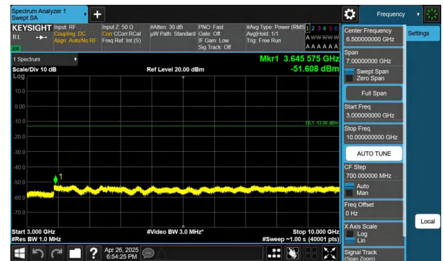
Band26(814-824)-1.4MHz-QPSK-26783-1RB#5-3000~10000-PAS
