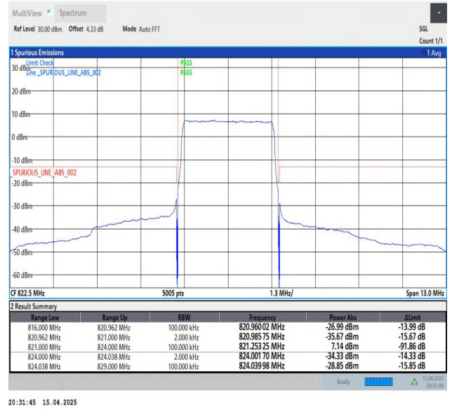
Band26(814-824)-3MHz-QPSK-26775-15RB#0-PASS
