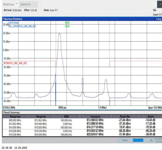
Band26(814-824)-5MHz-QPSK-26715-1RB#0-PASS
