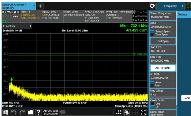
Band26(814-824)-1.4MHz-QPSK-26783-1RB#5-0.15~30-PASS
