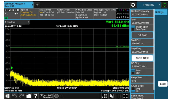
Band26(814-824)-1.4MHz-QPSK-26740-1RB#0-0.15~30-PASS
