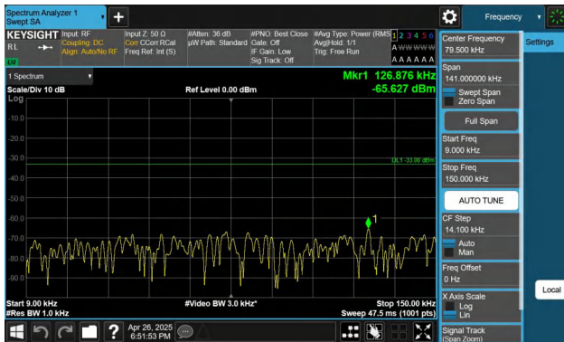
Band26(814-824)-1.4MHz-QPSK-26740-1RB#0-0.009~0.15-PASS
