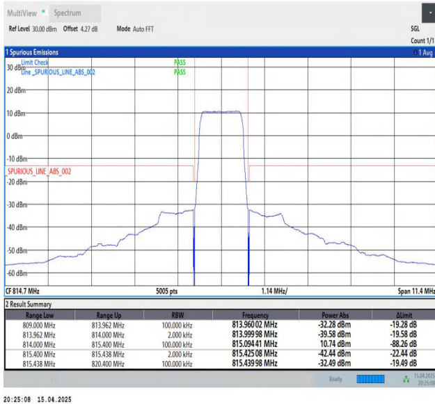
Band26(814-824)-1.4MHz-QPSK-26697-6RB#0-PASS
