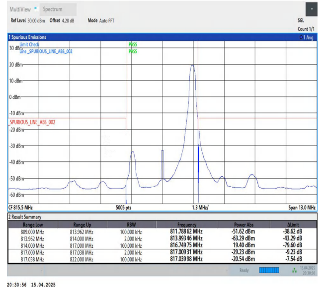
Band26(814-824)-3MHz-QPSK-26705-1RB#14-PASS
