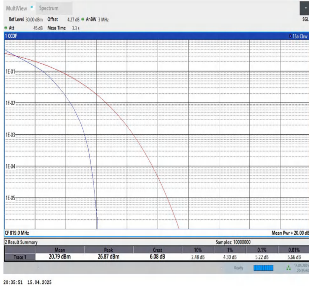
Band26(814-824)-3MHz-QPSK-26740-15RB#0-PASS
