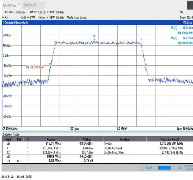
Band26(814-824)-5MHz-QPSK-26740-25RB#0-PASS
