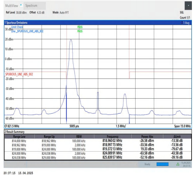
Band26(814-824)-5MHz-QPSK-26765-1RB#0-PASS
