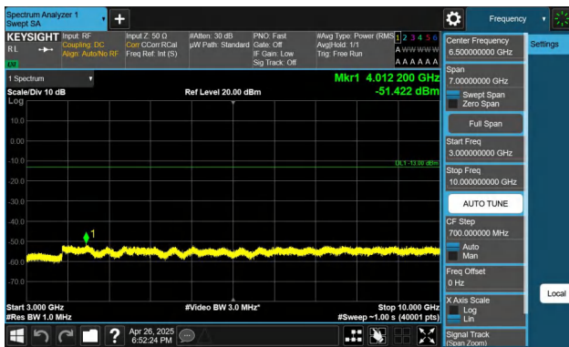
Band26(814-824)-1.4MHz-QPSK-26740-1RB#0-3000~10000-PAS
