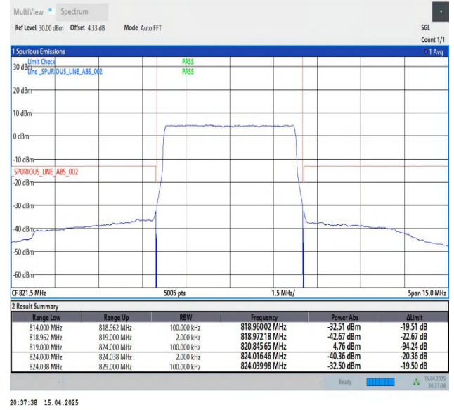
Band26(814-824)-5MHz-QPSK-26765-25RB#0-PASS
