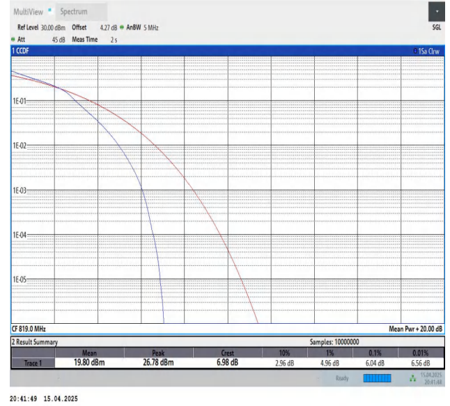
Band26(814-824)-5MHz-16QAM-26740-25RB#0-PASS
