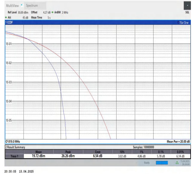
Band26(814-824)-1.4MHz-16QAM-26740-6RB#0-PASS
