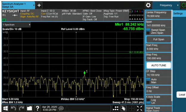
Band26(814-824)-1.4MHz-QPSK-26697-1RB#0-0.009~0.15-PASS
