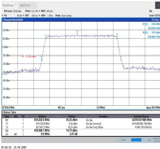
Band26(814-824)-10MHz-QPSK-26740-50RB#0-PASS
