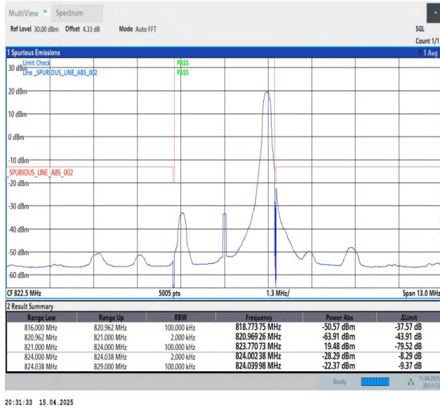
Band26(814-824)-3MHz-QPSK-26775-1RB#14-PASS
