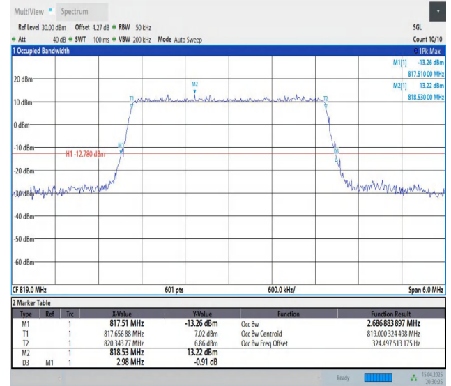
Band26(814-824)-3MHz-16QAM-26740-15RB#0-PASS
