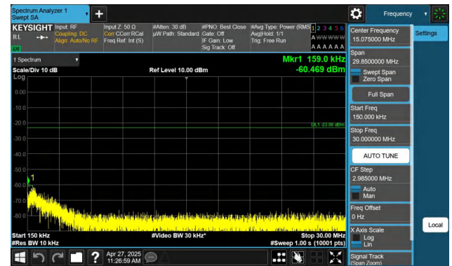
Band26(814-824)-1.4MHz-QPSK-26783-1RB#0-0.15~30-PASS
