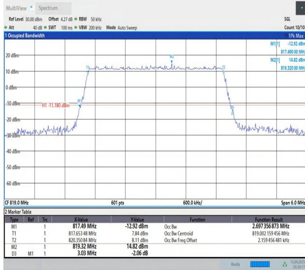
Band26(814-824)-3MHz-QPSK-26740-15RB#0-PASS
