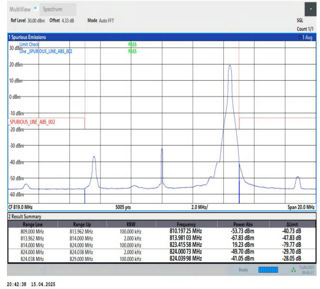
Band26(814-824)-10MHz-QPSK-26740-1RB#49-PASS
