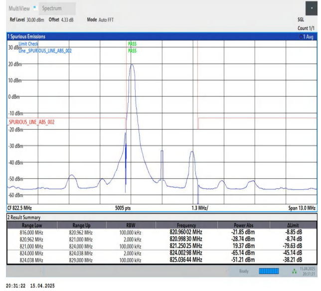
Band26(814-824)-3MHz-QPSK-26775-1RB#0-PASS
