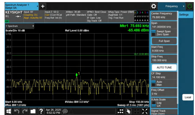
Band26(814-824)-1.4MHz-QPSK-26740-1RB#5-0.009~0.15-PASS
