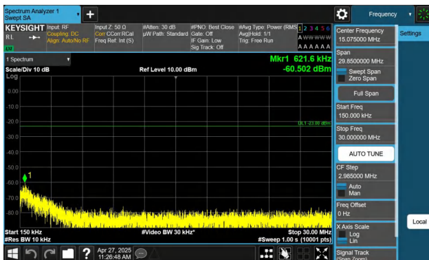
Band26(814-824)-1.4MHz-QPSK-26740-1RB#5-0.15~30-PASS
