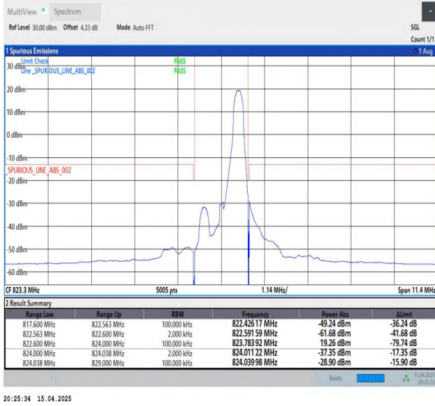
Band26(814-824)-1.4MHz-QPSK-26783-1RB#5-PASS
