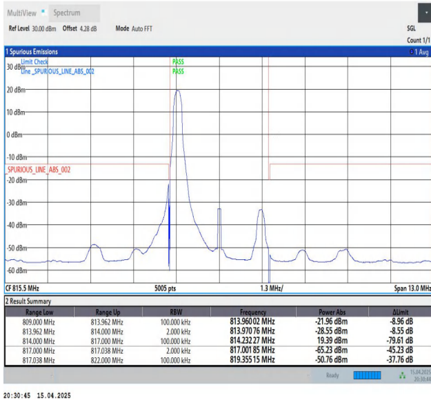
Band26(814-824)-3MHz-QPSK-26705-1RB#0-PASS
