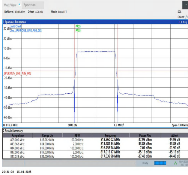
Band26(814-824)-3MHz-QPSK-26705-15RB#0-PASS
