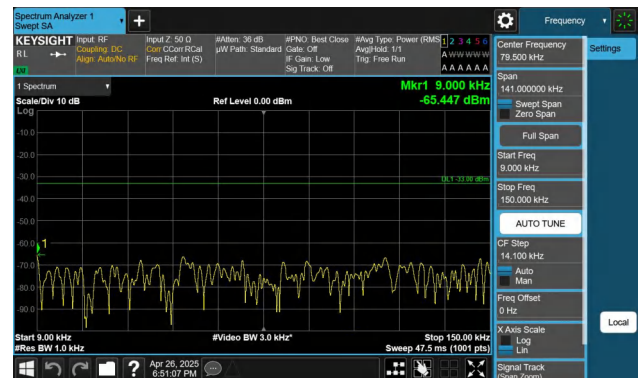
Band26(814-824)-1.4MHz-QPSK-26697-1RB#5-0.009~0.15-PASS
