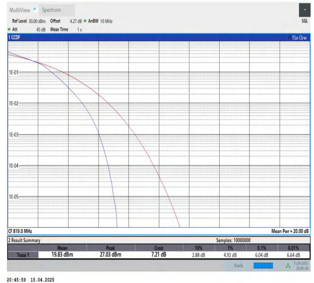
Band26(814-824)-10MHz-16QAM-26740-50RB#0-PASS
