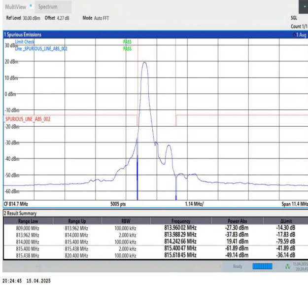
Band26(814-824)-1.4MHz-QPSK-26697-1RB#0-PASS
