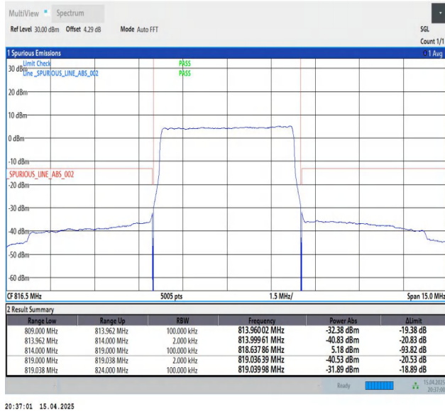
Band26(814-824)-5MHz-QPSK-26715-25RB#0-PASS
