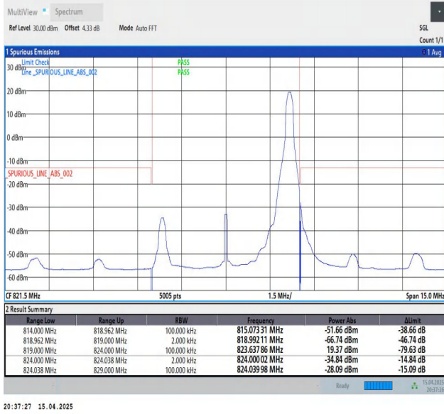
Band26(814-824)-5MHz-QPSK-26765-1RB#24-PASS
