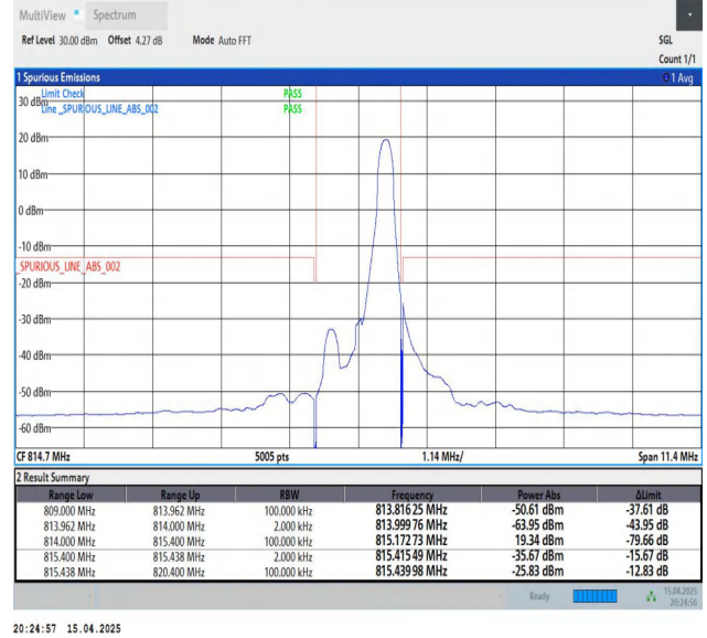
Band26(814-824)-1.4MHz-QPSK-26697-1RB#5-PASS
