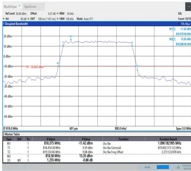
Band26(814-824)-1.4MHz-QPSK-26740-6RB#0-PASS
