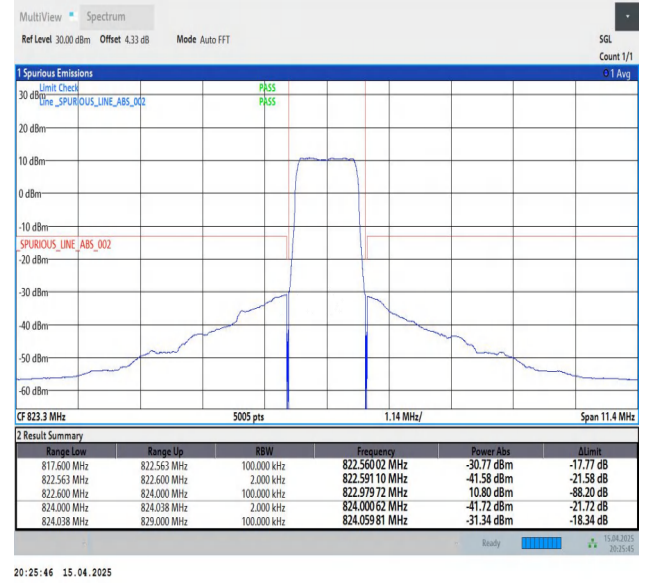
Band26(814-824)-1.4MHz-QPSK-26783-6RB#0-PASS
