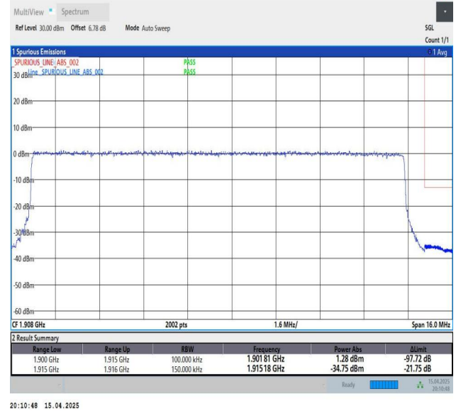
Band25-15MHz-QPSK-26615-75RB#0-PASS
