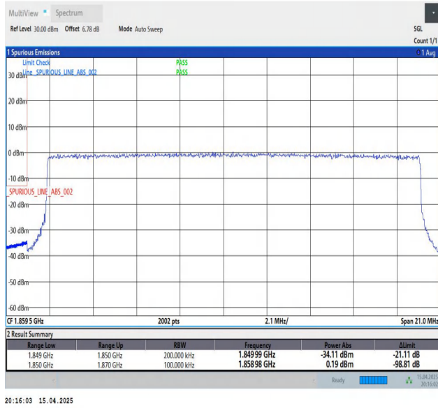
Band25-20MHz-QPSK-26140-100RB#0-PASS
