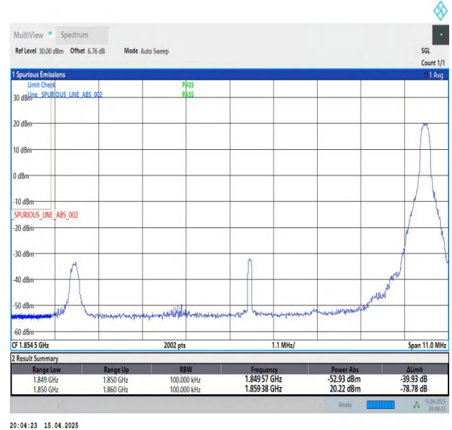
Band25-10MHz-QPSK-26090-1RB#49-PASS
