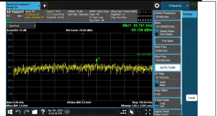
Band25-5MHz-QPSK-26065-1RB#24-0.009~0.15-PASS
