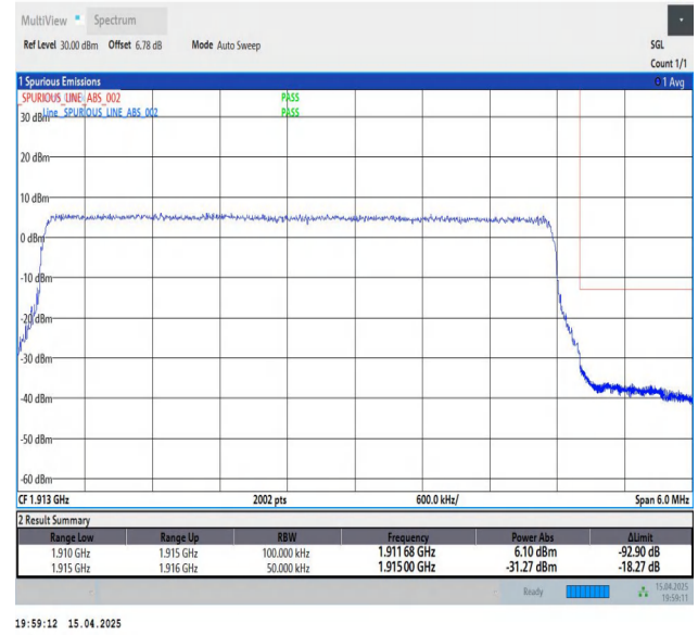
Band25-5MHz-QPSK-26665-25RB#0-PASS
