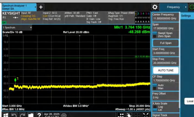
Band25-1.4MHz-QPSK-26365-1RB#0-3000~20000-PASS
