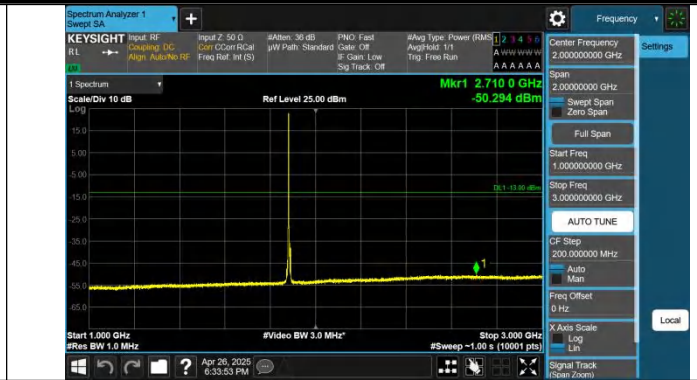
Band25-5MHz-QPSK-26365-1RB#0-1000~3000-PASS
