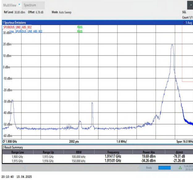
Band25-15MHz-QPSK-26615-1RB#74-PASS
