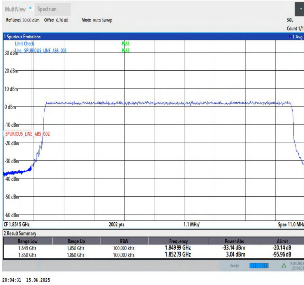
Band25-10MHz-QPSK-26090-50RB#0-PASS
