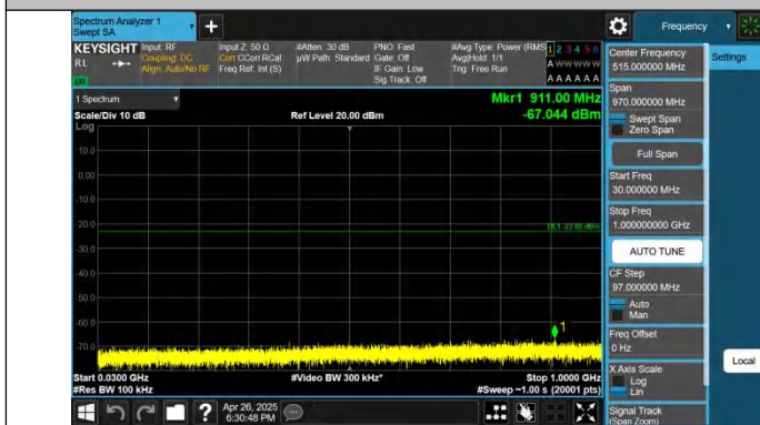
Band25-3MHz-QPSK-26675-1RB#0-30~1000-PASS
