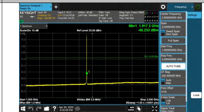
Band25-3MHz-QPSK-26675-1RB#0-1000~3000-PASS
