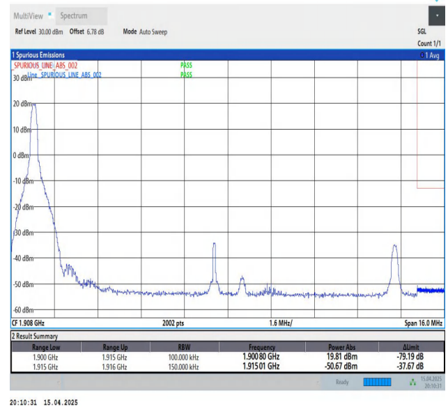
Band25-15MHz-QPSK-26615-1RB#0-PASS
