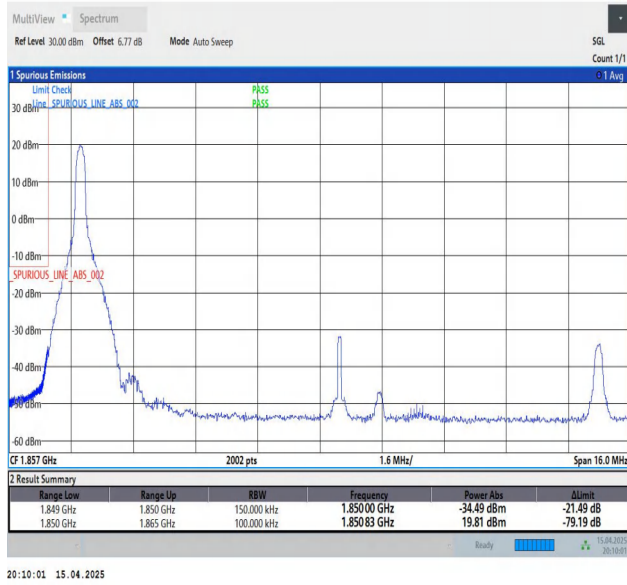
Band25-15MHz-QPSK-26115-1RB#0-PASS
