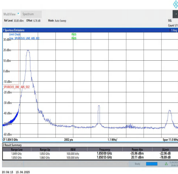
Band25-10MHz-QPSK-26090-1RB#0-PASS
