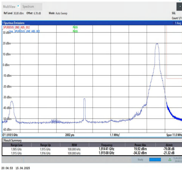
Band25-10MHz-QPSK-26640-1RB#49-PASS
