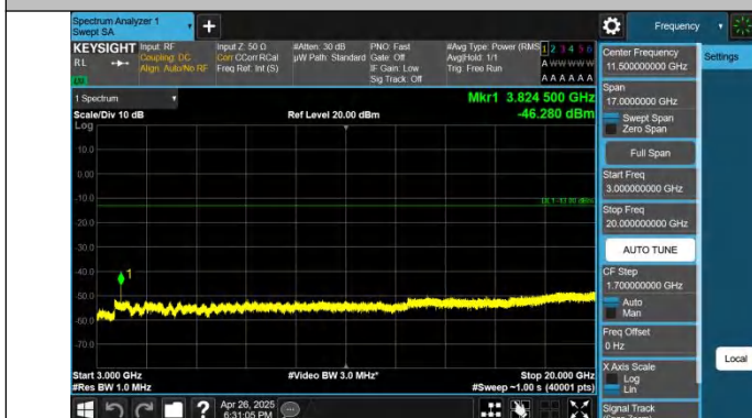
Band25-3MHz-QPSK-26675-1RB#0-3000~20000-PASS
