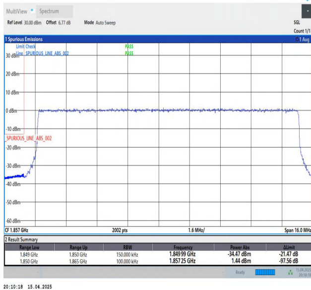
Band25-15MHz-QPSK-26115-75RB#0-PASS
