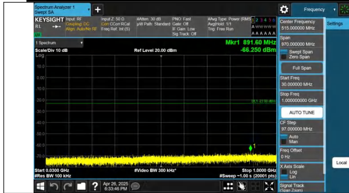
Band25-5MHz-QPSK-26365-1RB#0-30~1000-PASS
