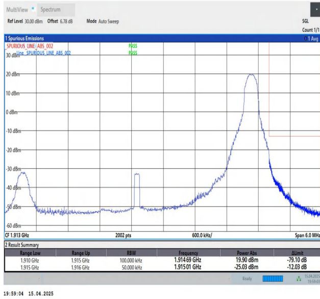
Band25-5MHz-QPSK-26665-1RB#24-PASS
