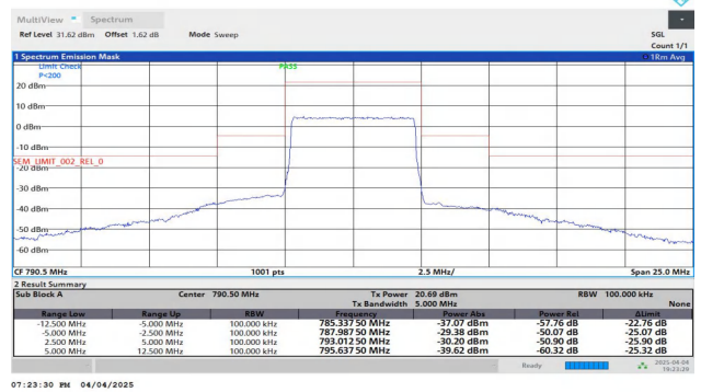
NTNV-Band14-5MHz-16QAM-23305-25RB#0--5.00--2.50-PASS
