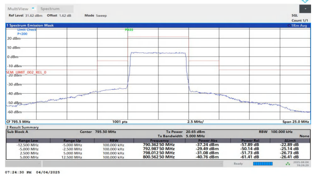
NTNV-Band14-5MHz-16QAM-23355-25RB#0-5.00-12.50-PASS
