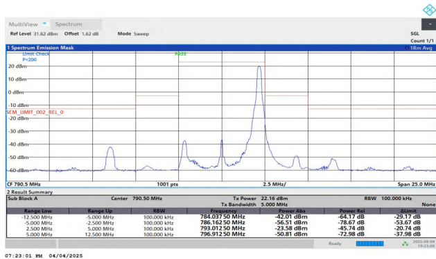
NTNV-Band14-5MHz-QPSK-23305-1RB#24--12.50--5.00-PASS
