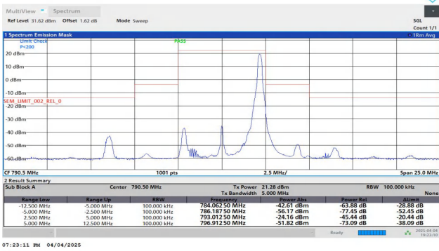
NTNV-Band14-5MHz-16QAM-23305-1RB#24-2.50-5.00-PASS
