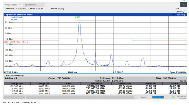
NTNV-Band14-5MHz-QPSK-23355-1RB#0--5.00--2.50-PASS
