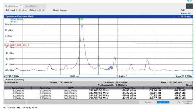
NTNV-Band14-5MHz-16QAM-23305-1RB#0-5.00-12.50-PASS
