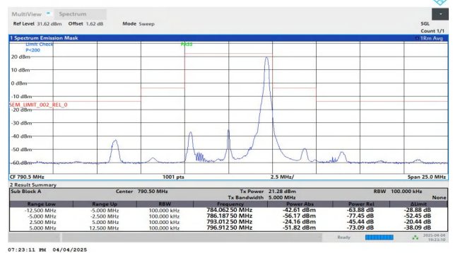
NTNV-Band14-5MHz-16QAM-23305-1RB#24--5.00--2.50-PASS
