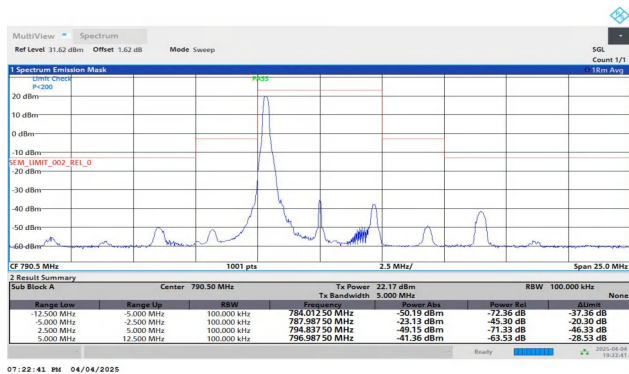
NTNV-Band14-5MHz-QPSK-23305-1RB#0-2.50-5.00-PASS
