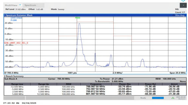
NTNV-Band14-5MHz-16QAM-23355-1RB#0-5.00-12.50-PASS
