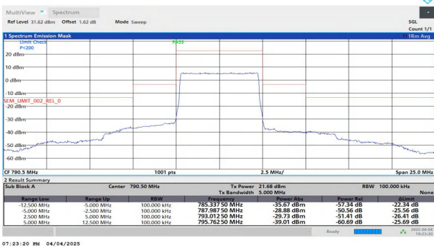
NTNV-Band14-5MHz-QPSK-23305-25RB#0-2.50-5.00-PASS
