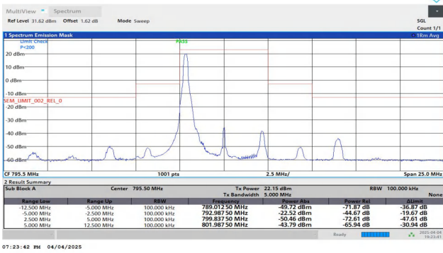
NTNV-Band14-5MHz-QPSK-23355-1RB#0--12.50--5.00-PASS
