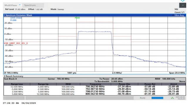
NTNV-Band14-5MHz-16QAM-23355-25RB#0--5.00--2.50-PASS
