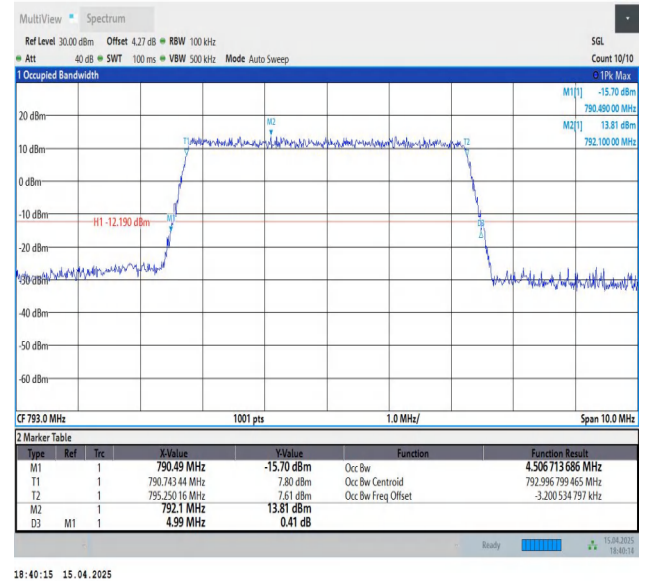
Band14-5MHz-16QAM-23330-25RB#0-PASS
