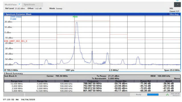
NTNV-Band14-5MHz-16QAM-23355-1RB#0--5.00--2.50-PASS
