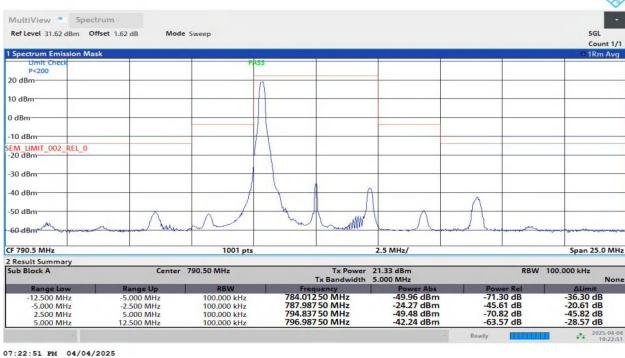
NTNV-Band14-5MHz-16QAM-23305-1RB#0-2.50-5.00-PASS
