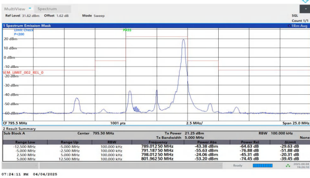
NTNV-Band14-5MHz-16QAM-23355-1RB#24--12.50--5.00-PASS
