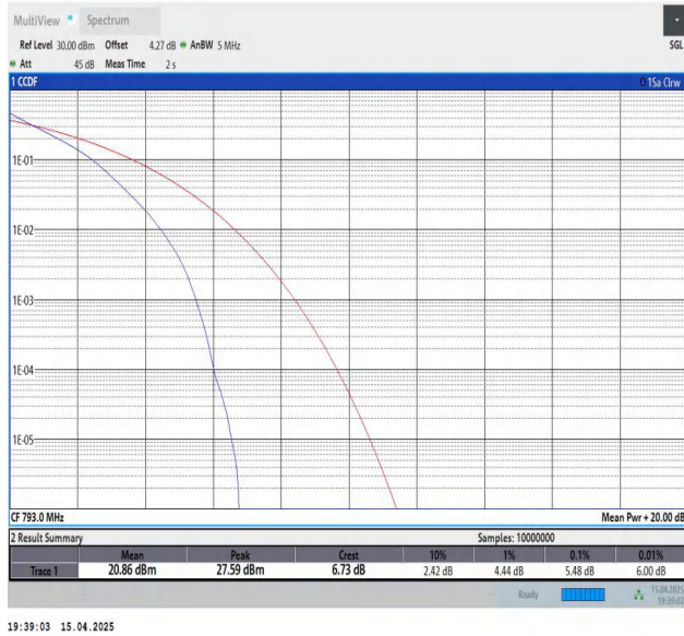
Band14-5MHz-QPSK-23330-25RB#0-PASS
