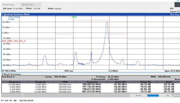
NTNV-Band14-5MHz-QPSK-23355-1RB#24-2.50-5.00-PASS
