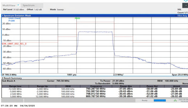
NTNV-Band14-5MHz-QPSK-23355-25RB#0-2.50-5.00-PASS
