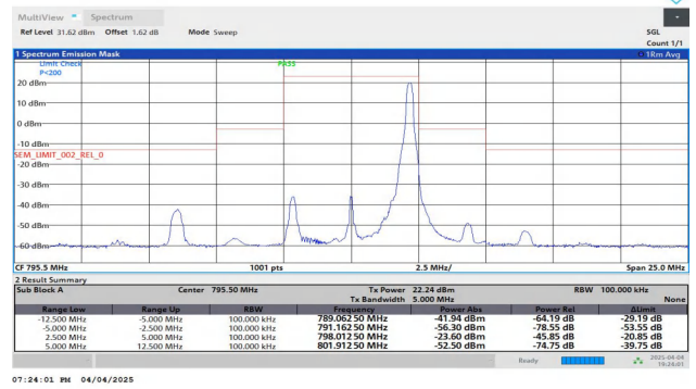
NTNV-Band14-5MHz-QPSK-23355-1RB#24-5.00-12.50-PASS
