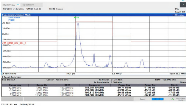
NTNV-Band14-5MHz-16QAM-23355-1RB#0--12.50--5.00-PASS
