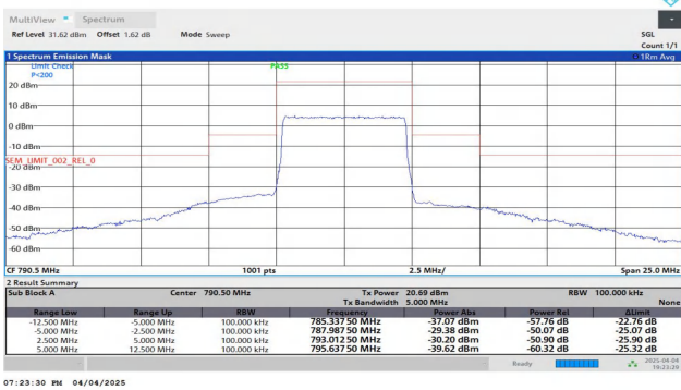
NTNV-Band14-5MHz-16QAM-23305-25RB#0--12.50--5.00-PASS
