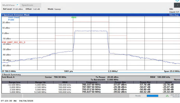
NTNV-Band14-5MHz-16QAM-23305-25RB#0-2.50-5.00-PASS
