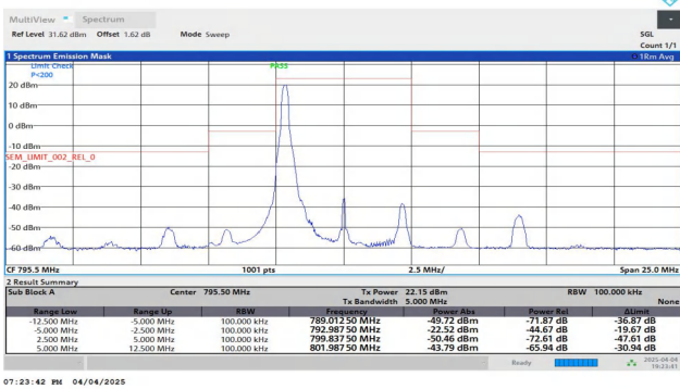
NTNV-Band14-5MHz-QPSK-23355-1RB#0-2.50-5.00-PASS
