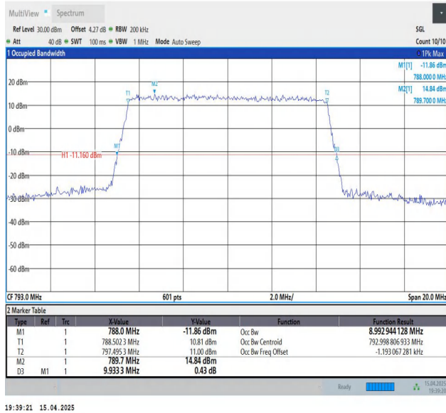
Band14-10MHz-QPSK-23330-50RB#0-PASS
