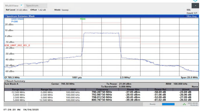
NTNV-Band14-5MHz-QPSK-23355-25RB#0-5.00-12.50-PASS
