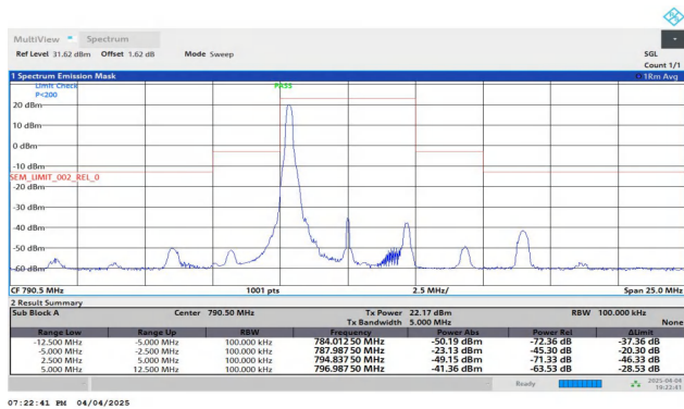
NTNV-Band14-5MHz-QPSK-23305-1RB#0--12.50--5.00-PASS
