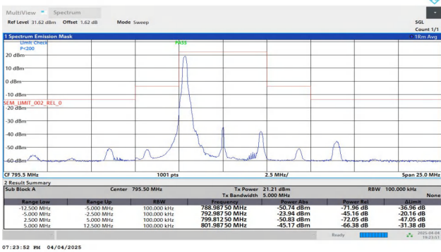
NTNV-Band14-5MHz-16QAM-23355-1RB#0-2.50-5.00-PASS
