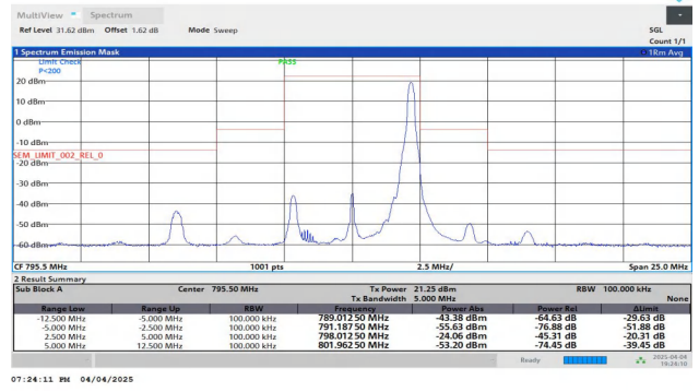
NTNV-Band14-5MHz-16QAM-23355-1RB#24-5.00-12.50-PASS
