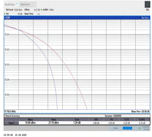
Band14-5MHz-16QAM-23330-25RB#0-PASS
