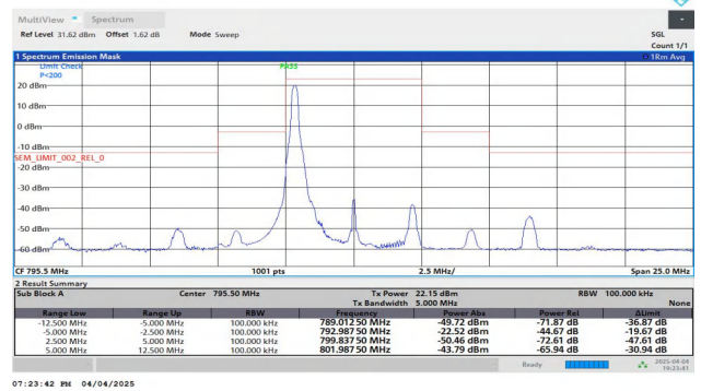
NTNV-Band14-5MHz-QPSK-23355-1RB#0-5.00-12.50-PASS
