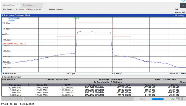
NTNV-Band14-5MHz-16QAM-23355-25RB#0--12.50--5.00-PASS
