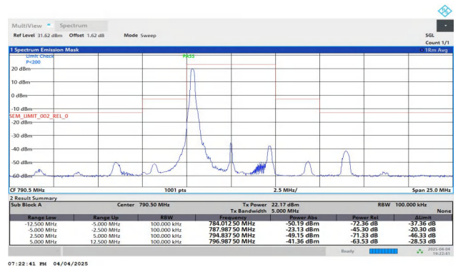
NTNV-Band14-5MHz-QPSK-23305-1RB#0-5.00-12.50-PASS
