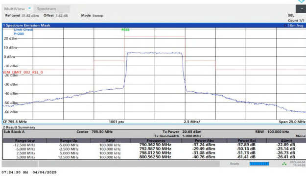
NTNV-Band14-5MHz-16QAM-23355-25RB#0-2.50-5.00-PASS
