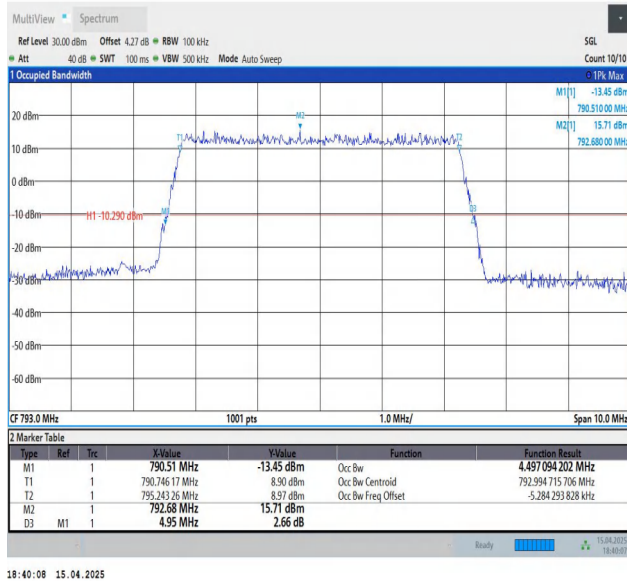
Band14-5MHz-QPSK-23330-25RB#0-PASS
