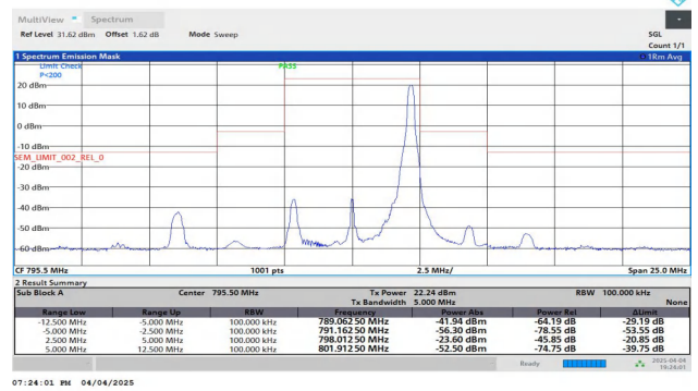
NTNV-Band14-5MHz-QPSK-23355-1RB#24--5.00--2.50-PASS
