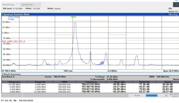
NTNV-Band14-5MHz-16QAM-23305-1RB#0--12.50--5.00-PASS
