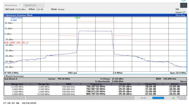
NTNV-Band14-5MHz-QPSK-23355-25RB#0--5.00--2.50-PASS
