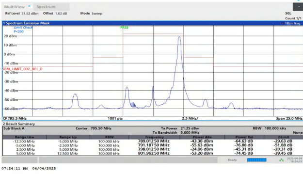
NTNV-Band14-5MHz-16QAM-23355-1RB#24-2.50-5.00-PASS
