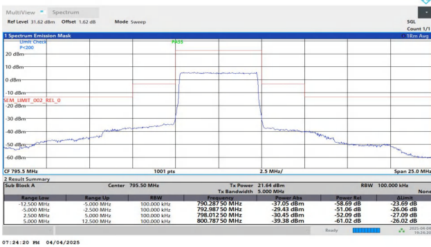
NTNV-Band14-5MHz-QPSK-23355-25RB#0--12.50--5.00-PASS
