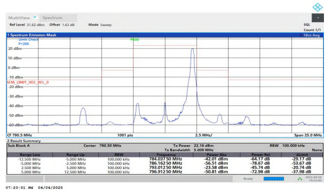
NTNV-Band14-5MHz-QPSK-23305-1RB#24--5.00--2.50-PASS
