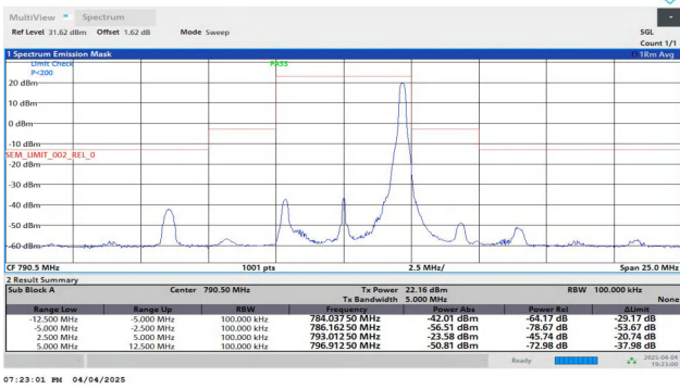
NTNV-Band14-5MHz-QPSK-23305-1RB#24-2.50-5.00-PASS
