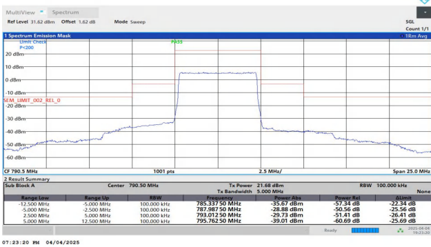
NTNV-Band14-5MHz-QPSK-23305-25RB#0--12.50--5.00-PASS
