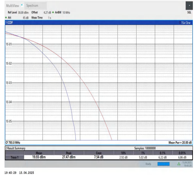
Band14-10MHz-16QAM-23330-50RB#0-PASS
