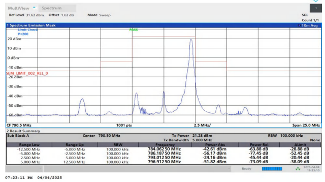
NTNV-Band14-5MHz-16QAM-23305-1RB#24-5.00-12.50-PASS
