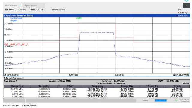
NTNV-Band14-5MHz-16QAM-23305-25RB#0-5.00-12.50-PASS
