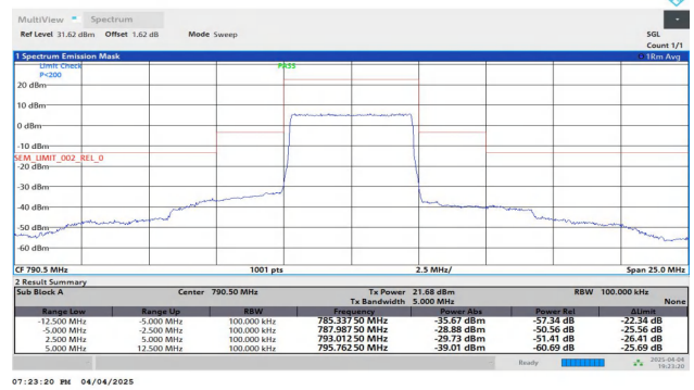
NTNV-Band14-5MHz-QPSK-23305-25RB#0-5.00-12.50-PASS
