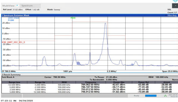
NTNV-Band14-5MHz-16QAM-23305-1RB#24--12.50--5.00-PASS
