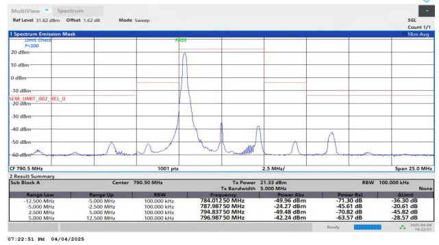
NTNV-Band14-5MHz-16QAM-23305-1RB#0--5.00--2.50-PASS
