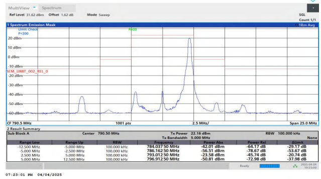
NTNV-Band14-5MHz-QPSK-23305-1RB#24-5.00-12.50-PASS
