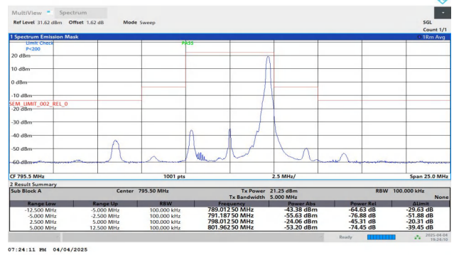
NTNV-Band14-5MHz-16QAM-23355-1RB#24--5.00--2.50-PASS
