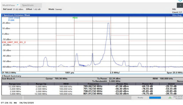
NTNV-Band14-5MHz-QPSK-23355-1RB#24--12.50--5.00-PASS
