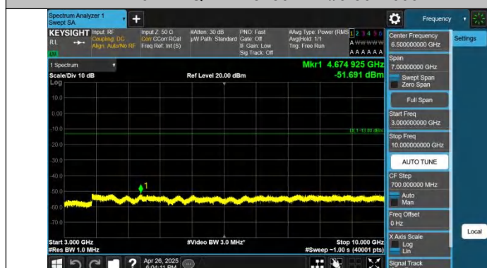
Band12-10MHz-QPSK-23130-1RB#0-3000~10000-PASS
