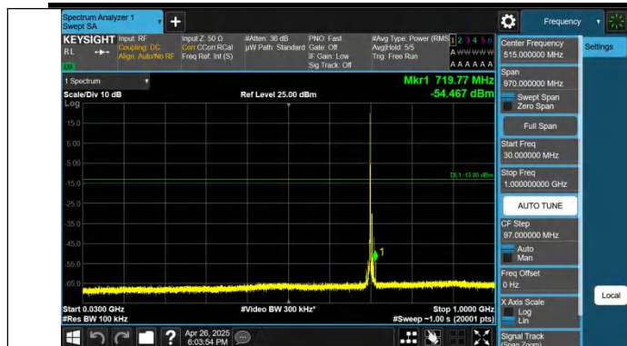
Band12-10MHz-QPSK-23130-1RB#0-30~1000-PASS
