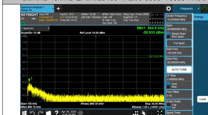
Band12-10MHz-QPSK-23130-1RB#49-0.15~30-PASS
