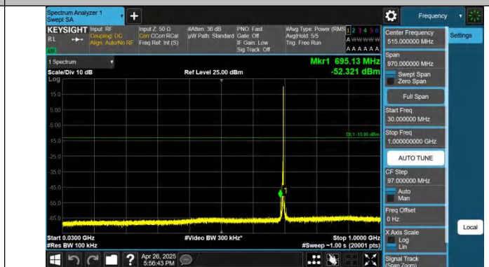
Band12-5MHz-QPSK-23035-1RB#24-30~1000-PASS
