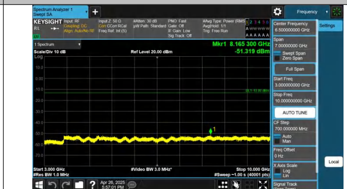
Band12-5MHz-QPSK-23035-1RB#24-3000~10000-PASS
