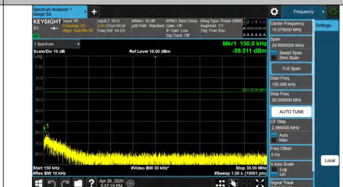
Band12-5MHz-QPSK-23095-1RB#0-0.15~30-PASS
