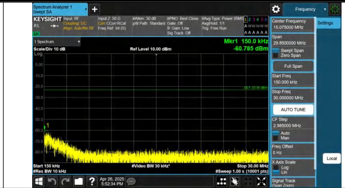
Band12-3MHz-QPSK-23095-1RB#0-0.15~30-PASS
