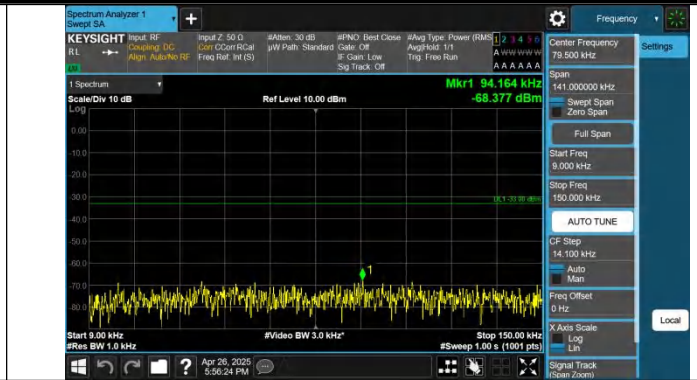
Band12-5MHz-QPSK-23035-1RB#24-0.009~0.15-PASS
