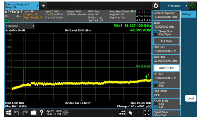
Band7-20MHz-QPSK-21350-1RB#0-1000~20000-PASS
