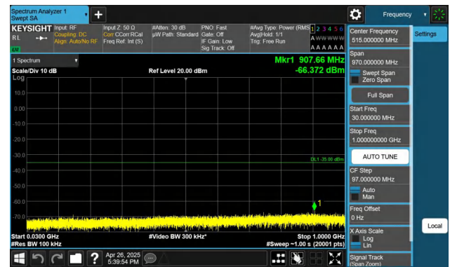
Band7-15MHz-QPSK-21375-1RB#74-30~1000-PASS
