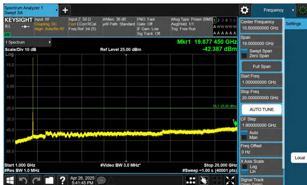
Band7-20MHz-QPSK-20850-1RB#99-1000~20000-PASS
