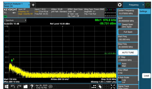
Band7-20MHz-QPSK-21100-1RB#0-0.15~30-PASS
