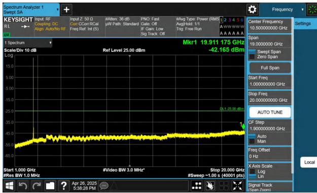
Band7-15MHz-QPSK-21100-1RB#74-1000~20000-PASS
