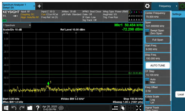
Band7-20MHz-QPSK-21100-1RB#0-0.009~0.15-PASS
