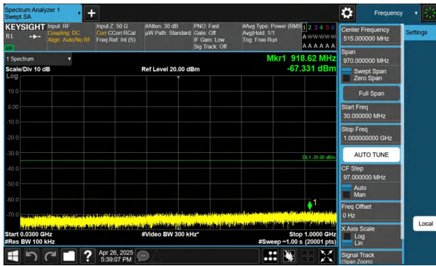
Band7-15MHz-QPSK-21375-1RB#0-30~1000-PASS
