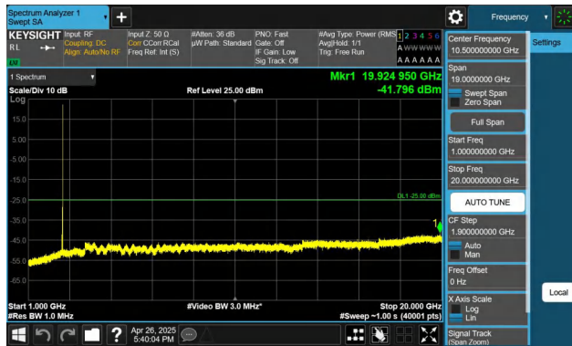
Band7-15MHz-QPSK-21375-1RB#74-1000~20000-PASS
