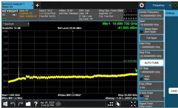
Band7-20MHz-QPSK-21100-1RB#99-1000~20000-PASS
