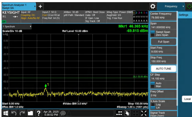
Band7-15MHz-QPSK-21375-1RB#0-0.009~0.15-PASS
