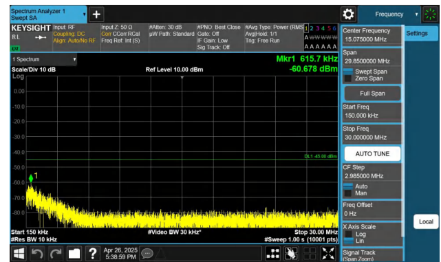
Band7-15MHz-QPSK-21375-1RB#0-0.15~30-PASS
