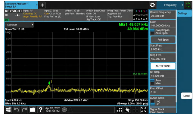
Band7-15MHz-QPSK-21375-1RB#74-0.009~0.15-PASS
