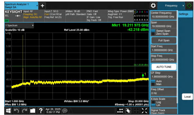
Band7-15MHz-QPSK-21375-1RB#0-1000~20000-PASS
