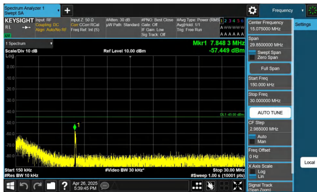
Band7-15MHz-QPSK-21375-1RB#74-0.15~30-PASS
