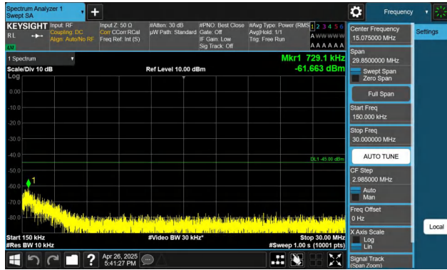
Band7-20MHz-QPSK-20850-1RB#99-0.15~30-PASS
