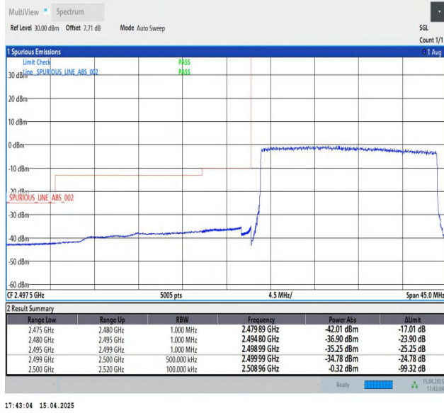
Band7-20MHz-QPSK-20850-100RB#0-PASS
