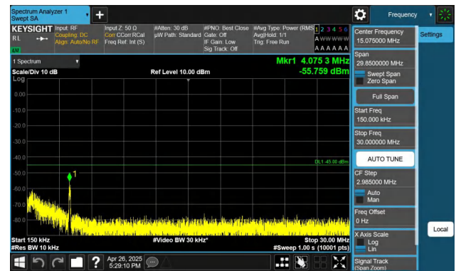
Band7-5MHz-QPSK-21425-1RB#0-0.15~30-PASS
