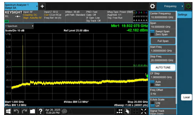
Band7-5MHz-QPSK-21425-1RB#0-1000~20000-PASS
