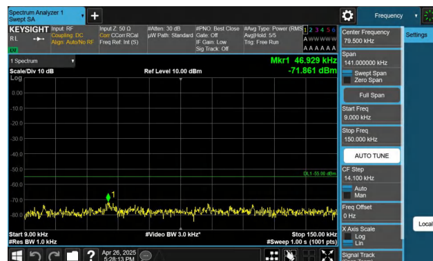
Band7-5MHz-QPSK-21100-1RB#24-0.009~0.15-PASS
