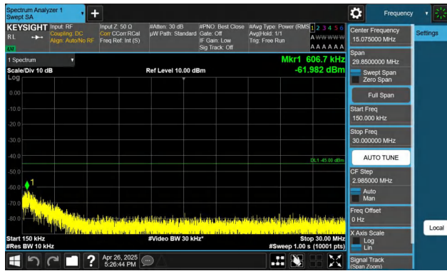
Band7-5MHz-QPSK-20775-1RB#24-0.15~30-PASS
