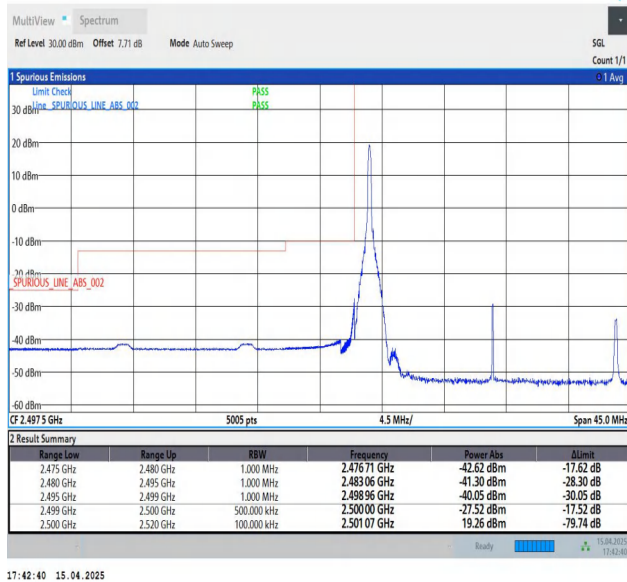
Band7-20MHz-QPSK-20850-1RB#0-PASS
