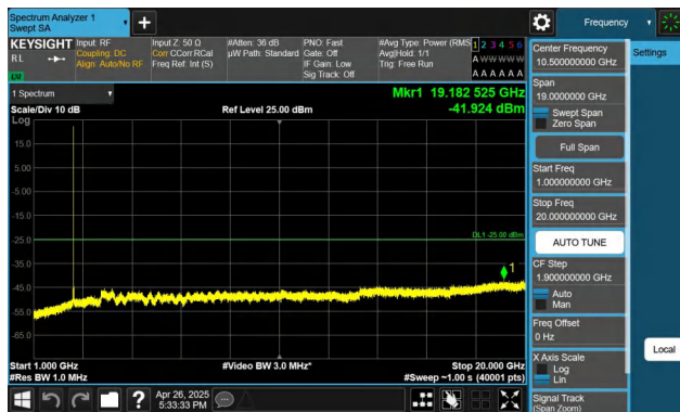
Band7-10MHz-QPSK-21100-1RB#49-1000~20000-PASS
