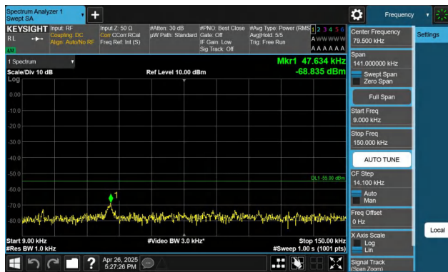
Band7-5MHz-QPSK-21100-1RB#0-0.009~0.15-PASS
