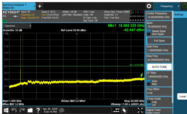
Band7-5MHz-QPSK-21425-1RB#24-1000~20000-PASS
