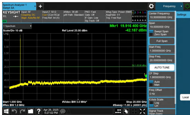
Band7-5MHz-QPSK-20775-1RB#24-1000~20000-PASS
