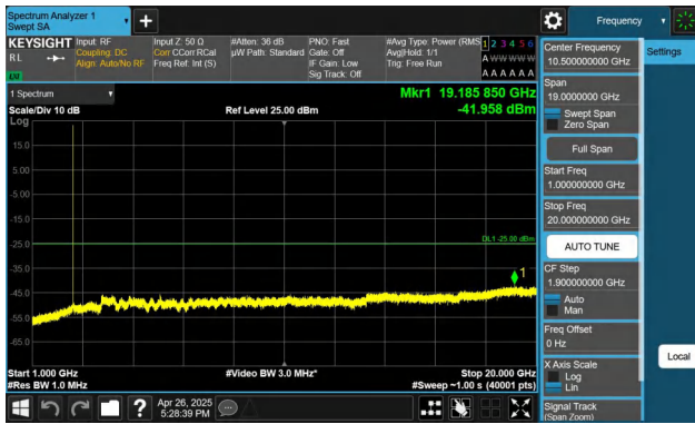
Band7-5MHz-QPSK-21100-1RB#24-1000~20000-PASS
