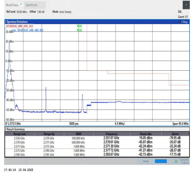
Band7-20MHz-QPSK-21350-1RB#0-PASS
