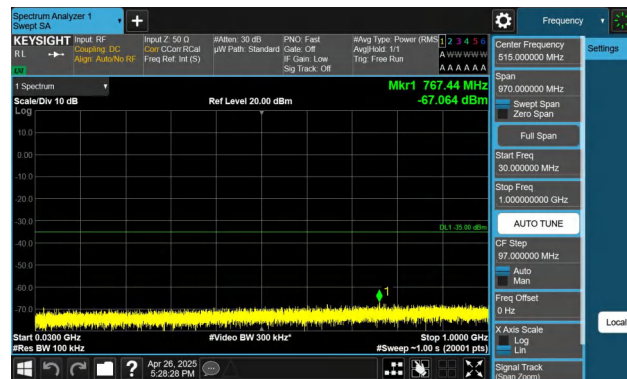
Band7-5MHz-QPSK-21100-1RB#24-30~1000-PASS
