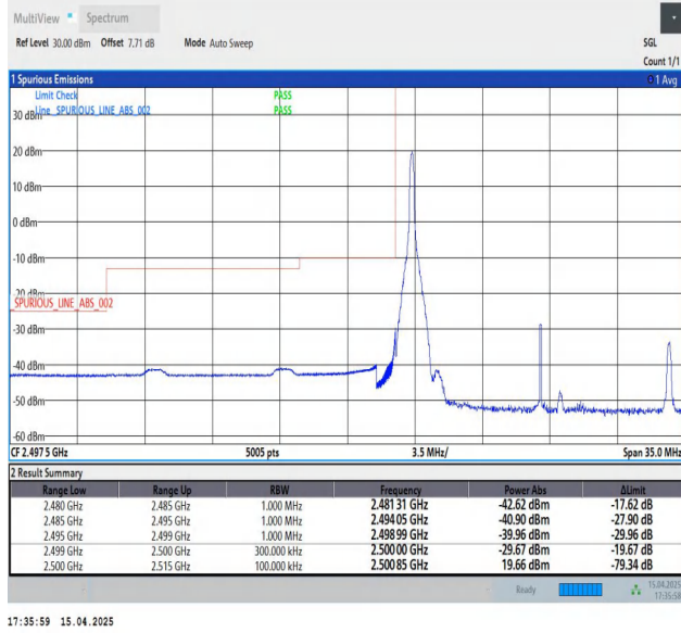
Band7-15MHz-QPSK-20825-1RB#0-PASS
