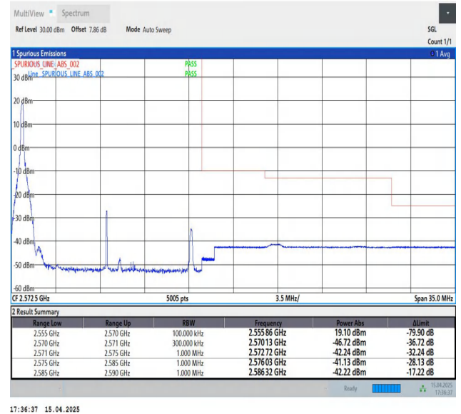
Band7-15MHz-QPSK-21375-1RB#0-PASS
