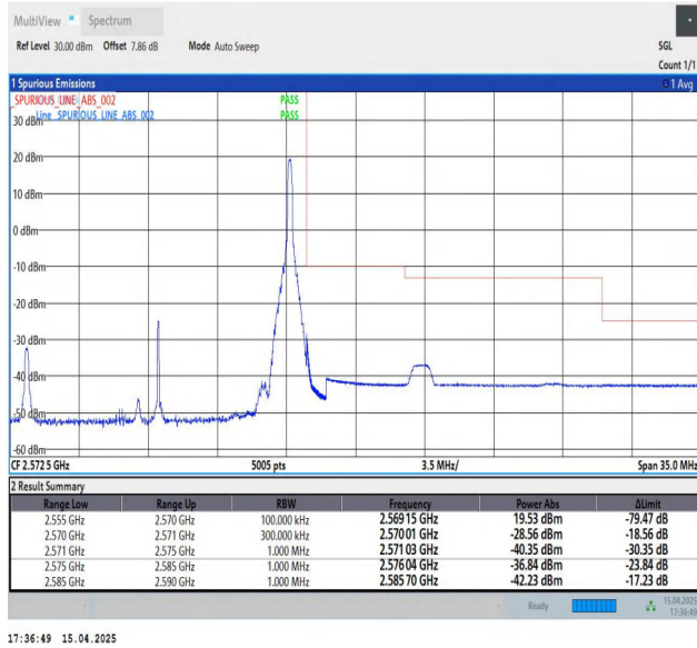
Band7-15MHz-QPSK-21375-1RB#74-PASS
