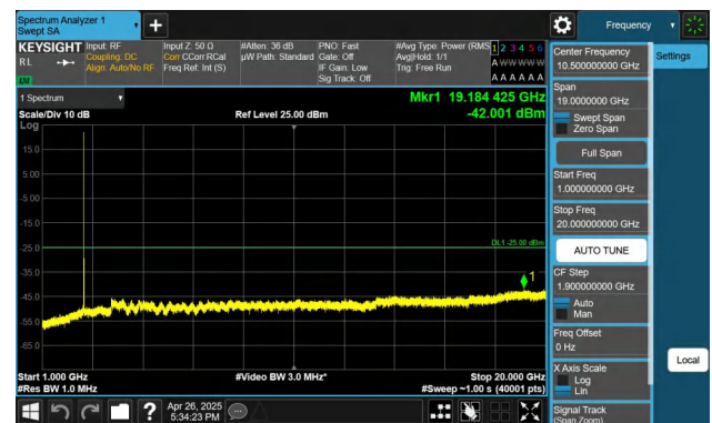
Band7-10MHz-QPSK-21400-1RB#0-1000~20000-PASS
