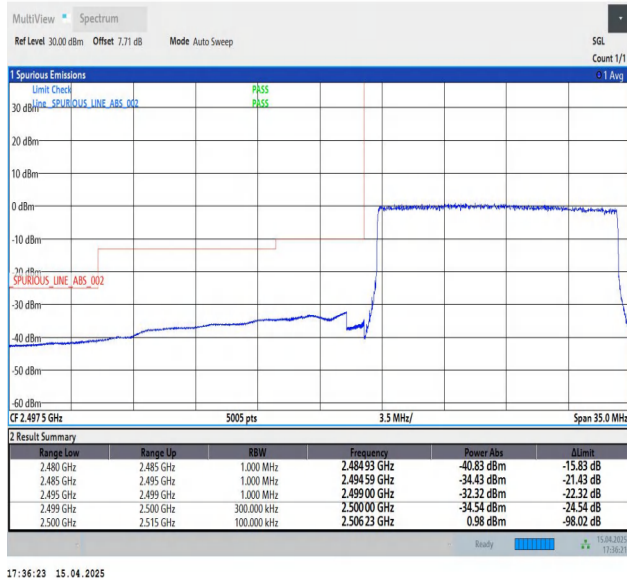
Band7-15MHz-QPSK-20825-75RB#0-PASS
