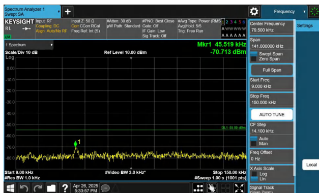
Band7-10MHz-QPSK-21400-1RB#0-0.009~0.15-PASS
