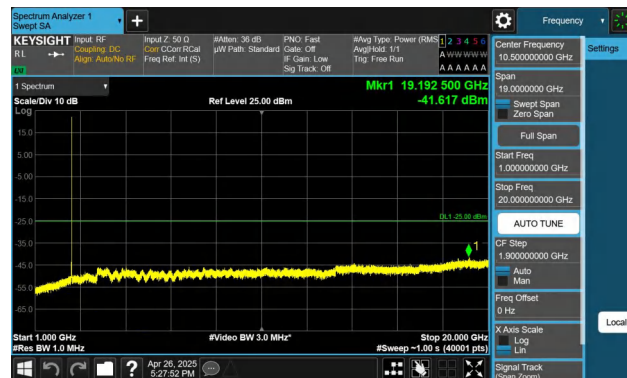
Band7-5MHz-QPSK-21100-1RB#0-1000~20000-PASS
