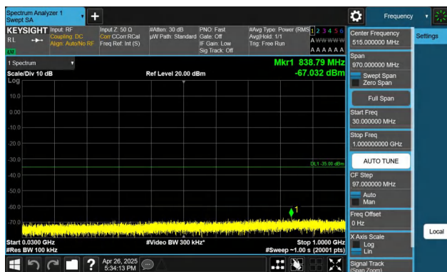
Band7-10MHz-QPSK-21400-1RB#0-30~1000-PASS
