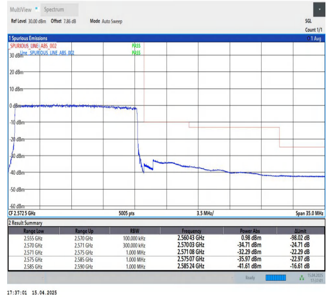
Band7-15MHz-QPSK-21375-75RB#0-PASS
